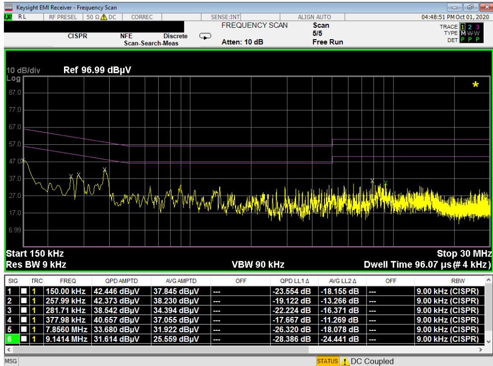
Plot 7-53. Line-Conducted Test Plot (N) with WCP
