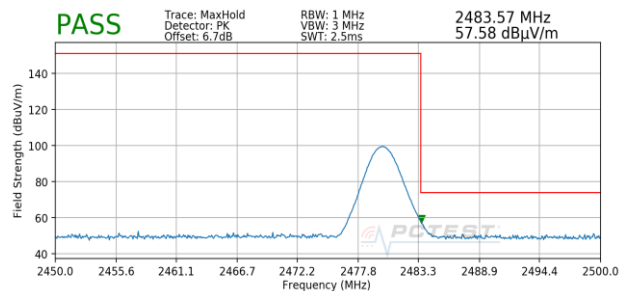
Plot 7-48. Radiated Restricted Upper Band Edge Measurement with WCP (Peak)
