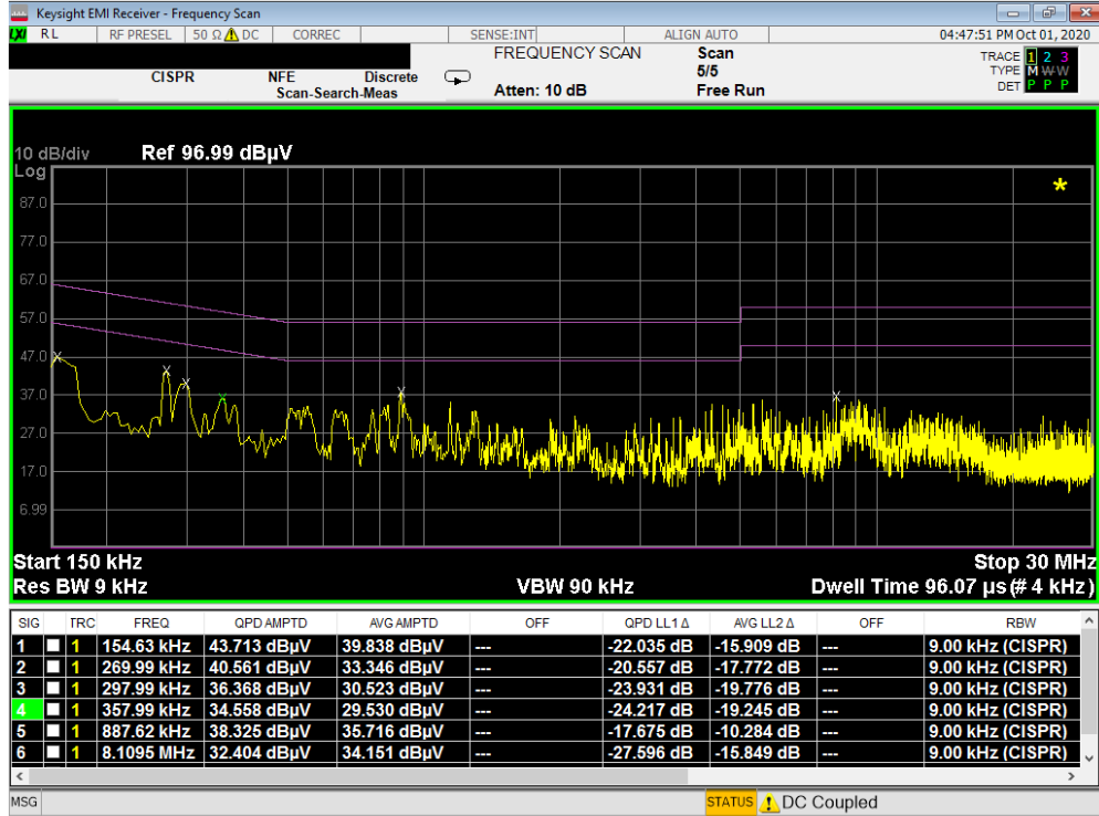
Plot 7-52. Line-Conducted Test Plot (L1) with WCP
