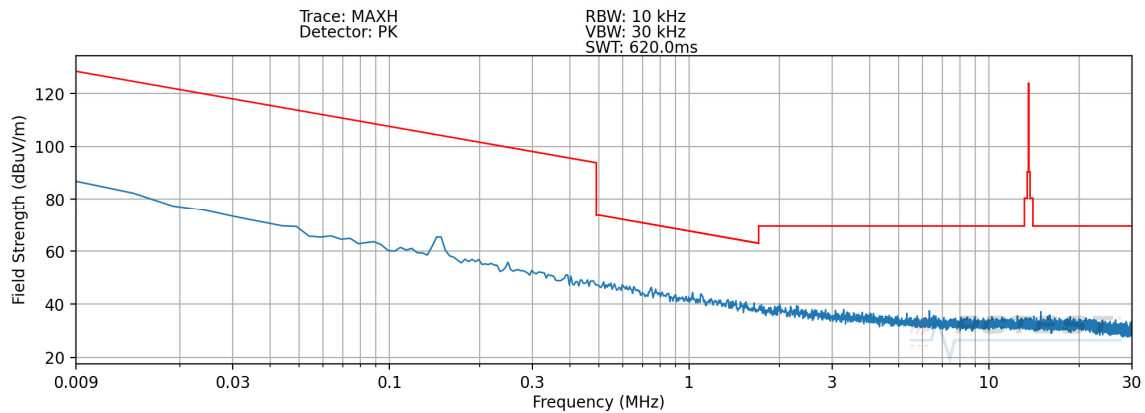
Plot 7-3. Radiated Spurious Plot 9kHz – 30MHz (Pol. Z – Device to Device WPT)
