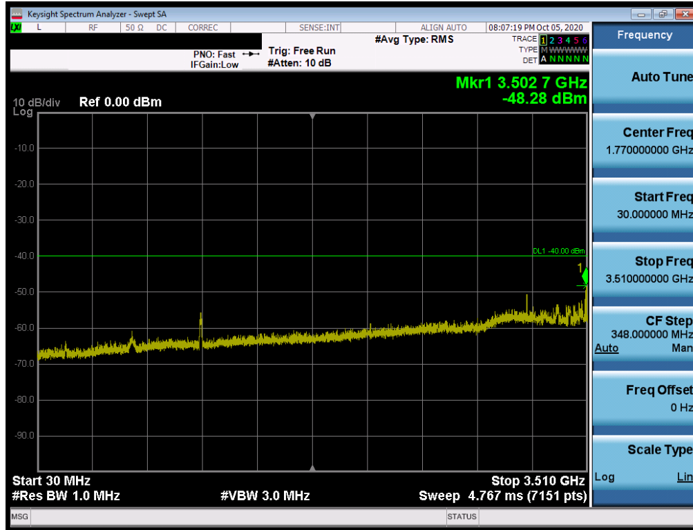
Plot 7-37. Conducted Spurious Plot (LTE Band 48 - 20MHz QPSK - RB Size 1, RB Offset 0 - Mid Channel)
