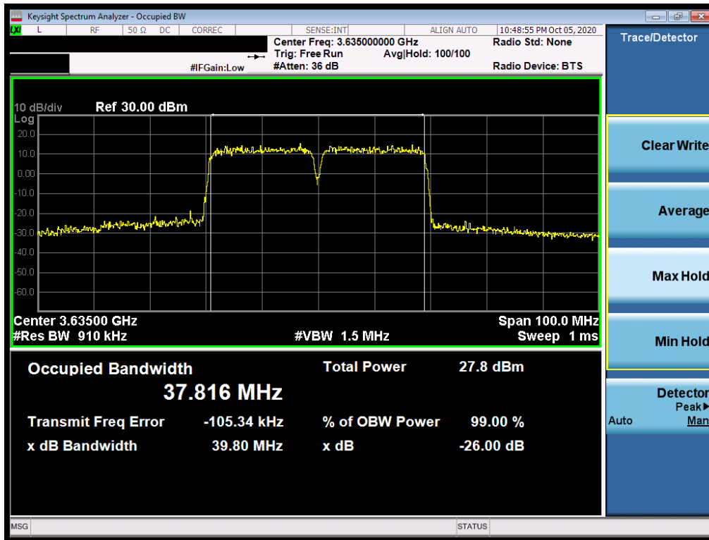
Plot 7-19. Occupied Bandwidth Plot (ULCA - 40.0MHz 64-QAM - Full RB Configuration)
