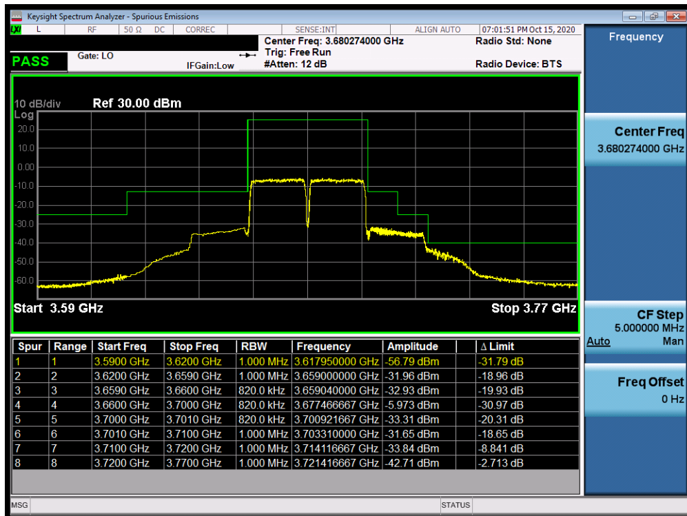
Plot 7-67. Upper Band Edge Plot (Band 48 QPSK – PCC:20 MHz SCC:20 MHz – Full RB)
