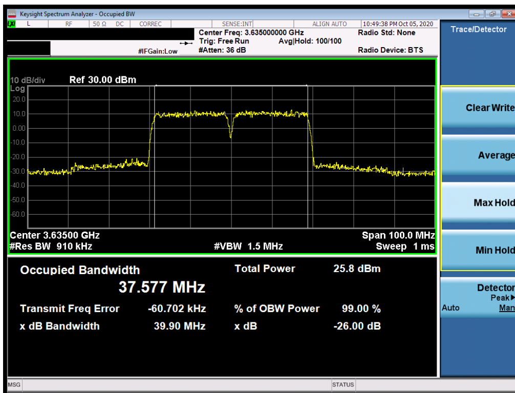
Plot 7-20. Occupied Bandwidth Plot (ULCA - 40.0MHz 256-QAM - Full RB Configuration)
