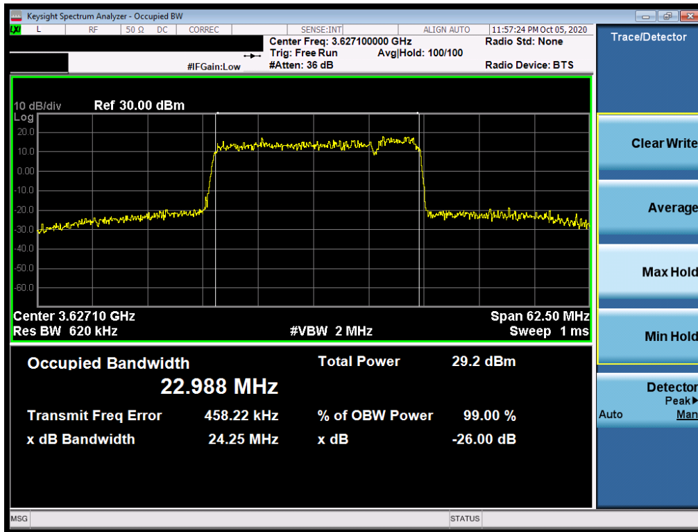
Plot 7-29. Occupied Bandwidth Plot (ULCA - 25.0MHz QPSK - Full RB Configuration)
