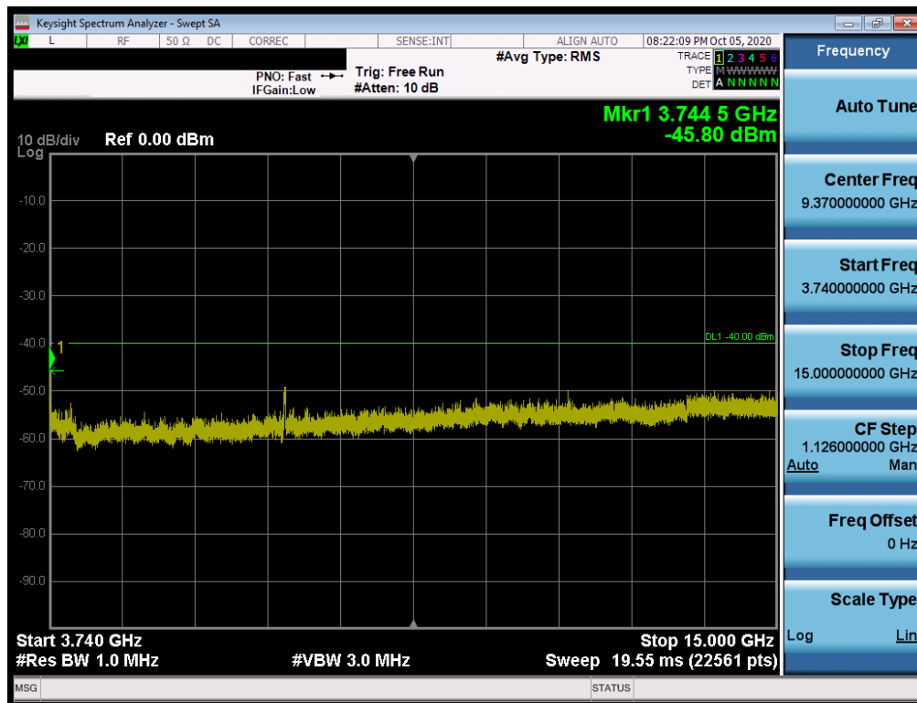
Plot 7-42. Conducted Spurious Plot (LTE Band 48 - 20MHz QPSK - RB Size 1, RB Offset 0 - High Channel)
