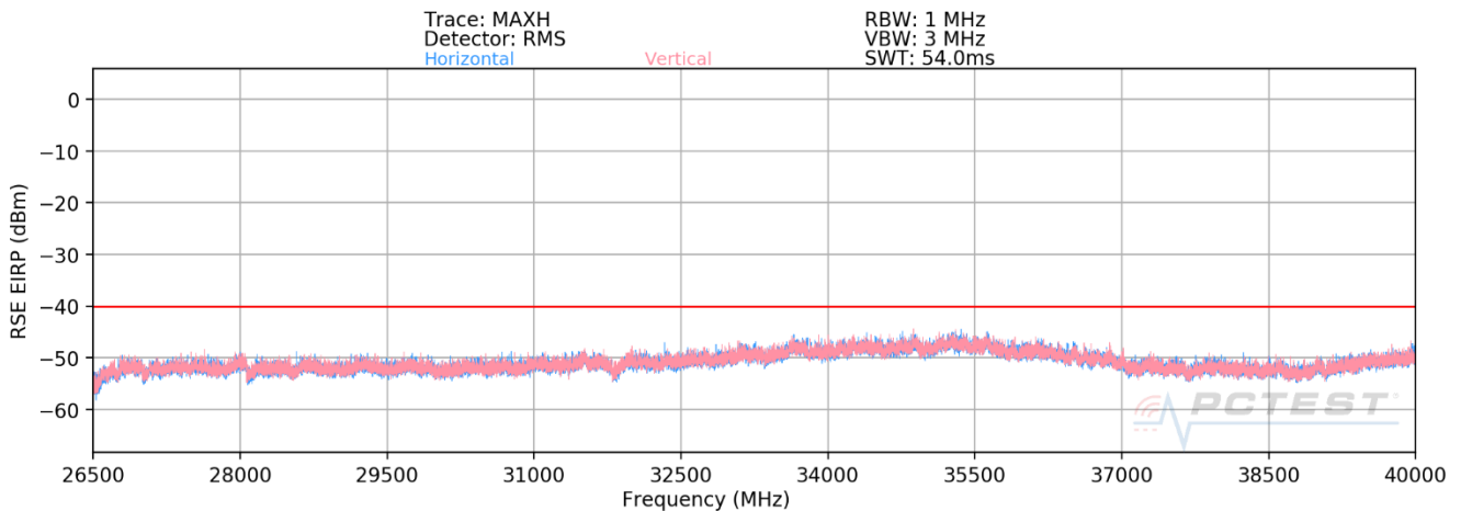
Plot 7-70. Radiated Spurious Plot 26.5 - 40GHz (Band 48)
