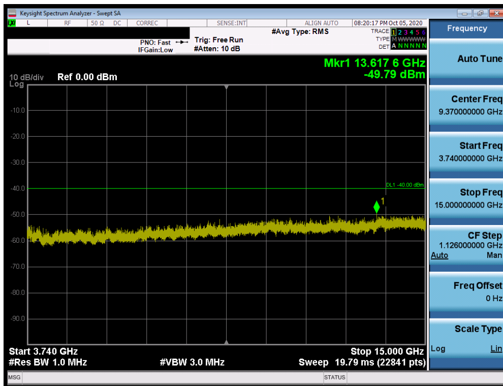
Plot 7-34. Conducted Spurious Plot (LTE Band 48 - 20MHz QPSK - RB Size 1, RB Offset 0 - Low Channel)
