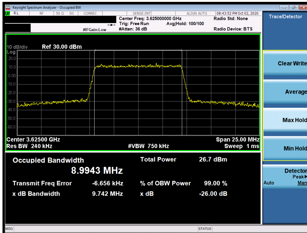
Plot 7-12. Occupied Bandwidth Plot (LTE Band 48 - 10.0MHz 256-QAM - Full RB Configuration)
