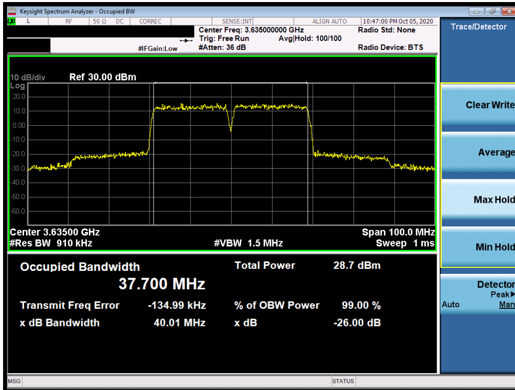
Plot 7-17. Occupied Bandwidth Plot (ULCA - 40.0MHz QPSK - Full RB Configuration)
