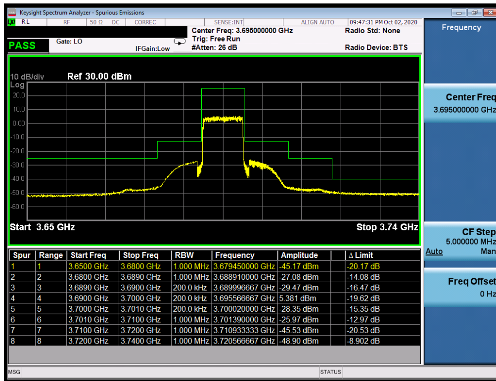
Plot 7-50. Upper ACP Plot (LTE Band 48 - 10MHz QPSK – Full RB Configuration)
