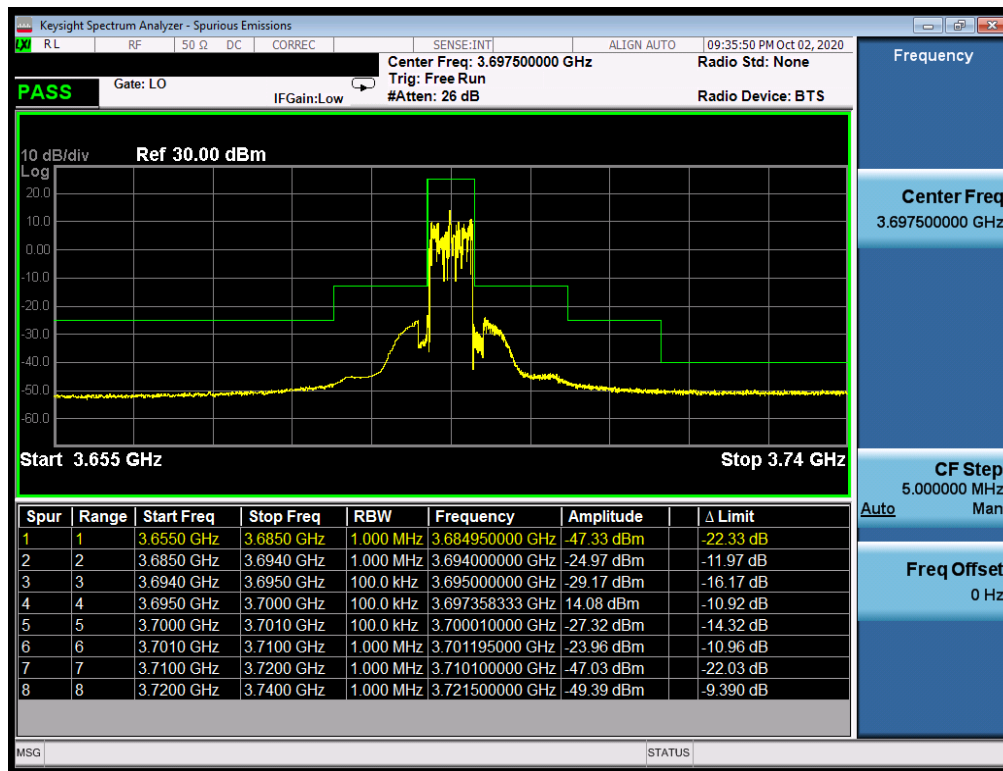
Plot 7-52. Upper ACP Plot (LTE Band 48 - 5MHz QPSK – Full RB Configuration)
