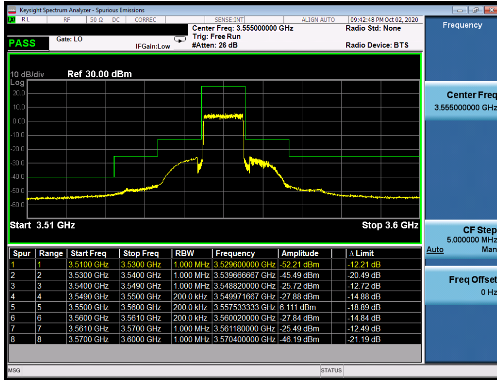
Plot 7-49. Lower ACP Plot (LTE Band 48 - 10MHz QPSK – Full RB Configuration)
