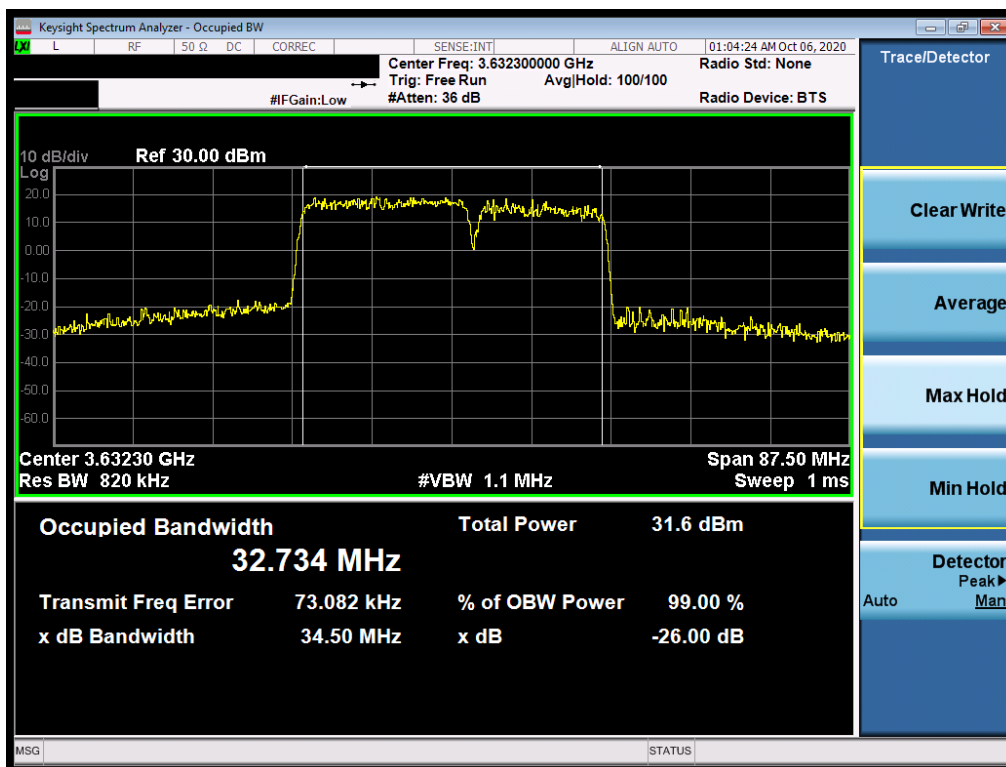
Plot 7-22. Occupied Bandwidth Plot (ULCA - 35.0MHz 16-QAM - Full RB Configuration)
