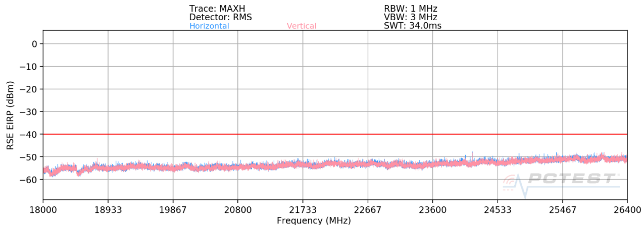
Plot 7-74. Radiated Spurious Plot 18GHz – 26.5GHz (ULCA Band 48)
