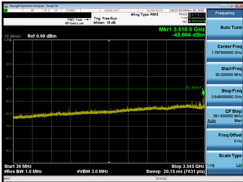
Plot 7-57. Conducted Spurious Plot (Band 48 – 20.0MHz QPSK – PCC 1/99 SCC 1/0 – Mid Channel)
