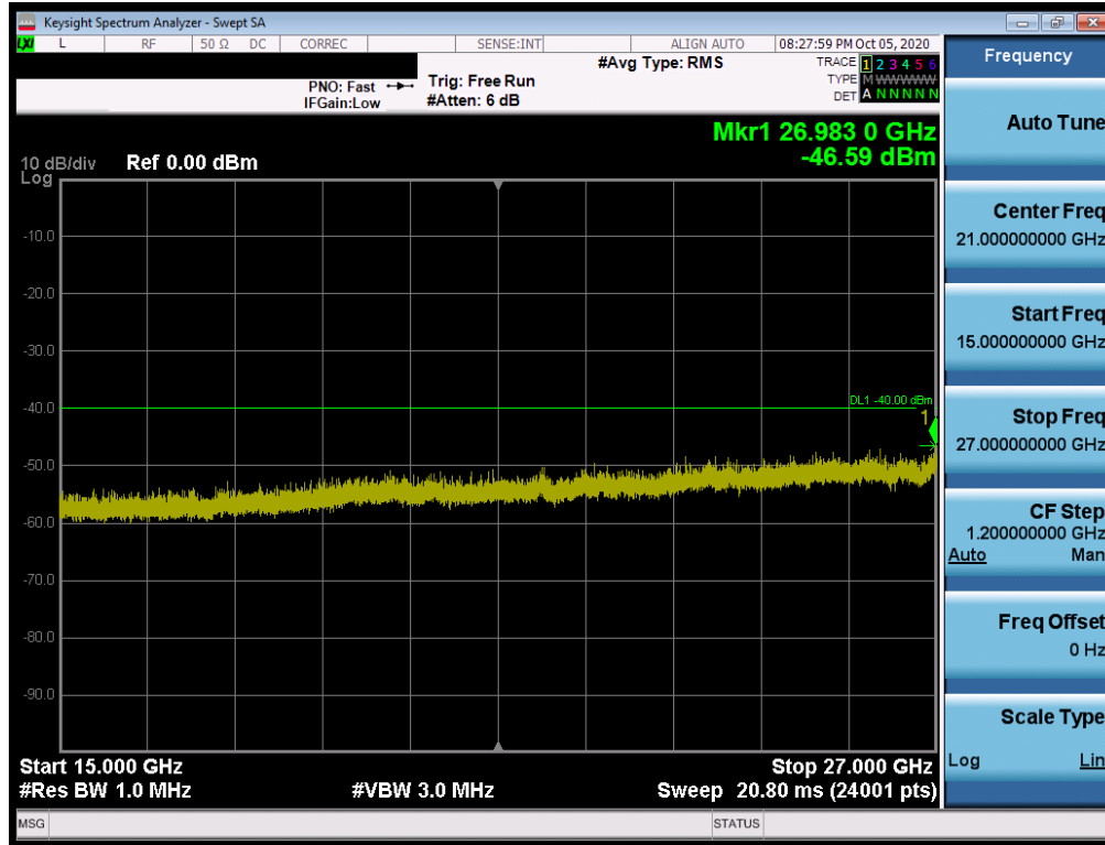
Plot 7-43. Conducted Spurious Plot (LTE Band 48 - 20MHz QPSK - RB Size 1, RB Offset 0 - High Channel)
