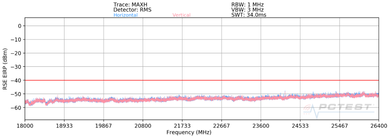
Plot 7-69. Radiated Spurious Plot 18 - 26.5GHz (Band 48)
