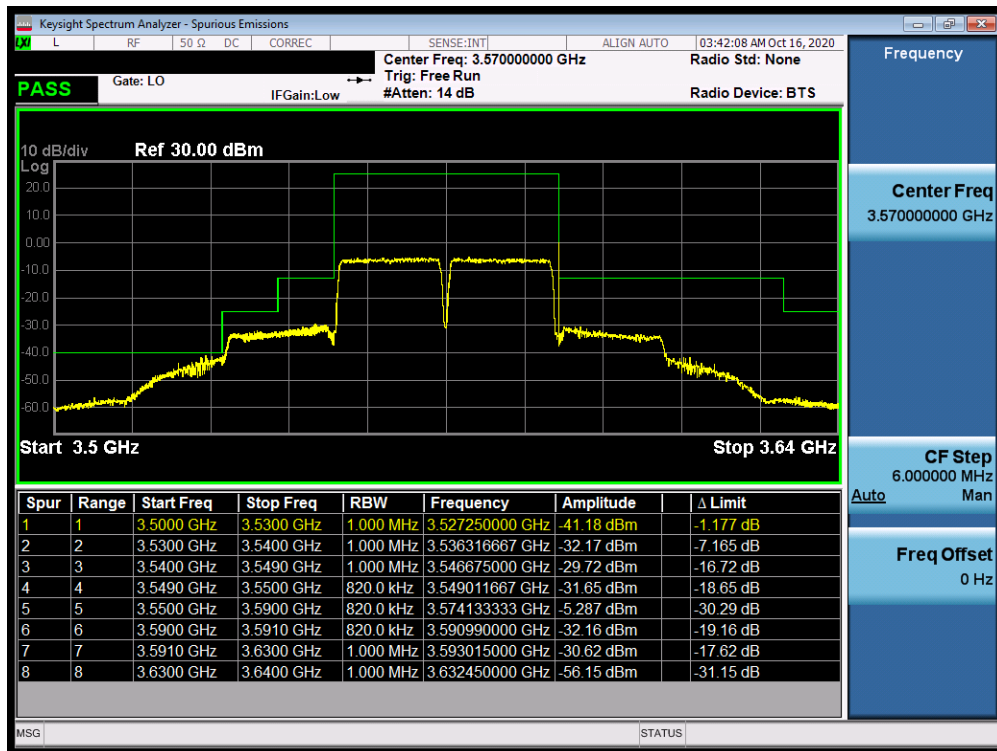
Plot 7-65. Lower Band Edge Plot (Band 48 QPSK – PCC:20 MHz SCC:20 MHz – Full RB)
