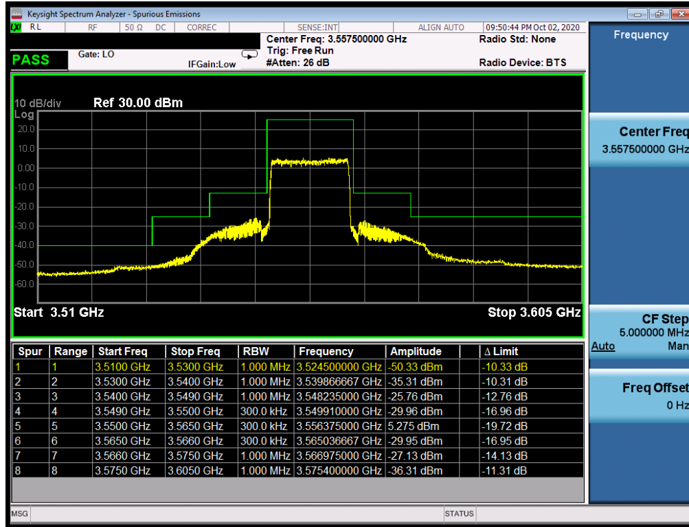
Plot 7-47. Lower ACP Plot (LTE Band 48 - 15MHz QPSK – Full RB Configuration)
