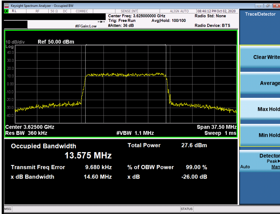
Plot 7-7. Occupied Bandwidth Plot (LTE Band 48 - 15.0MHz 64-QAM - Full RB Configuration)
