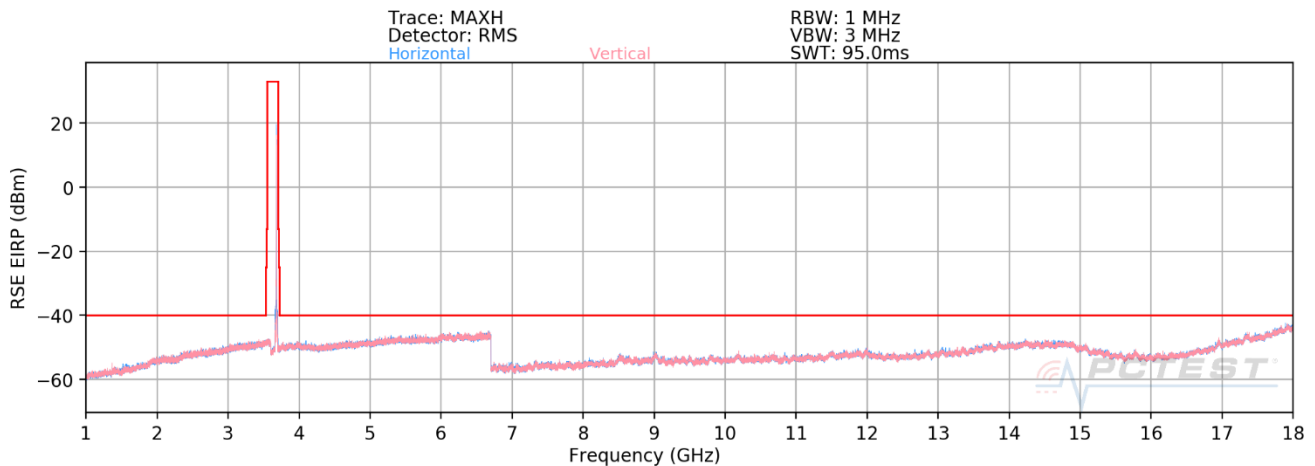
Plot 7-73. Radiated Spurious Plot 1GHz - 18GHz (ULCA Band 48) High Channel – PCC/SCC: 1RB)
