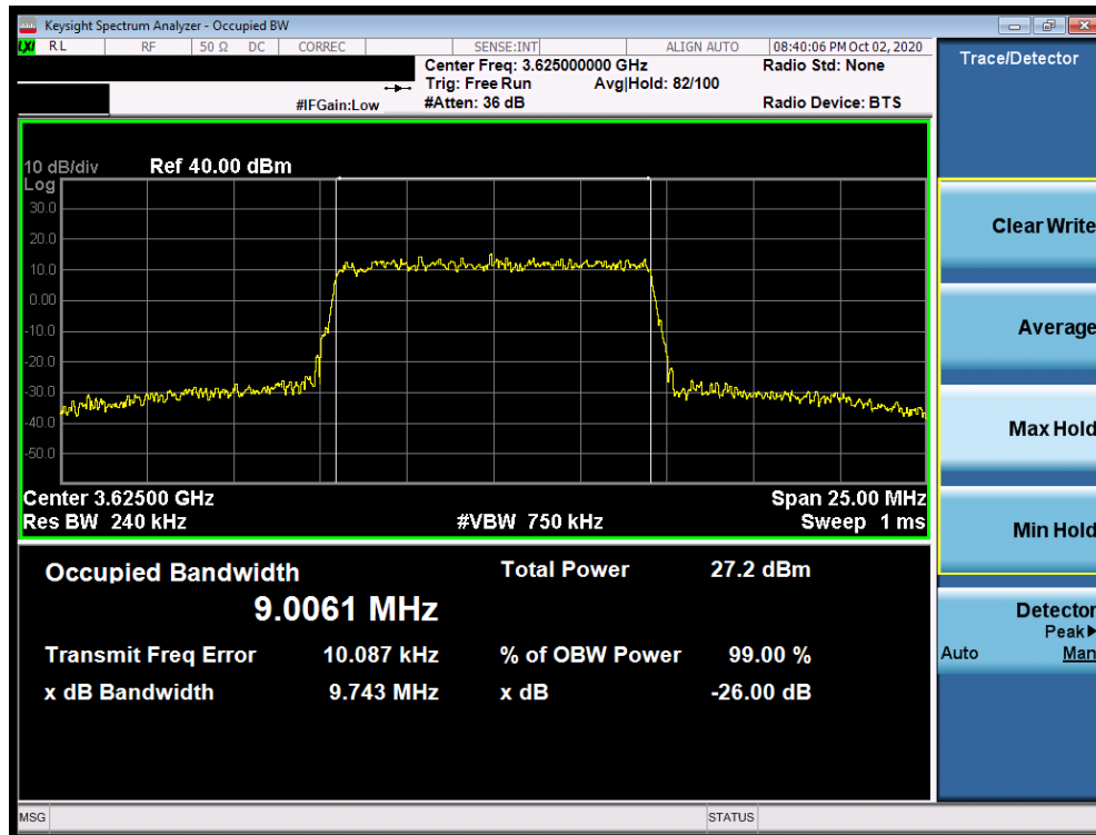
Plot 7-11. Occupied Bandwidth Plot (LTE Band 48 - 10.0MHz 64-QAM - Full RB Configuration)
