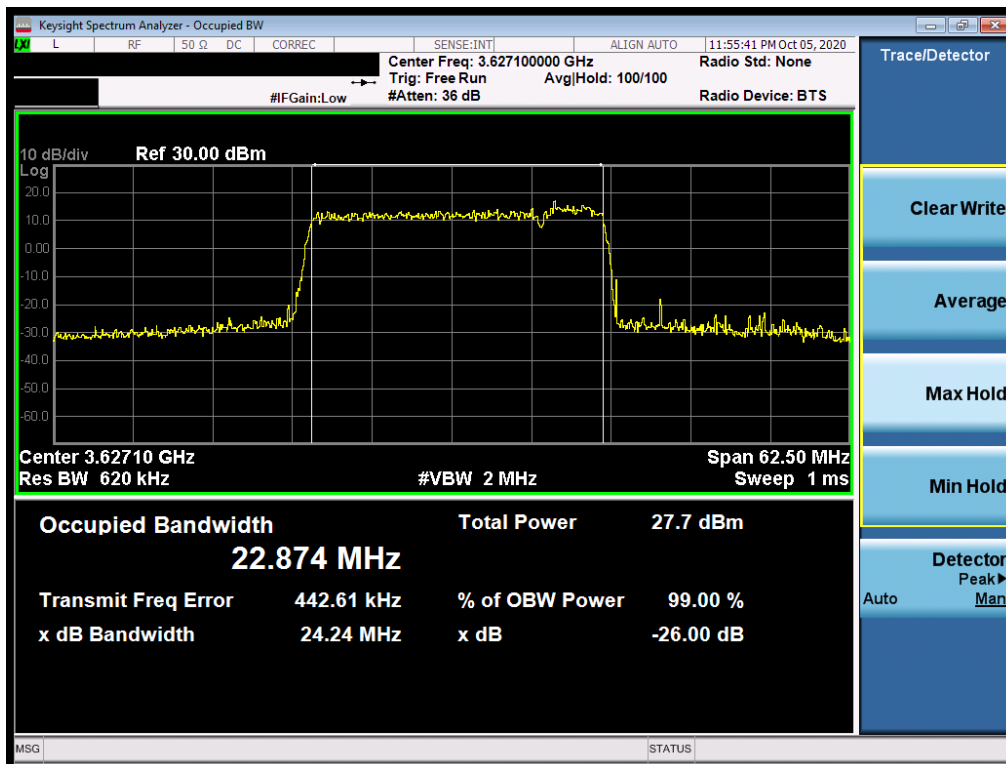
Plot 7-32. Occupied Bandwidth Plot (ULCA - 25.0MHz 256-QAM - Full RB Configuration)
