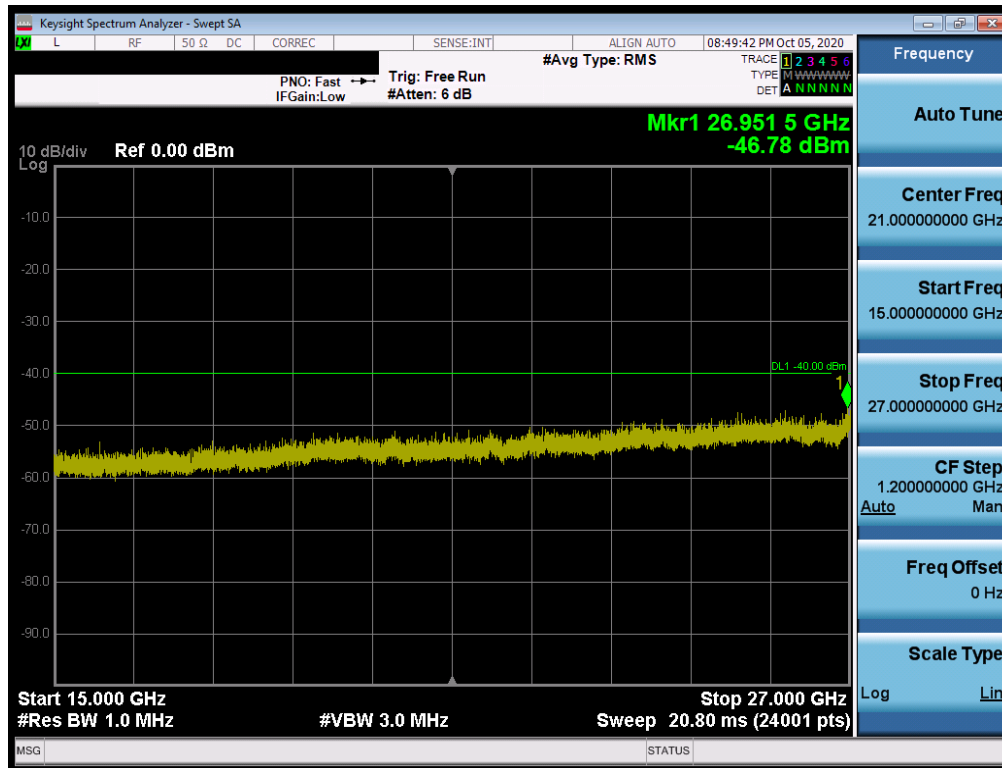
Plot 7-35. Conducted Spurious Plot (LTE Band 48 - 20MHz QPSK - RB Size 1, RB Offset 0 - Low Channel)
