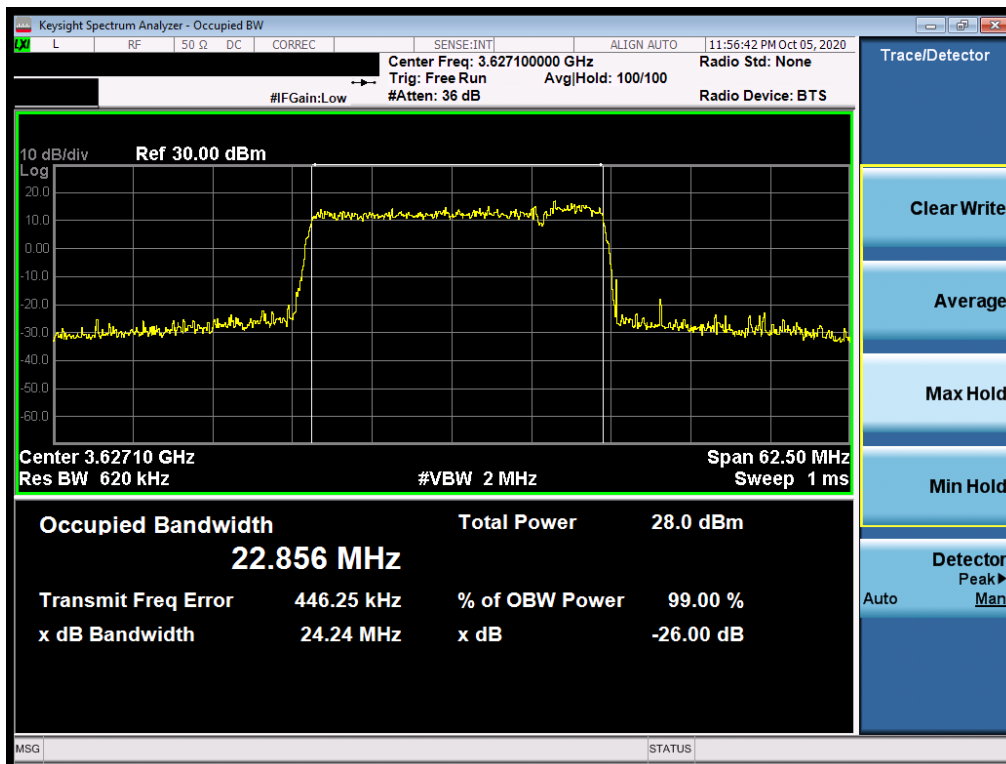
Plot 7-30. Occupied Bandwidth Plot (ULCA - 25.0MHz 16-QAM - Full RB Configuration)
