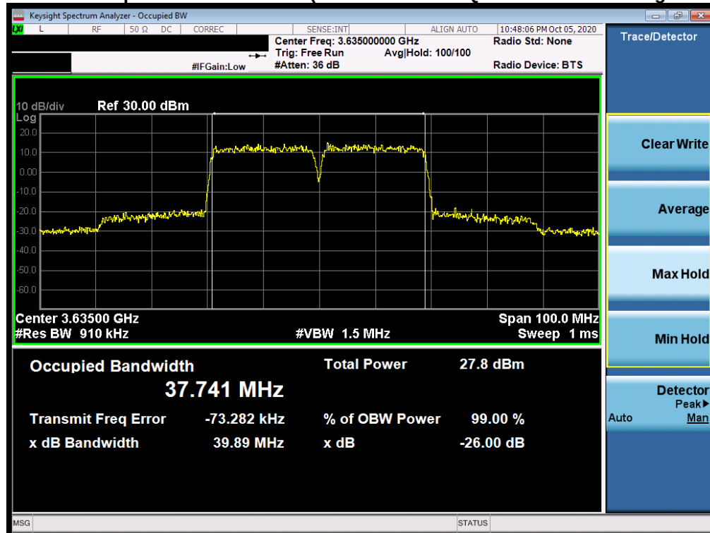
Plot 7-18. Occupied Bandwidth Plot (ULCA - 40.0MHz 16-QAM - Full RB Configuration)
