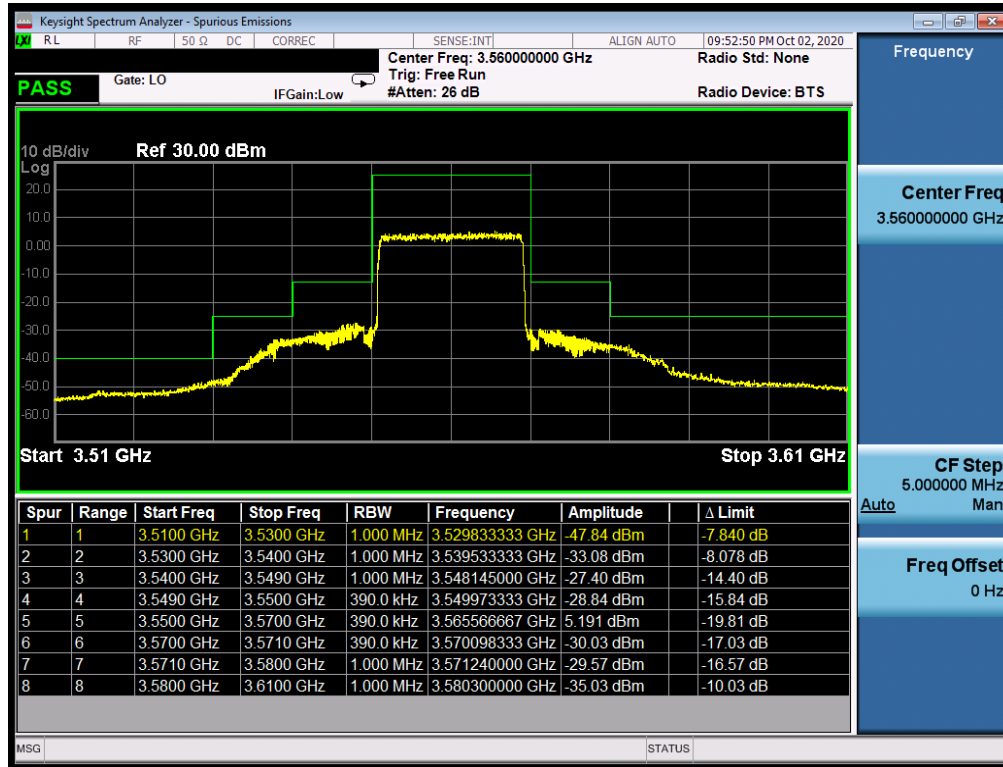
Plot 7-45. Lower ACP Plot (LTE Band 48 - 20MHz QPSK – Full RB Configuration)
