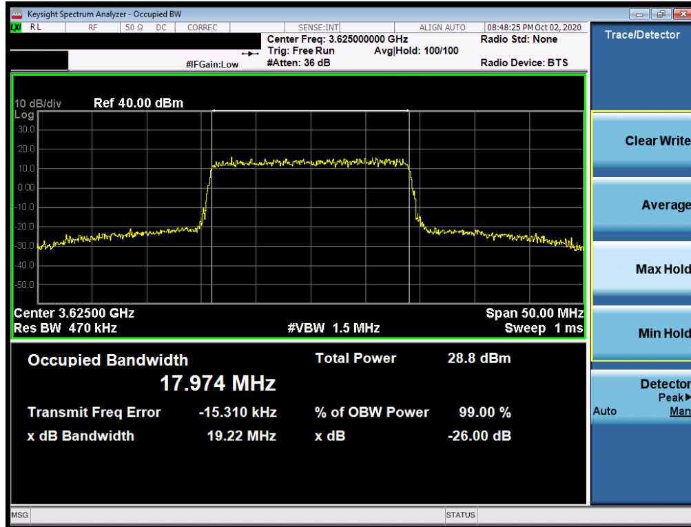
Plot 7-1. Occupied Bandwidth Plot (LTE Band 48 - 20.0MHz QPSK - Full RB Configuration)
