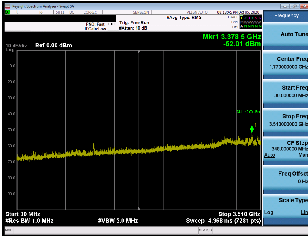
Plot 7-41. Conducted Spurious Plot (LTE Band 48 - 20MHz QPSK - RB Size 1, RB Offset 0 - High Channel)
