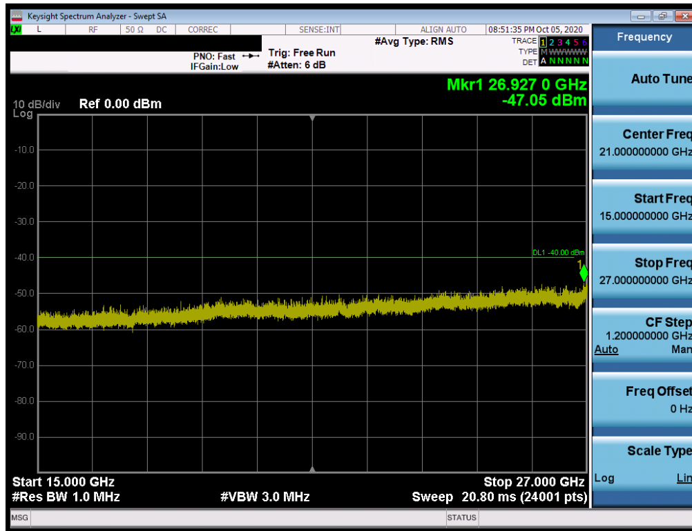
Plot 7-39. Conducted Spurious Plot (LTE Band 48 - 20MHz QPSK - RB Size 1, RB Offset 0 - Mid Channel)
