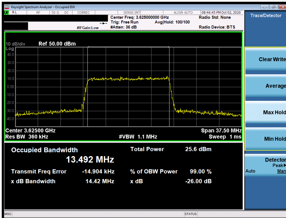
Plot 7-8. Occupied Bandwidth Plot (LTE Band 48 - 15.0MHz 256-QAM - Full RB Configuration)
