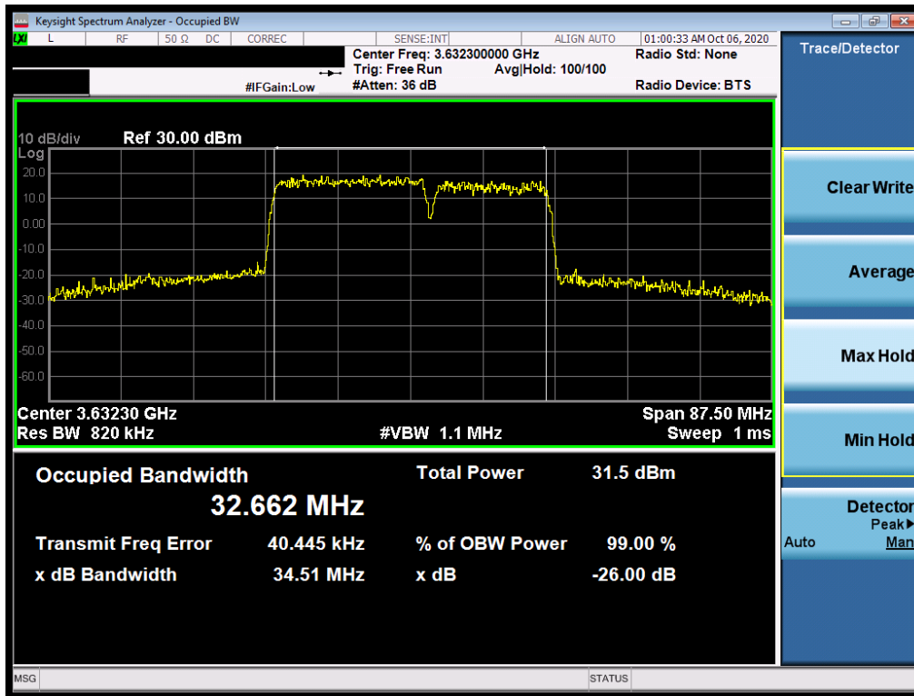
Plot 7-21. Occupied Bandwidth Plot (ULCA - 35.0MHz QPSK - Full RB Configuration)
