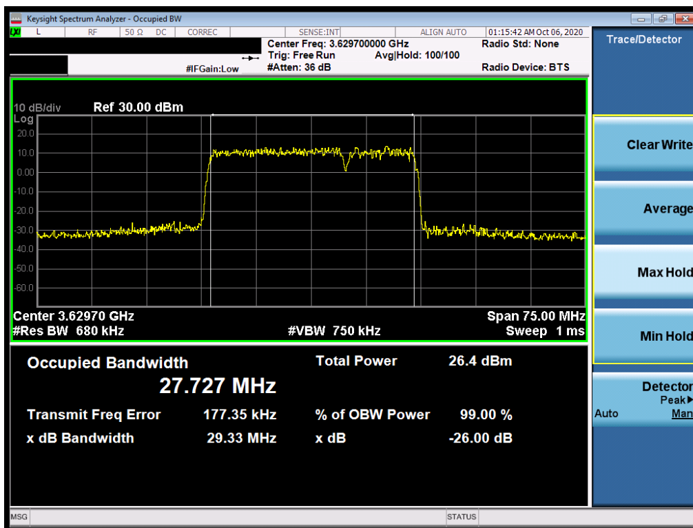
Plot 7-28. Occupied Bandwidth Plot (ULCA - 30.0MHz 256-QAM - Full RB Configuration)
