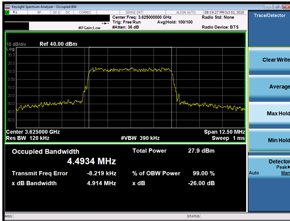
Plot 7-15. Occupied Bandwidth Plot (LTE Band 48 - 5.0MHz 64-QAM - Full RB Configuration)
