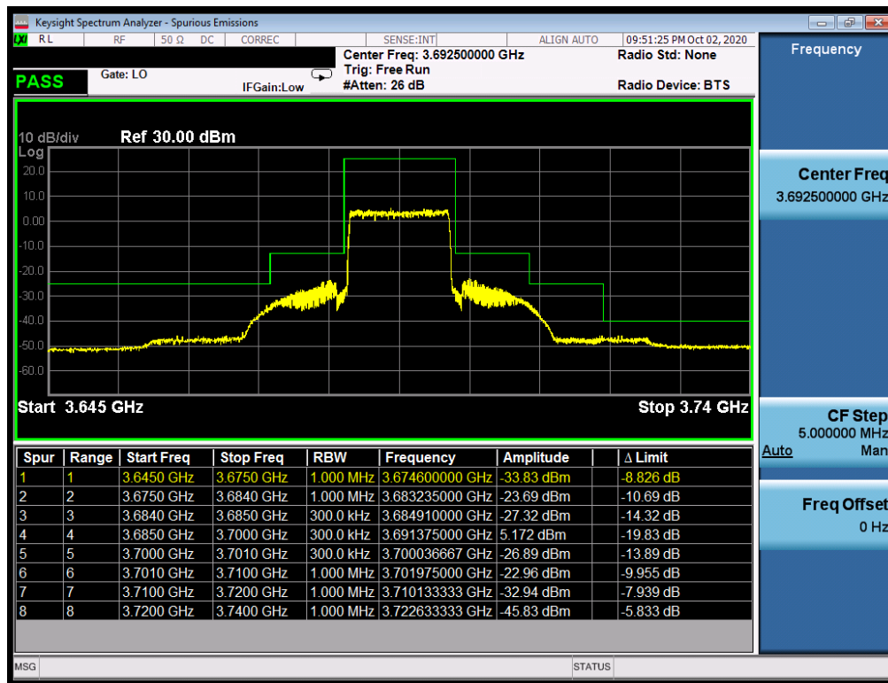
Plot 7-48. Upper ACP Plot (LTE Band 48 - 15MHz QPSK – Full RB Configuration)
