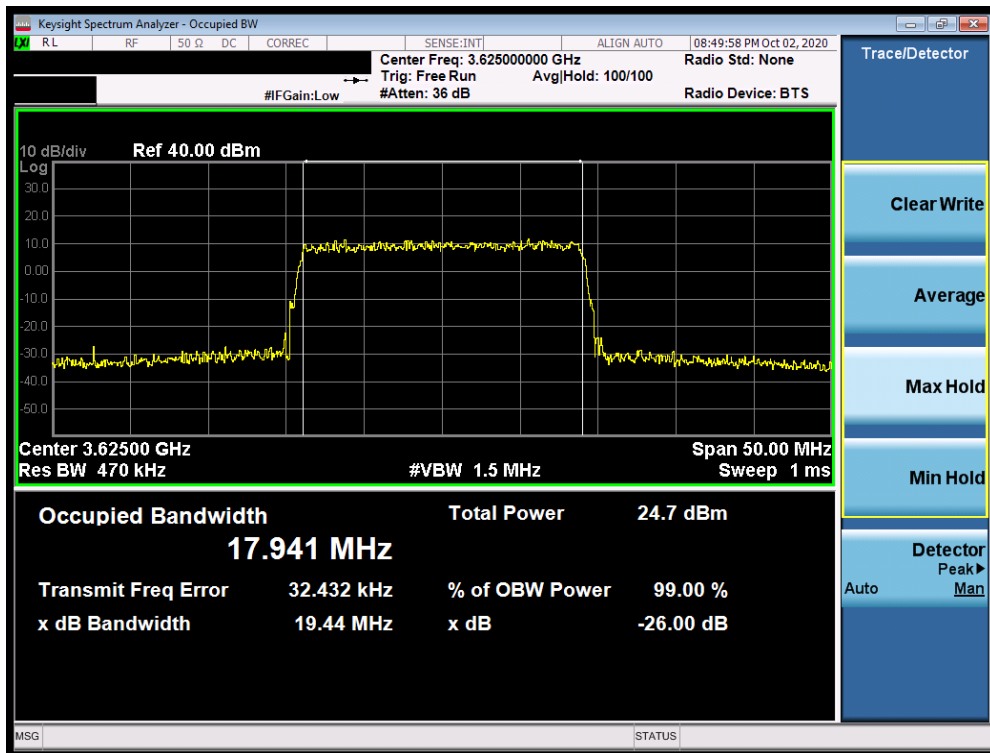
Plot 7-4. Occupied Bandwidth Plot (LTE Band 48 - 20.0MHz 256-QAM - Full RB Configuration)
