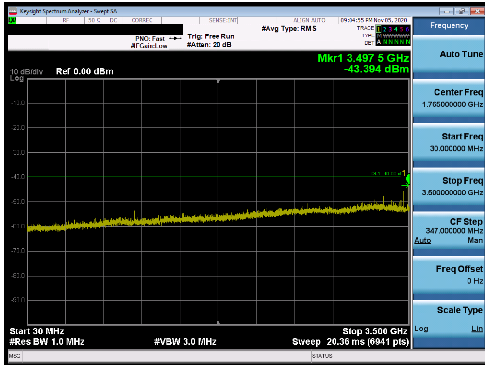
Plot 7-53. Conducted Spurious Plot (Band 48 – 20.0MHz QPSK – PCC 1/99 SCC 1/0 – Low Channel)
