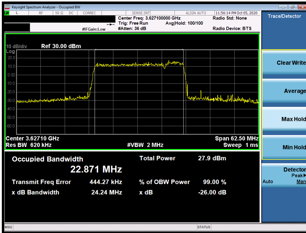
Plot 7-31. Occupied Bandwidth Plot (ULCA - 25.0MHz 64-QAM - Full RB Configuration)
