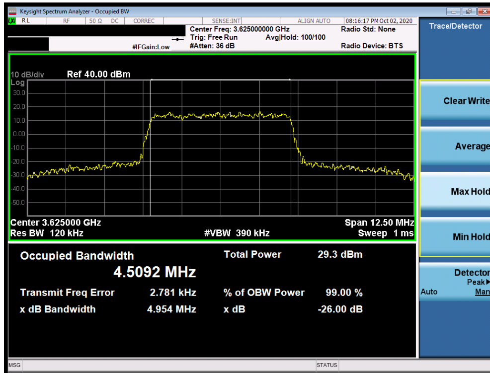
Plot 7-13. Occupied Bandwidth Plot (LTE Band 48 - 5.0MHz QPSK - Full RB Configuration)
