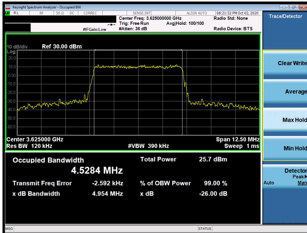
Plot 7-16. Occupied Bandwidth Plot (LTE Band 48 - 5.0MHz 256-QAM - Full RB Configuration)
