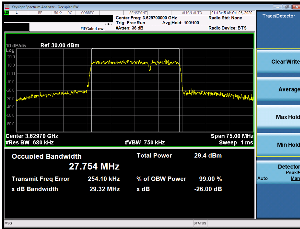
Plot 7-25. Occupied Bandwidth Plot (ULCA - 30.0MHz QPSK - Full RB Configuration)
