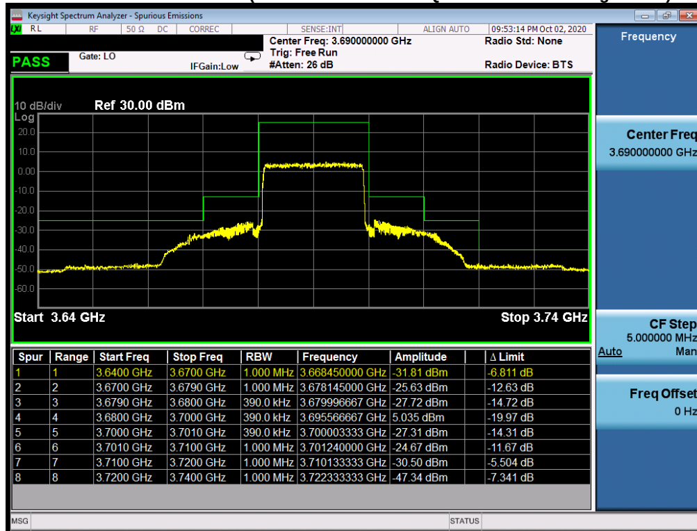
Plot 7-46. Upper ACP Plot (LTE Band 48 - 20MHz QPSK – Full RB Configuration)
