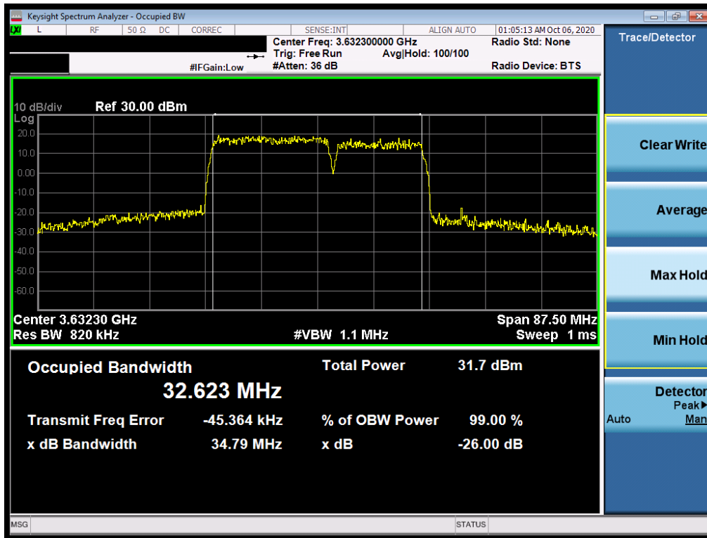
Plot 7-23. Occupied Bandwidth Plot (ULCA - 35.0MHz 64-QAM - Full RB Configuration)
