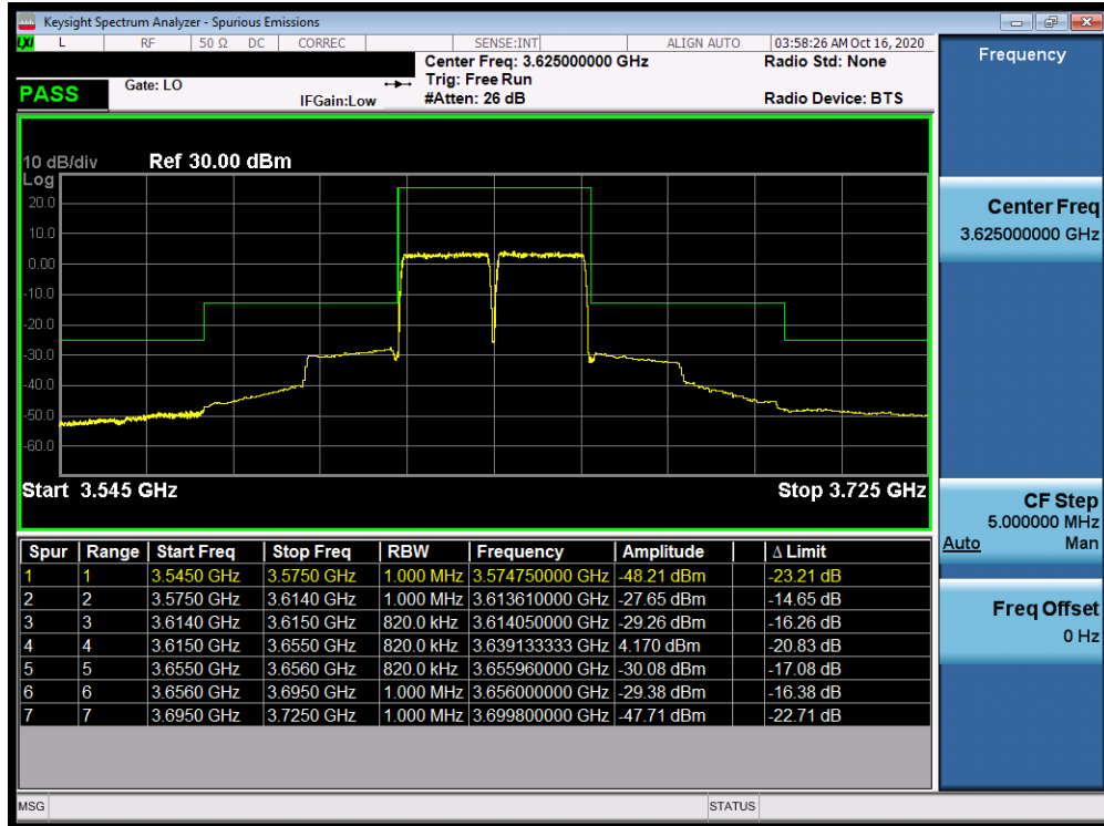
Plot 7-66. Mid Band Edge Plot (Band 48 QPSK – PCC:20 MHz SCC:20 MHz – Full RB)
