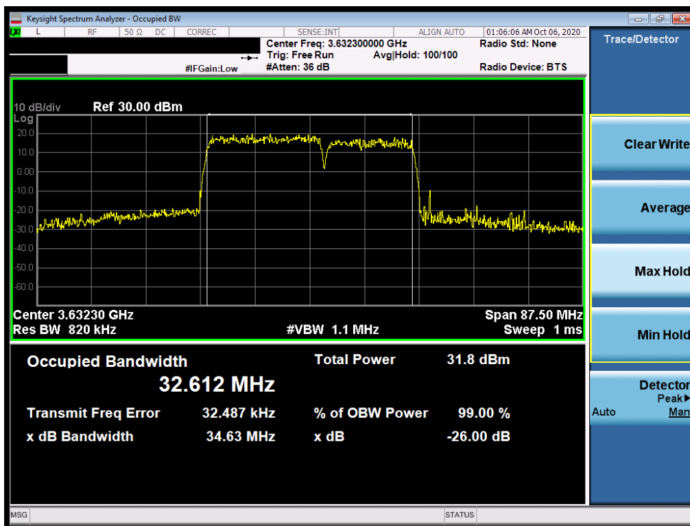
Plot 7-24. Occupied Bandwidth Plot (ULCA - 35.0MHz 256-QAM - Full RB Configuration)
