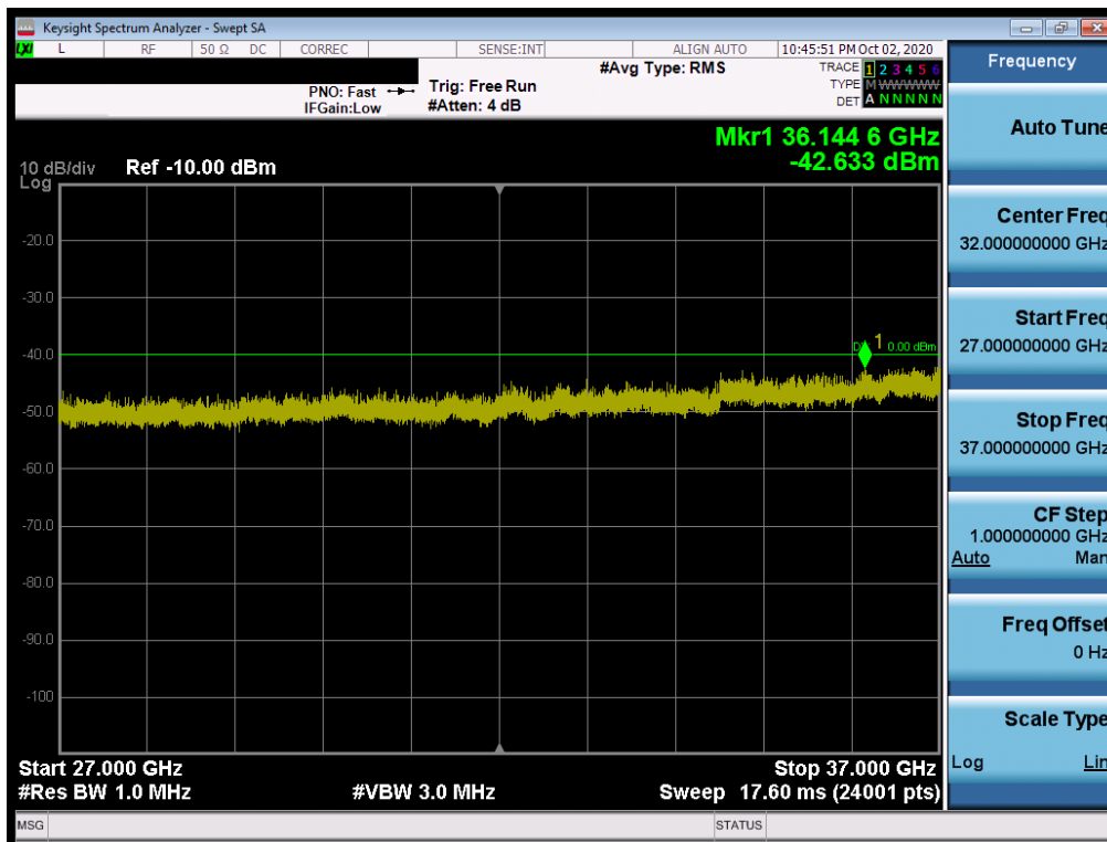
Plot 7-40. Conducted Spurious Plot (LTE Band 48 - 20MHz QPSK - RB Size 1, RB Offset 0 - Mid Channel)
