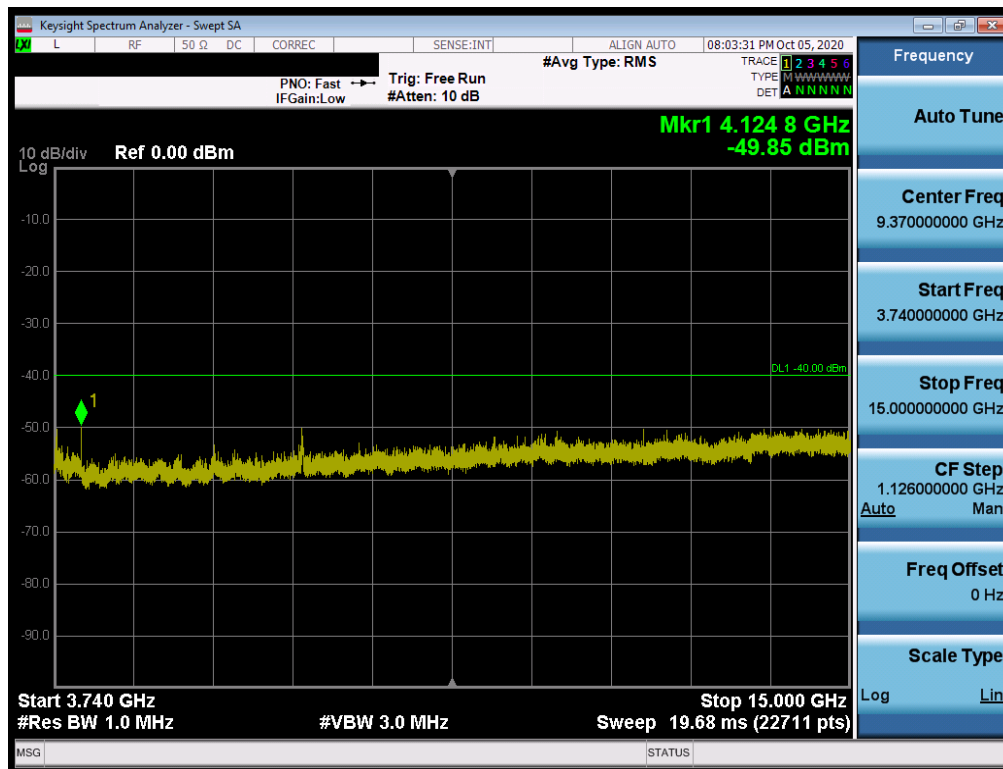
Plot 7-38. Conducted Spurious Plot (LTE Band 48 - 20MHz QPSK - RB Size 1, RB Offset 0 - Mid Channel)
