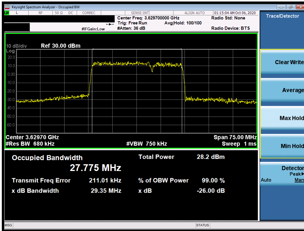
Plot 7-27. Occupied Bandwidth Plot (ULCA - 30.0MHz 64-QAM - Full RB Configuration)
