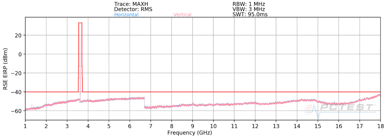
Plot 7-68. Radiated Spurious Plot 1 - 18GHz (Band 48)
