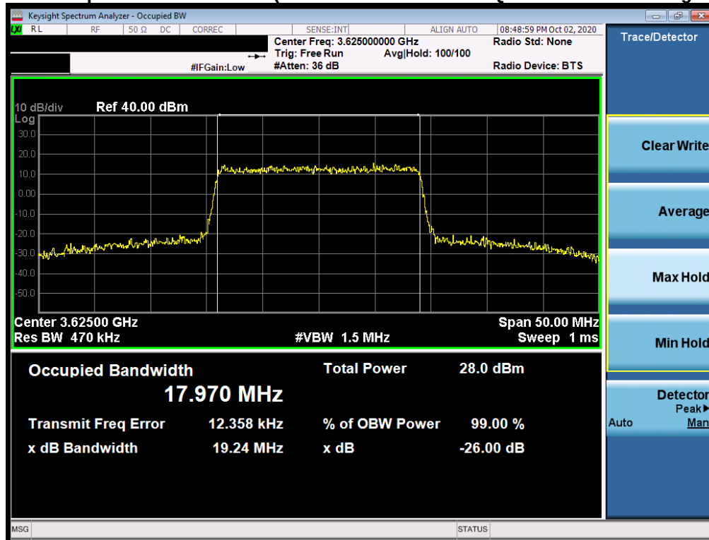
Plot 7-2. Occupied Bandwidth Plot (LTE Band 48 - 20.0MHz 16-QAM - Full RB Configuration)
