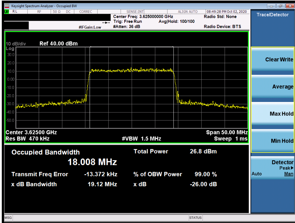
Plot 7-3. Occupied Bandwidth Plot (LTE Band 48 - 20.0MHz 64-QAM - Full RB Configuration)
