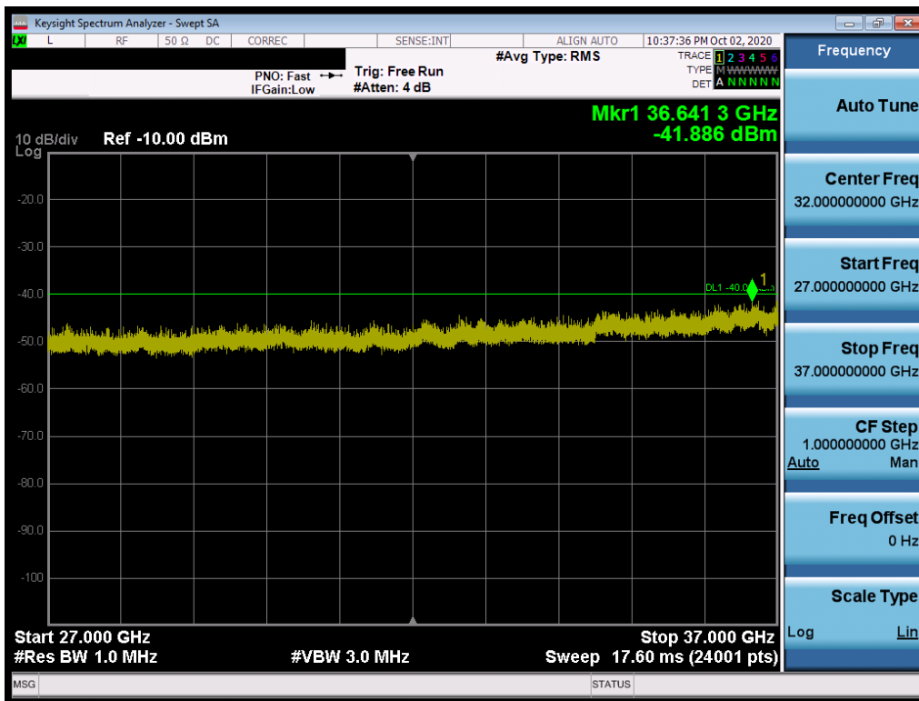
Plot 7-44. Conducted Spurious Plot (LTE Band 48 - 20MHz QPSK - RB Size 1, RB Offset 0 - High Channel)
