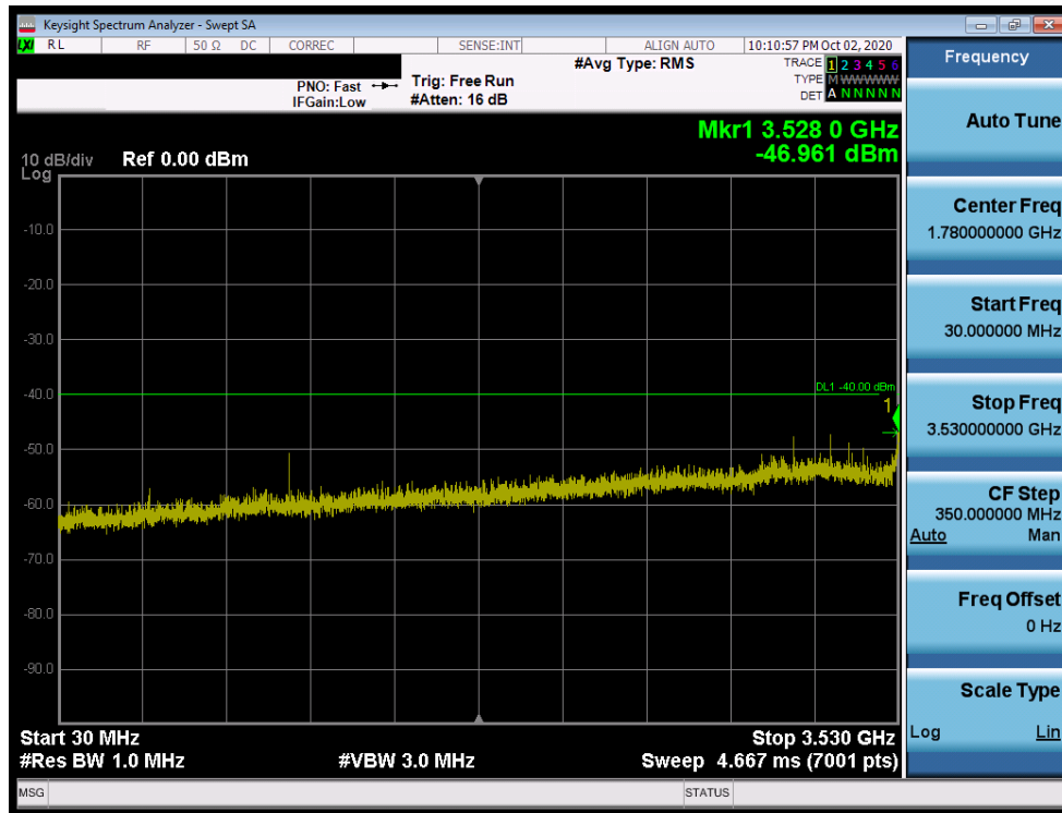
Plot 7-33. Conducted Spurious Plot (LTE Band 48 - 20MHz QPSK - RB Size 1, RB Offset 0 - Low Channel)
