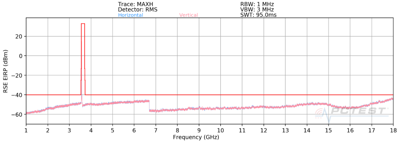
Plot 7-71. Radiated Spurious Plot 1GHz - 18GHz (ULCA Band 48) Low Channel – PCC/SCC: 1RB)
