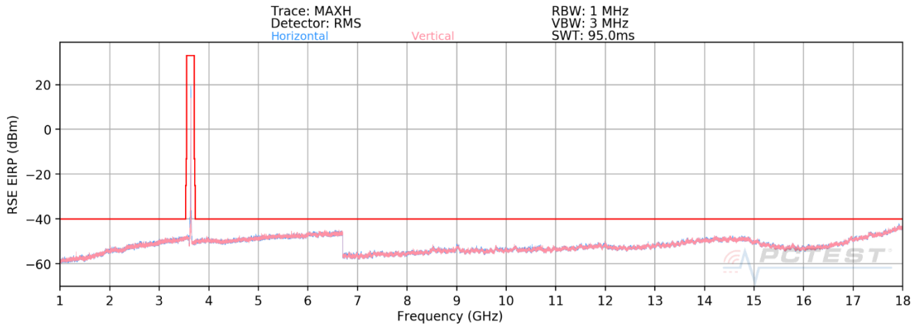
Plot 7-72. Radiated Spurious Plot 1GHz - 18GHz (ULCA Band 48) Mid Channel – PCC/SCC: 1RB)
