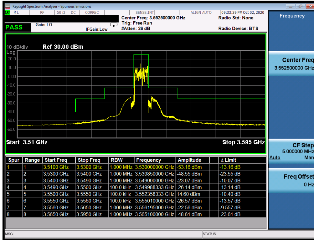
Plot 7-51. Lower ACP Plot (LTE Band 48 - 5MHz QPSK – Full RB Configuration)
