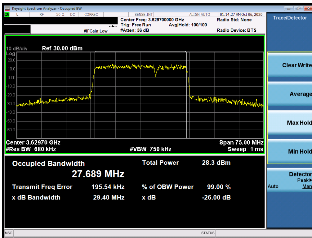
Plot 7-26. Occupied Bandwidth Plot (ULCA - 30.0MHz 16-QAM - Full RB Configuration)
