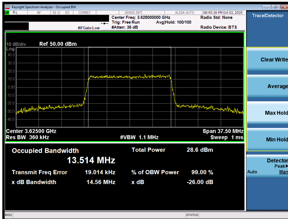
Plot 7-6. Occupied Bandwidth Plot (LTE Band 48 - 15.0MHz 16-QAM - Full RB Configuration)
