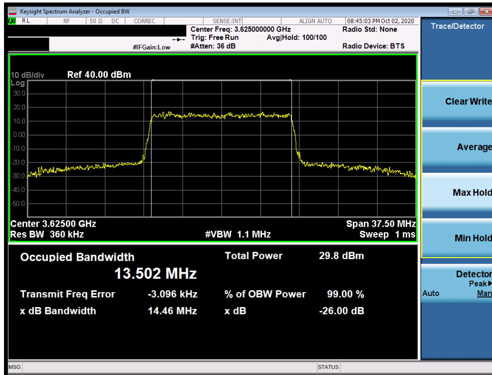
Plot 7-5. Occupied Bandwidth Plot (LTE Band 48 - 15.0MHz QPSK - Full RB Configuration)
