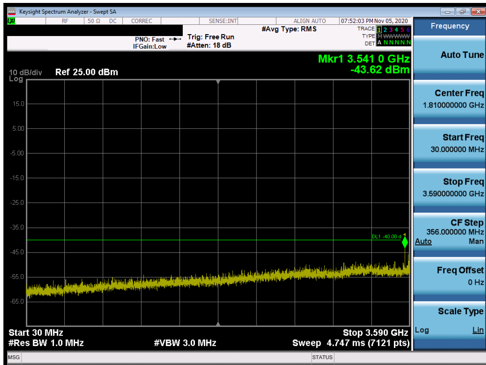
Plot 7-61. Conducted Spurious Plot (Band 48 – 20.0MHz QPSK – PCC 1/0 SCC 1/99 – High Channel)
