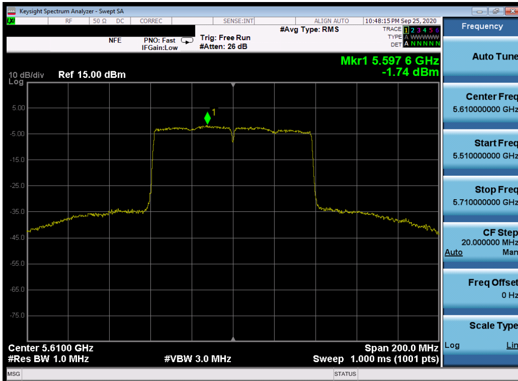
Plot 7-242. Power Spectral Density Plot SISO ANT2 (80MHz BW 802.11ac (UNII Band 2C) – Ch. 122)
