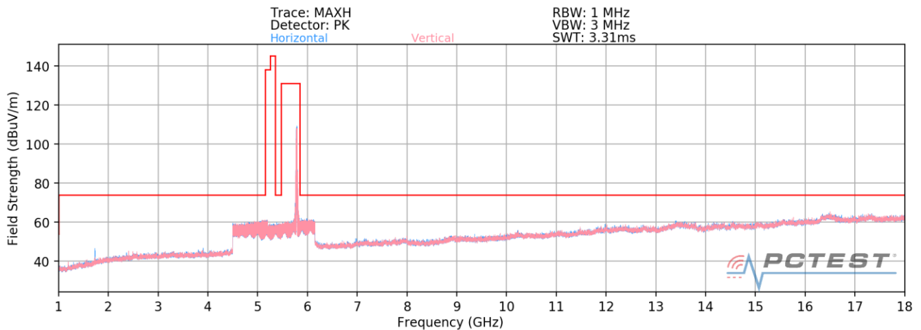
Plot 7-277. Radiated Spurious Plot above 1GHz MIMO (802.11a – U3 Ch. 157)
