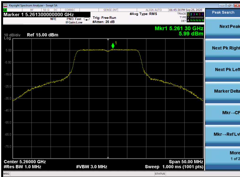
Plot 7-211. Power Spectral Density Plot SISO ANT2 (802.11a (UNII Band 2A) - Ch. 52)
