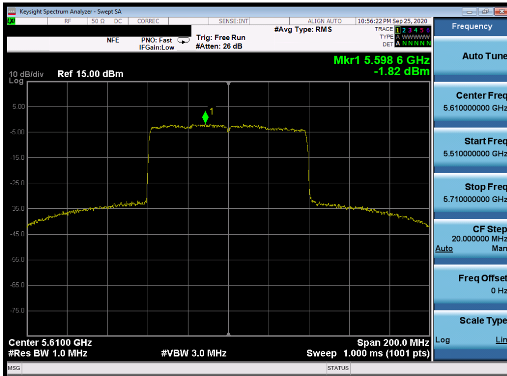
Plot 7-245. Power Spectral Density Plot SISO ANT2 (80MHz BW 802.11ax (UNII Band 2C) – Ch. 122)
