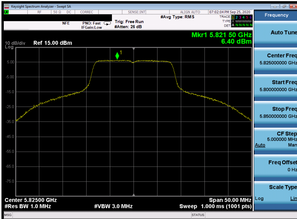
Plot 7-249. Power Spectral Density Plot SISO ANT2 (802.11a (UNII Band 3) – Ch. 165)
