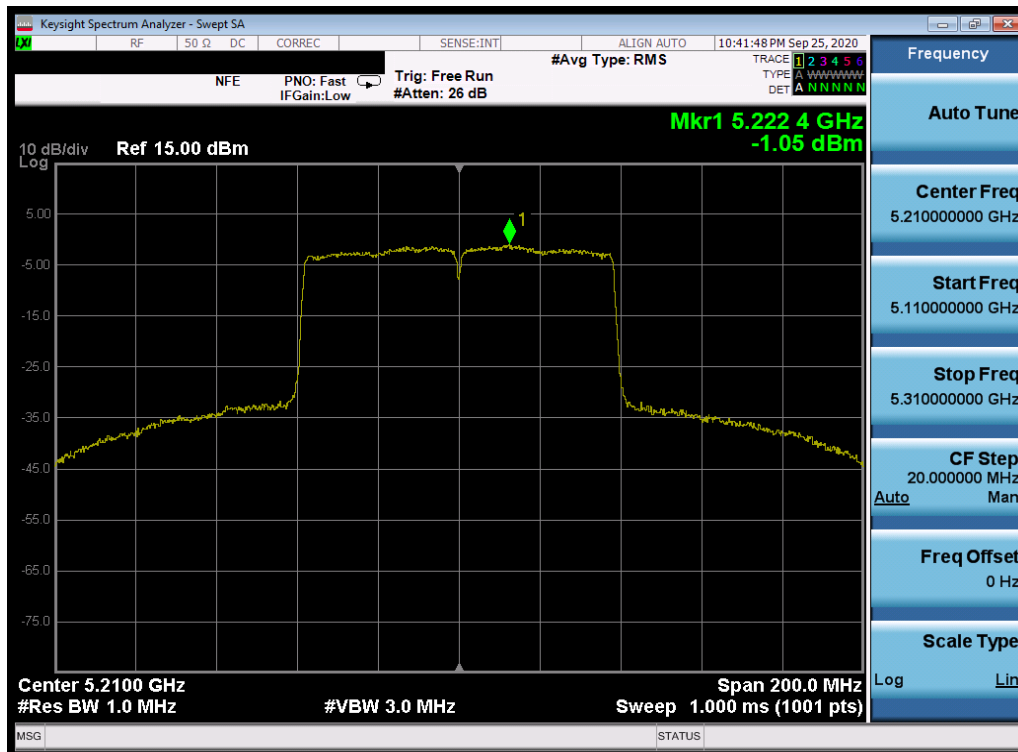
Plot 7-209. Power Spectral Density Plot SISO ANT2 (80MHz BW 802.11ac (UNII Band 1) – Ch. 42)
