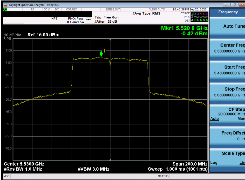
Plot 7-241. Power Spectral Density Plot SISO ANT2 (80MHz BW 802.11ac (UNII Band 2C) – Ch. 106)
