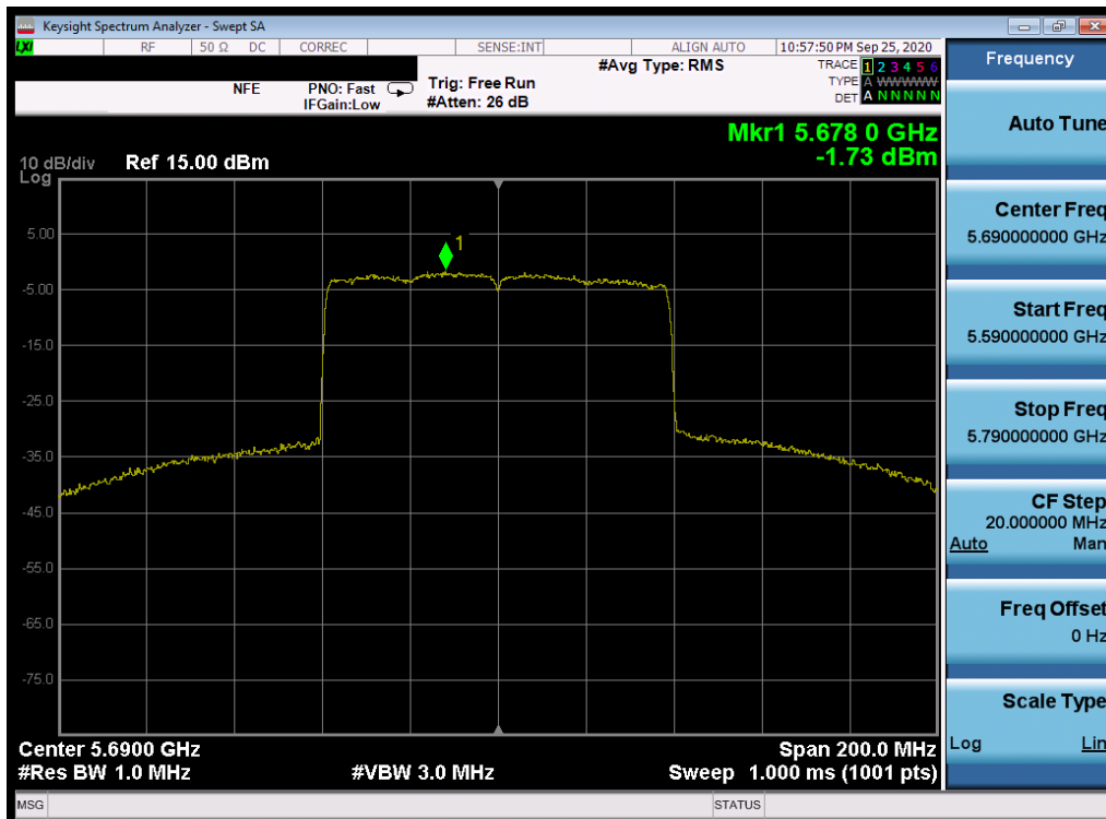
Plot 7-246. Power Spectral Density Plot SISO ANT2 (80MHz BW 802.11ax (UNII Band 2C) – Ch. 138)
