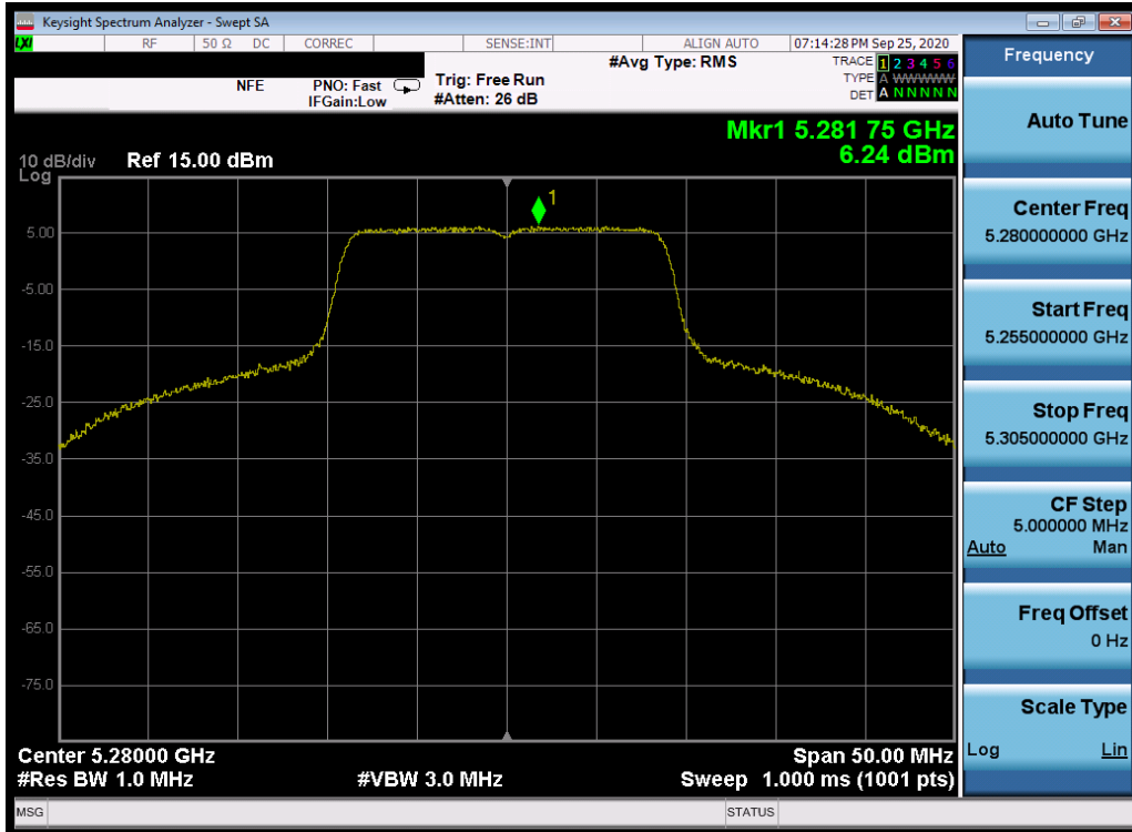
Plot 7-215. Power Spectral Density Plot SISO ANT2 (20MHz BW 802.11n (UNII Band 2A) – Ch. 56)
