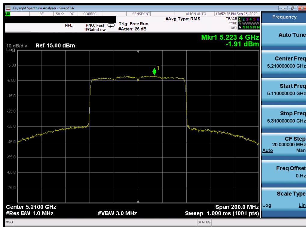
Plot 7-210. Power Spectral Density Plot SISO ANT2 (80MHz BW 802.11ax (UNII Band 1) – Ch. 42)
