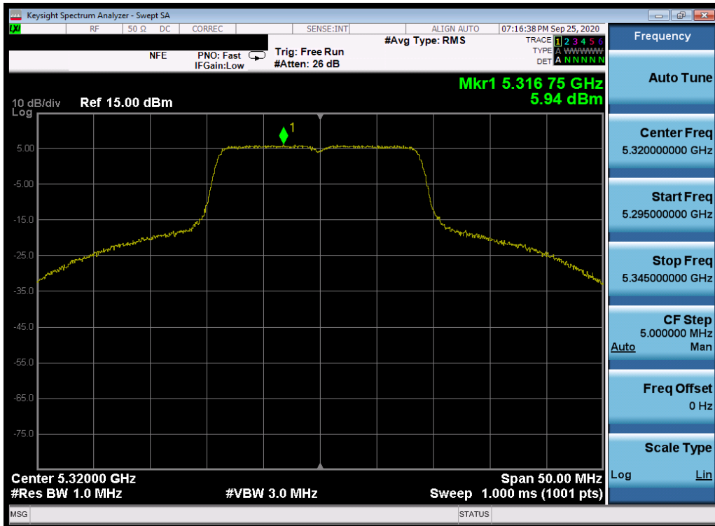
Plot 7-216. Power Spectral Density Plot SISO ANT2 (20MHz BW 802.11n (UNII Band 2A) – Ch. 64)
