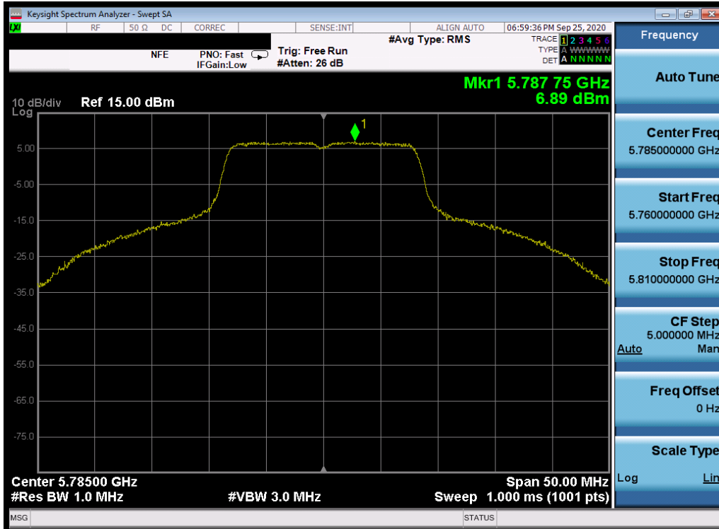
Plot 7-248. Power Spectral Density Plot SISO ANT2 (802.11a (UNII Band 3) – Ch. 157)
