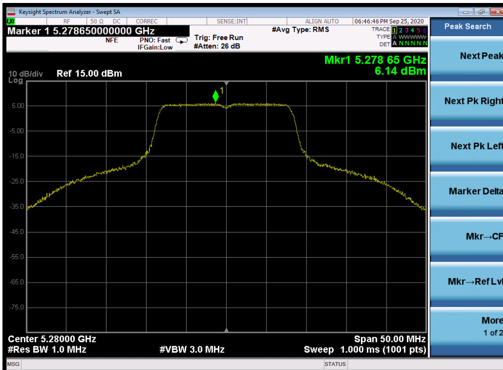
Plot 7-212. Power Spectral Density Plot SISO ANT2 (802.11a (UNII Band 2A) - Ch. 56)
