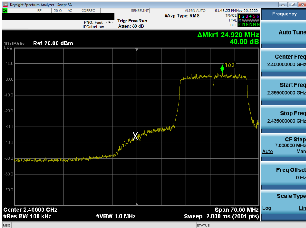
Plot 7-77. Band Edge Plot SISO ANT2 (802.11ax (2.4GHz) – Ch. 3)
