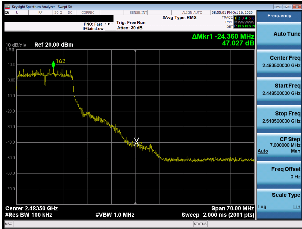
Plot 7-53. Band Edge Plot SISO ANT1 (802.11g- Ch. 10)
