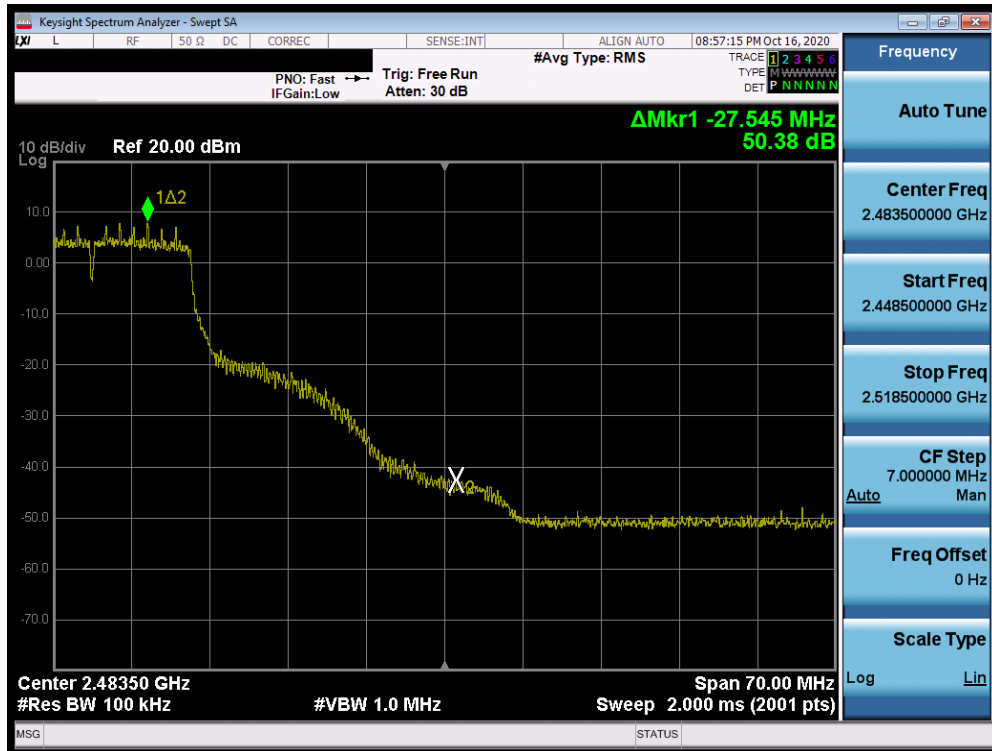
Plot 7-57. Band Edge Plot SISO ANT1 (802.11n (2.4GHz) – Ch. 9)
