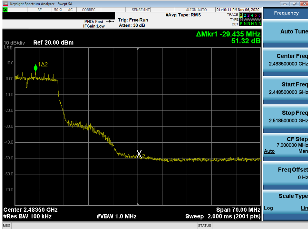
Plot 7-72. Band Edge Plot SISO ANT2 (802.11n (2.4GHz) – Ch. 9)
