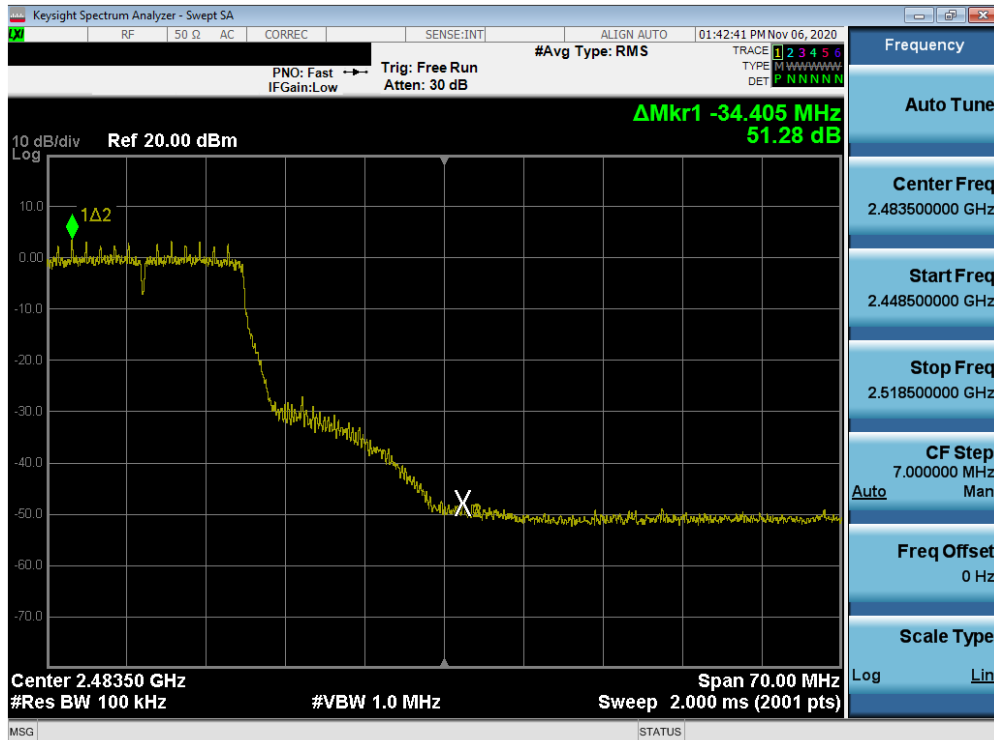
Plot 7-73. Band Edge Plot SISO ANT2 (802.11n (2.4GHz) – Ch. 10)
