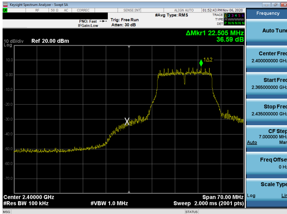
Plot 7-67. Band Edge Plot SISO ANT2 (802.11g- Ch. 2)
