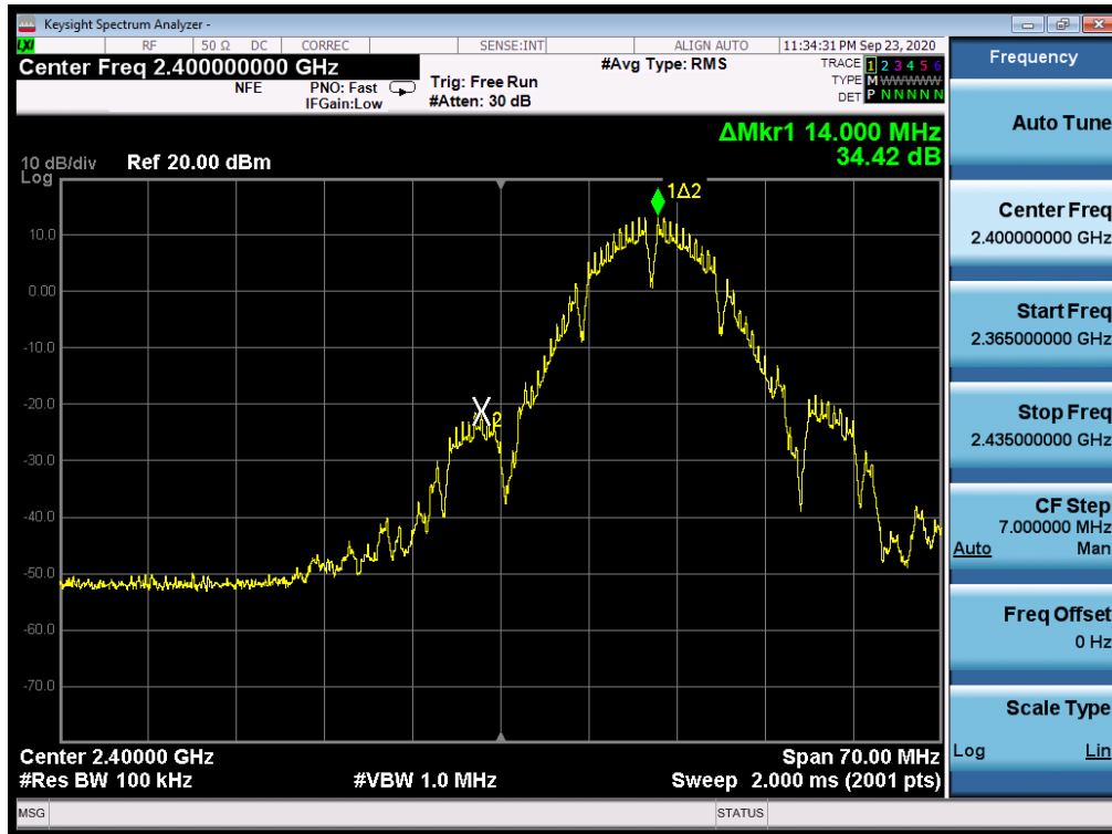
Plot 7-64. Band Edge Plot SISO ANT2 (802.11b – Ch. 1)
