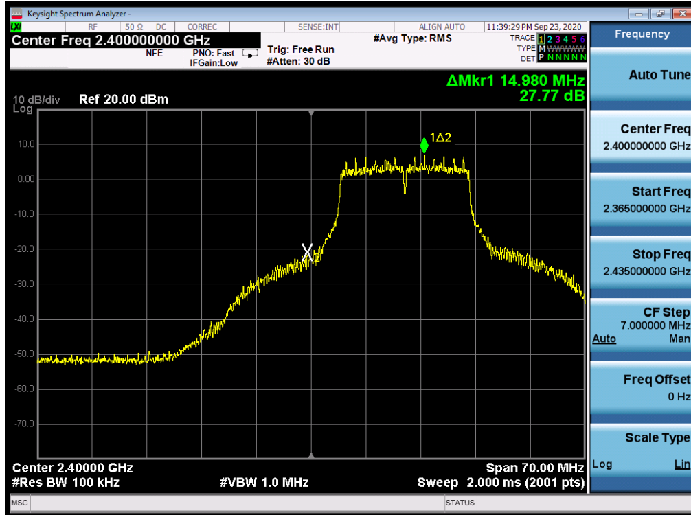
Plot 7-66. Band Edge Plot SISO ANT2 (802.11g- Ch. 1)
