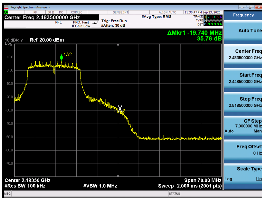
Plot 7-59. Band Edge Plot SISO ANT1 (802.11n (2.4GHz) - Ch. 11)
