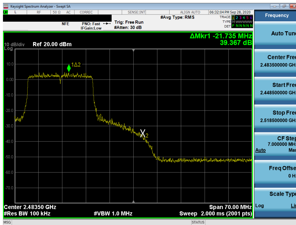
Plot 7-80. Band Edge Plot SISO ANT2 (802.11ax (2.4GHz) – Ch. 11)
