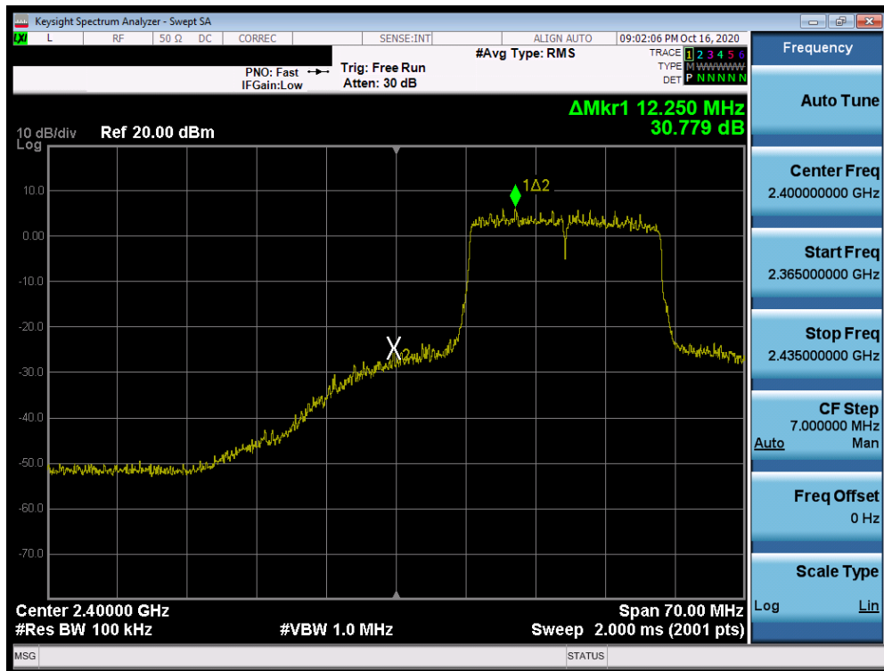
Plot 7-61. Band Edge Plot SISO ANT1 (802.11ax (2.4GHz) – Ch. 2)
