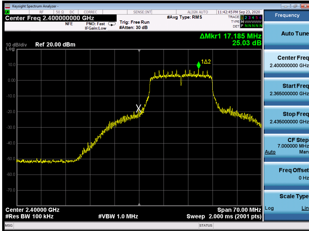
Plot 7-70. Band Edge Plot SISO ANT2 (802.11n (2.4GHz) – Ch. 1)
