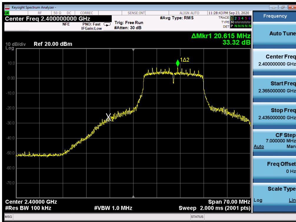
Plot 7-55. Band Edge Plot SISO ANT1 (802.11n (2.4GHz) – Ch. 1)
