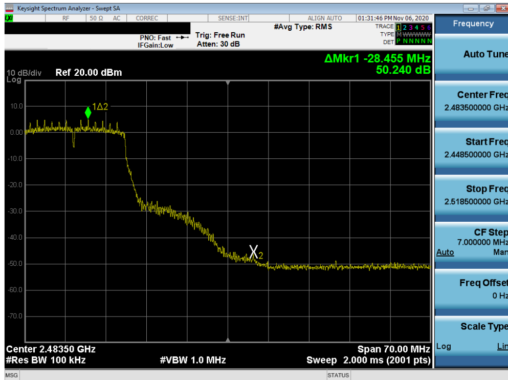
Plot 7-58. Band Edge Plot SISO ANT1 (802.11n (2.4GHz) - Ch. 10)
