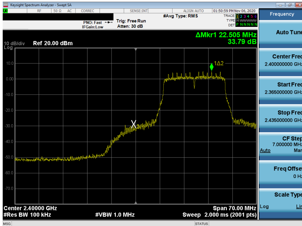
Plot 7-71. Band Edge Plot SISO ANT2 (802.11n (2.4GHz) – Ch. 2)
