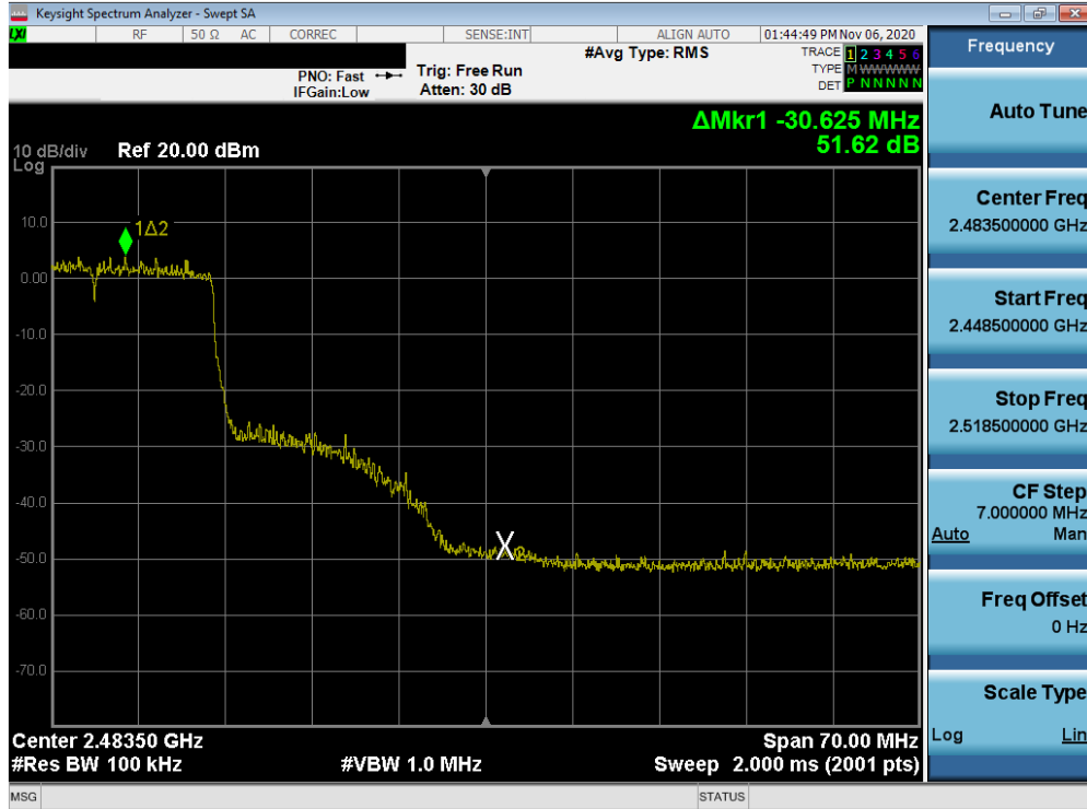
Plot 7-78. Band Edge Plot SISO ANT2 (802.11ax (2.4GHz) – Ch. 9)
