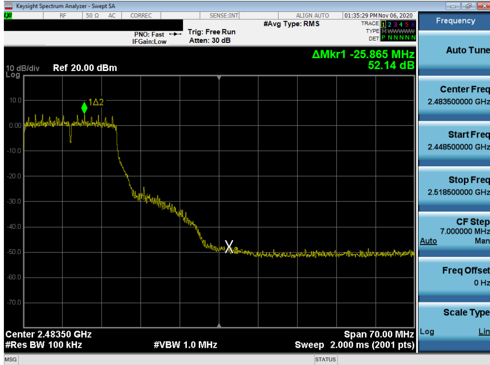
Plot 7-68. Band Edge Plot SISO ANT2 (802.11g- Ch. 10)
