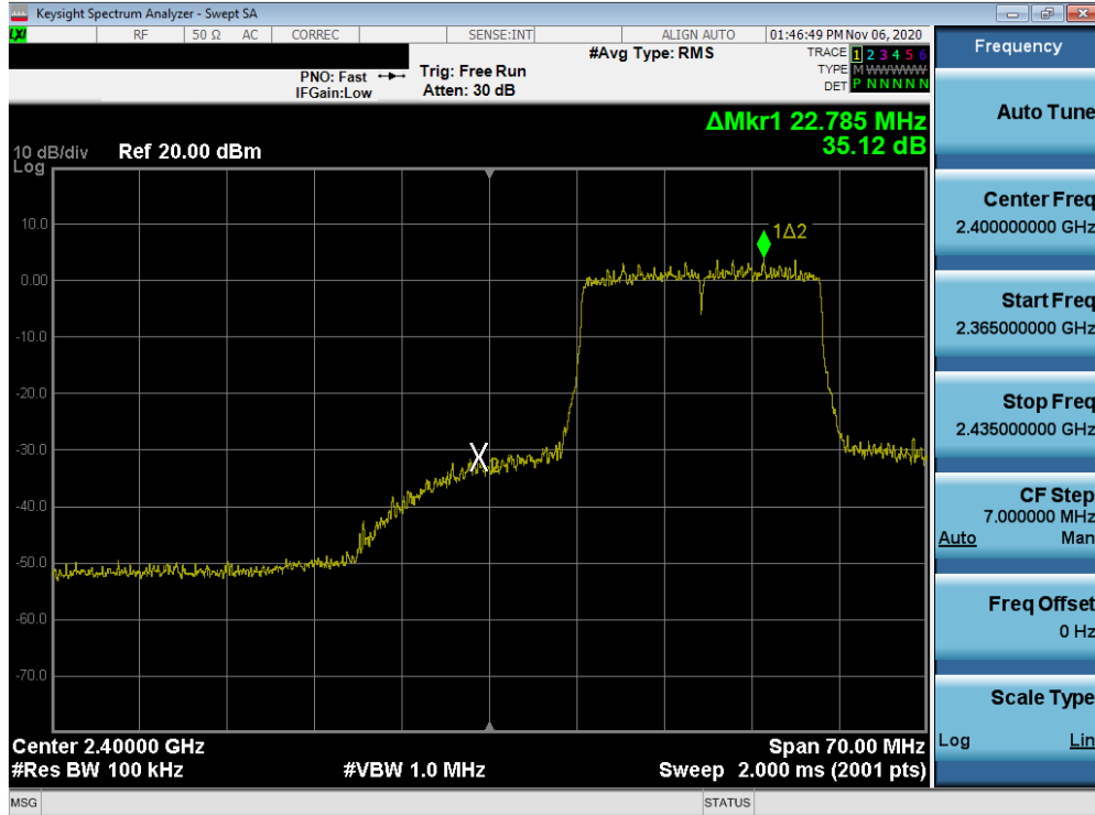
Plot 7-76. Band Edge Plot SISO ANT2 (802.11ax (2.4GHz) – Ch. 2)
