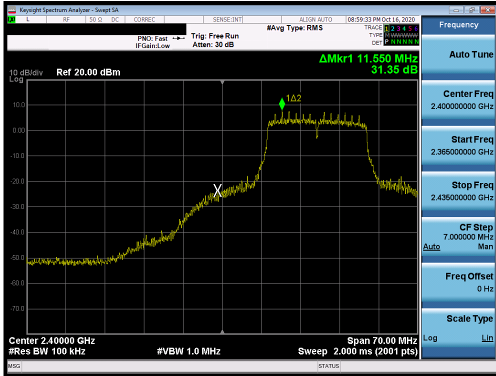
Plot 7-56. Band Edge Plot SISO ANT1 (802.11n (2.4GHz) – Ch. 2)
