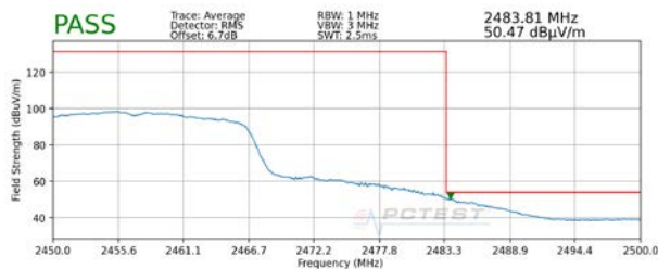
Plot 7-133. Radiated Restricted Band Edge Measurement MIMO with WCP (Average)
