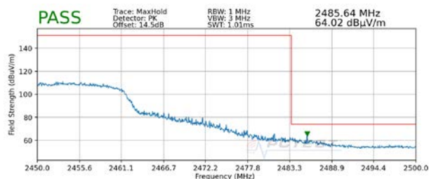
Plot 7-112. Radiated Restricted Upper Band Edge Measurement SISO ANT1 (Peak)
