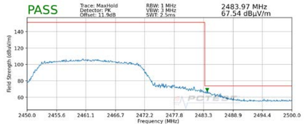
Plot 7-124. Radiated Restricted Upper Band Edge Measurement SISO ANT2 (Peak)
