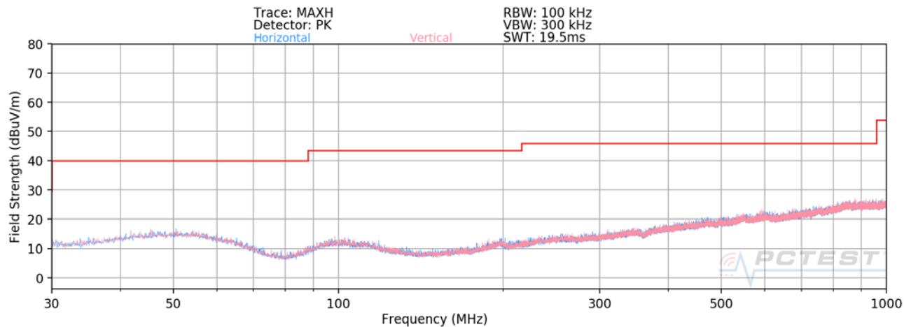
Plot 7-135. Radiated Spurious Plot below 1GHz MIMO
