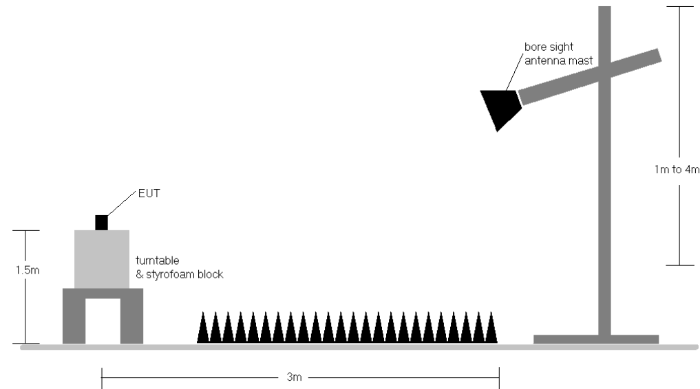
Figure 7-6. Test Instrument & Measurement Setup
