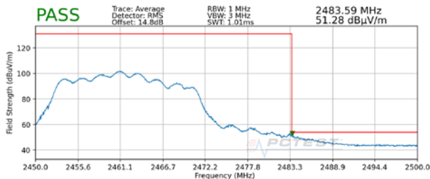
Plot 7-131. Radiated Restricted Upper Band Edge Measurement MIMO (Average)
