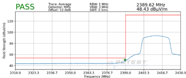
Plot 7-117. Radiated Restricted Lower Band Edge Measurement SISO ANT2 (Average)
