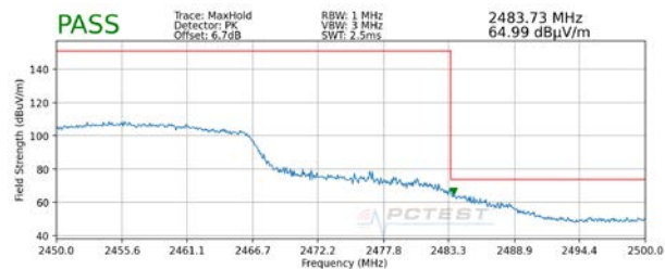
Plot 7-134. Radiated Restricted Band Edge Measurement MIMO with WCP (Peak)
