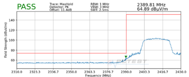
Plot 7-118. Radiated Restricted Lower Band Edge Measurement SISO ANT2 (Peak)
