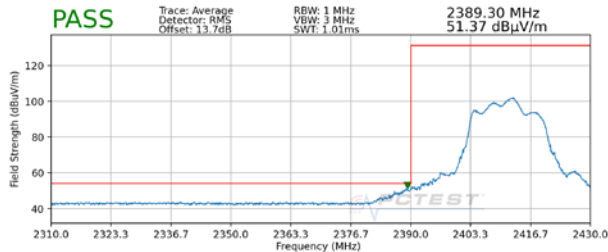
Plot 7-125. Radiated Restricted Lower Band Edge Measurement MIMO (Average)
