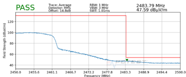
Plot 7-111. Radiated Restricted Upper Band Edge Measurement SISO ANT1 (Average)
