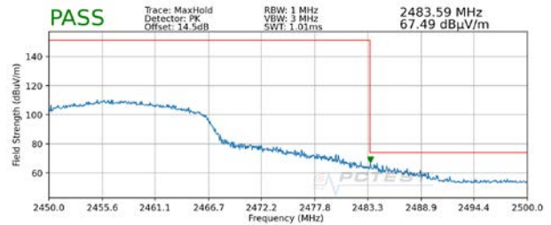
Plot 7-114. Radiated Restricted Upper Band Edge Measurement SISO ANT1 (Peak)
