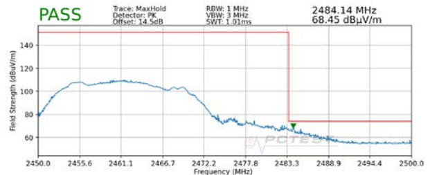
Plot 7-132. Radiated Restricted Upper Band Edge Measurement MIMO (Peak)
