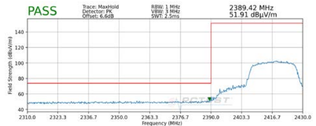
Plot 7-120. Radiated Restricted Lower Band Edge Measurement SISO ANT2 (Peak)
