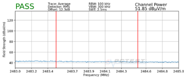
Plot 7-115. Radiated Restricted Upper Band Edge Measurement SISO ANT1 (Average)
