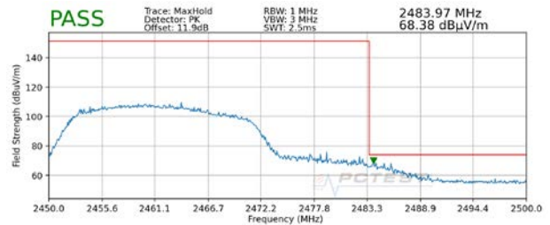
Plot 7-116. Radiated Restricted Upper Band Edge Measurement SISO ANT1 (Peak)
