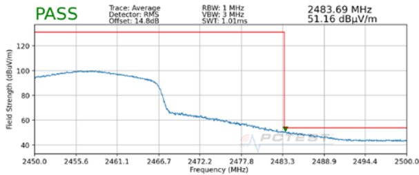
Plot 7-113. Radiated Restricted Upper Band Edge Measurement SISO ANT1 (Average)
