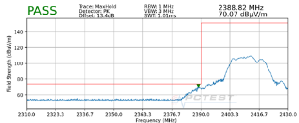
Plot 7-126. Radiated Restricted Lower Band Edge Measurement MIMO (Peak)
