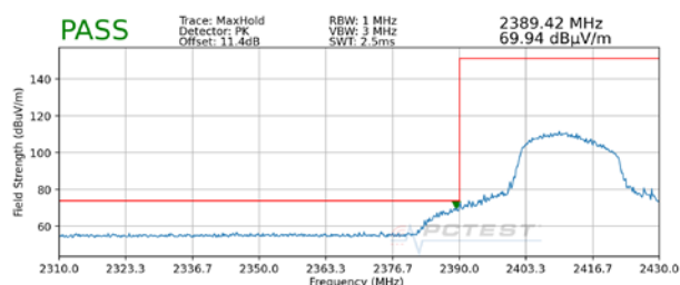
Plot 7-106. Radiated Restricted Lower Band Edge Measurement SISO ANT1 (Peak)
