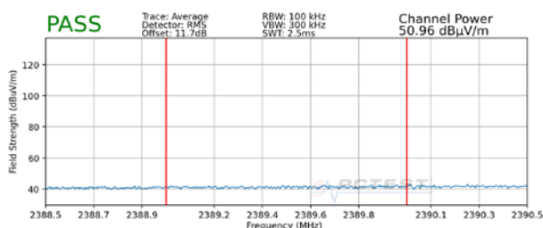
Plot 7-105. Radiated Restricted Lower Band Edge Measurement SISO ANT1 (Average)
