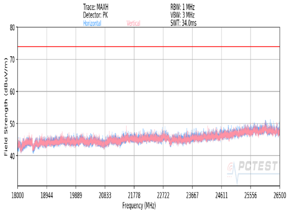
Plot 7-104. Radiated Spurious Plot above 18GHz MIMO/CDD
