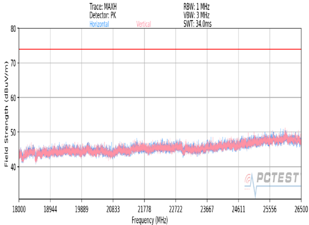
Plot 7-100. Radiated Spurious Plot above 18GHz SISO ANT2
