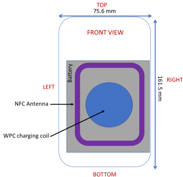
Figure E-2 NFC Antenna Locations
