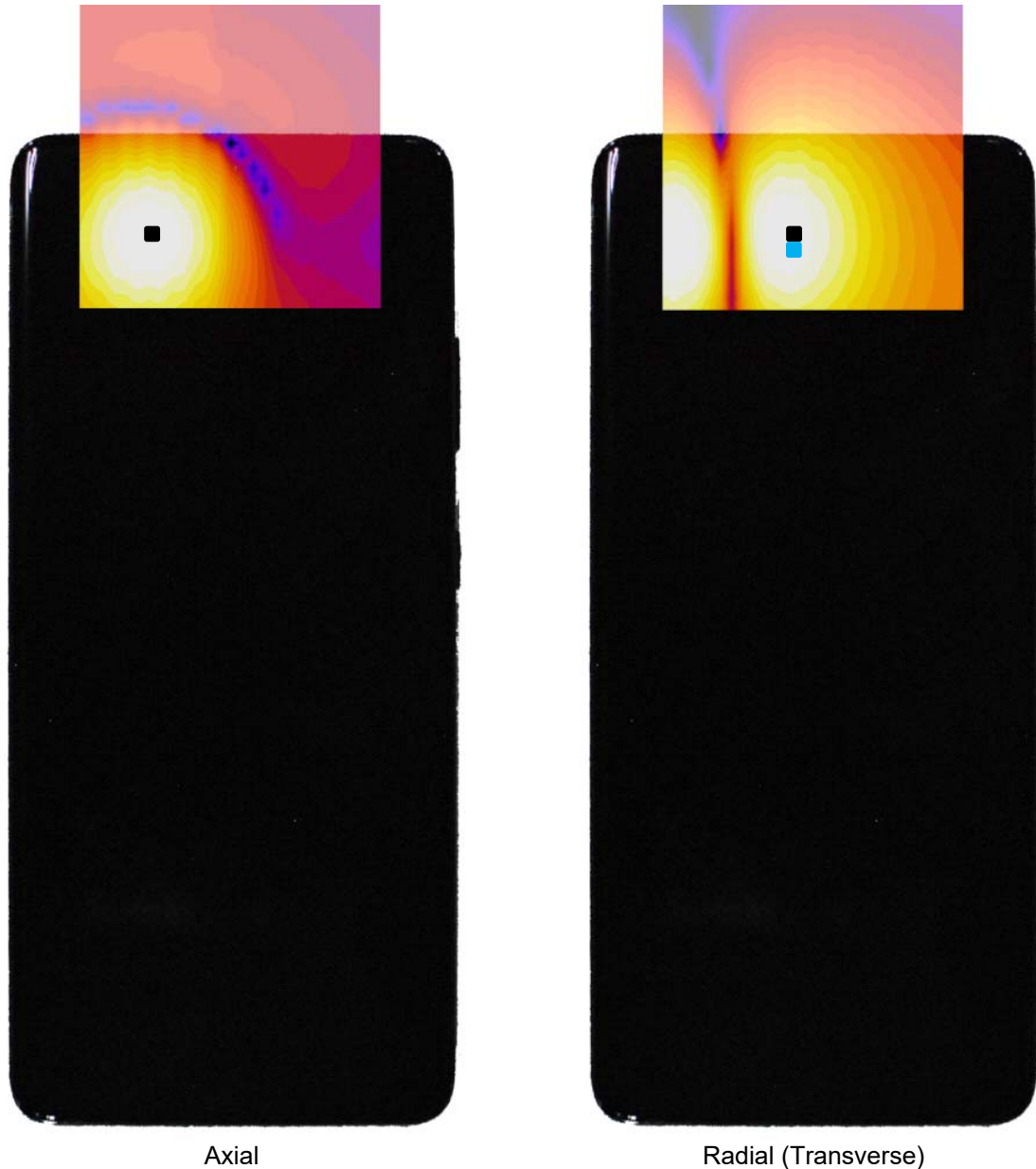
Figure 16-3 T-Coil Scan Overlay Magnetic Field Distributions
