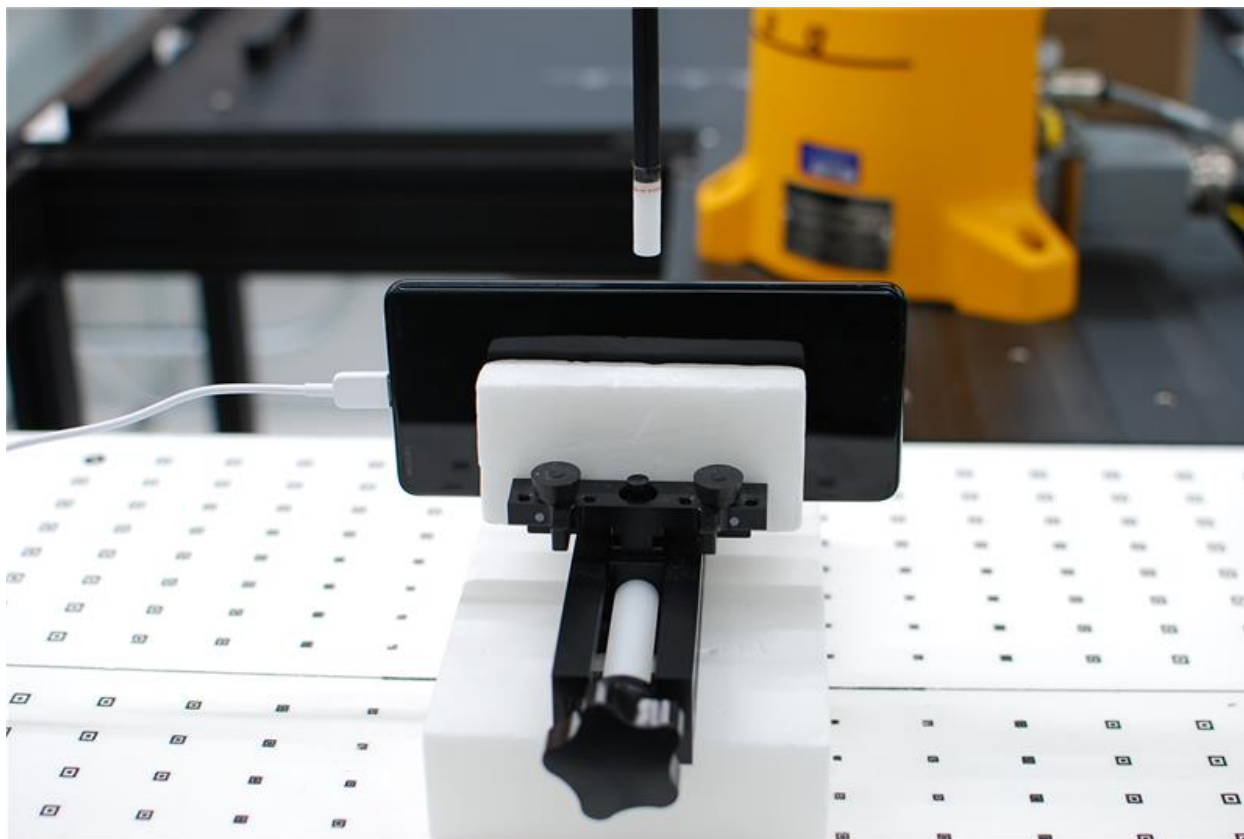
Figure D-8 Near Field Power Density Test Setup Photo - Left at 10mm
