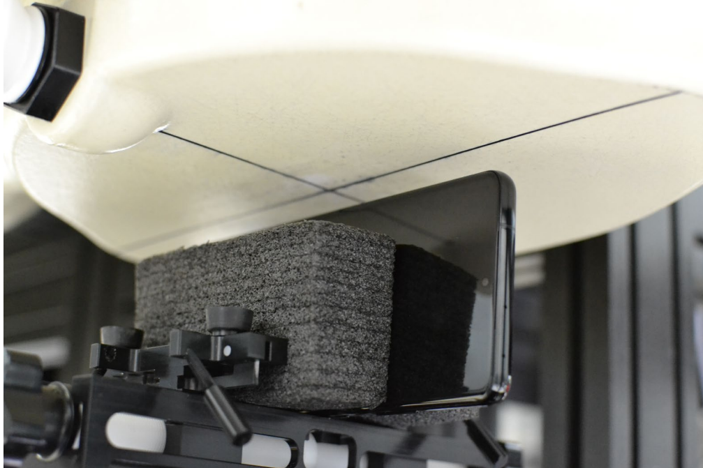
SAR Test Setup Photo 9 – Left Side at 10 mm
