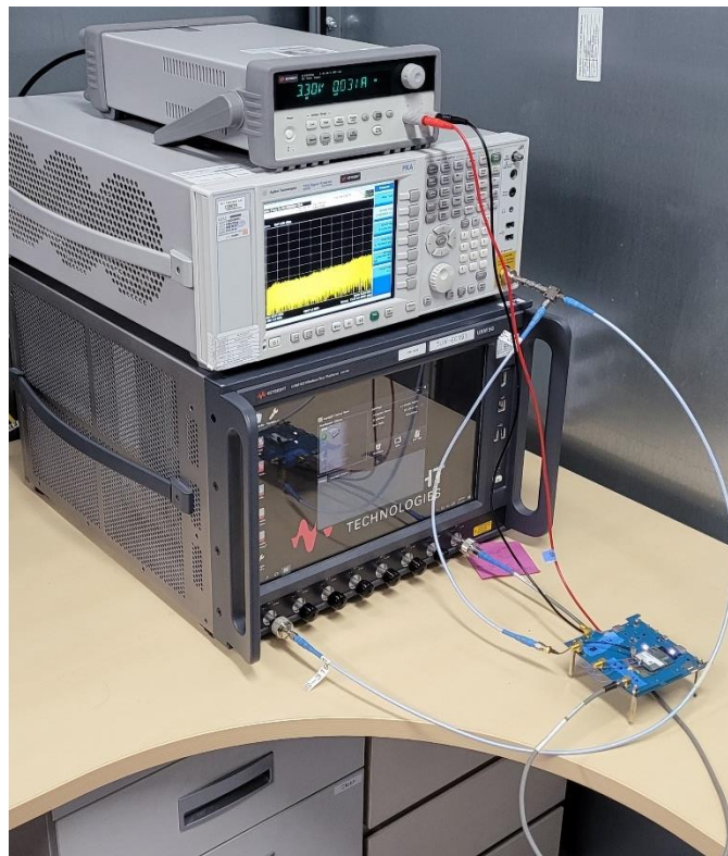
LICENSED BAND TEST PHOTO
