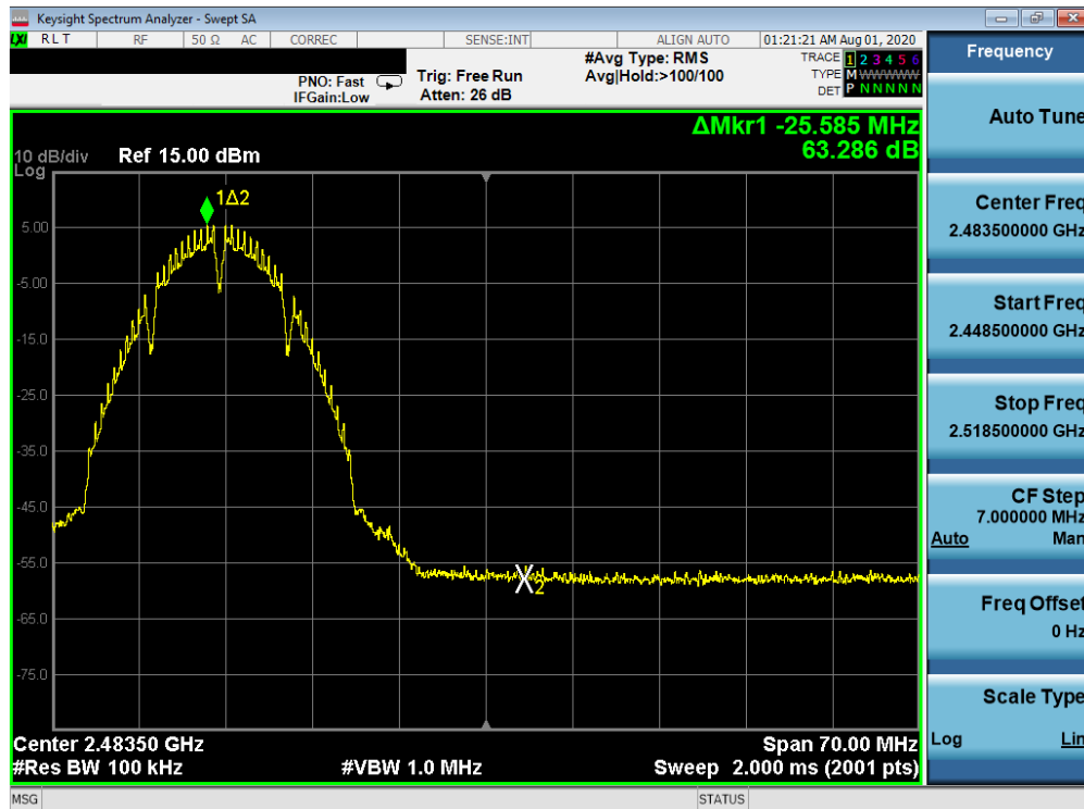
Plot 7-114. Band Edge Plot ANT2 (802.11b – Ch. 11)
