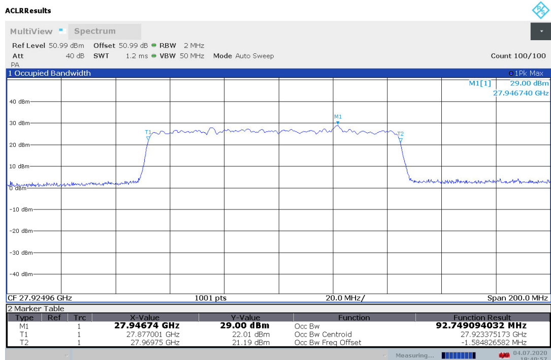
Plot 7-1. Occupied Bandwidth Plot (100MHz-1CC – \pi/2 BPSK – Mid Channel)
