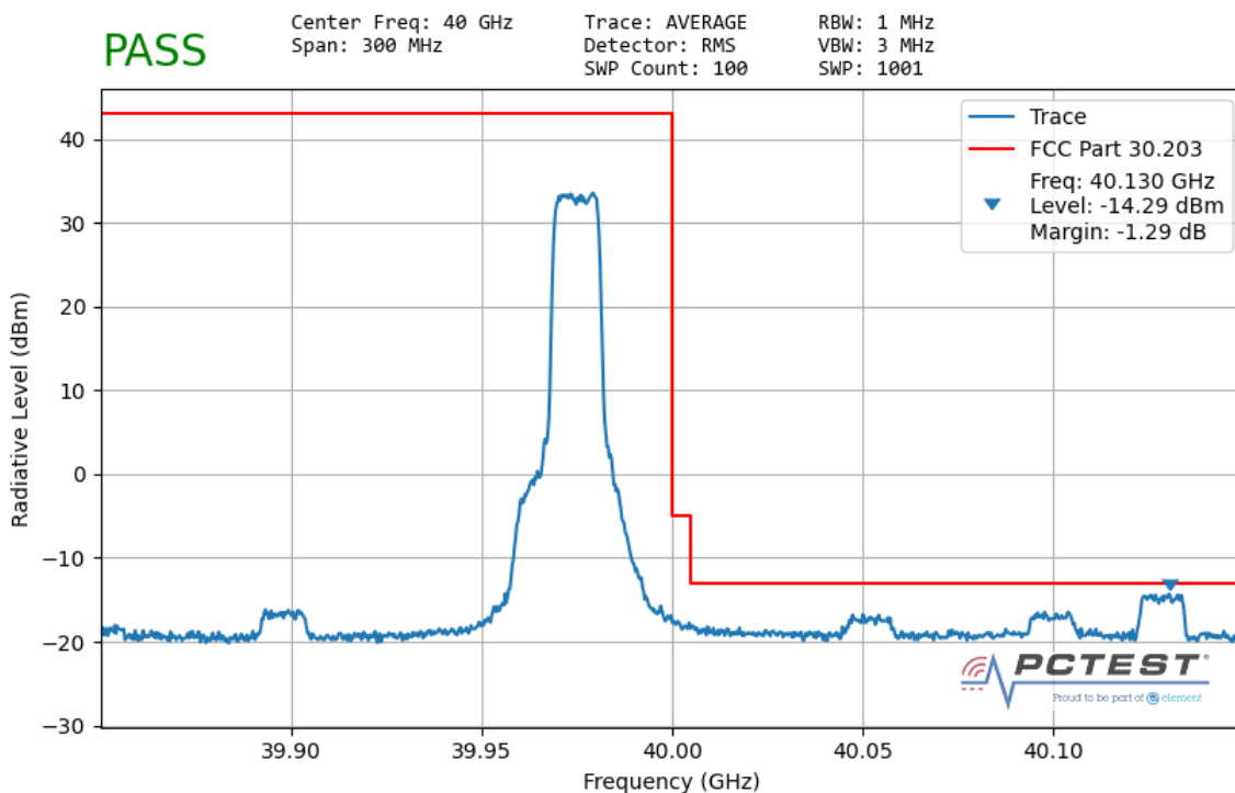
Plot 7-47. Upper Band Edge (50MHz-1CC – QPSK 8 RB)
