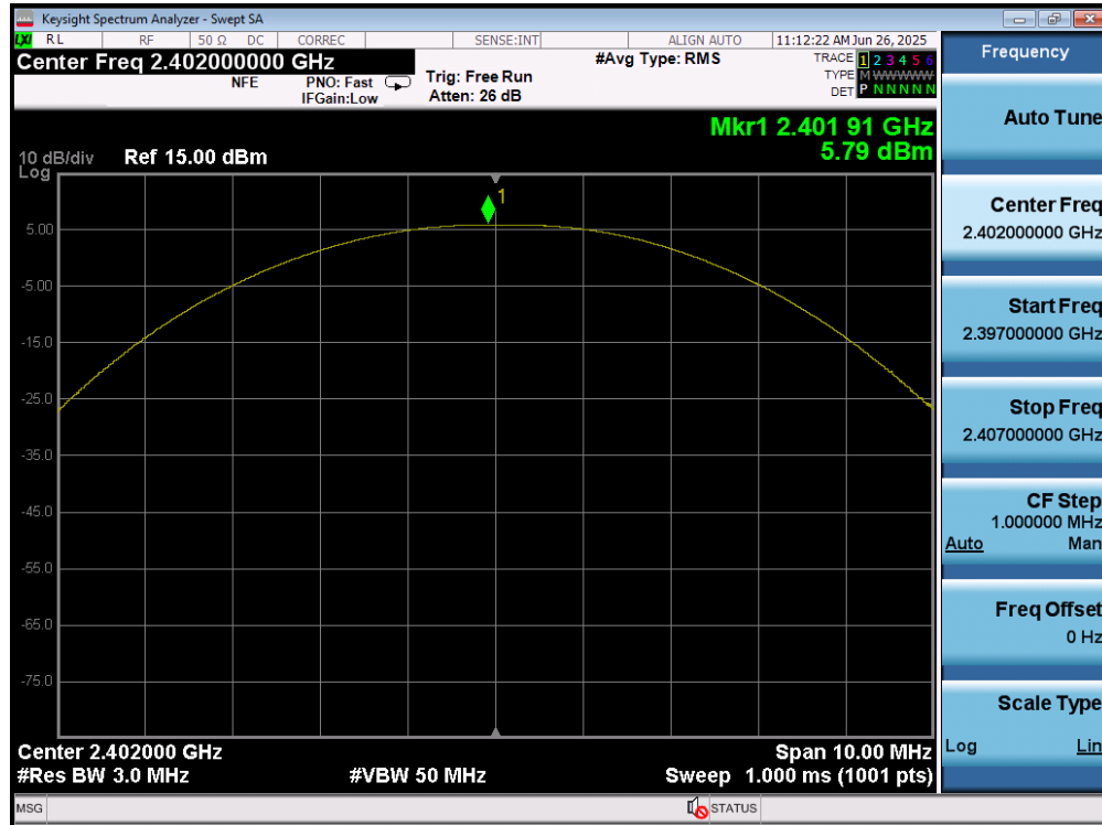
Plot 7-61. Peak Power Plot (Bluetooth (LE), 1Mbps – Ch. 37) – Dual Ant 1
