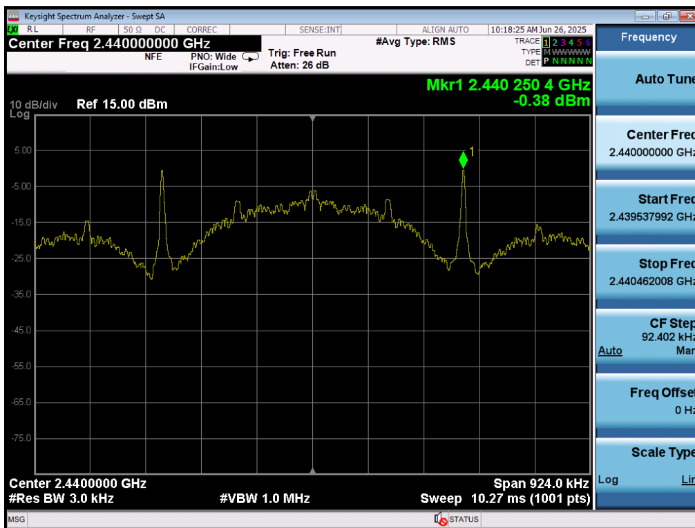
Plot 7-74. Power Spectral Density Plot (Bluetooth (LE), 125kbps – Ch. 19) – Ant 1
