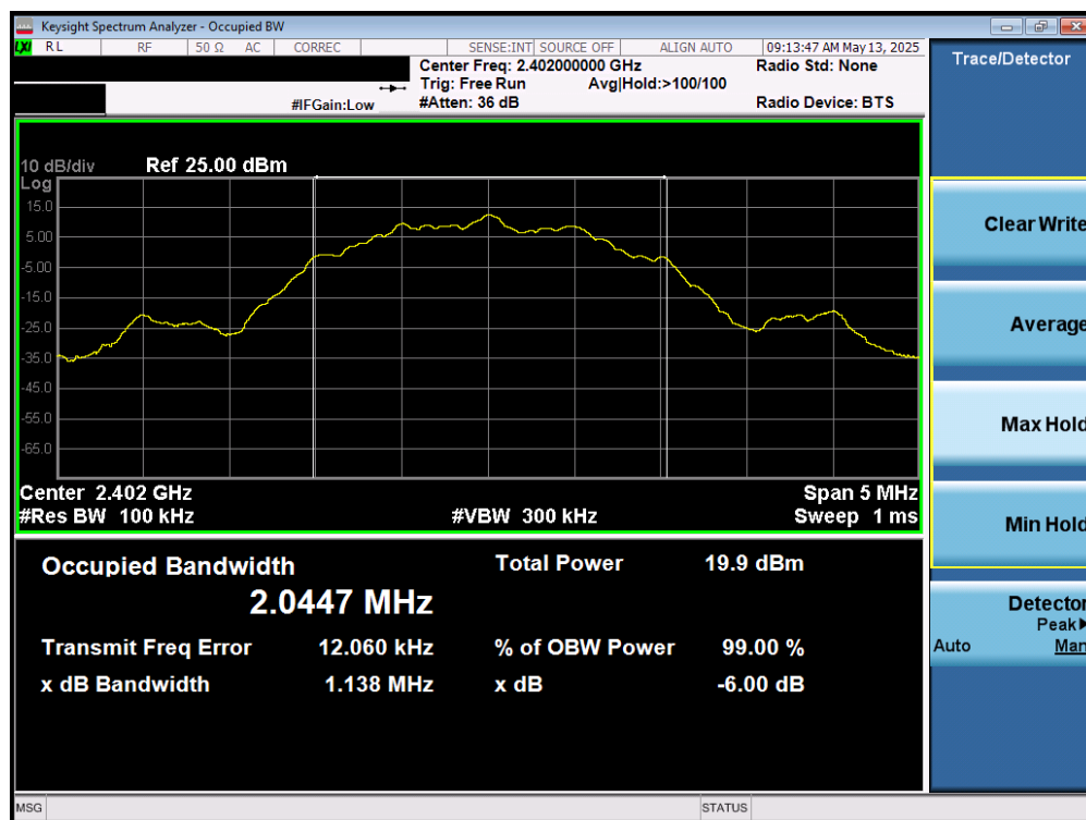
Plot 7-34. 6dB Bandwidth Plot (Bluetooth (LE), 2Mbps – Ch. 37) – Dual Ant 2
