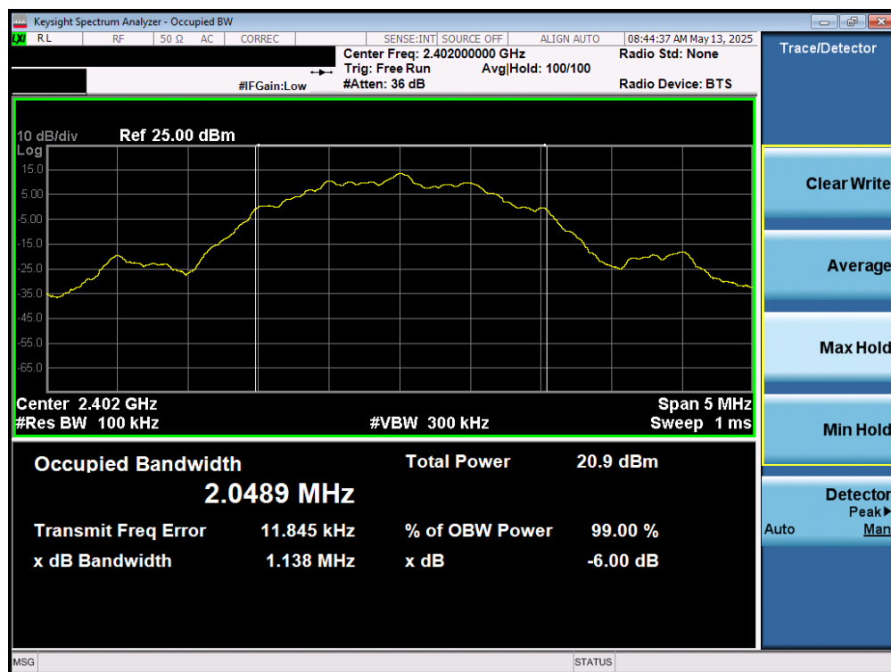
Plot 7-28. 6dB Bandwidth Plot (Bluetooth (LE), 2Mbps – Ch. 37) – Dual Ant 1
