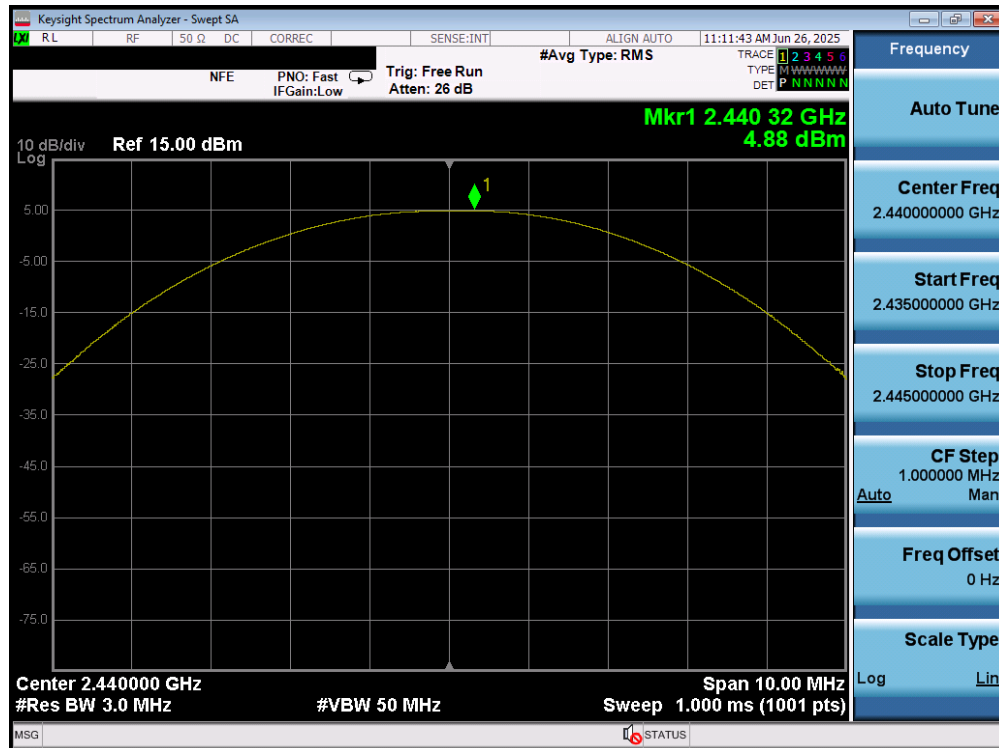
Plot 7-62. Peak Power Plot (Bluetooth (LE), 1Mbps – Ch. 17) – Dual Ant 1
