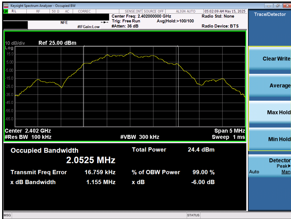
Plot 7-10. 6dB Bandwidth Plot (Bluetooth (LE), 2Mbps – Ch. 37) – Ant 1
