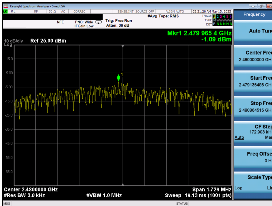
Plot 7-96. Power Spectral Density Plot (Bluetooth (LE), 2Mbps – Ch. 39) – Ant 2
