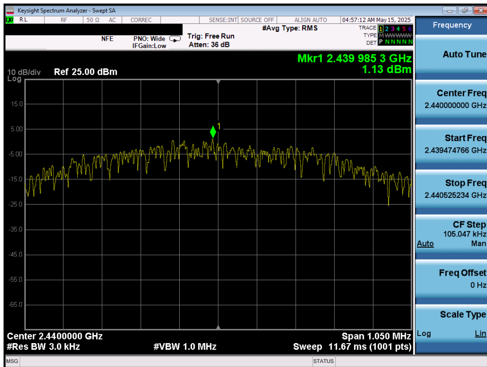
Plot 7-80. Power Spectral Density Plot (Bluetooth (LE), 1Mbps – Ch. 17) – Ant 1
