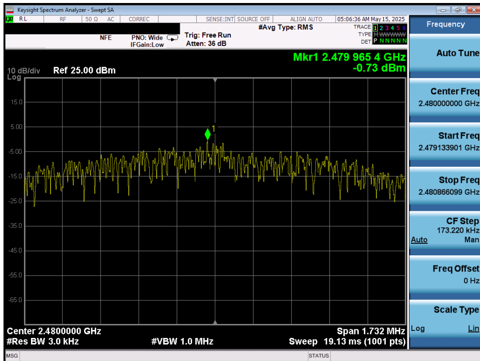
Plot 7-84. Power Spectral Density Plot (Bluetooth (LE), 2Mbps – Ch. 39) – Ant 1
