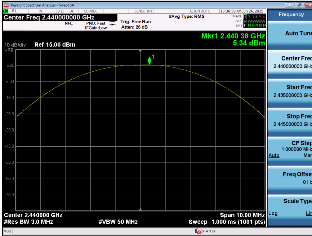
Plot 7-53. Peak Power Plot (Bluetooth (LE), 500kbps – Ch. 19) – Ant 2
