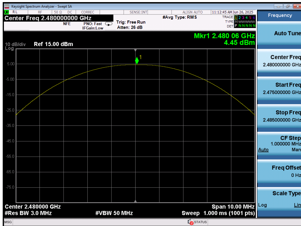
Plot 7-63. Peak Power Plot (Bluetooth (LE), 1Mbps – Ch. 39) – Dual Ant 1
