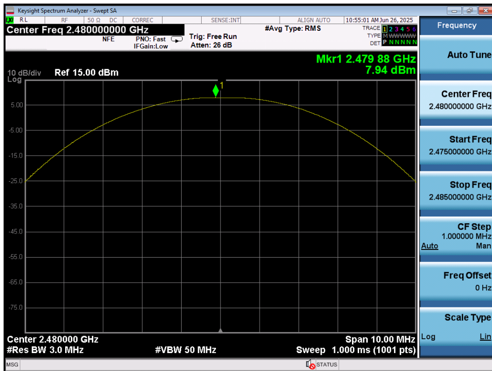
Plot 7-57. Peak Power Plot (Bluetooth (LE), 1Mbps – Ch. 39) – Ant 2
