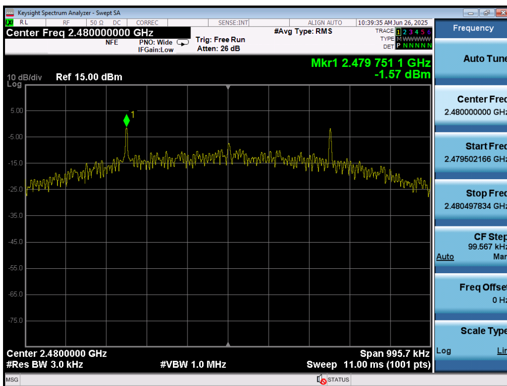
Plot 7-90. Power Spectral Density Plot (Bluetooth (LE), 500kbps – Ch. 39) – Ant 2
