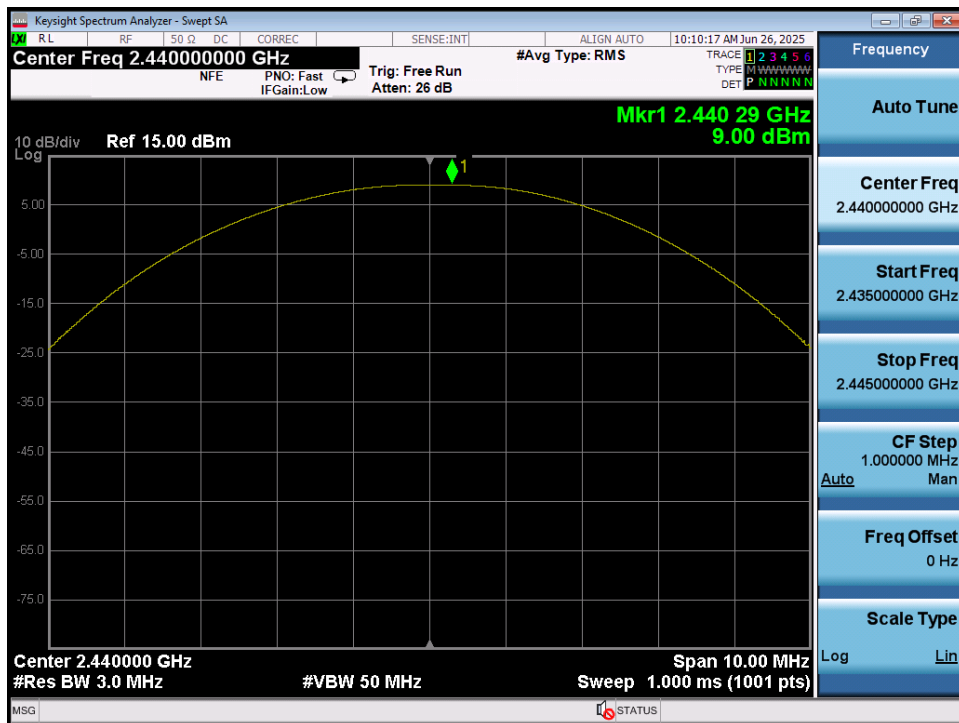
Plot 7-44. Peak Power Plot (Bluetooth (LE), 1Mbps – Ch. 17) – Ant 1
