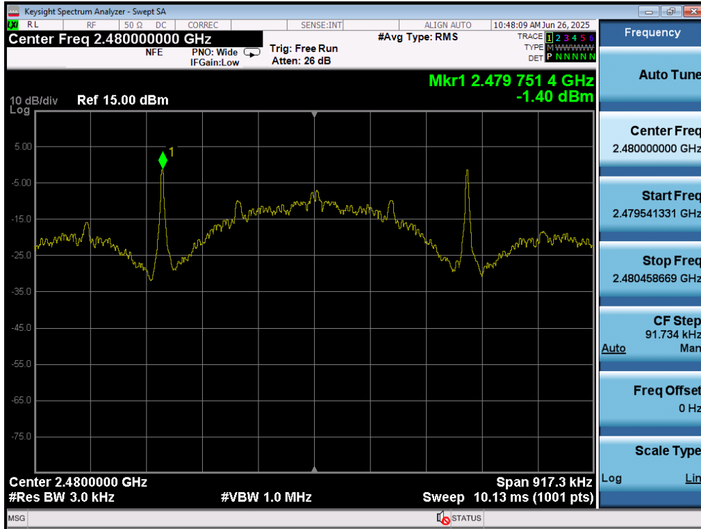
Plot 7-87. Power Spectral Density Plot (Bluetooth (LE), 125kbps – Ch. 39) – Ant 2
