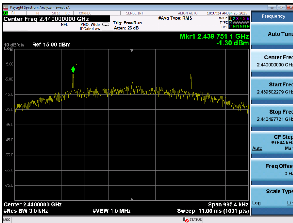
Plot 7-89. Power Spectral Density Plot (Bluetooth (LE), 500kbps – Ch. 19) – Ant 2
