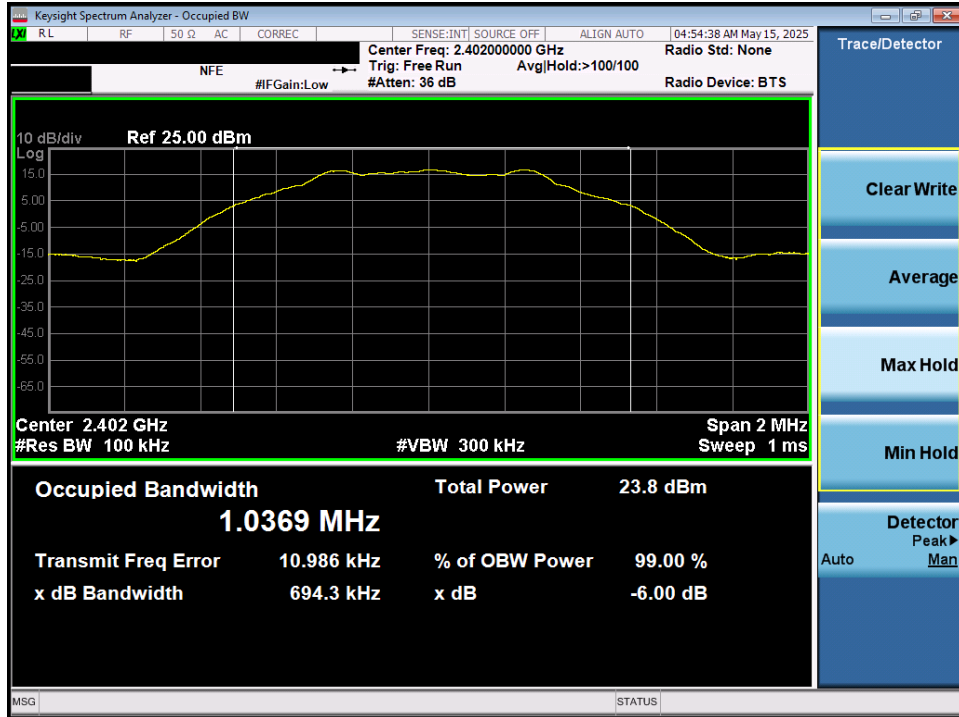
Plot 7-7. 6dB Bandwidth Plot (Bluetooth (LE), 1Mbps – Ch. 37) – Ant 1
