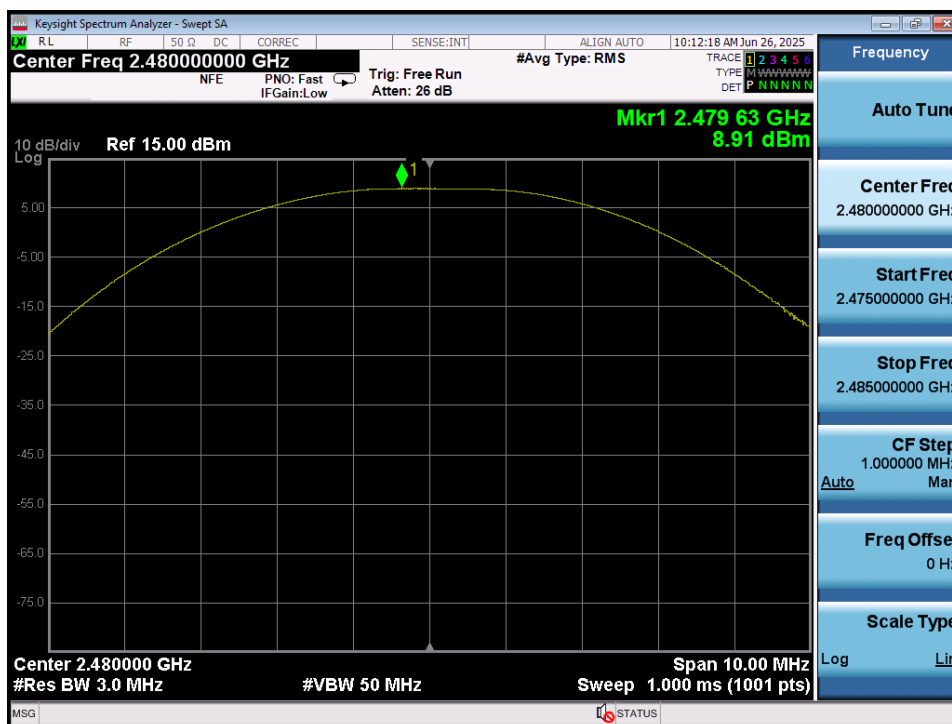
Plot 7-48. Peak Power Plot (Bluetooth (LE), 2Mbps – Ch. 39) – Ant 1
