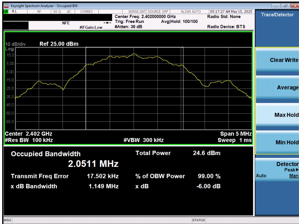
Plot 7-22. 6dB Bandwidth Plot (Bluetooth (LE), 2Mbps – Ch. 37) – Ant 2
