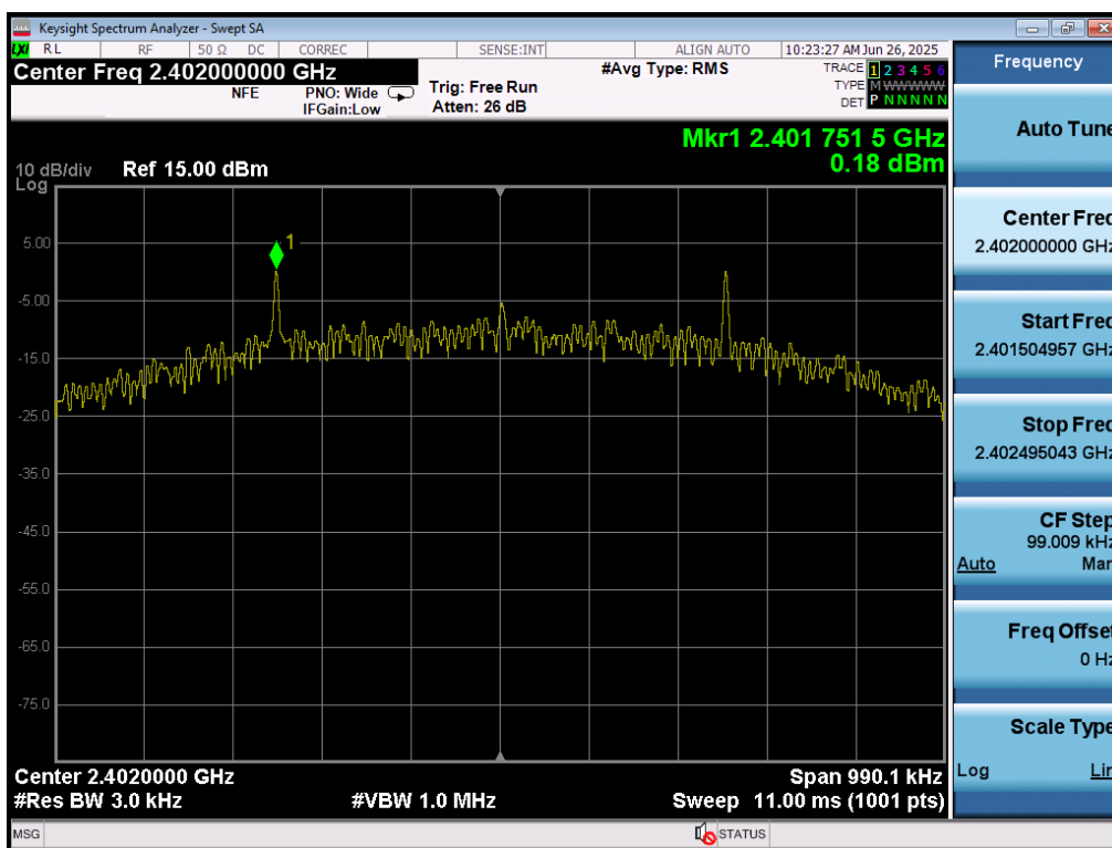
Plot 7-76. Power Spectral Density Plot (Bluetooth (LE), 500kbps – Ch. 0) – Ant 1
