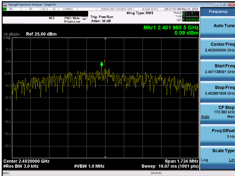
Plot 7-94. Power Spectral Density Plot (Bluetooth (LE), 2Mbps – Ch. 37) – Ant 2
