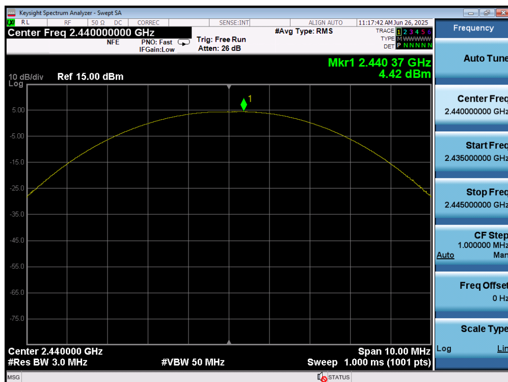
Plot 7-68. Peak Power Plot (Bluetooth (LE), 1Mbps – Ch. 17) – Dual Ant 2
