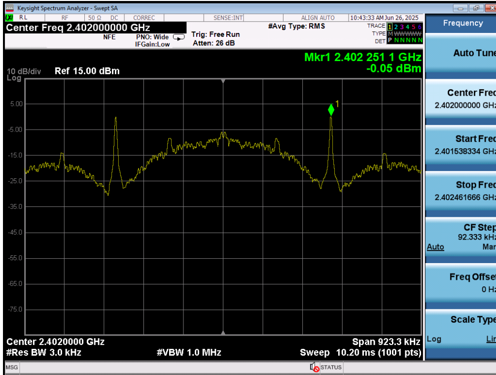
Plot 7-85. Power Spectral Density Plot (Bluetooth (LE), 125kbps – Ch. 0) – Ant 2
