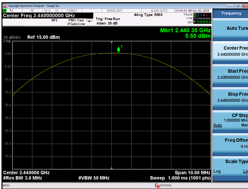
Plot 7-50. Peak Power Plot (Bluetooth (LE), 125kbps - Ch. 19) - Ant 2
