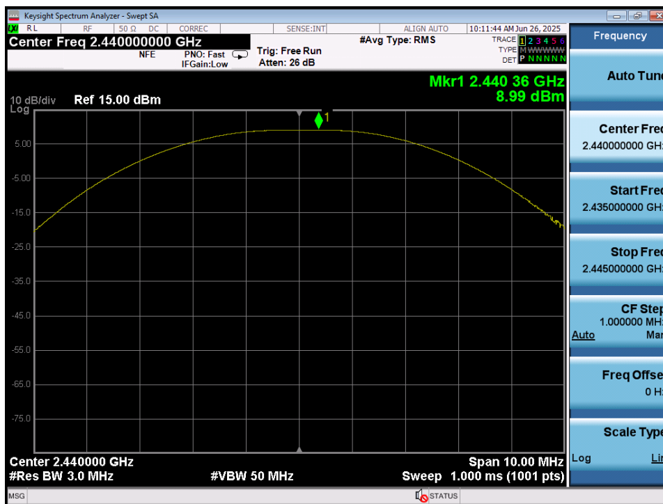
Plot 7-47. Peak Power Plot (Bluetooth (LE), 2Mbps – Ch. 17) – Ant 1
