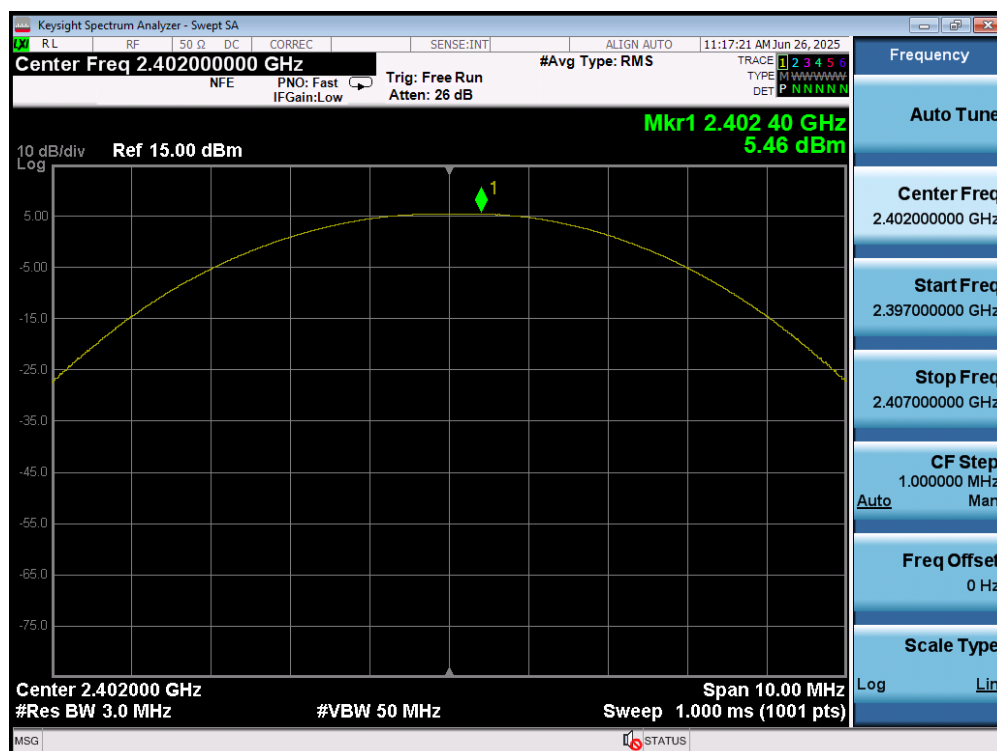
Plot 7-67. Peak Power Plot (Bluetooth (LE), 1Mbps – Ch. 37) – Dual Ant 2
