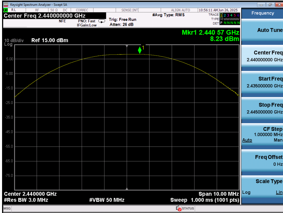
Plot 7-59. Peak Power Plot (Bluetooth (LE), 2Mbps – Ch. 17) – Ant 2
