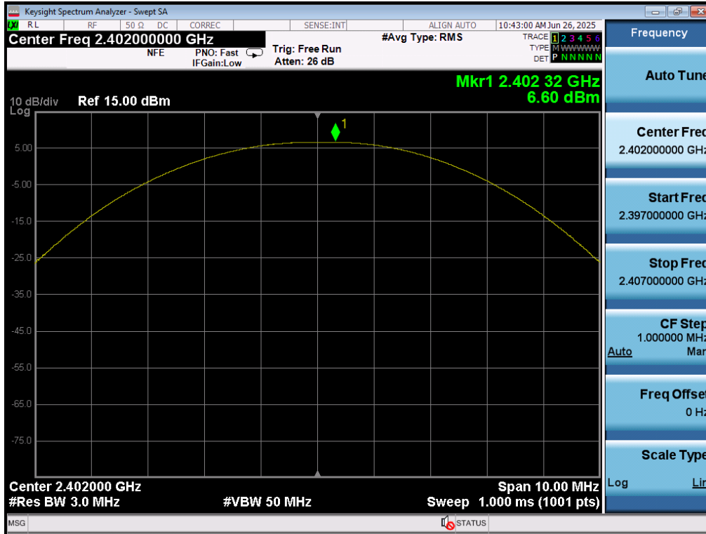
Plot 7-49. Peak Power Plot (Bluetooth (LE), 125kbps - Ch. 0) - Ant 2
