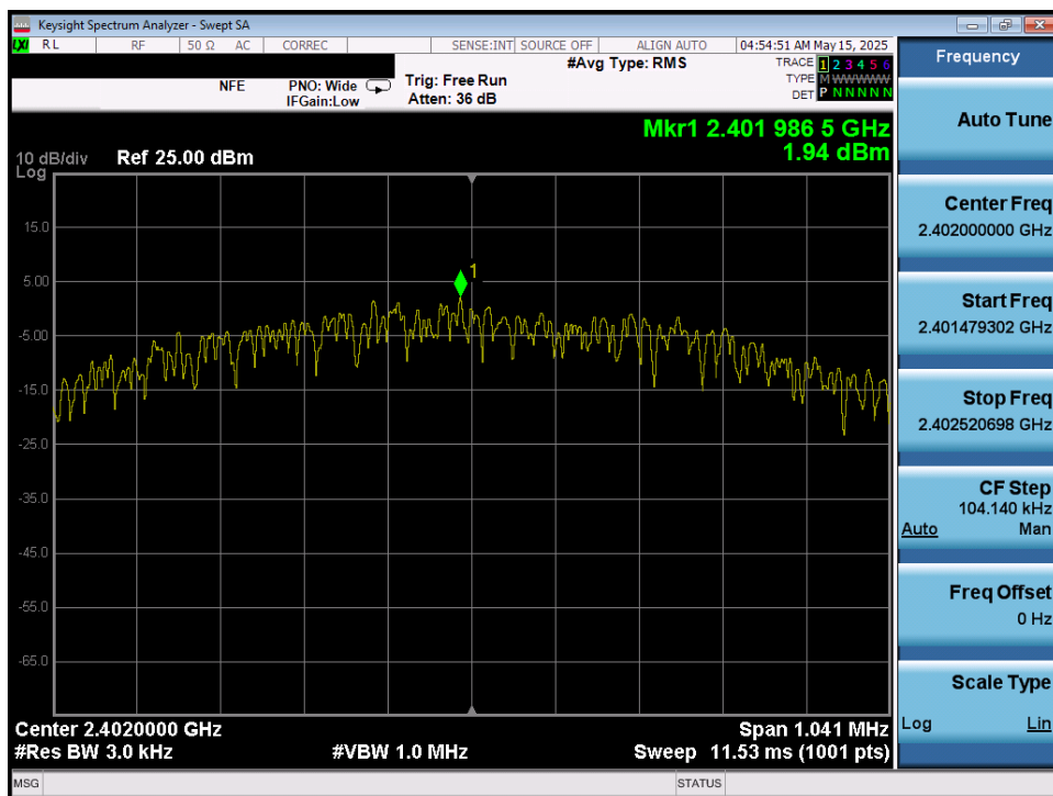
Plot 7-79. Power Spectral Density Plot (Bluetooth (LE), 1Mbps – Ch. 37) – Ant 1
