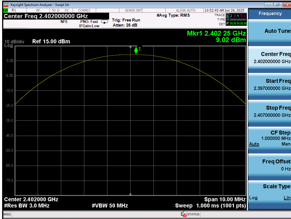
Plot 7-55. Peak Power Plot (Bluetooth (LE), 1Mbps – Ch. 37) – Ant 2
