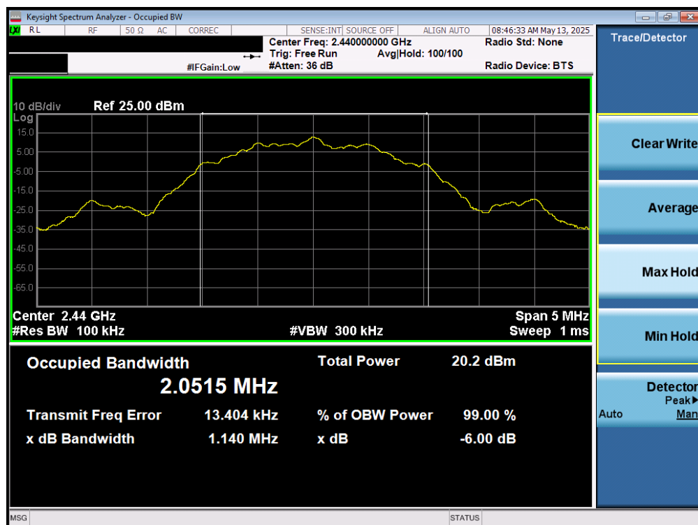
Plot 7-29. 6dB Bandwidth Plot (Bluetooth (LE), 2Mbps – Ch. 17) – Dual Ant 1
