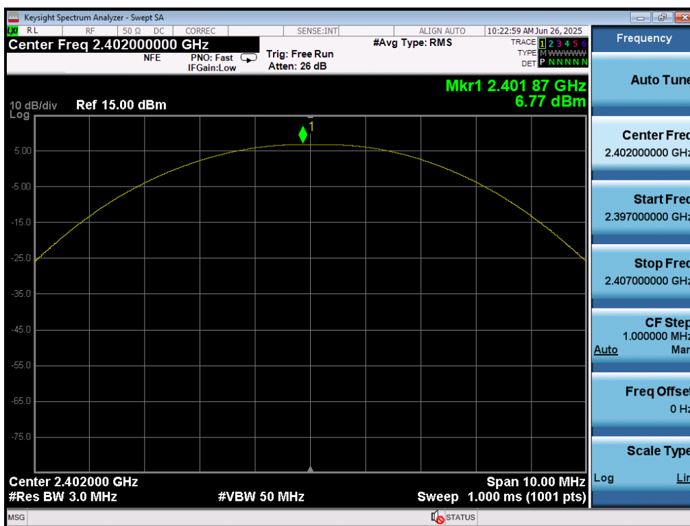
Plot 7-40. Peak Power Plot (Bluetooth (LE), 500kbps – Ch. 0) – Ant 1
