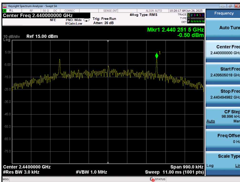
Plot 7-77. Power Spectral Density Plot (Bluetooth (LE), 500kbps – Ch. 19) – Ant 1
