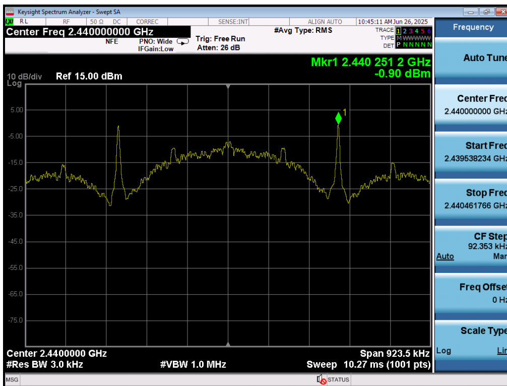
Plot 7-86. Power Spectral Density Plot (Bluetooth (LE), 125kbps – Ch. 19) – Ant 2
