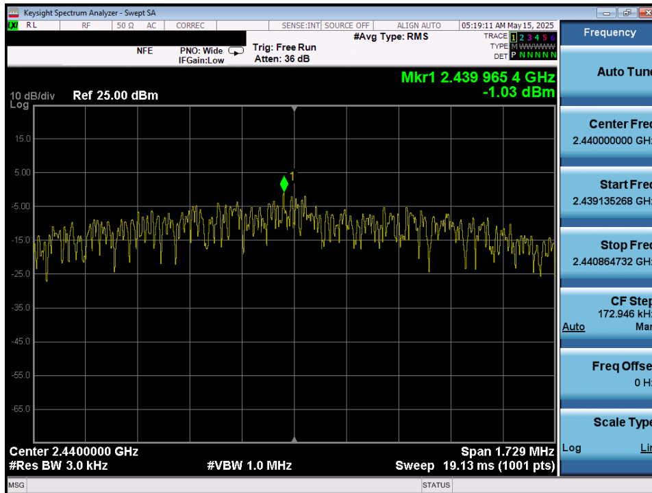
Plot 7-95. Power Spectral Density Plot (Bluetooth (LE), 2Mbps – Ch. 17) – Ant 2
