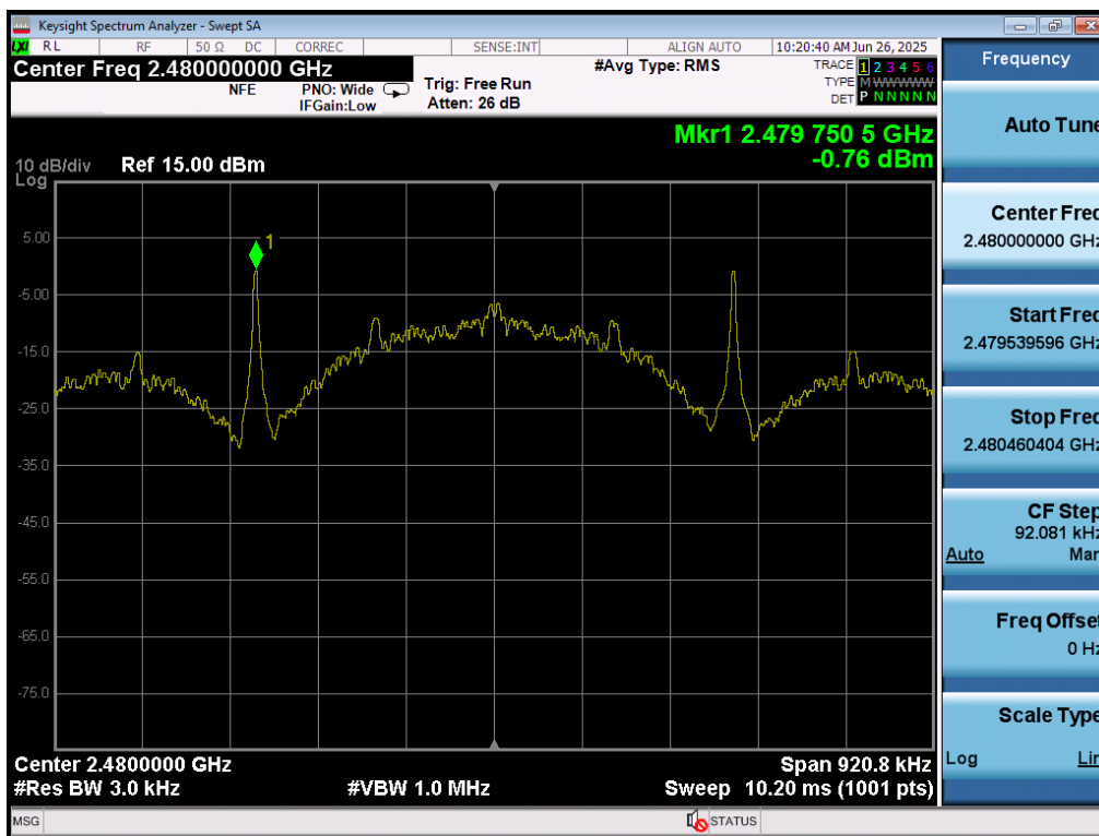
Plot 7-75. Power Spectral Density Plot (Bluetooth (LE), 125kbps – Ch. 39) – Ant 1
