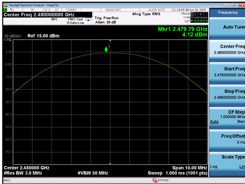
Plot 7-69. Peak Power Plot (Bluetooth (LE), 1Mbps – Ch. 39) – Dual Ant 2
