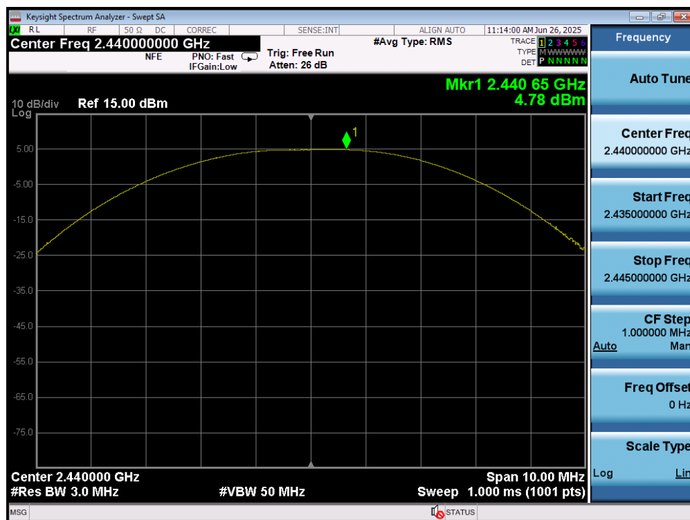
Plot 7-65. Peak Power Plot (Bluetooth (LE), 2Mbps – Ch. 17) – Dual Ant 1
