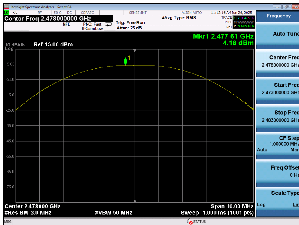
Plot 7-66. Peak Power Plot (Bluetooth (LE), 2Mbps – Ch. 39) – Dual Ant 1
