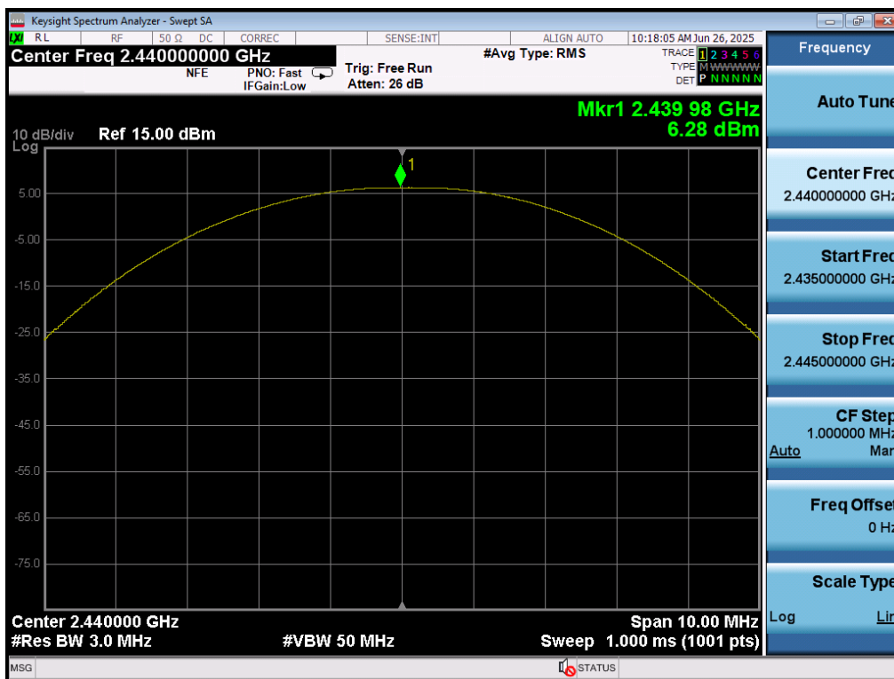
Plot 7-38. Peak Power Plot (Bluetooth (LE), 125kbps – Ch. 19) – Ant 1
