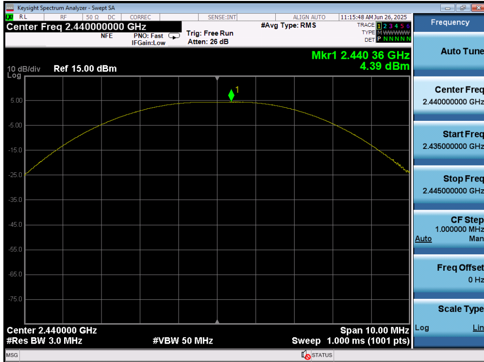
Plot 7-71. Peak Power Plot (Bluetooth (LE), 2Mbps – Ch. 17) – Dual Ant 2
