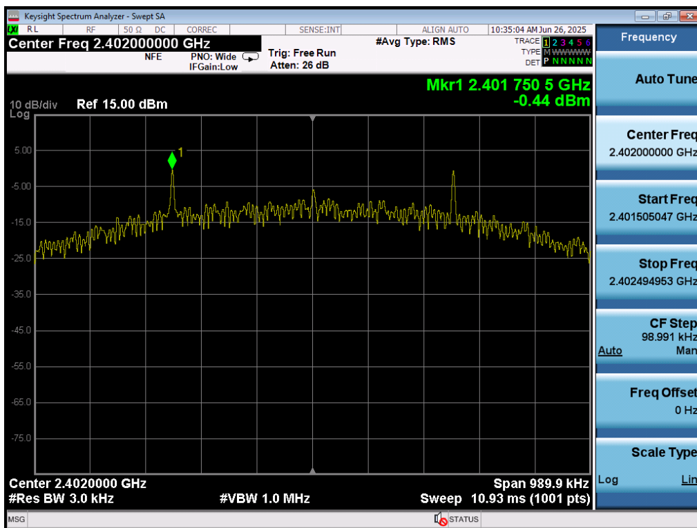
Plot 7-88. Power Spectral Density Plot (Bluetooth (LE), 500kbps – Ch. 0) – Ant 2
