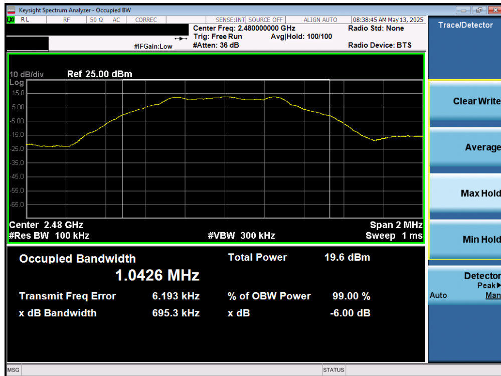
Plot 7-27. 6dB Bandwidth Plot (Bluetooth (LE), 1Mbps – Ch. 39) – Dual Ant 1
