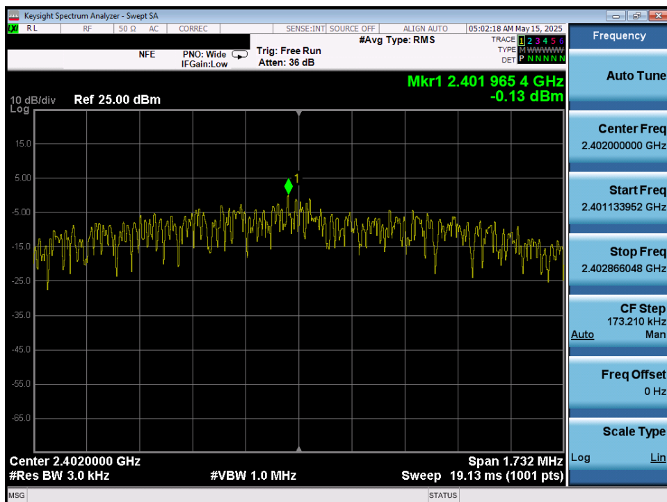
Plot 7-82. Power Spectral Density Plot (Bluetooth (LE), 2Mbps – Ch. 37) – Ant 1
