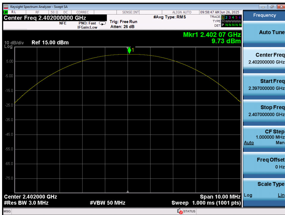
Plot 7-43. Peak Power Plot (Bluetooth (LE), 1Mbps – Ch. 37) – Ant 1
