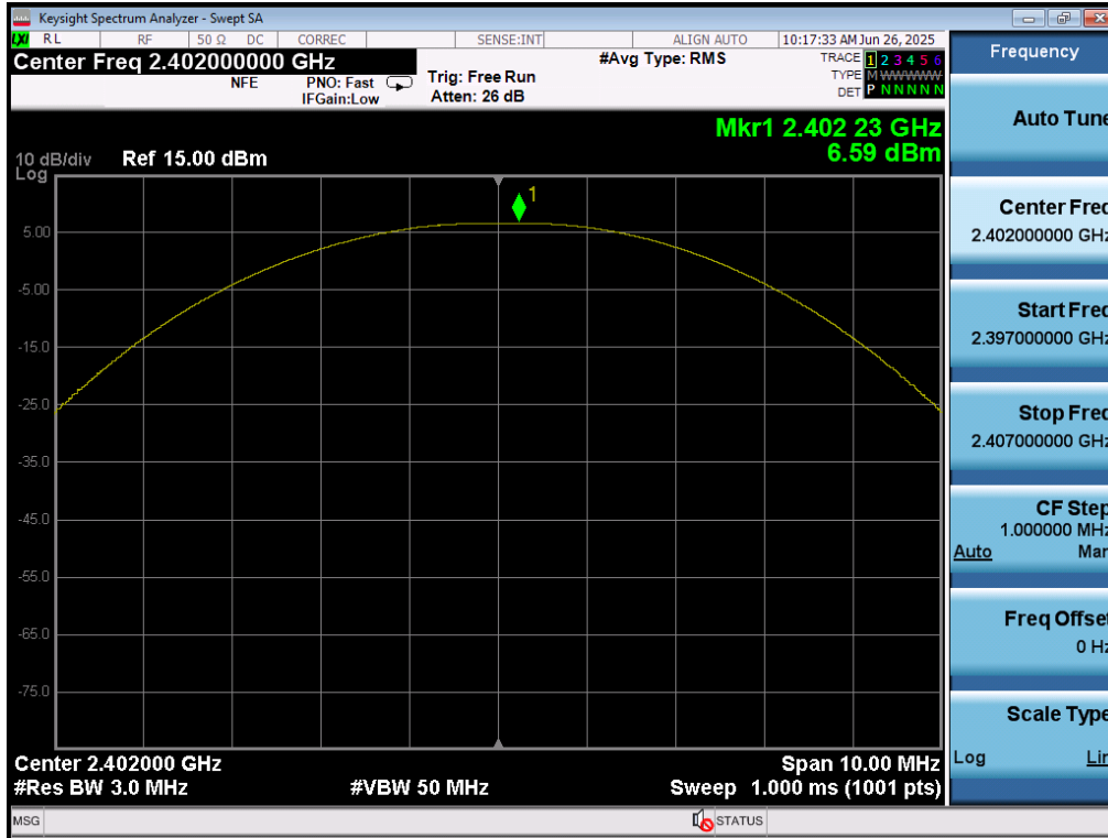
Plot 7-37. Peak Power Plot (Bluetooth (LE), 125kbps – Ch. 0) – Ant 1
