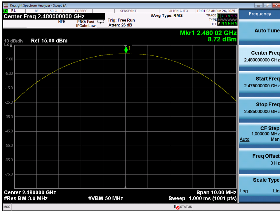
Plot 7-45. Peak Power Plot (Bluetooth (LE), 1Mbps – Ch. 39) – Ant 1
