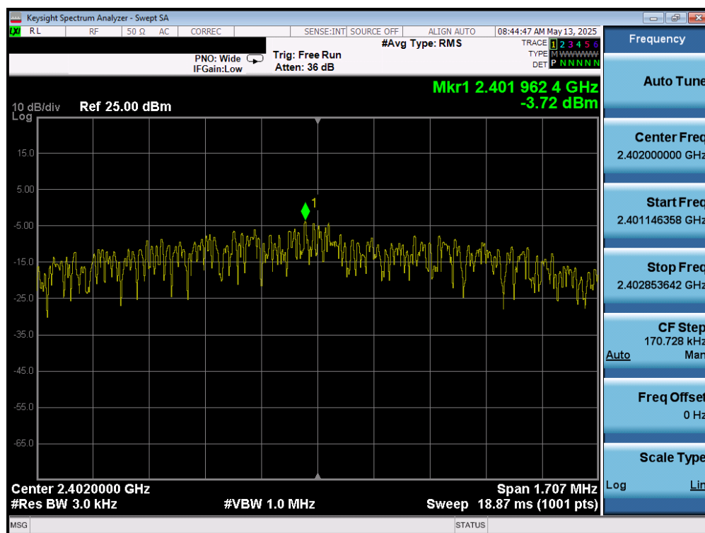
Plot 7-100. Power Spectral Density Plot (Bluetooth (LE), 2Mbps – Ch. 37) – Dual Ant 1
