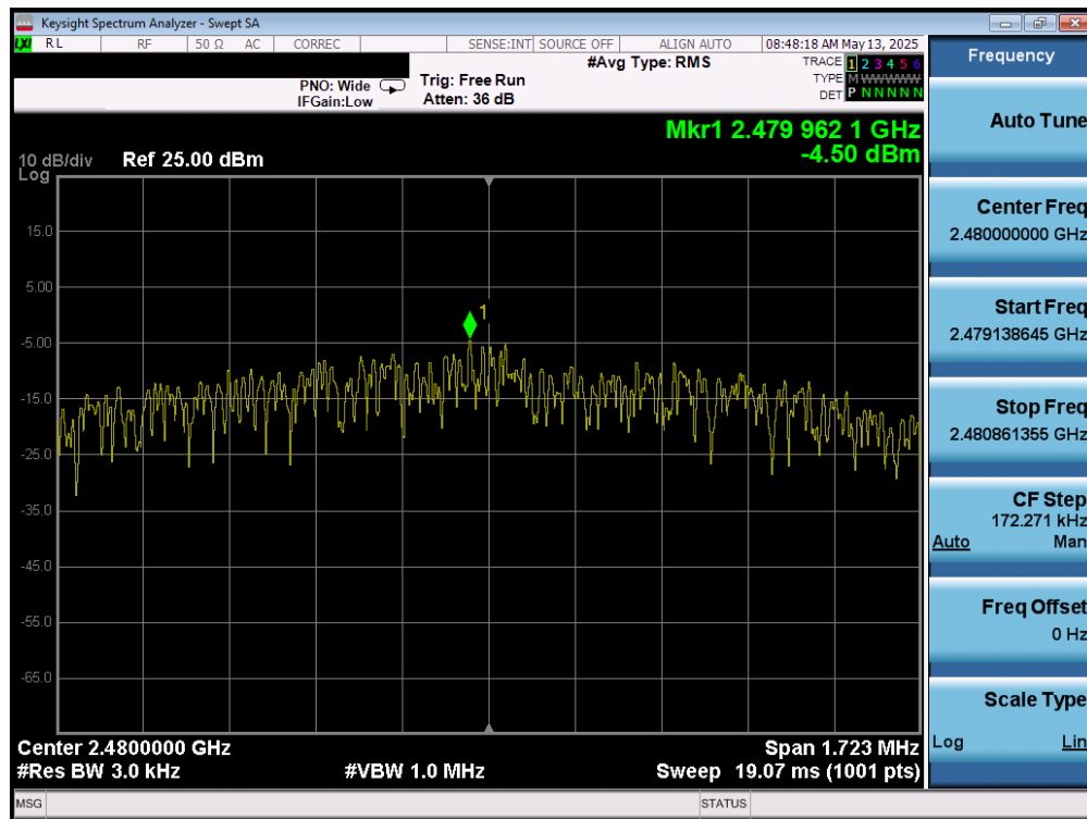
Plot 7-102. Power Spectral Density Plot (Bluetooth (LE), 2Mbps – Ch. 39) – Dual Ant 1
