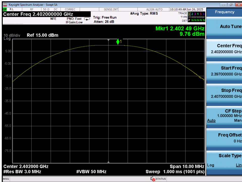
Plot 7-46. Peak Power Plot (Bluetooth (LE), 2Mbps – Ch. 37) – Ant 1
