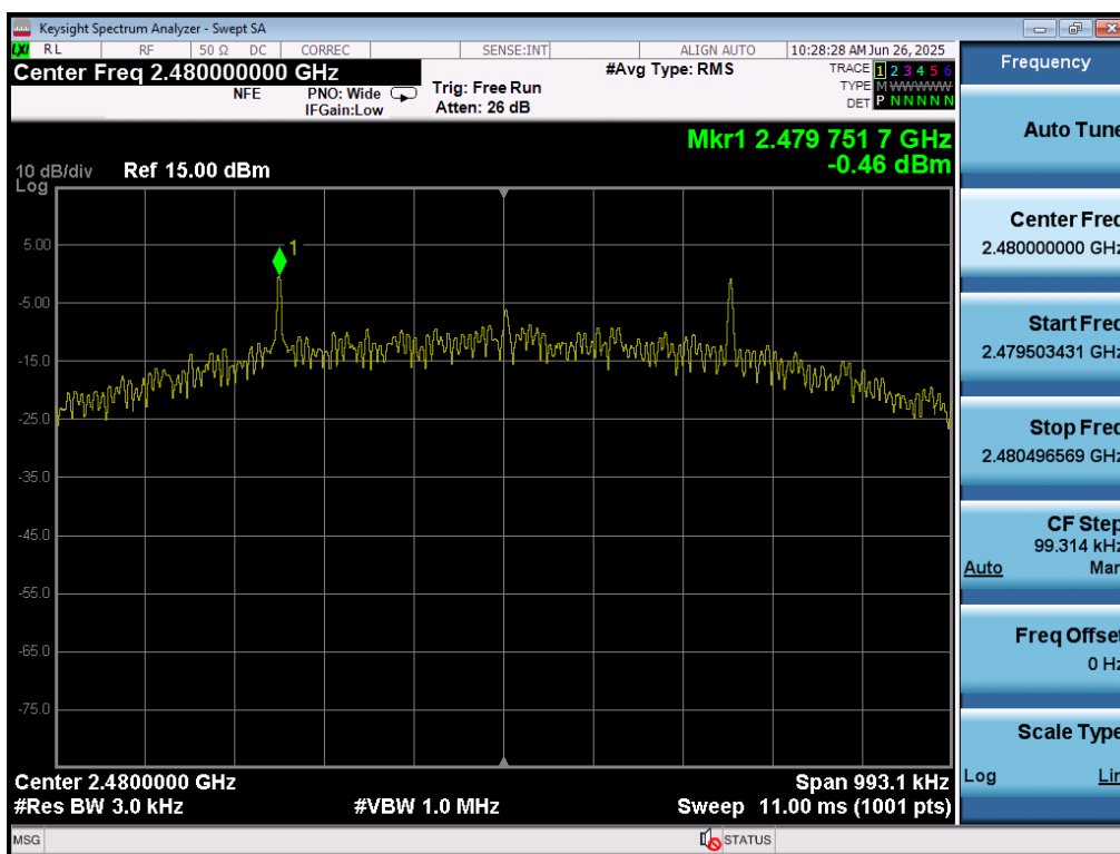
Plot 7-78. Power Spectral Density Plot (Bluetooth (LE), 500kbps – Ch. 39) – Ant 1
