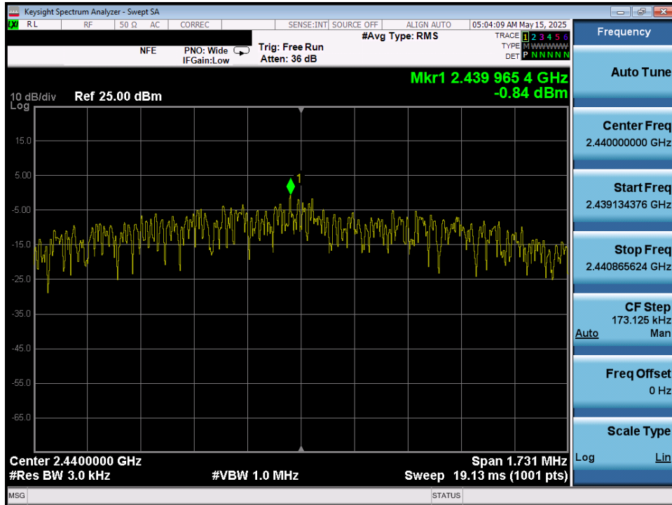
Plot 7-83. Power Spectral Density Plot (Bluetooth (LE), 2Mbps – Ch. 17) – Ant 1
