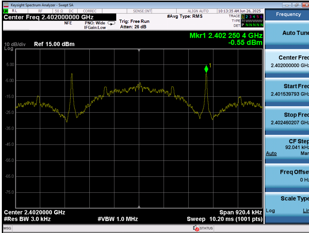
Plot 7-73. Power Spectral Density Plot (Bluetooth (LE), 125kbps – Ch. 0) – Ant 1
