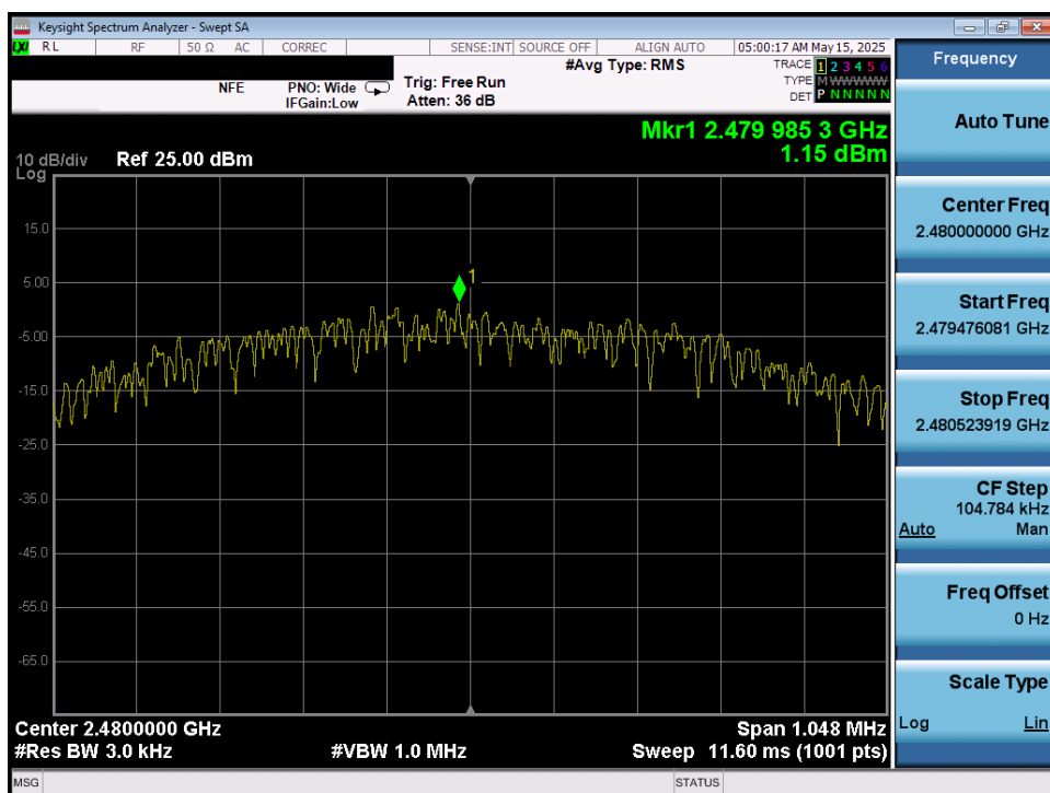
Plot 7-81. Power Spectral Density Plot (Bluetooth (LE), 1Mbps – Ch. 39) – Ant 1
