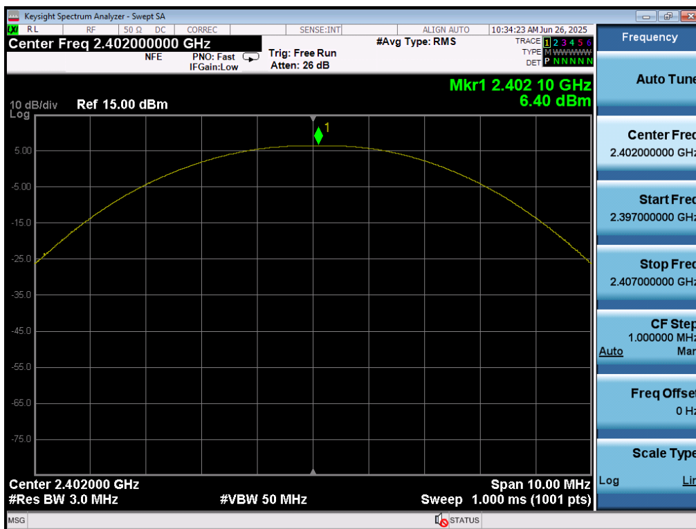
Plot 7-52. Peak Power Plot (Bluetooth (LE), 500kbps – Ch. 0) – Ant 2
