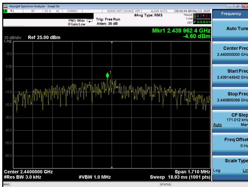
Plot 7-101. Power Spectral Density Plot (Bluetooth (LE), 2Mbps – Ch. 17) – Dual Ant 1
