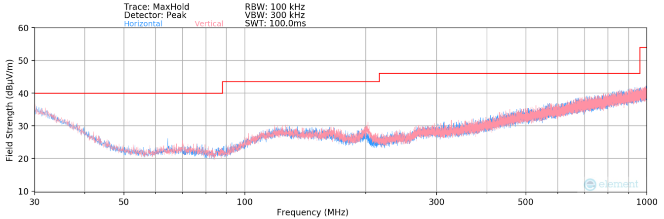
Plot 7-7. Radiated Spurious Plot below 1GHz TOF Camera
