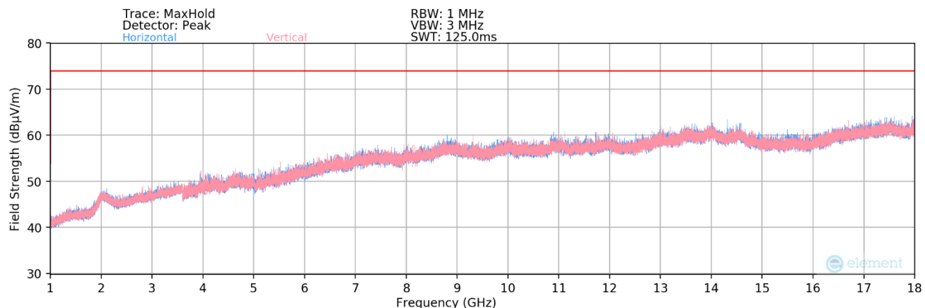
Plot 7-4. Radiated Spurious Plot above 1GHz ET Camera
