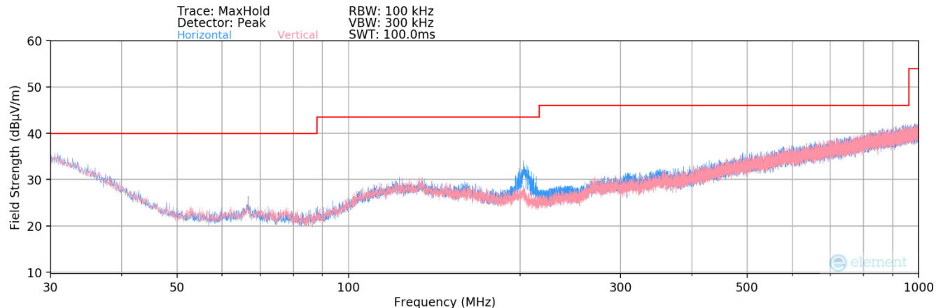
Plot 7-9. Radiated Spurious Plot below 1GHz Controllers
