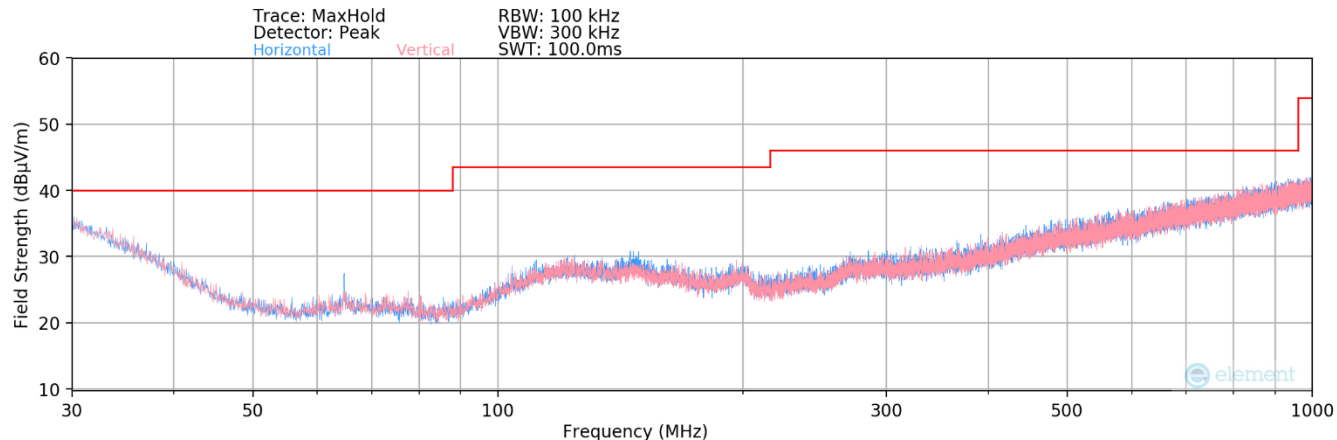
Plot 7-3. Radiated Spurious Plot below 1GHz ET Camera
