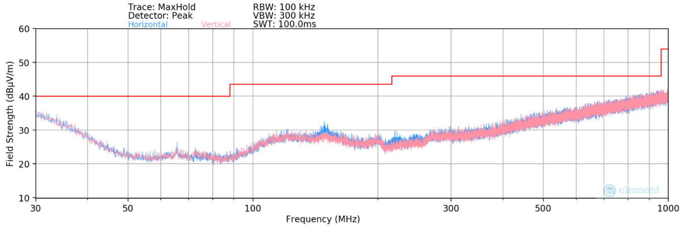
Plot 7-1. Radiated Spurious Plot below 1GHz – HIET Camera
