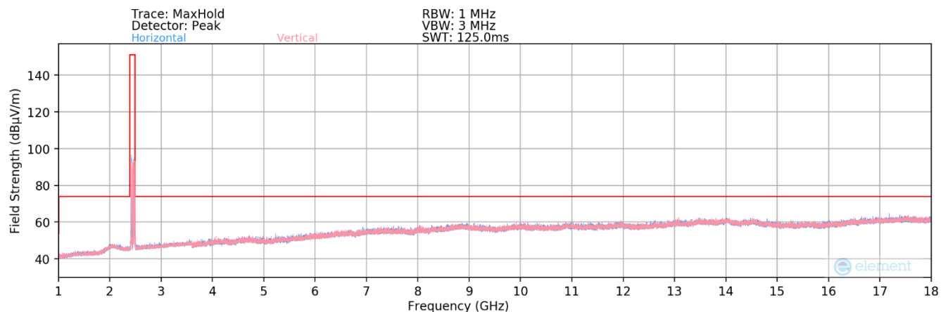
Plot 7-10. Radiated Spurious Plot above 1GHz Controllers
