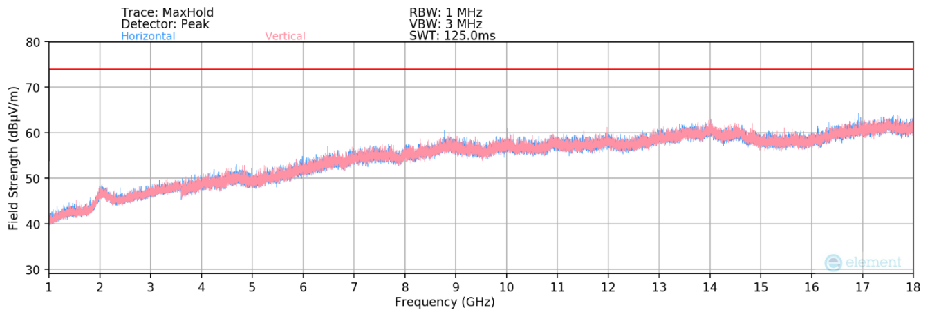
Plot 7-2. Radiated Spurious Plot above 1GHz – HIET Camera
