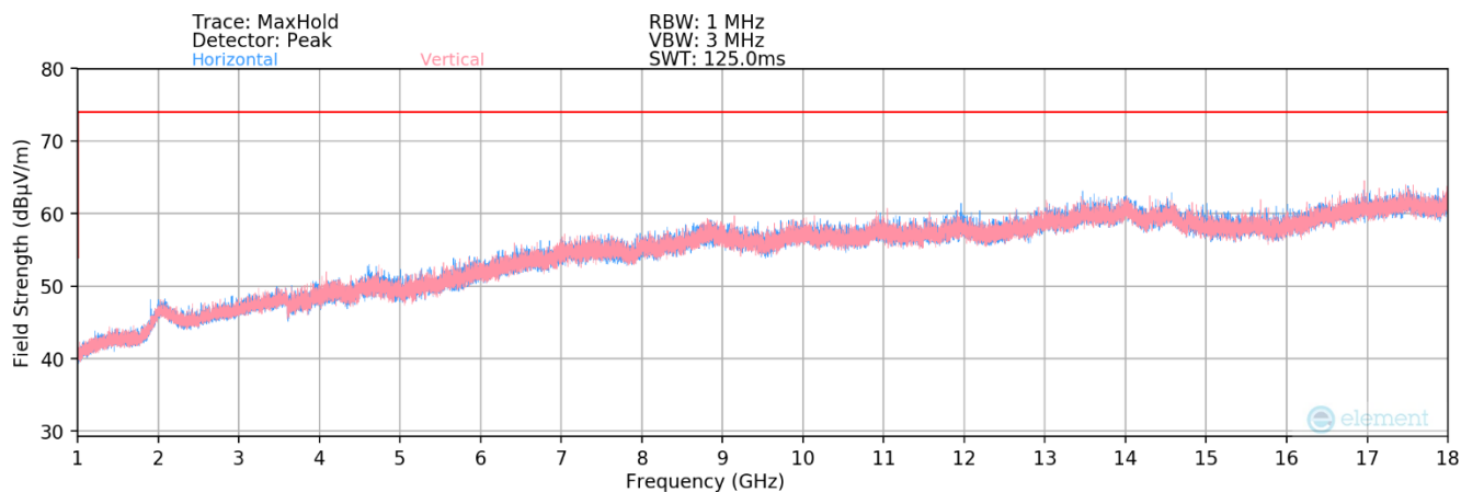
Plot 7-6. Radiated Spurious Plot above 1GHz Passthrough Camera
