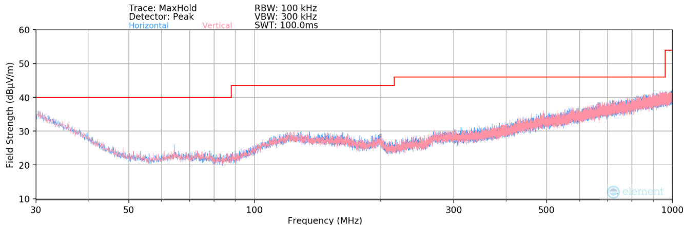
Plot 7-5. Radiated Spurious Plot below 1GHz Passthrough Camera
