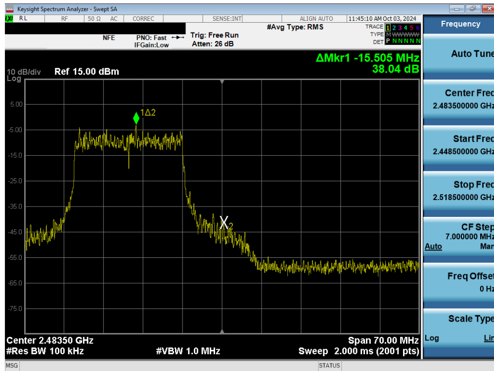
Plot 7-63. Band Edge Plot (802.11ax/be (2.4GHz) – Ch. 12) MIMO ANT1
