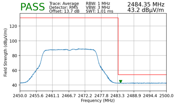
Plot 7-102. Radiated Restricted Upper Band Edge Measurement (Average)
