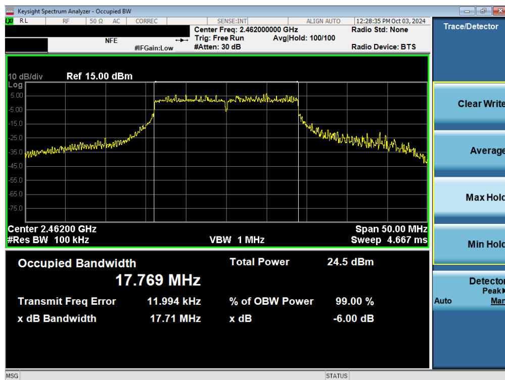
Plot 7-21. 6dB Bandwidth Plot (802.11n/ac (2.4GHz) – Ch. 11) MIMO ANT2
