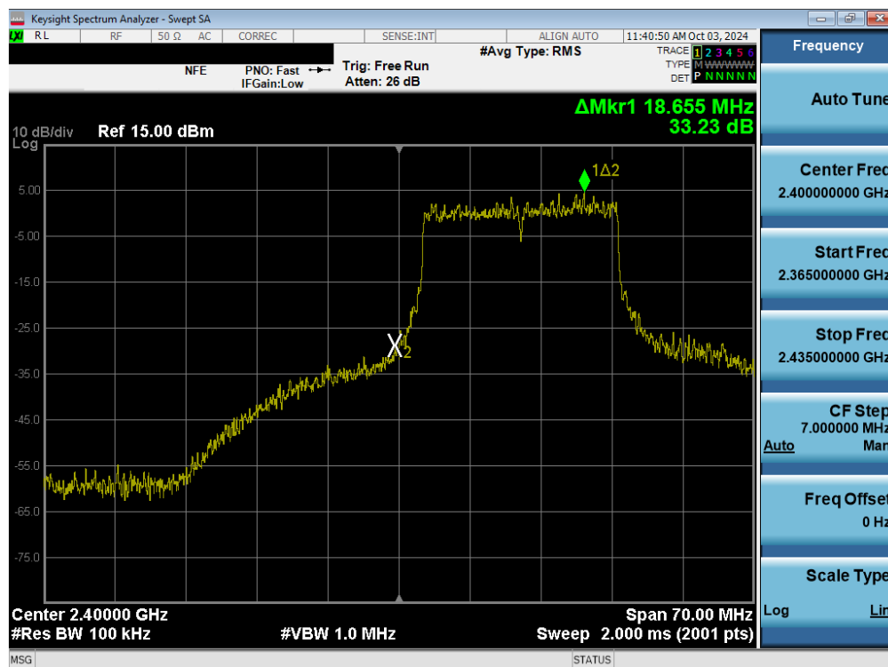
Plot 7-61. Band Edge Plot (802.11ax/be (2.4GHz) – Ch. 1) MIMO ANT1
