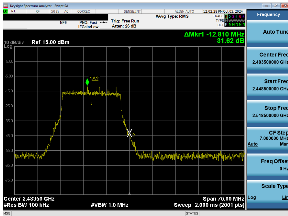
Plot 7-60. Band Edge Plot (802.11n/ac (2.4GHz) – Ch. 13) MIMO ANT1
