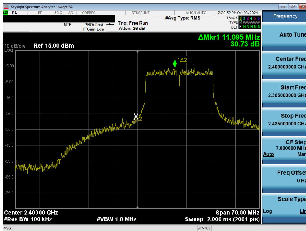
Plot 7-77. Band Edge Plot (802.11ax/be (2.4GHz) – Ch. 1) MIMO ANT2
