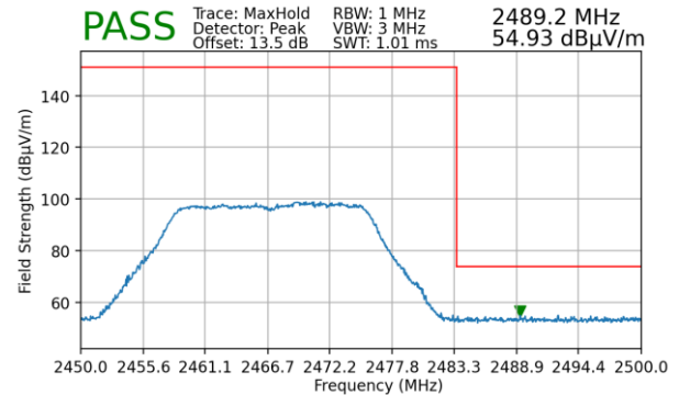
Plot 7-103. Radiated Restricted Upper Band Edge Measurement (Peak)
