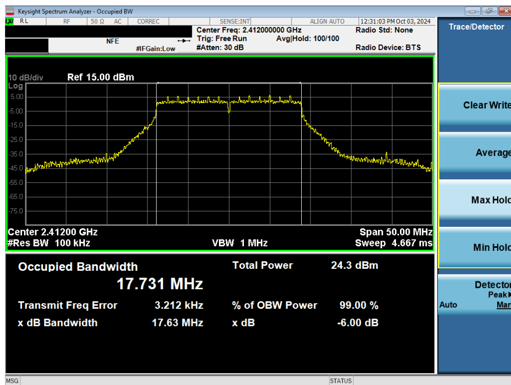
Plot 7-19. 6dB Bandwidth Plot (802.11n/ac (2.4GHz) – Ch. 1) MIMO ANT2
