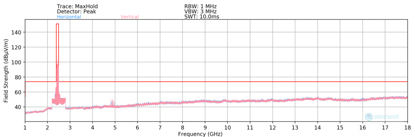
Plot 7-95. Radiated Spurious Plot above 1GHz (802.11b – Ch. 6) MIMO
