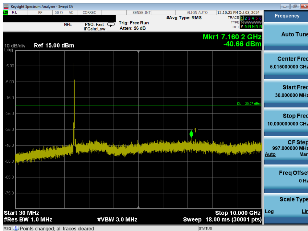
Plot 7-81. Conducted Spurious Plot (802.11b – Ch. 1) MIMO ANT1
