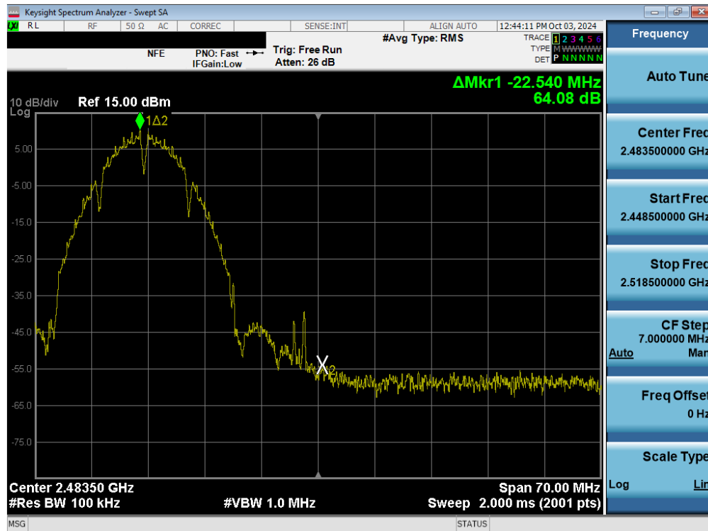
Plot 7-66. Band Edge Plot (802.11b – Ch. 11) MIMO ANT2
