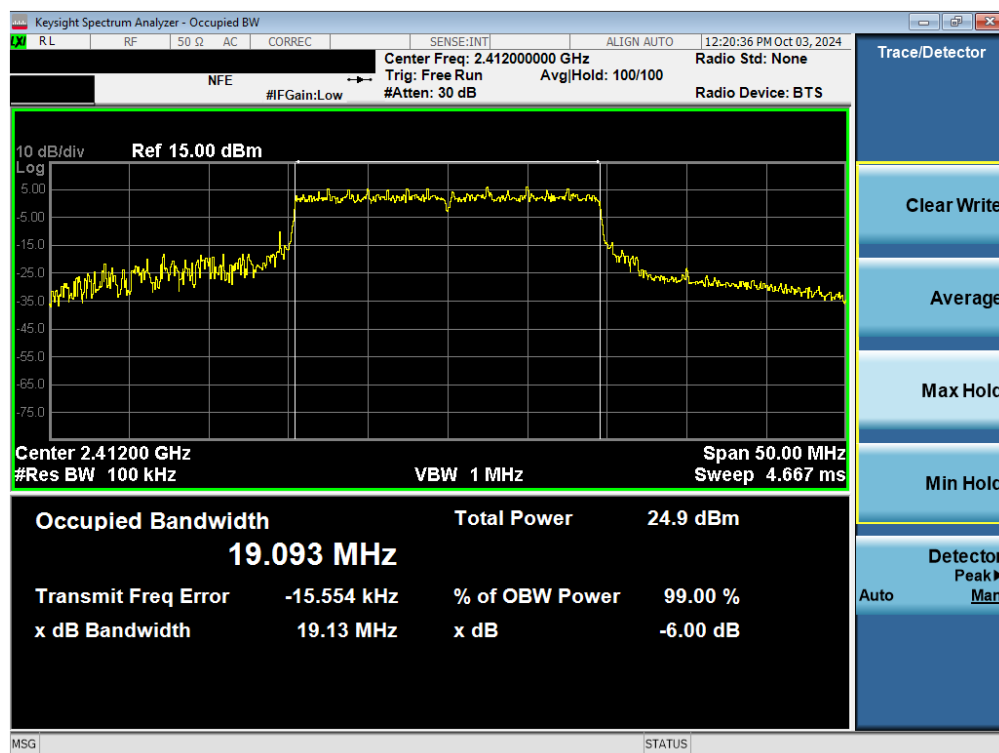
Plot 7-22. 6dB Bandwidth Plot (802.11ax/be (2.4GHz) – Ch. 1) MIMO ANT2
