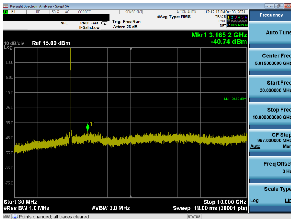
Plot 7-89. Conducted Spurious Plot (802.11b – Ch. 6) MIMO ANT2
