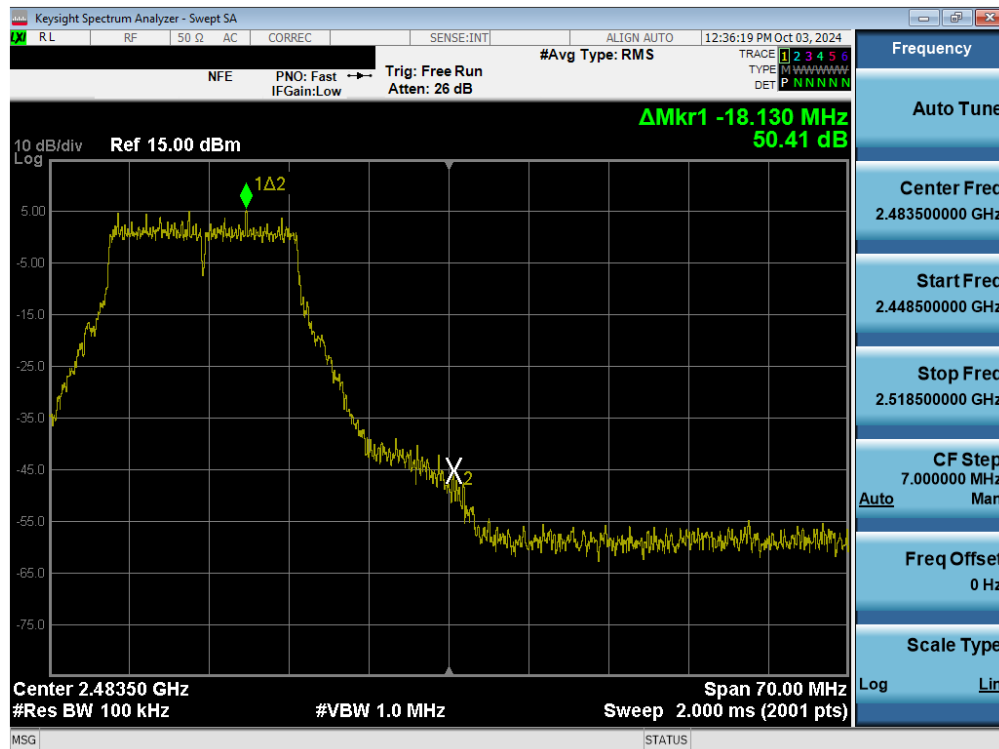
Plot 7-70. Band Edge Plot (802.11g – Ch. 11) MIMO ANT2
