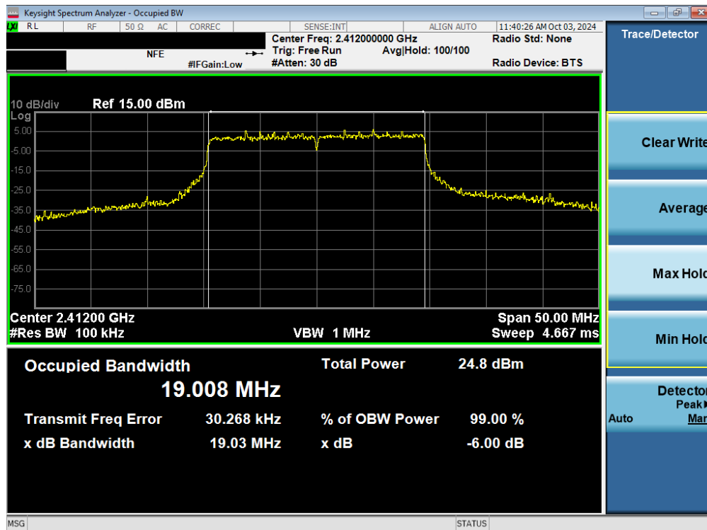
Plot 7-10. 6dB Bandwidth Plot (802.11ax/be (2.4GHz) – Ch. 1) MIMO ANT1
