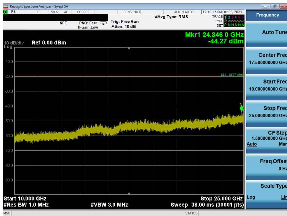
Plot 7-82. Conducted Spurious Plot (802.11b – Ch. 1) MIMO ANT1
