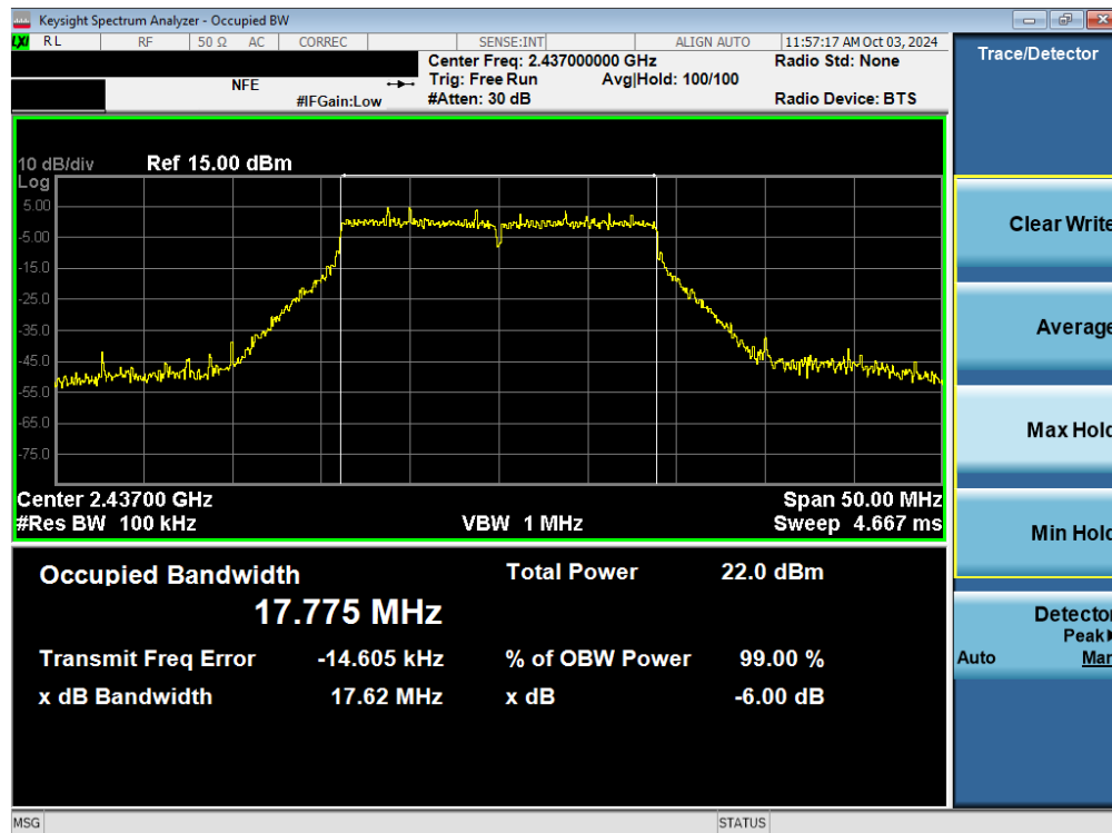
Plot 7-8. 6dB Bandwidth Plot (802.11n/ac (2.4GHz) – Ch. 6) MIMO ANT1
