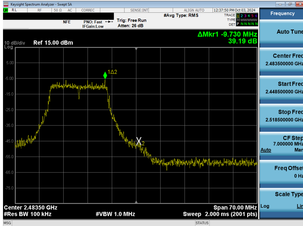
Plot 7-71. Band Edge Plot (802.11g – Ch. 12) MIMO ANT2
