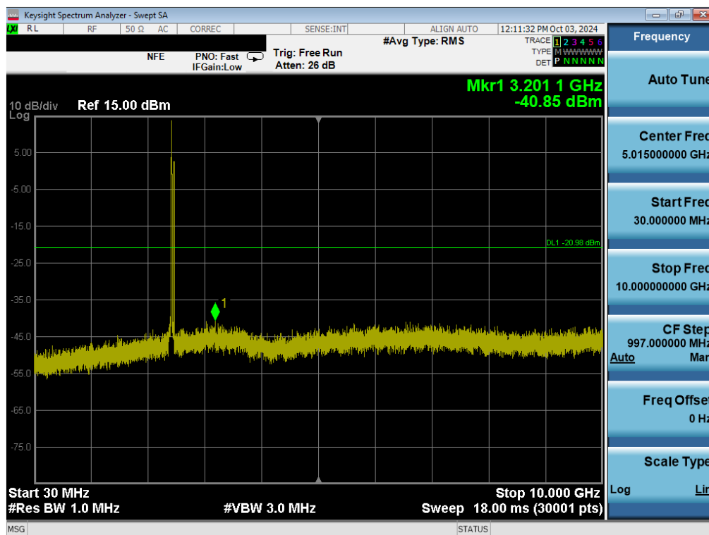
Plot 7-83. Conducted Spurious Plot (802.11b – Ch. 6) MIMO ANT1
