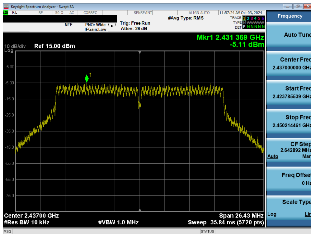
Plot 7-32. Power Spectral Density Plot (802.11n/ac (2.4GHz) – Ch. 6) MIMO ANT1
