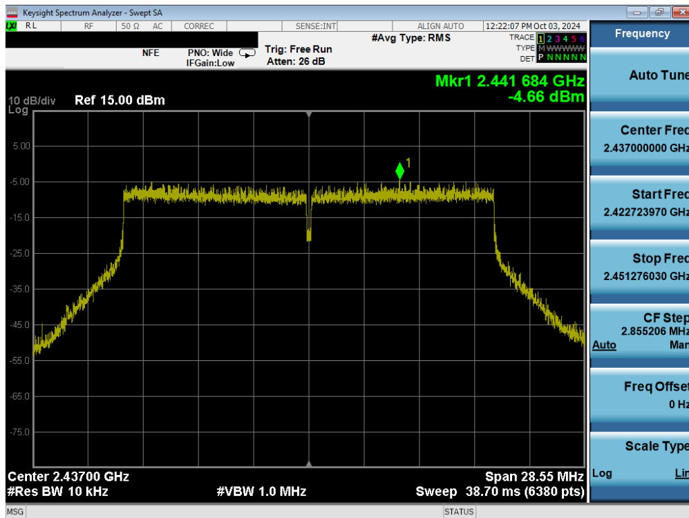
Plot 7-47. Power Spectral Density Plot (802.11ax/be (2.4GHz) – Ch. 6) MIMO ANT2
