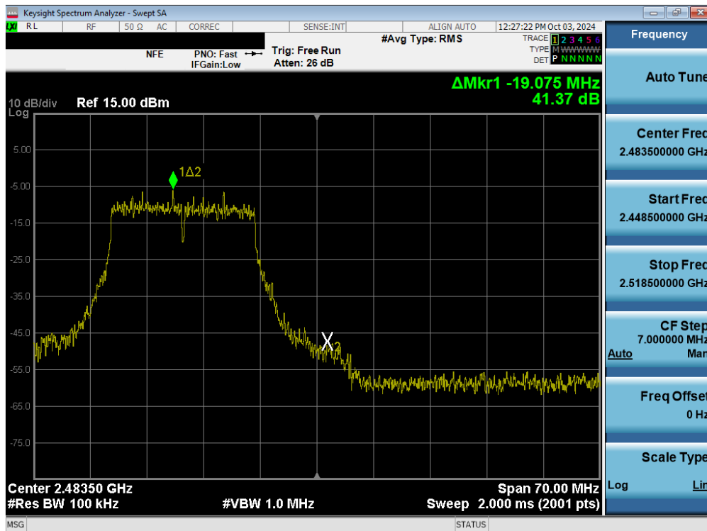
Plot 7-75. Band Edge Plot (802.11n/ac (2.4GHz) – Ch. 12) MIMO ANT2
