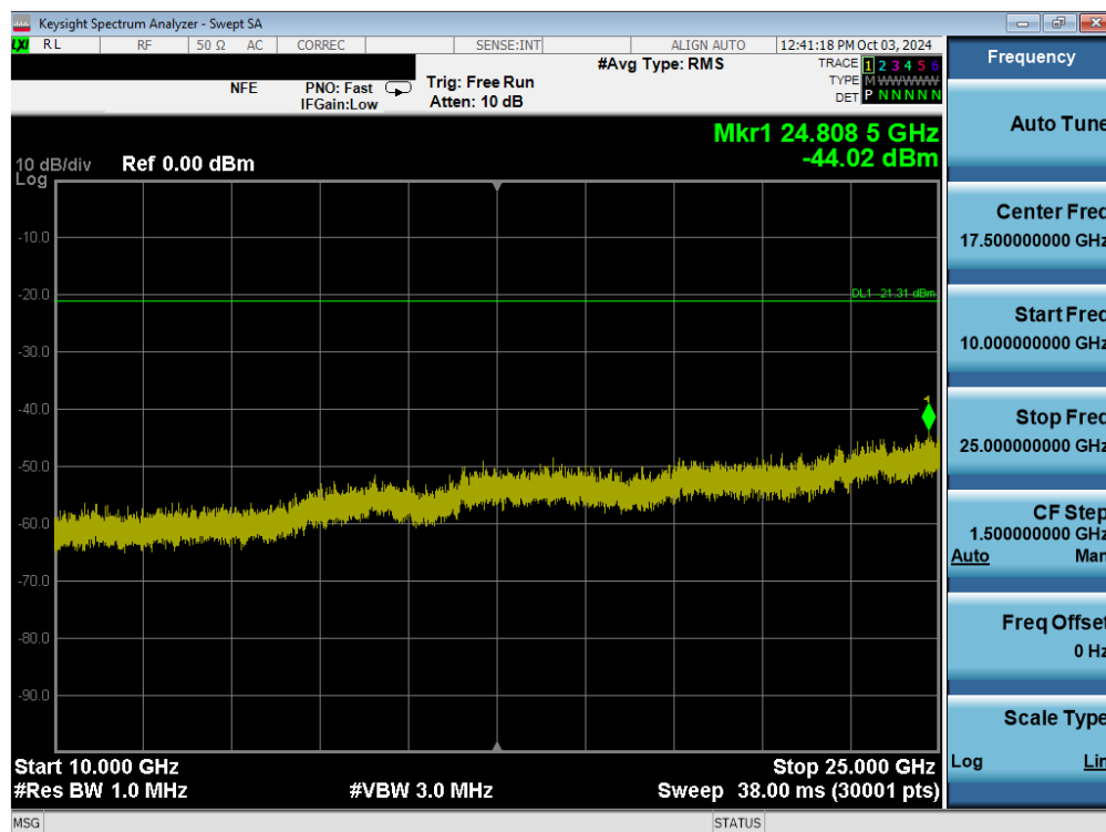
Plot 7-88. Conducted Spurious Plot (802.11b – Ch. 1) MIMO ANT2
