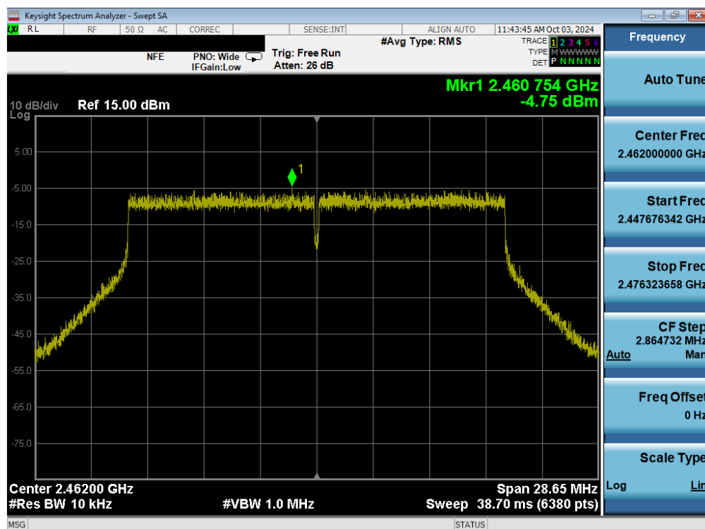
Plot 7-36. Power Spectral Density Plot (802.11ax/be (2.4GHz) – Ch. 11) MIMO ANT1
