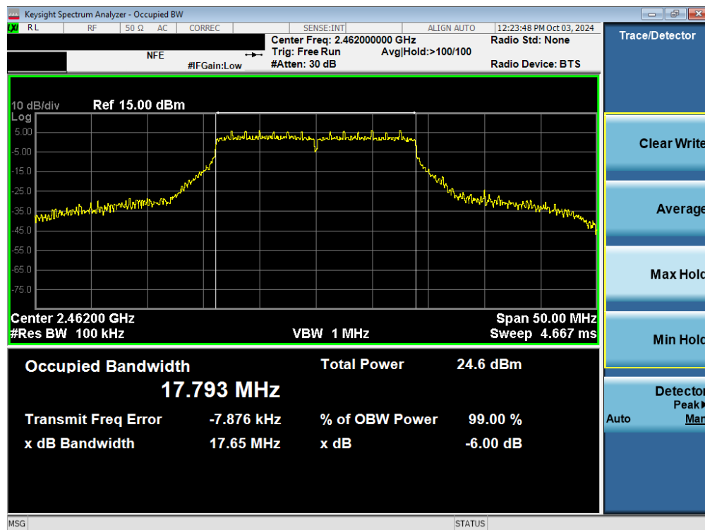
Plot 7-24. 6dB Bandwidth Plot (802.11ax/be (2.4GHz) – Ch. 11) MIMO ANT2
