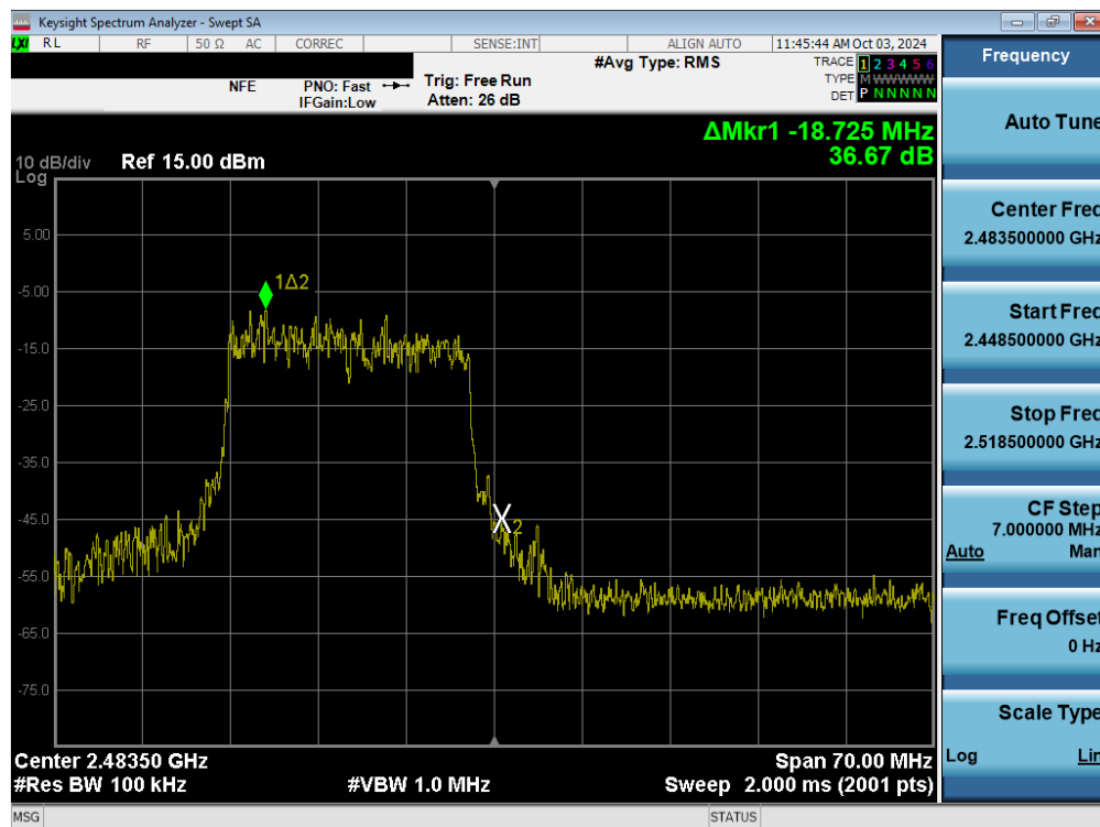
Plot 7-64. Band Edge Plot (802.11ax/be (2.4GHz) – Ch. 13) MIMO ANT1
