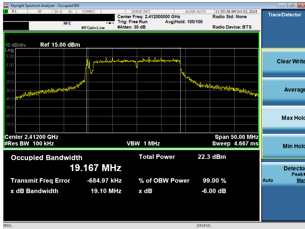
Plot 7-7. 6dB Bandwidth Plot (802.11n/ac (2.4GHz) – Ch. 1) MIMO ANT1
