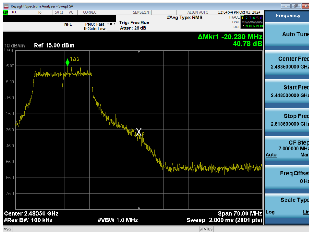
Plot 7-54. Band Edge Plot (802.11g – Ch. 11) MIMO ANT1
