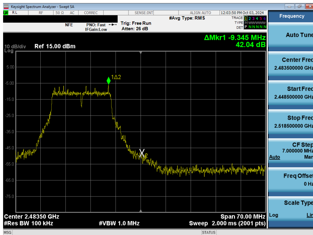
Plot 7-55. Band Edge Plot (802.11g – Ch. 12) MIMO ANT1
