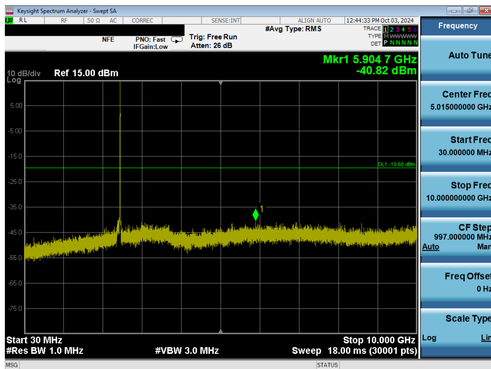
Plot 7-91. Conducted Spurious Plot (802.11b – Ch. 11) MIMO ANT2
