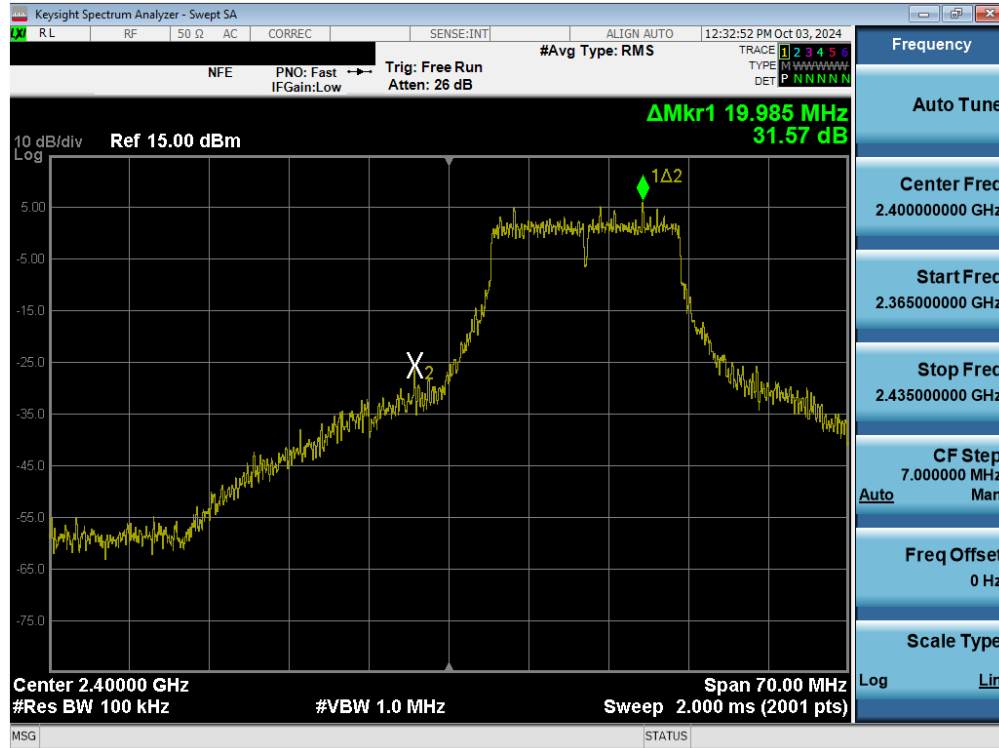
Plot 7-69. Band Edge Plot (802.11g– Ch. 1) MIMO ANT2
