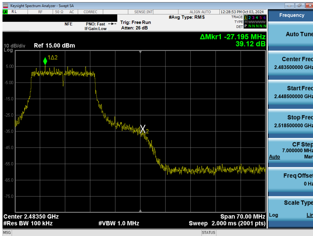
Plot 7-74. Band Edge Plot (802.11n/ac (2.4GHz) – Ch. 11) MIMO ANT2
