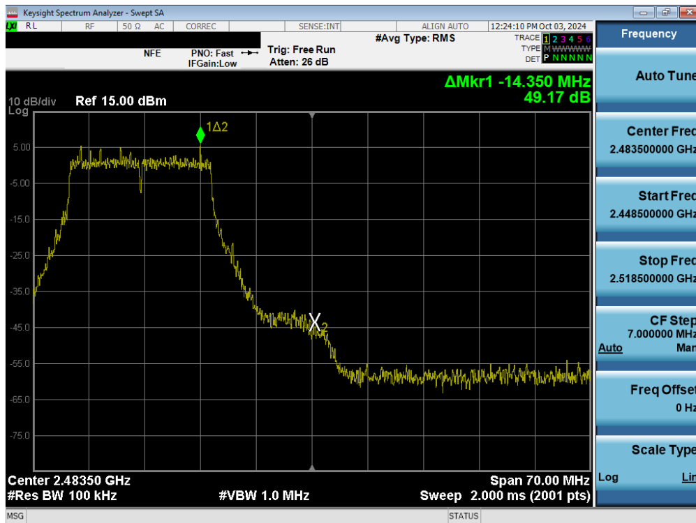
Plot 7-78. Band Edge Plot (802.11ax/be (2.4GHz) – Ch. 11) MIMO ANT2
