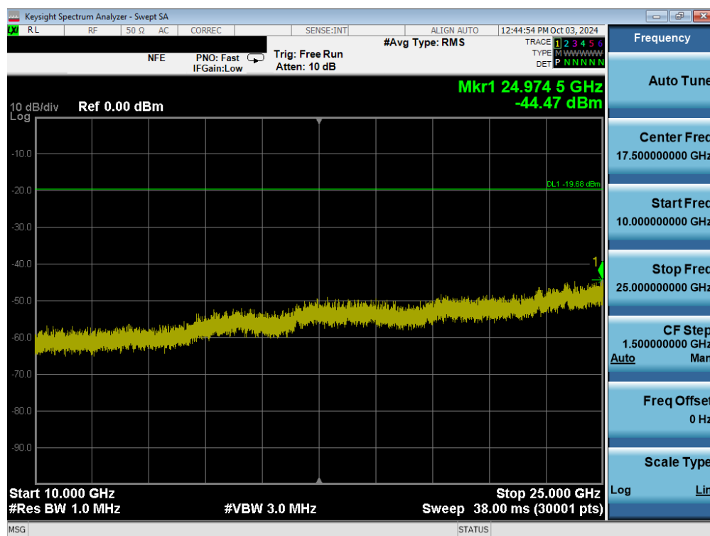
Plot 7-92. Conducted Spurious Plot (802.11b – Ch. 11) MIMO ANT2
