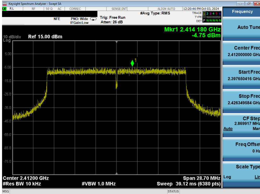
Plot 7-46. Power Spectral Density Plot (802.11ax/be (2.4GHz) – Ch. 1) MIMO ANT2
