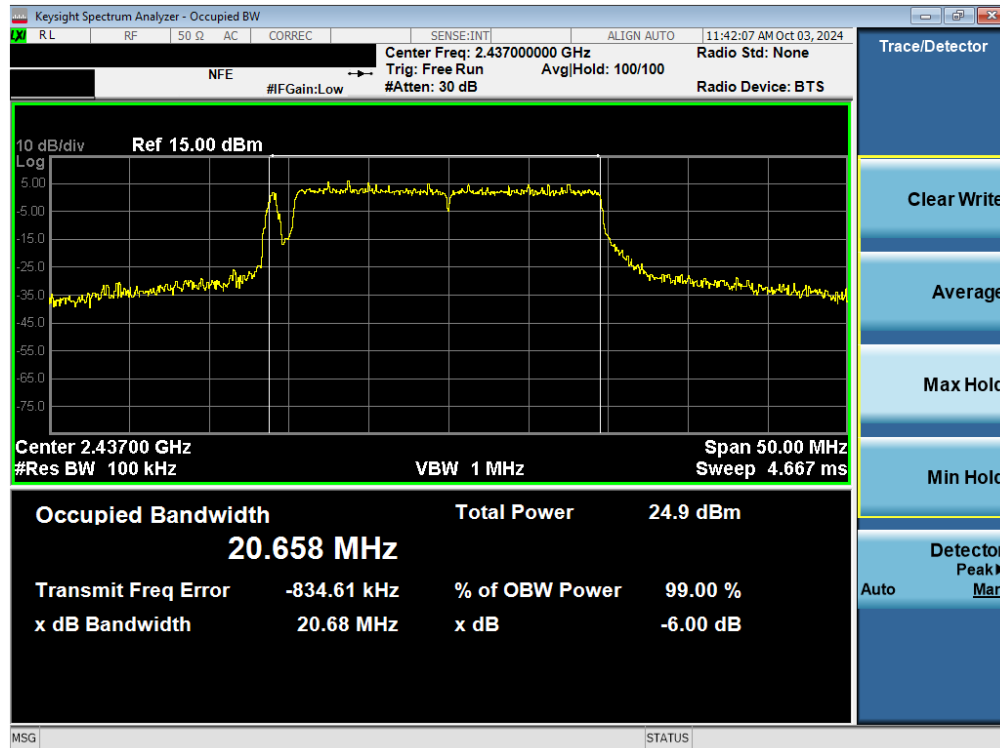
Plot 7-11. 6dB Bandwidth Plot (802.11ax/be (2.4GHz) – Ch. 6) MIMO ANT1
