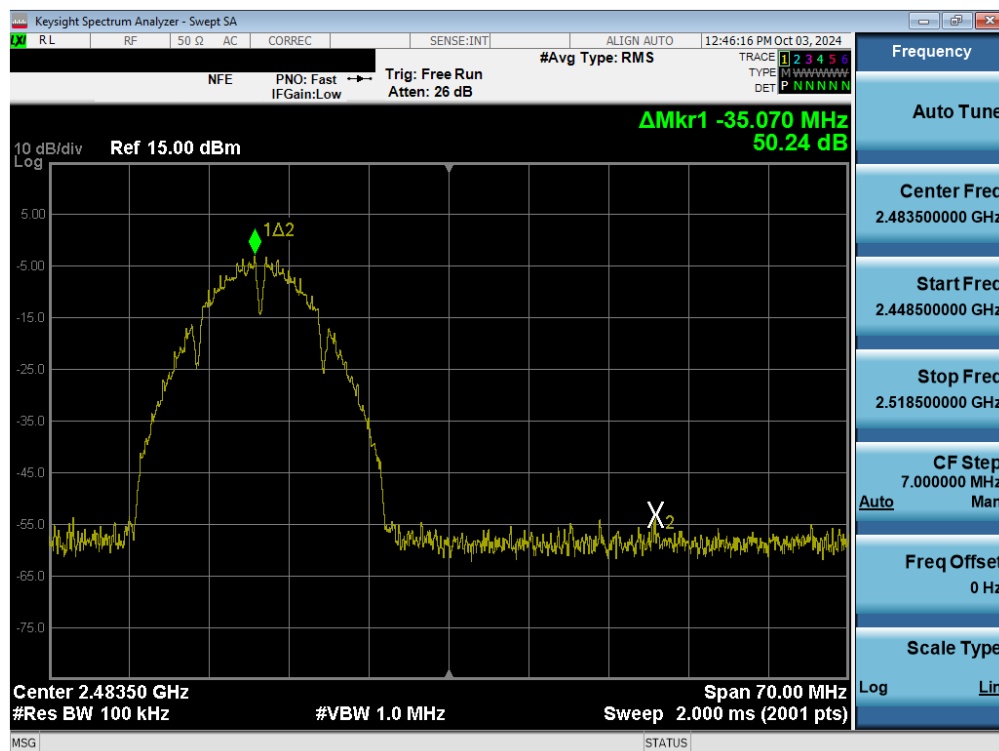
Plot 7-67. Band Edge Plot (802.11b – Ch. 12) MIMO ANT2
