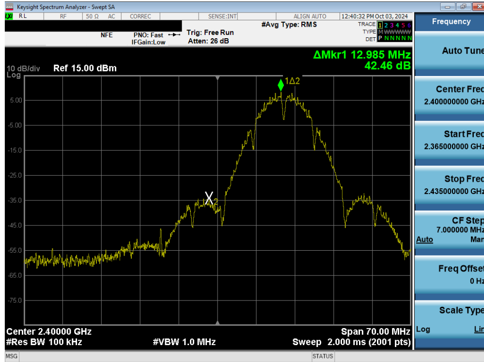
Plot 7-65. Band Edge Plot (802.11b – Ch. 1) – MIMO ANT2
