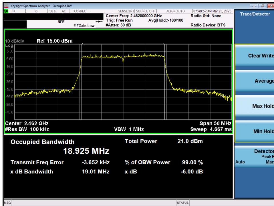
Plot 7-12. 6dB Bandwidth Plot (802.11ax/be (2.4GHz) – Ch. 11) MIMO ANT1
