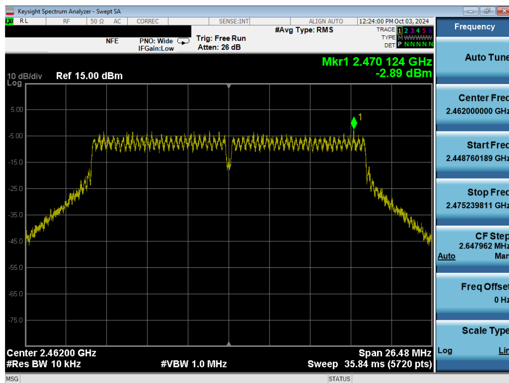
Plot 7-48. Power Spectral Density Plot (802.11ax/be (2.4GHz) – Ch. 11) MIMO ANT2
