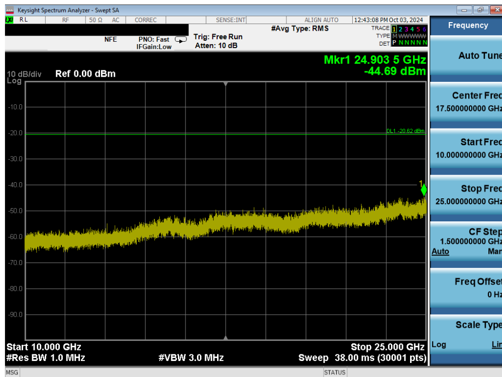
Plot 7-90. Conducted Spurious Plot (802.11b – Ch. 6) MIMO ANT2
