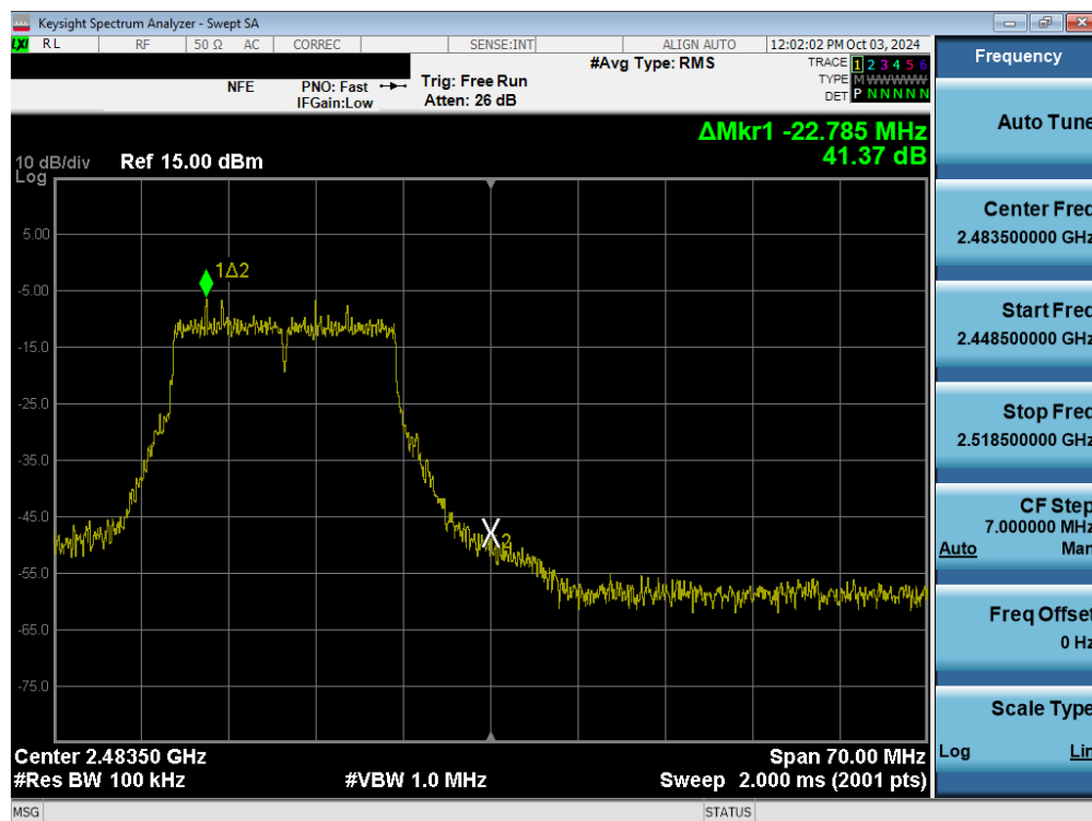
Plot 7-59. Band Edge Plot (802.11n/ac (2.4GHz) – Ch. 12) MIMO ANT1
