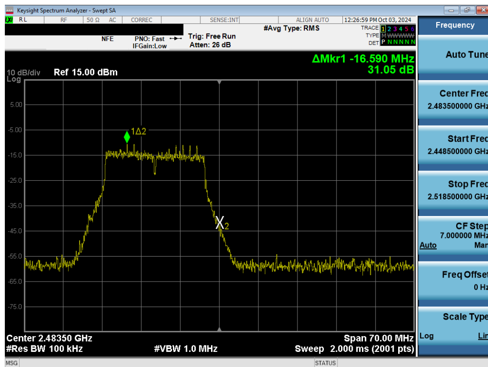
Plot 7-76. Band Edge Plot (802.11n/ac (2.4GHz) – Ch. 13) MIMO ANT2
