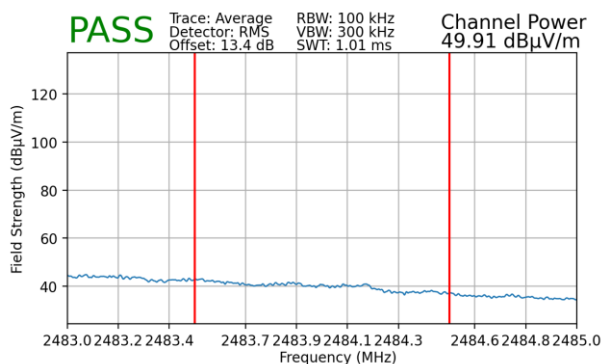
Plot 7-104. Radiated Restricted Upper Band Edge Measurement (Average)
