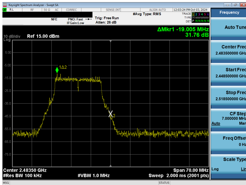
Plot 7-56. Band Edge Plot (802.11g – Ch. 13) MIMO ANT1
