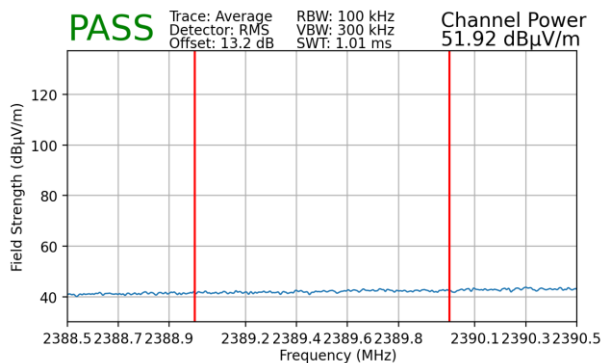
Plot 7-98. Radiated Restricted Lower Band Edge Measurement (Average)
