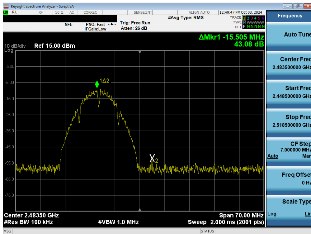
Plot 7-68. Band Edge Plot (802.11b – Ch. 13) MIMO ANT2
