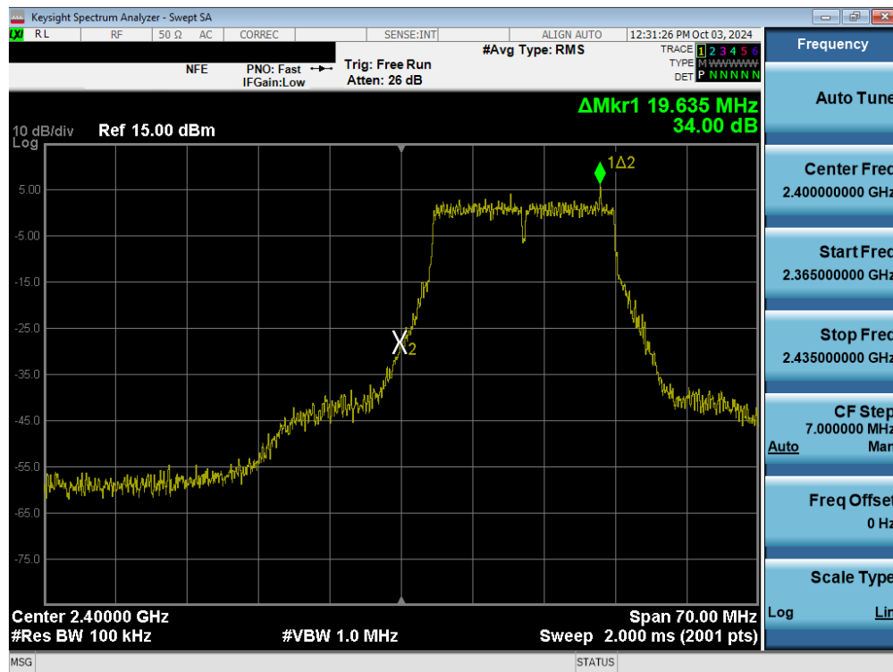
Plot 7-73. Band Edge Plot (802.11n/ac (2.4GHz) – Ch. 1) MIMO ANT2
