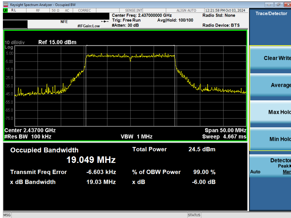
Plot 7-23. 6dB Bandwidth Plot (802.11ax/be (2.4GHz) – Ch. 6) MIMO ANT2
