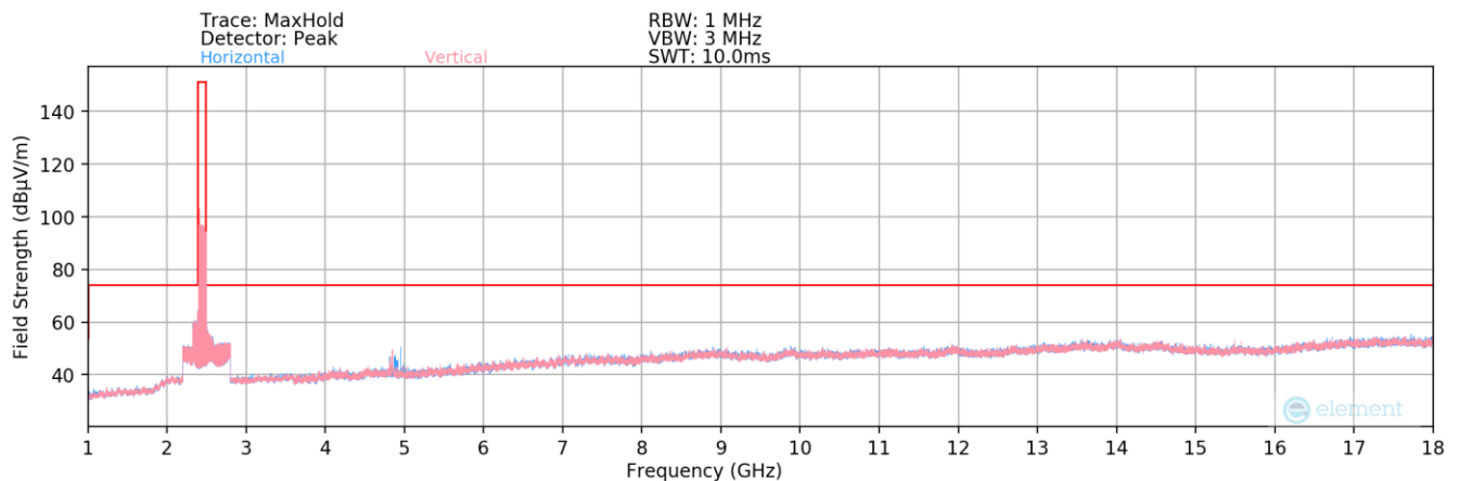
Plot 7-94. Radiated Spurious Plot above 1GHz (802.11b – Ch. 1) MIMO
