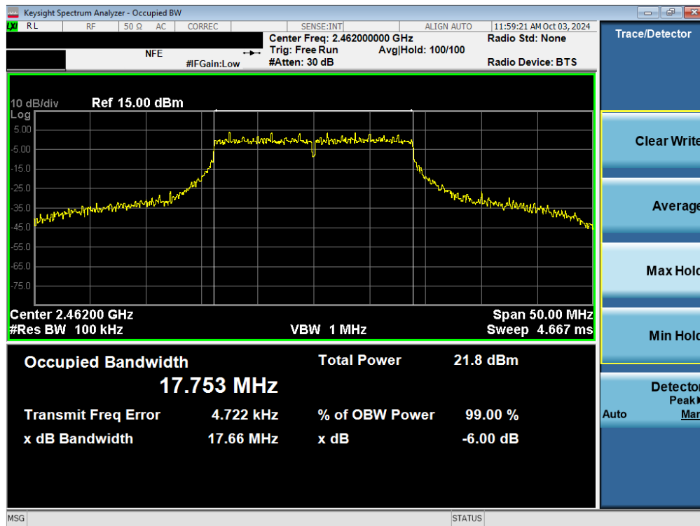
Plot 7-9. 6dB Bandwidth Plot (802.11n/ac (2.4GHz) – Ch. 11) MIMO ANT1
