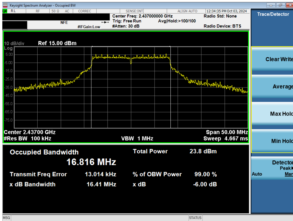
Plot 7-17. 6dB Bandwidth Plot (802.11g – Ch. 6) MIMO ANT2
