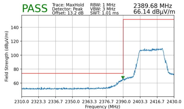
Plot 7-99. Radiated Restricted Lower Band Edge Measurement (Peak)
