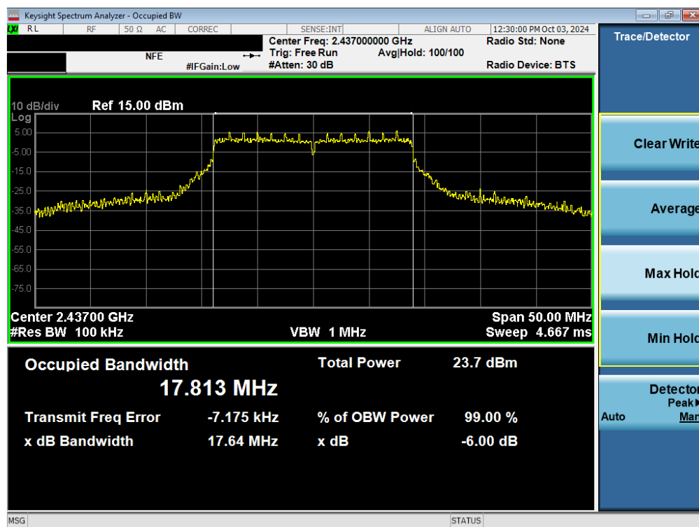
Plot 7-20. 6dB Bandwidth Plot (802.11n/ac (2.4GHz) – Ch. 6) MIMO ANT2
