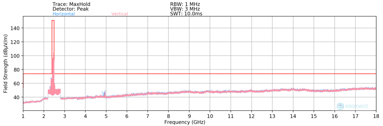
Plot 7-96. Radiated Spurious Plot above 1GHz (802.11b – Ch. 11) MIMO
