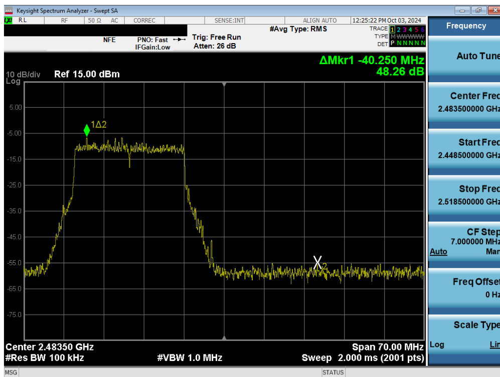
Plot 7-79. Band Edge Plot (802.11ax/be (2.4GHz) – Ch. 12) MIMO ANT2
