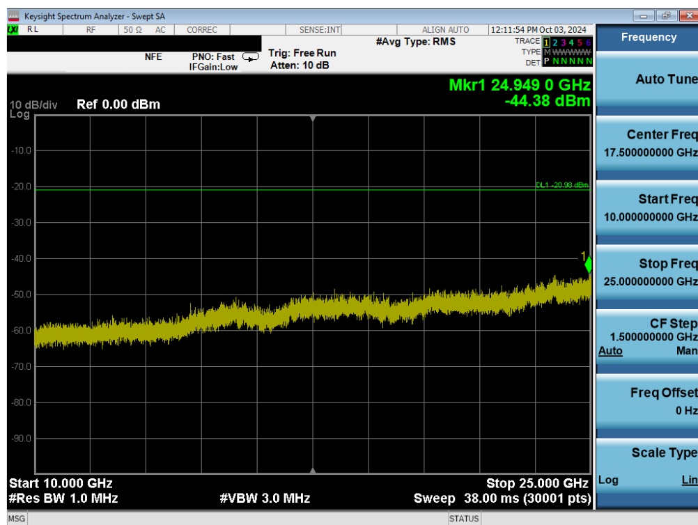
Plot 7-84. Conducted Spurious Plot (802.11b – Ch. 6) MIMO ANT1
