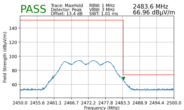
Plot 7-105. Radiated Restricted Upper Band Edge Measurement (Peak)
