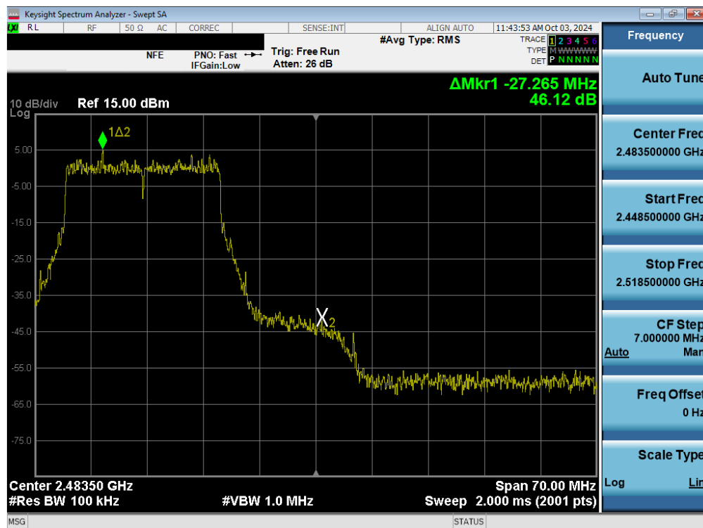
Plot 7-62. Band Edge Plot (802.11ax/be (2.4GHz) – Ch. 11) MIMO ANT1
