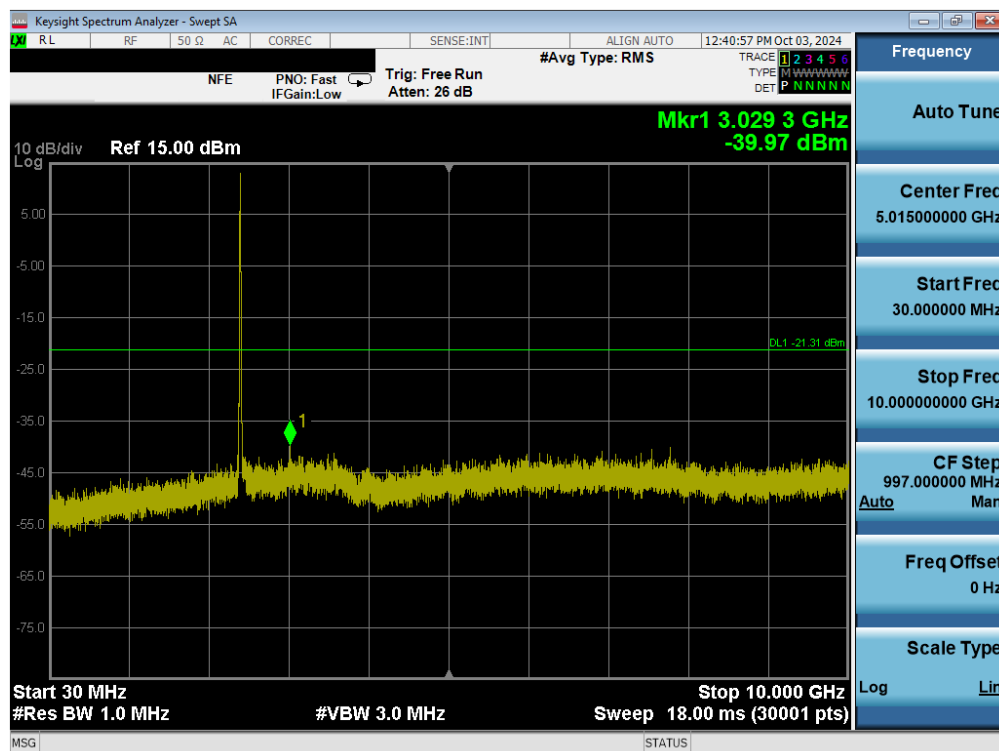
Plot 7-87. Conducted Spurious Plot (802.11b – Ch. 1) MIMO ANT2
