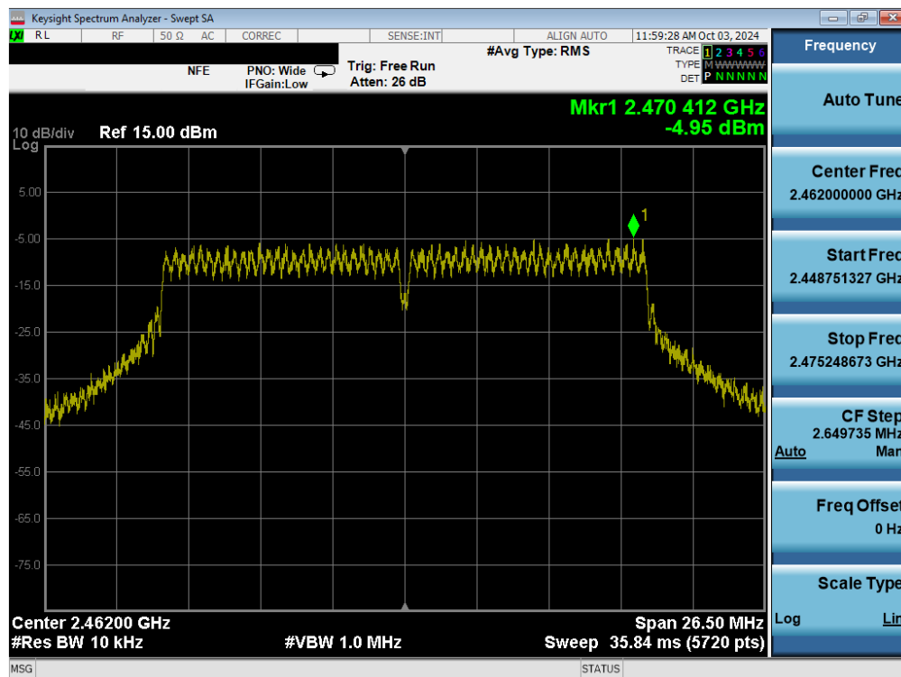
Plot 7-33. Power Spectral Density Plot (802.11n/ac (2.4GHz) – Ch. 11) MIMO ANT1
