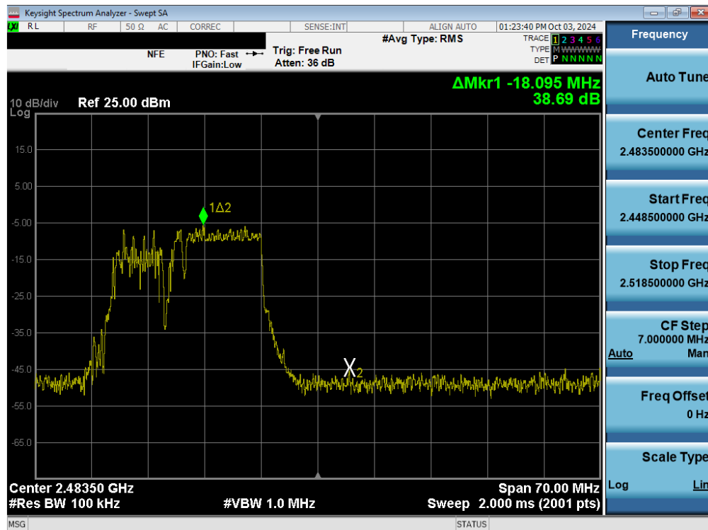
Plot 7-30. Band Edge Plot MIMO ANT1 (802.11be OFDMA – 106+26 Tones – Ch. 12)
