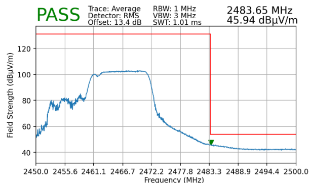
Plot 7-91. Radiated Restricted Upper Band Edge Measurement MIMO (Average – 106+26 Tones)
