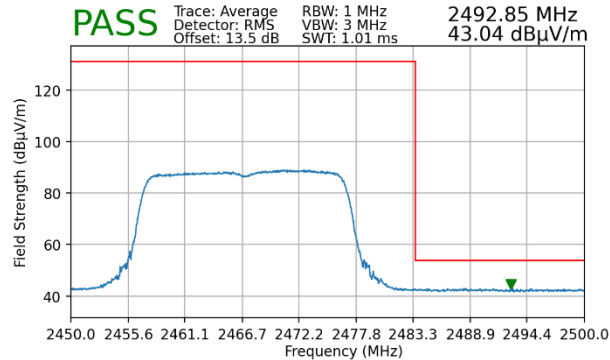
Plot 7-101. Radiated Restricted Upper Band Edge Measurement MIMO (Average – 242 Tones)
