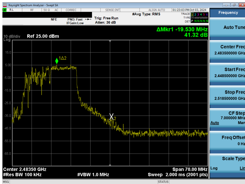
Plot 7-28. Band Edge Plot MIMO ANT1 (802.11be OFDMA – 106+26 Tones – Ch. 11)
