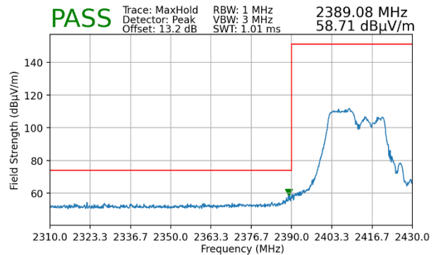
Plot 7-82. Radiated Restricted Lower Band Edge Measurement MIMO (Peak – 106 Tones)
