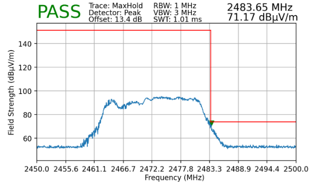
Plot 7-96. Radiated Restricted Upper Band Edge Measurement MIMO (Peak – 106+26 Tones)
