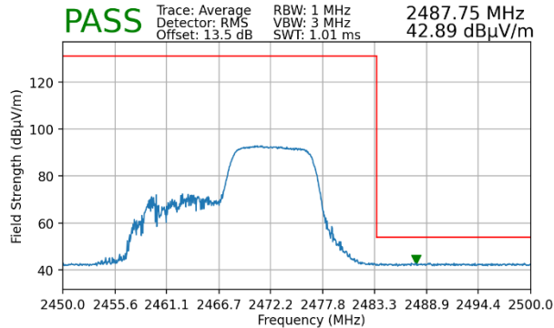
Plot 7-85. Radiated Restricted Upper Band Edge Measurement MIMO (Average – 106 Tones)
