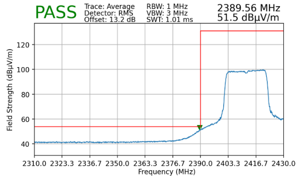
Plot 7-97. Radiated Restricted Lower Band Edge Measurement MIMO (Average – 242 Tones)
