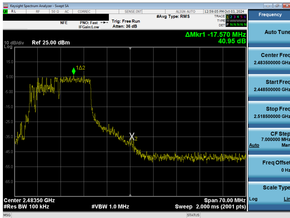
Plot 7-40. Band Edge Plot MIMO ANT2 (802.11be OFDMA – 106+26 Tones – Ch. 11)
