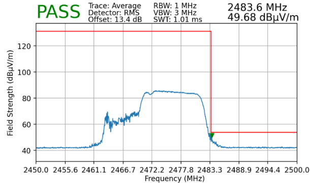
Plot 7-95. Radiated Restricted Upper Band Edge Measurement MIMO (Average – 106+26 Tones)
