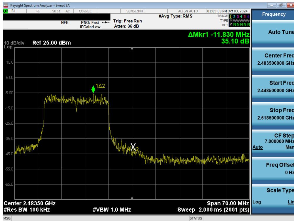
Plot 7-47. Band Edge Plot MIMO ANT2 (802.11ax/be OFDMA – 242 Tones – Ch. 10)
