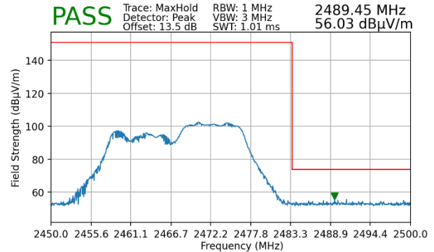
Plot 7-86. Radiated Restricted Upper Band Edge Measurement MIMO (Peak – 106 Tones)
