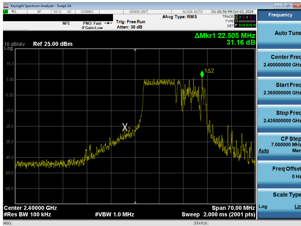
Plot 7-38. Band Edge Plot MIMO ANT2 (802.11be OFDMA – 106+26 Tones – Ch. 1)
