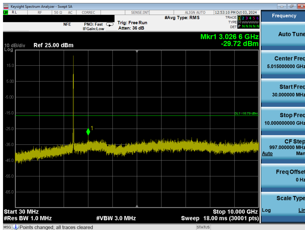
Plot 7-61. Conducted Spurious Plot MIMO ANT2 (802.11ax/be OFDMA – 26 Tones – Ch. 1)
