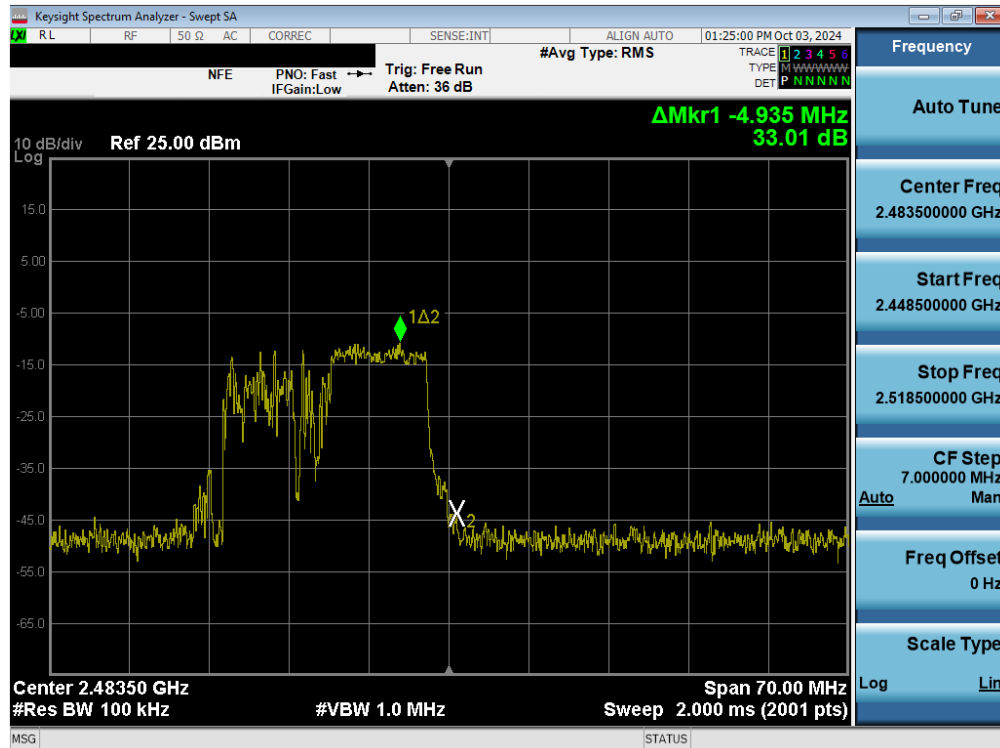
Plot 7-31. Band Edge Plot MIMO ANT1 (802.11ax/be OFDMA – 106 Tones – Ch. 13)
