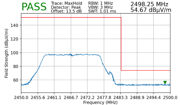
Plot 7-102. Radiated Restricted Upper Band Edge Measurement MIMO (Peak – 242 Tones)
