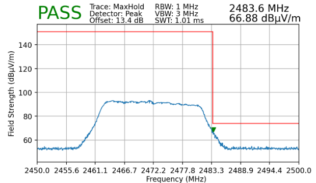
Plot 7-104. Radiated Restricted Upper Band Edge Measurement MIMO (Peak – 242 Tones)
