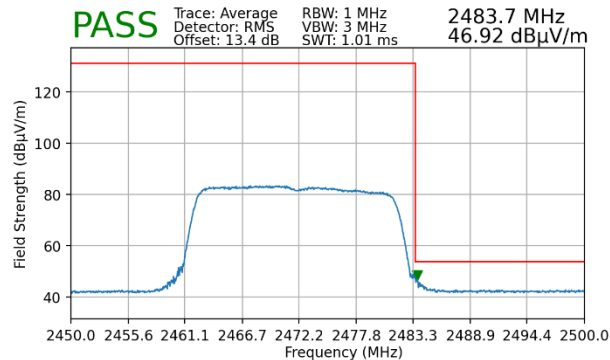
Plot 7-103. Radiated Restricted Upper Band Edge Measurement MIMO (Average – 242 Tones)
