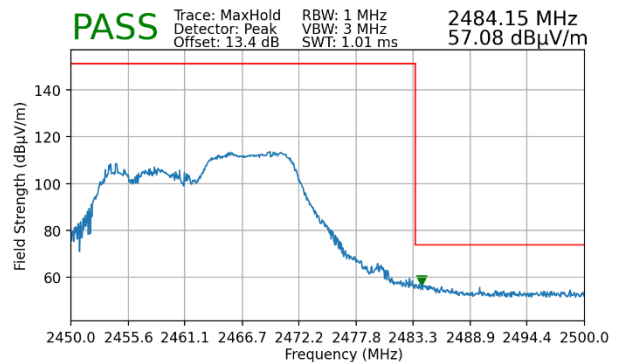
Plot 7-84. Radiated Restricted Upper Band Edge Measurement MIMO (Peak – 106 Tones)
