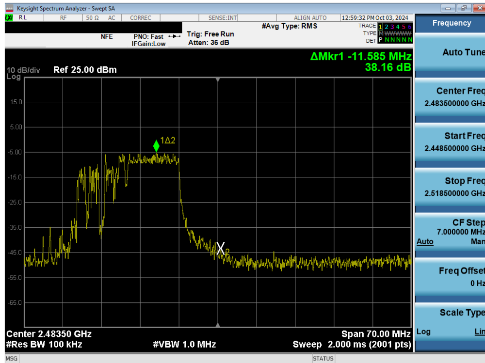
Plot 7-42. Band Edge Plot MIMO ANT2 (802.11be OFDMA – 106+26 Tones – Ch. 12)
