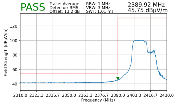
Plot 7-89. Radiated Restricted Lower Band Edge Measurement MIMO (Average – 106+26 Tones)
