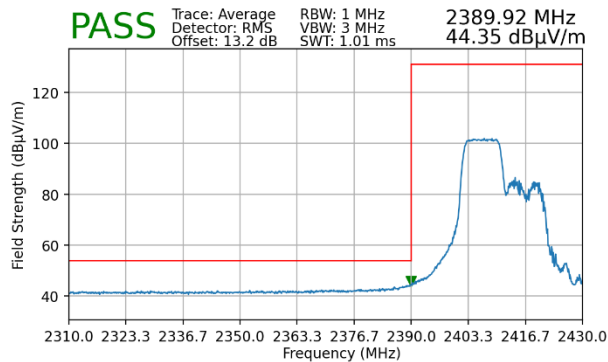
Plot 7-81. Radiated Restricted Lower Band Edge Measurement MIMO (Average – 106 Tones)
