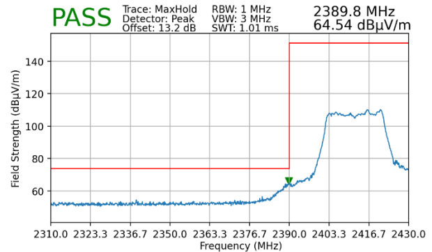
Plot 7-98. Radiated Restricted Lower Band Edge Measurement MIMO (Peak – 242 Tones)
