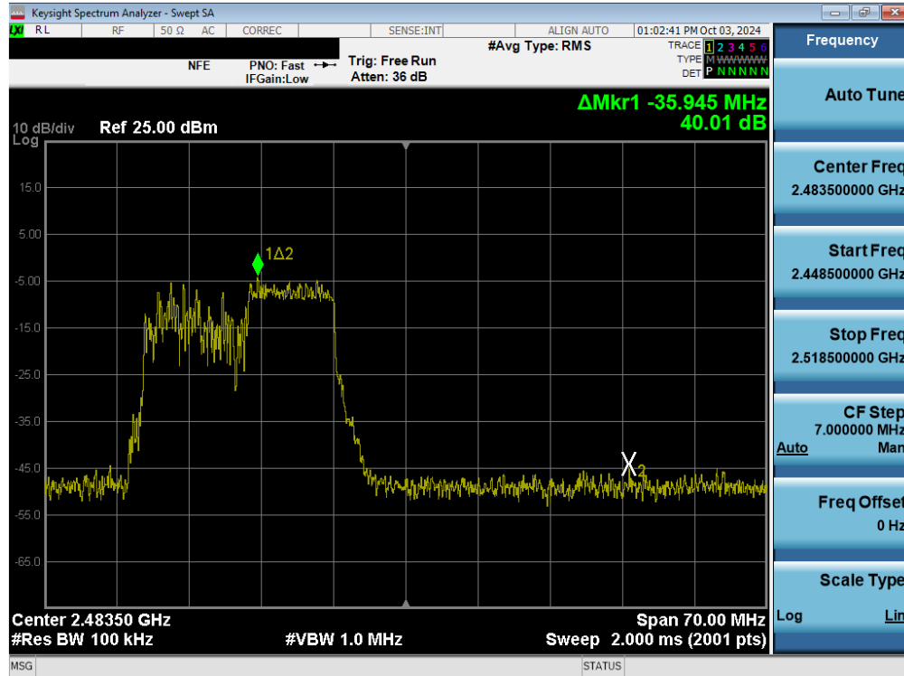
Plot 7-41. Band Edge Plot MIMO ANT2 (802.11ax/be OFDMA – 106 Tones – Ch. 12)
