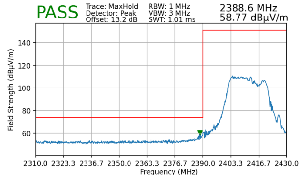
Plot 7-90. Radiated Restricted Lower Band Edge Measurement MIMO (Peak – 106+26 Tones)
