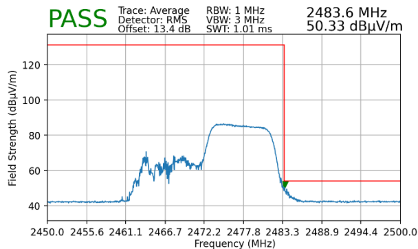
Plot 7-87. Radiated Restricted Upper Band Edge Measurement MIMO (Average – 106 Tones)
