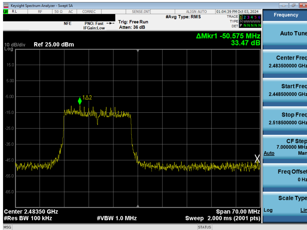
Plot 7-48. Band Edge Plot MIMO ANT2 (802.11ax/be OFDMA – 242 Tones – Ch. 11)
