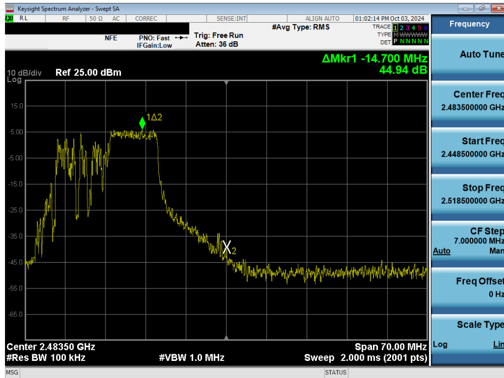
Plot 7-39. Band Edge Plot MIMO ANT2 (802.11ax/be OFDMA – 106 Tones – Ch. 11)
