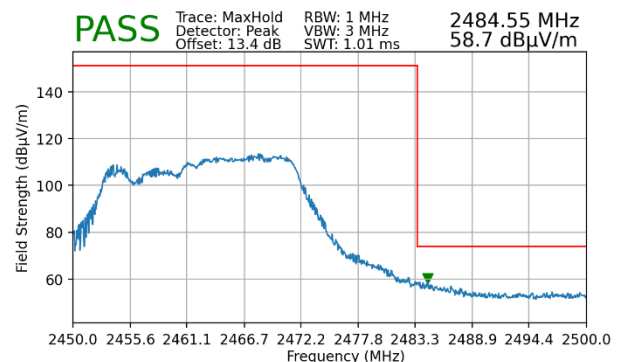
Plot 7-92. Radiated Restricted Upper Band Edge Measurement MIMO (Peak – 106+26 Tones)
