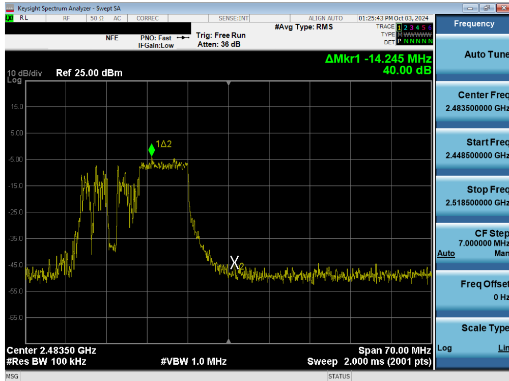
Plot 7-29. Band Edge Plot MIMO ANT1 (802.11ax/be OFDMA – 106 Tones – Ch. 12)
