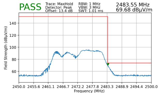
Plot 7-88. Radiated Restricted Upper Band Edge Measurement MIMO (Peak – 106 Tones)
