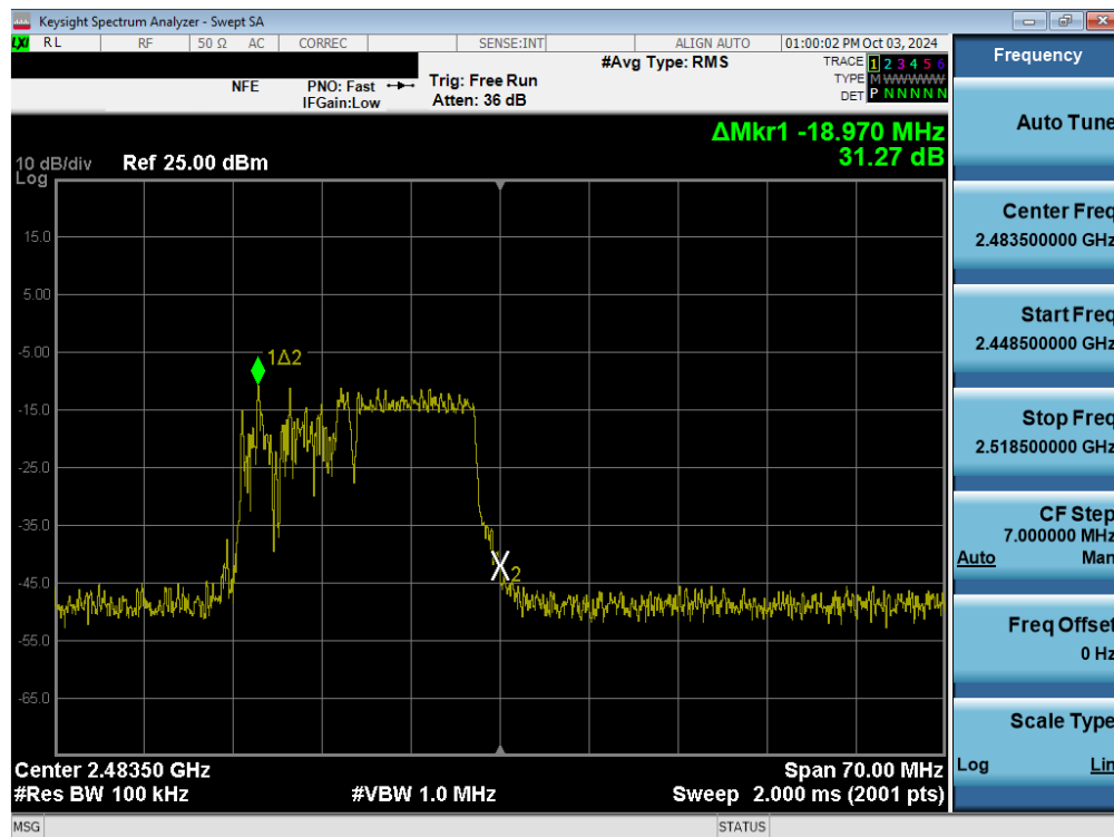
Plot 7-44. Band Edge Plot MIMO ANT2 (802.11be OFDMA – 106+26 Tones – Ch. 13)
