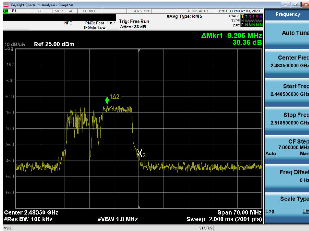
Plot 7-43. Band Edge Plot MIMO ANT2 (802.11ax/be OFDMA – 106 Tones – Ch. 13)
