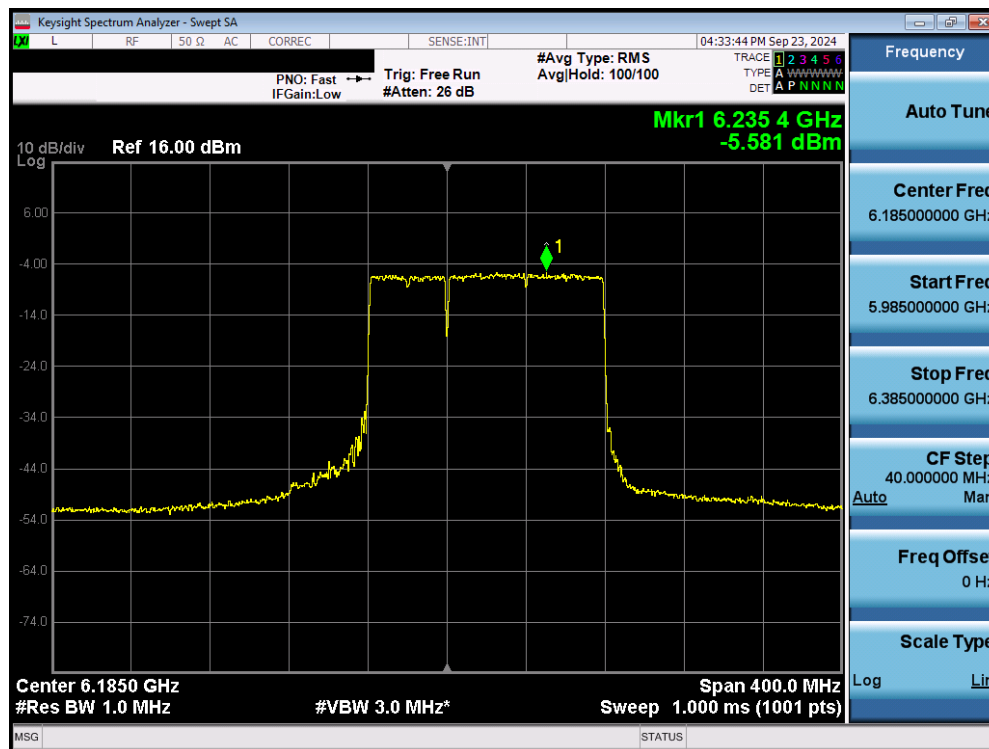
Plot 7-35. Power Spectral Density Plot MIMO ANT2 (160MHz 802.11be (UNII Band 5) – Ch. 47) – 40MHz Punctured - LPI
