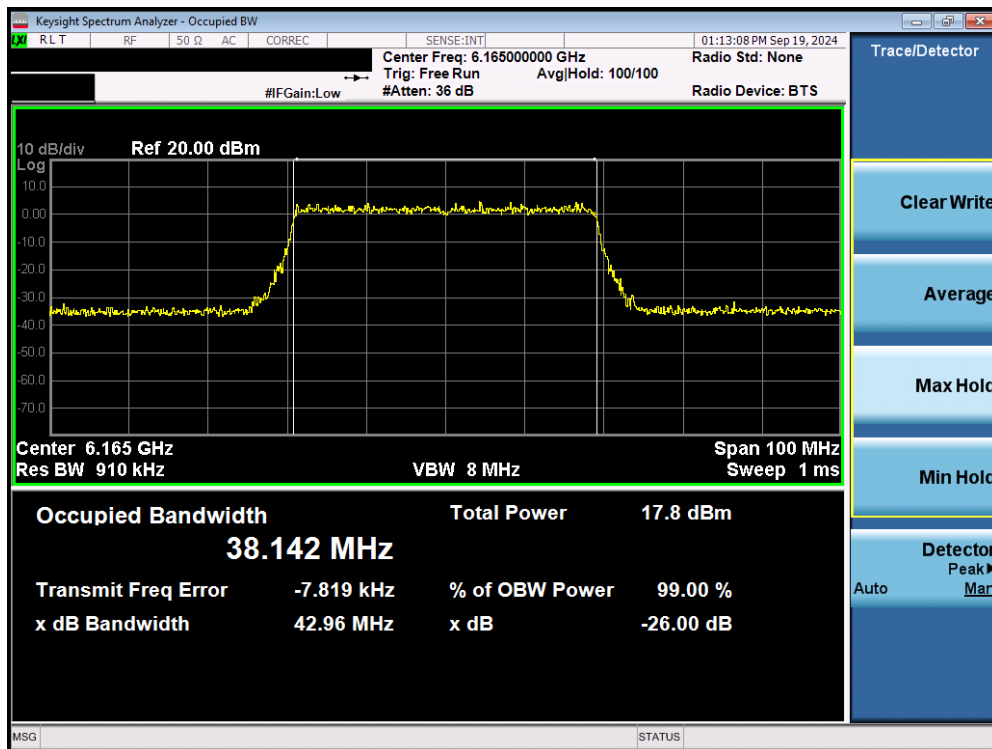
Plot 7-12. 26dB Bandwidth Plot MIMO ANT2 (40MHz 802.11ax/be (UNII Band 5) – Ch. 43) - LPI
