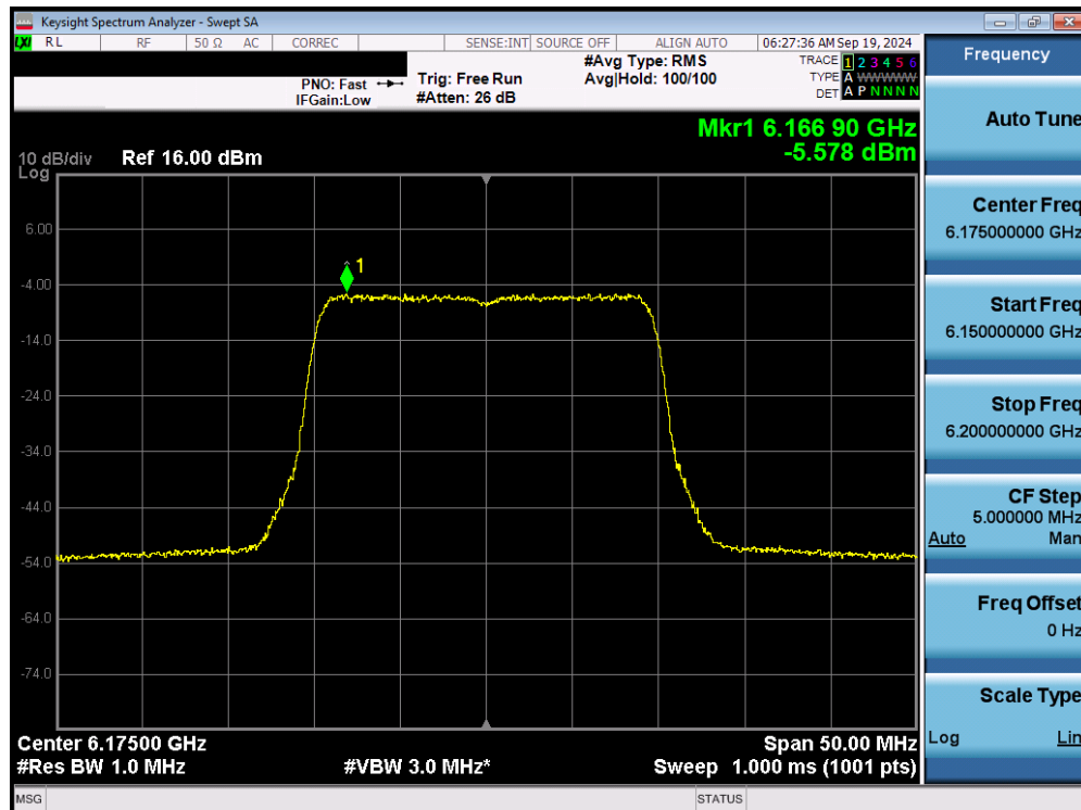
Plot 7-20. Power Spectral Density Plot MIMO ANT1 (20MHz 802.11ax/be (UNII Band 5) – Ch. 45) - LPI
