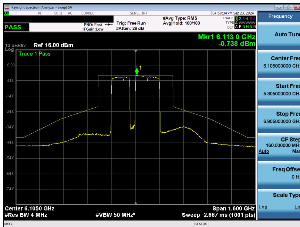
Plot 7-54. In Band Emissions Plot MIMO ANT2 (320MHz 802.11be (UNII Band 5) – Ch. 31) – 40MHz Punctured – LPI
