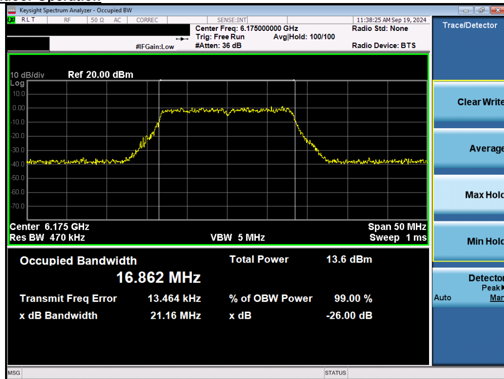
Plot 7-10. 26dB Bandwidth Plot MIMO ANT2 (20MHz 802.11a (UNII Band 5) – Ch. 45) - LPI
