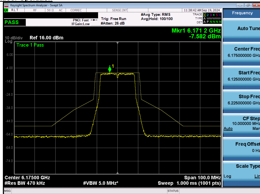
Plot 7-46. In Band Emissions Plot MIMO ANT2 (20MHz 802.11a (UNII Band 5) – Ch. 45) - LPI
