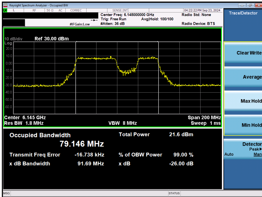
Plot 7-16. 26dB Bandwidth Plot MIMO ANT2 (80MHz 802.11be (UNII Band 5) – Ch. 39) – 20MHz Punctured - LPI
