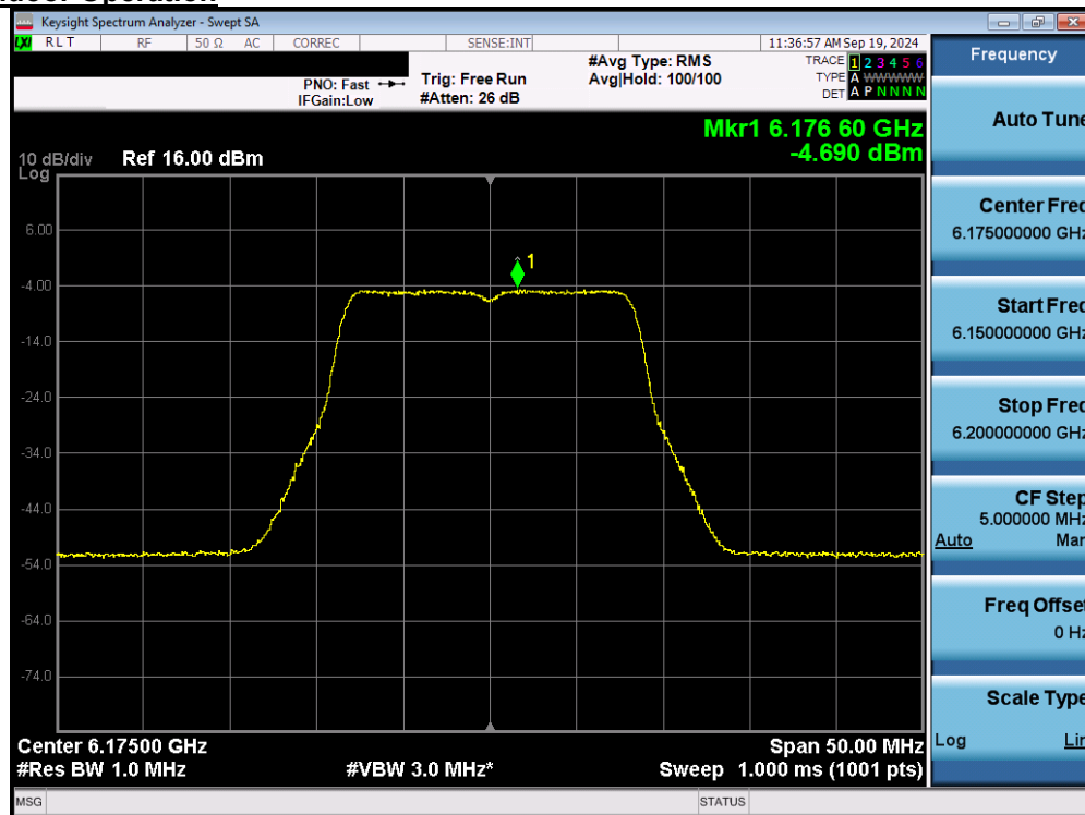
Plot 7-28. Power Spectral Density Plot MIMO ANT2 (20MHz 802.11a (UNII Band 5) – Ch. 45) - LPI
