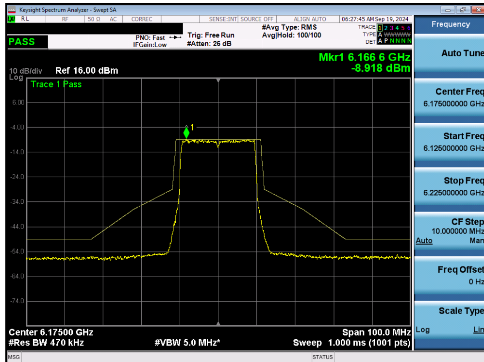
Plot 7-38. In Band Emissions Plot MIMO ANT1 (20MHz 802.11ax/be (UNII Band 5) – Ch. 45) - LPI
