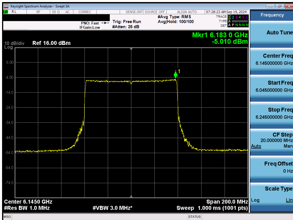
Plot 7-22. Power Spectral Density Plot MIMO ANT1 (80MHz 802.11ax/be (UNII Band 5) – Ch. 39) - LPI
