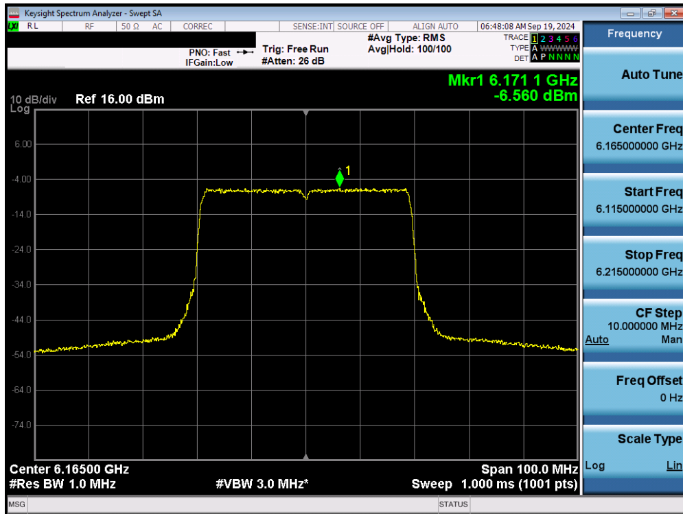
Plot 7-21. Power Spectral Density Plot MIMO ANT1 (40MHz 802.11ax/be (UNII Band 5) – Ch. 43) - LPI
