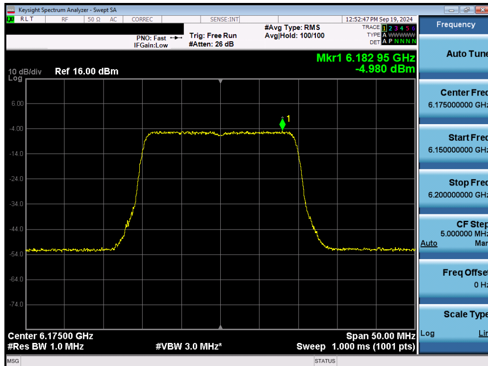
Plot 7-29. Power Spectral Density Plot MIMO ANT2 (20MHz 802.11ax/be (UNII Band 5) – Ch. 45) - LPI
