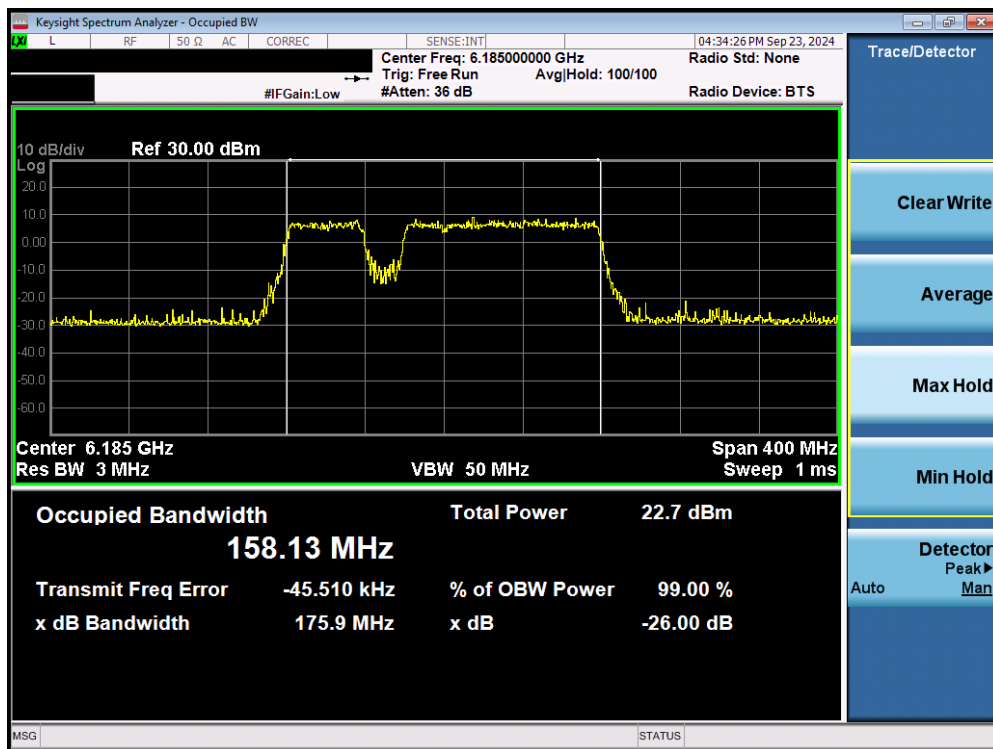
Plot 7-17. 26dB Bandwidth Plot MIMO ANT2 (160MHz 802.11be (UNII Band 5) – Ch. 47) – 20MHz Punctured - LPI
