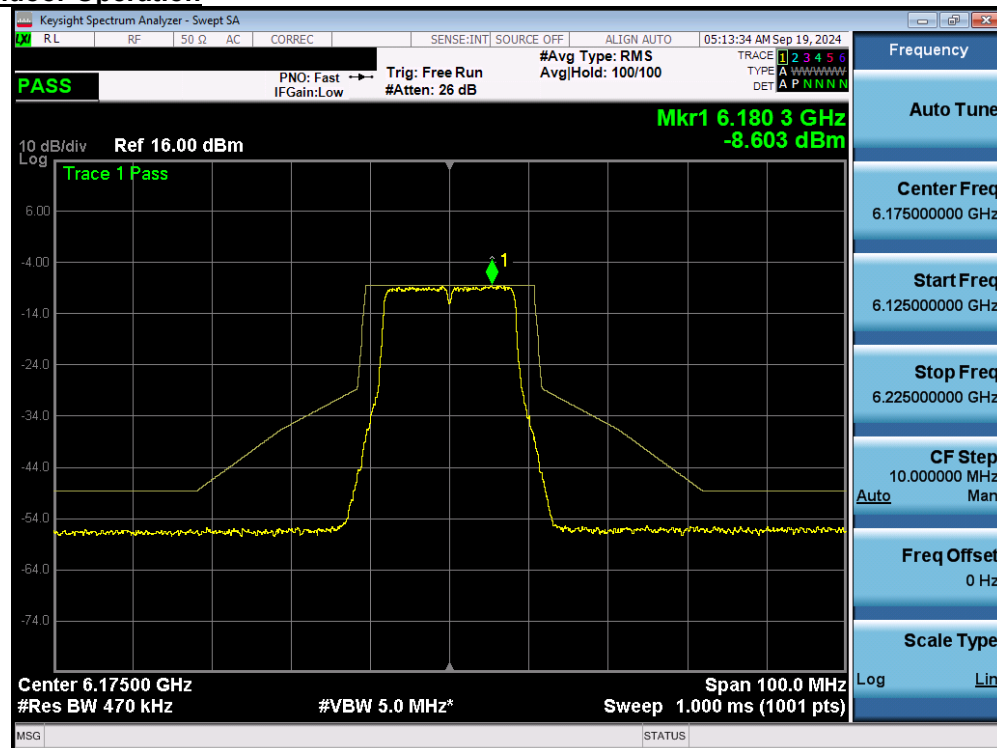
Plot 7-37. In Band Emissions Plot MIMO ANT1 (20MHz 802.11a (UNII Band 5) – Ch. 45) - LPI
