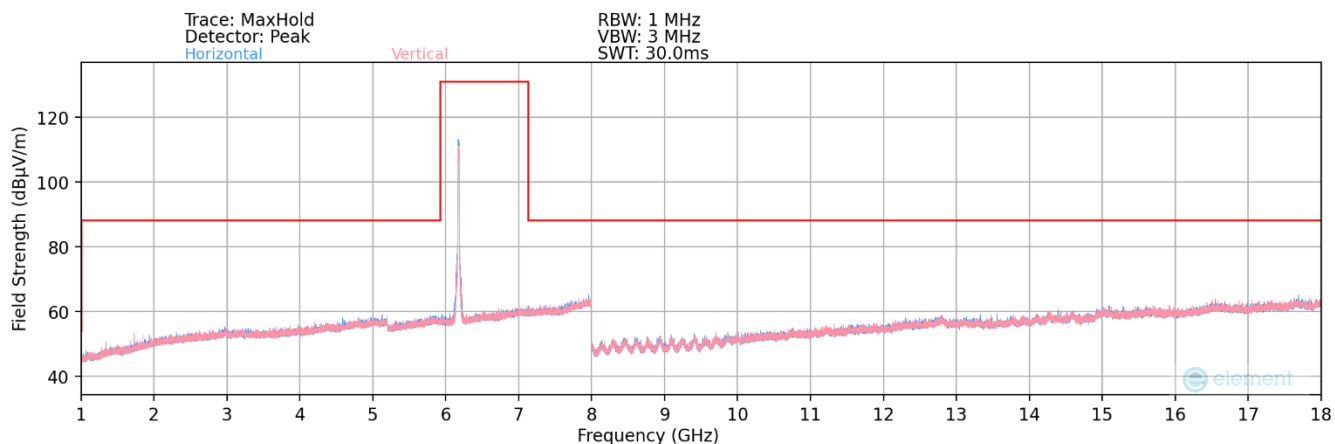
Plot 7-76. Radiated Spurious Plot 1GHz – 18GHz MIMO (802.11a – UNII Band 5 Ch. 45)
