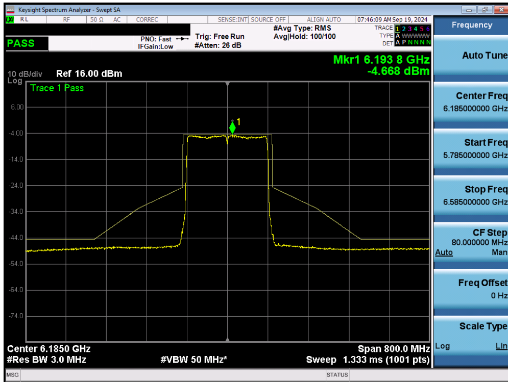
Plot 7-41. In Band Emissions Plot MIMO ANT1 (160MHz 802.11ax/be (UNII Band 5) – Ch. 47) - LPI
