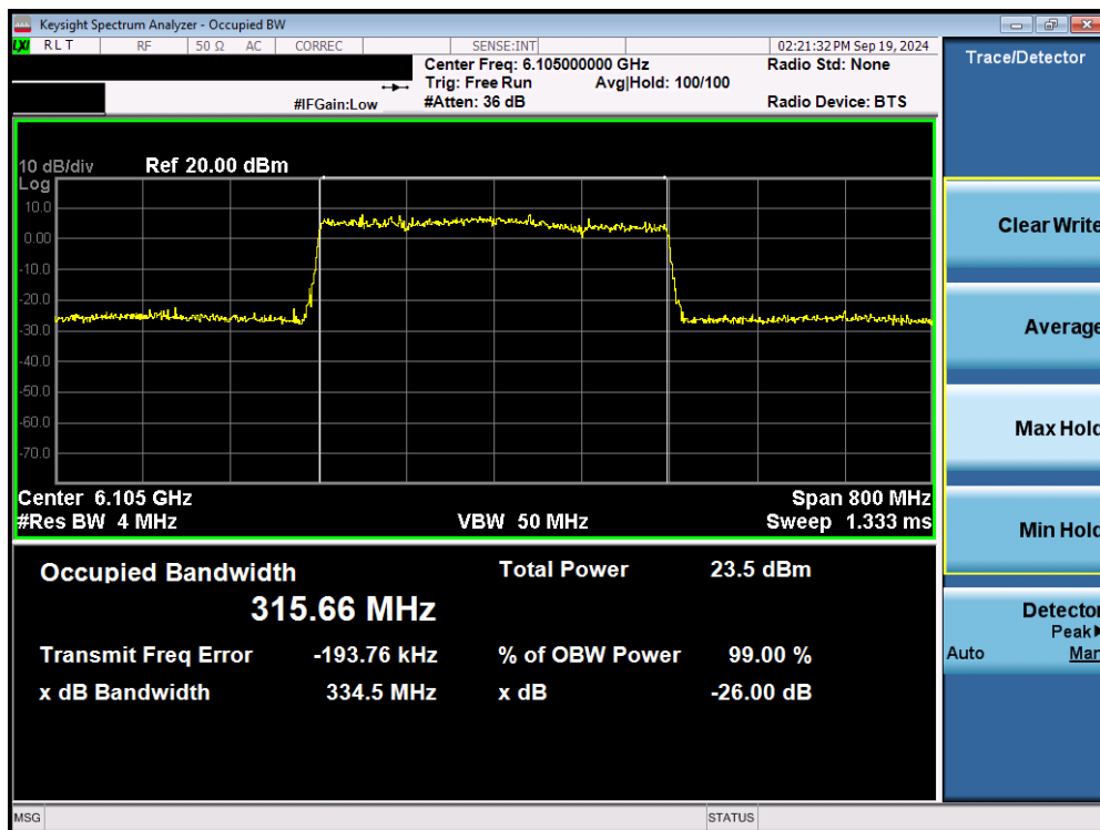
Plot 7-15. 26dB Bandwidth Plot MIMO ANT2 (320MHz 802.11ax/be (UNII Band 5) – Ch. 31) - LPI
