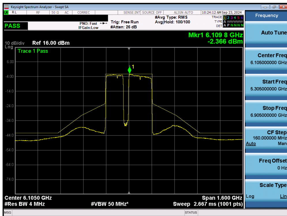
Plot 7-45. In Band Emissions Plot MIMO ANT1 (320MHz 802.11be (UNII Band 5) – Ch. 31) – 40MHz Punctured – LPI
