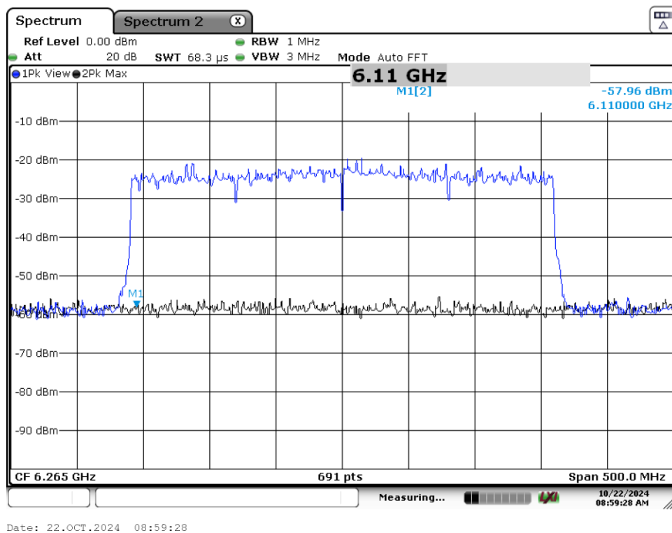
Plot 7-72. CBP 320MHz Channel - Injection Lower Edge – [6110 MHz]
