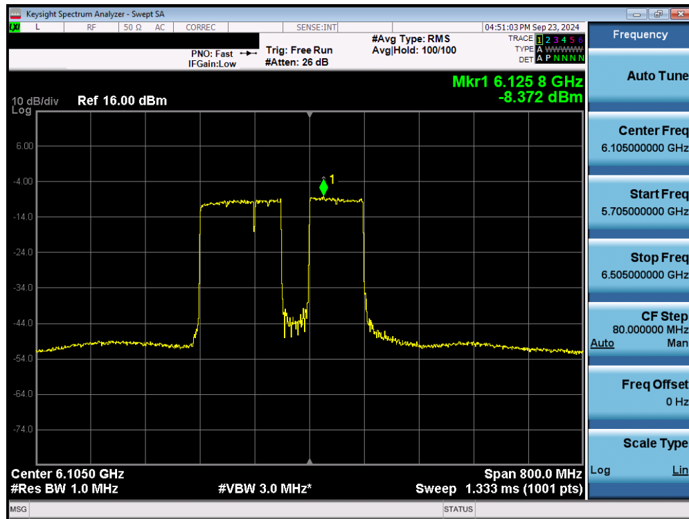
Plot 7-36. Power Spectral Density Plot MIMO ANT2 (320MHz 802.11be (UNII Band 5) – Ch. 31) – 120MHz Punctured – LPI
