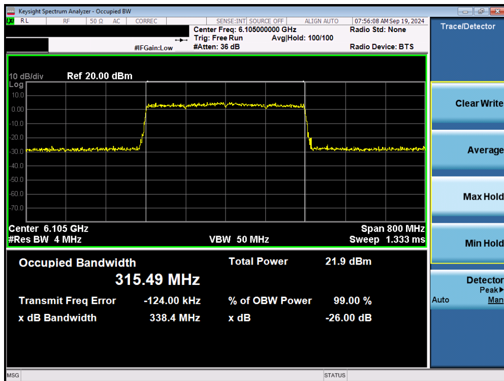
Plot 7-6. 26dB Bandwidth Plot MIMO ANT1 (320MHz 802.11ax/be (UNII Band 5) – Ch. 31) - LPI
