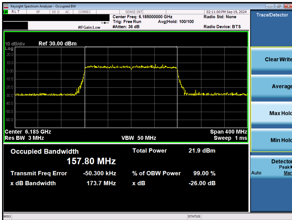
Plot 7-14. 26dB Bandwidth Plot MIMO ANT2 (160MHz 802.11ax/be (UNII Band 5) – Ch. 47) - LPI
