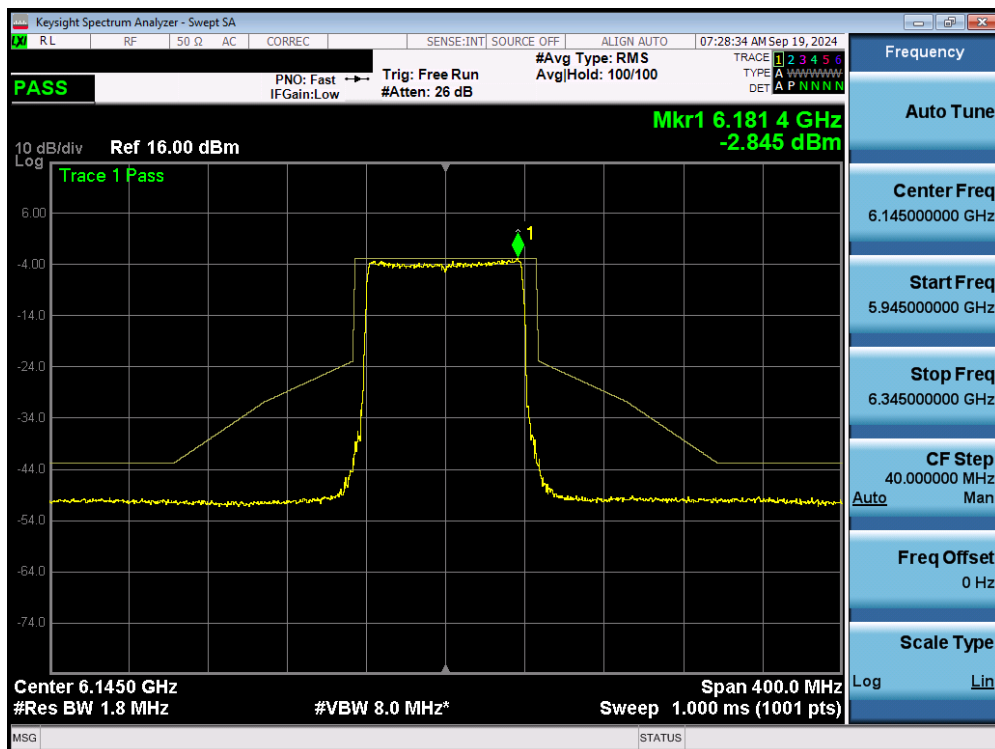
Plot 7-40. In Band Emissions Plot MIMO ANT1 (80MHz 802.11ax/be (UNII Band 5) – Ch. 39) - LPI
