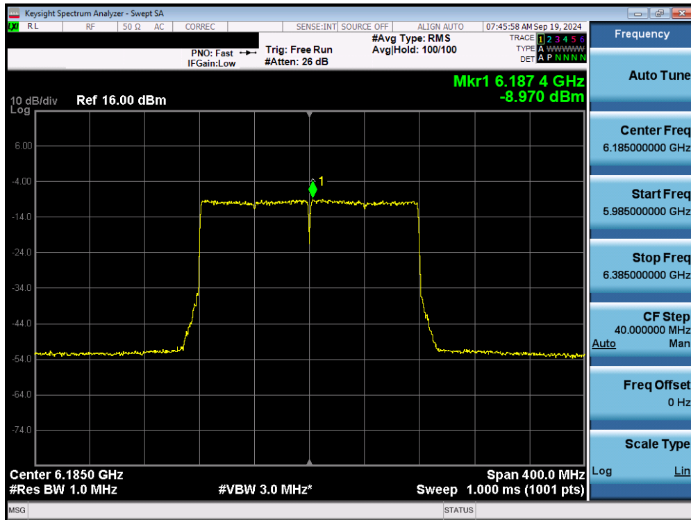
Plot 7-23. Power Spectral Density Plot MIMO ANT1 (160MHz 802.11ax/be (UNII Band 5) – Ch. 47) - LPI
