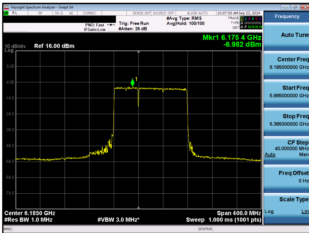
Plot 7-26. Power Spectral Density Plot MIMO ANT1 (160MHz 802.11be (UNII Band 5) – Ch. 47) – 40MHz Punctured - LPI
