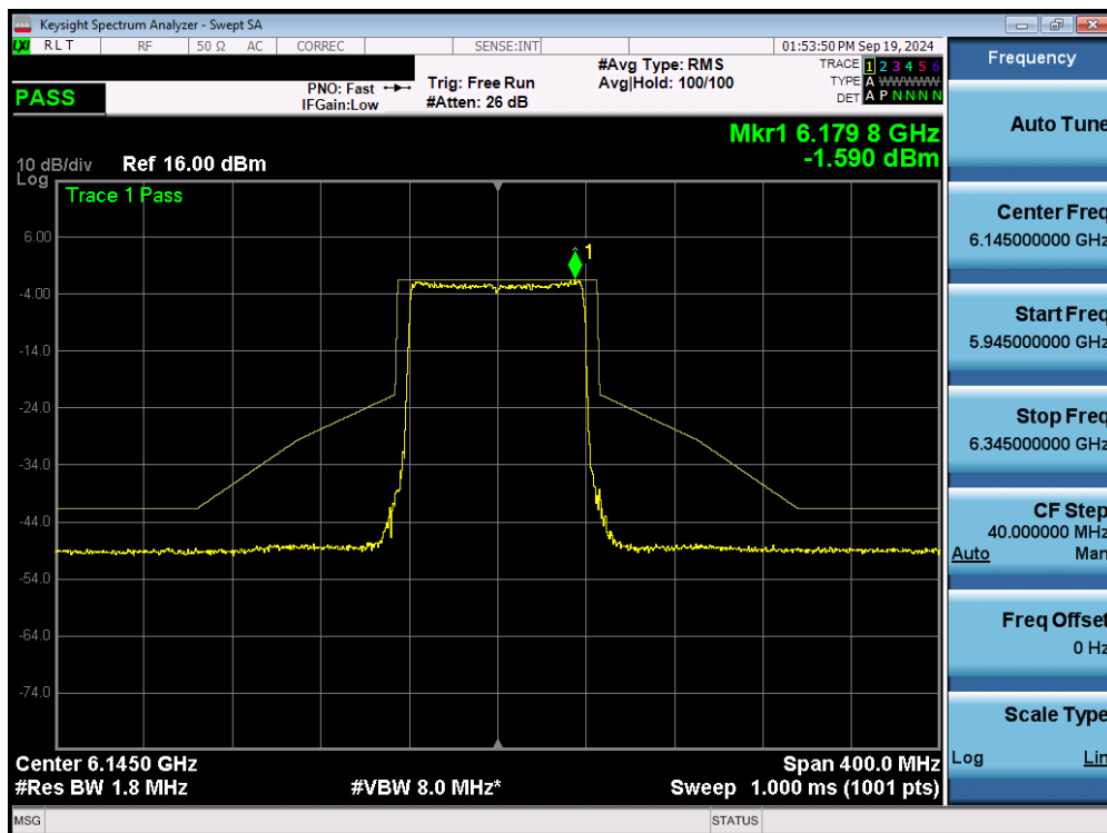
Plot 7-49. In Band Emissions Plot MIMO ANT2 (80MHz 802.11ax/be (UNII Band 5) – Ch. 39) - LPI
