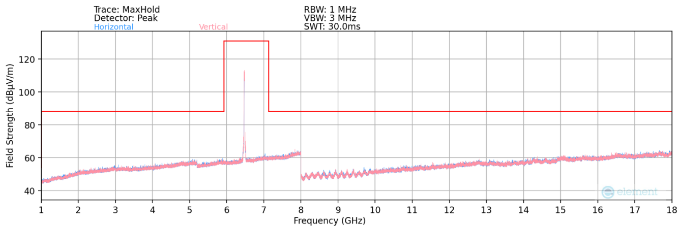
Plot 7-77. Radiated Spurious Plot 1GHz – 18GHz MIMO (802.11a – UNII Band 6 Ch. 105)
