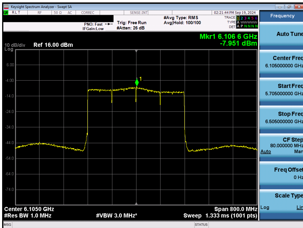
Plot 7-33. Power Spectral Density Plot MIMO ANT2 (320MHz 802.11ax/be (UNII Band 5) – Ch. 31) - LPI
