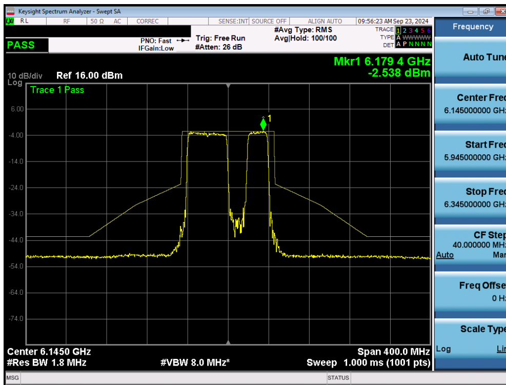
Plot 7-43. In Band Emissions Plot MIMO ANT1 (80MHz 802.11be (UNII Band 5) – Ch. 39) – 20MHz Punctured - LPI
