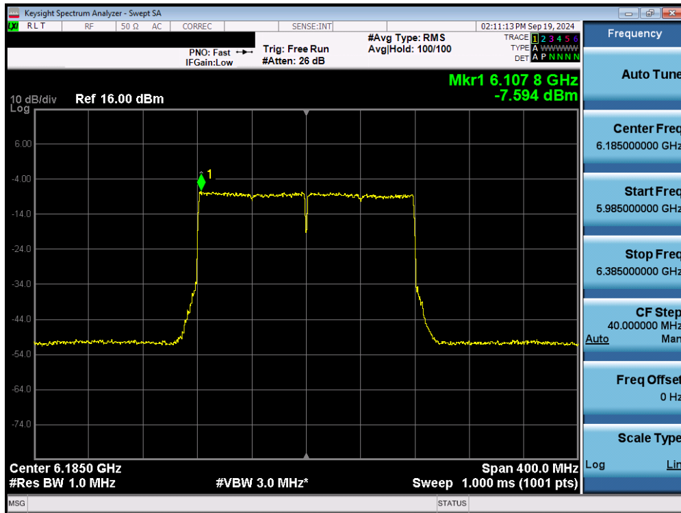
Plot 7-32. Power Spectral Density Plot MIMO ANT2 (160MHz 802.11ax/be (UNII Band 5) – Ch. 47) - LPI
