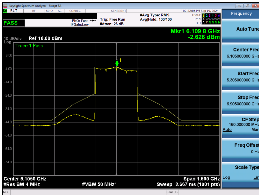
Plot 7-51. In Band Emissions Plot MIMO ANT2 (320MHz 802.11ax/be (UNII Band 5) – Ch. 31) - LPI
