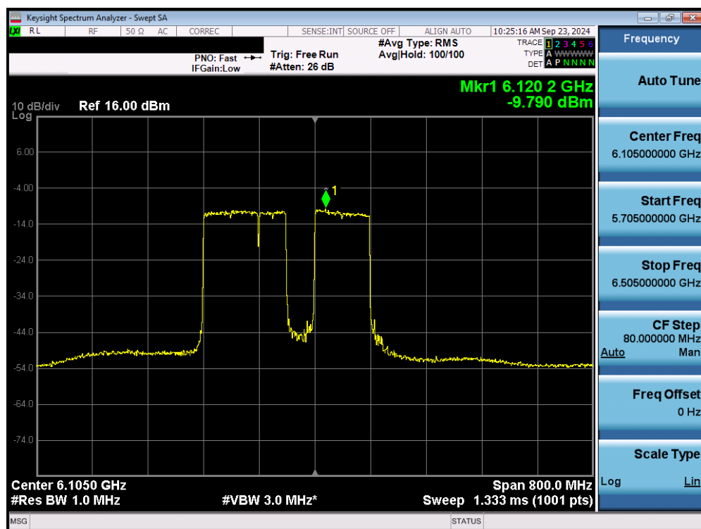
Plot 7-27. Power Spectral Density Plot MIMO ANT1 (320MHz 802.11be (UNII Band 5) – Ch. 31) – 120MHz Punctured – LPI
