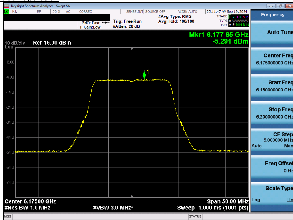
Plot 7-19. Power Spectral Density Plot MIMO ANT1 (20MHz 802.11a (UNII Band 5) – Ch. 45) - LPI
