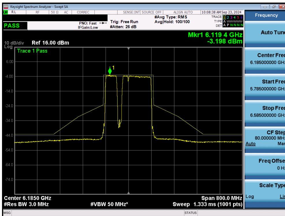
Plot 7-44. In Band Emissions Plot MIMO ANT1 (160MHz 802.11be (UNII Band 5) – Ch. 47) – 20MHz Punctured - LPI
