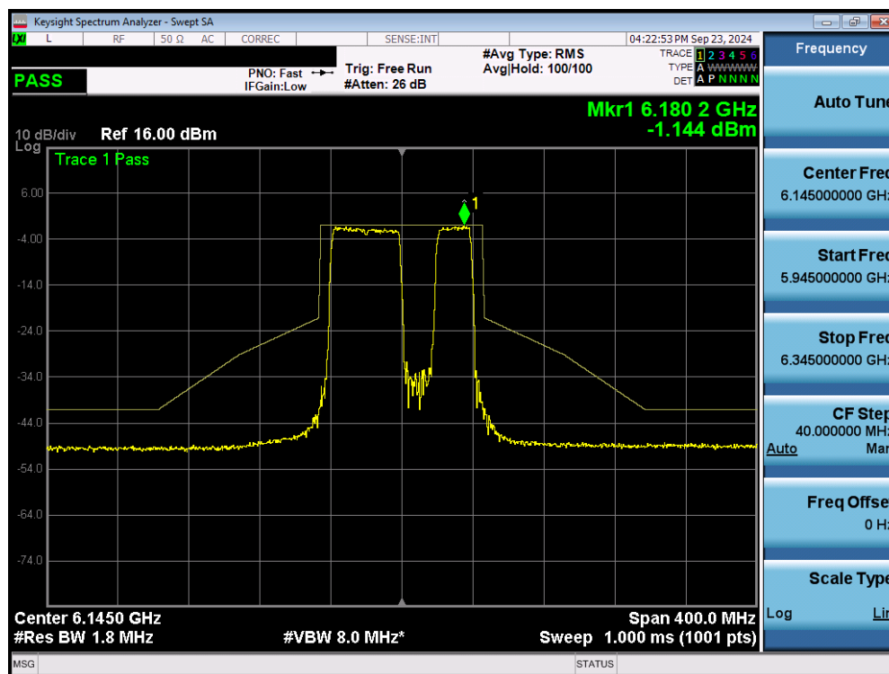
Plot 7-52. In Band Emissions Plot MIMO ANT2 (80MHz 802.11be (UNII Band 5) – Ch. 39) – 20MHz Punctured - LPI
