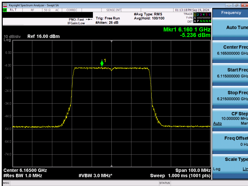
Plot 7-30. Power Spectral Density Plot MIMO ANT2 (40MHz 802.11ax/be (UNII Band 5) – Ch. 43) - LPI
