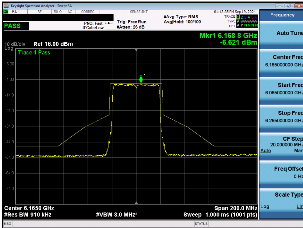
Plot 7-48. In Band Emissions Plot MIMO ANT2 (40MHz 802.11ax/be (UNII Band 5) – Ch. 43) - LPI
