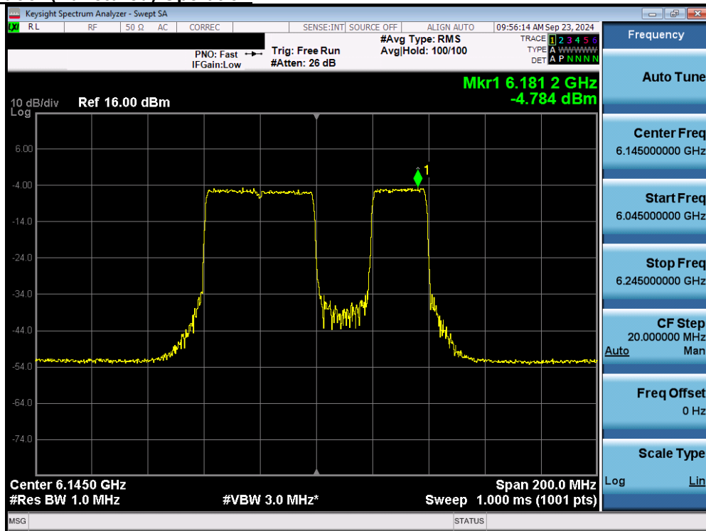
Plot 7-25. Power Spectral Density Plot MIMO ANT1 (80MHz 802.11be (UNII Band 5) – Ch. 39) – 20MHz Punctured - LPI
