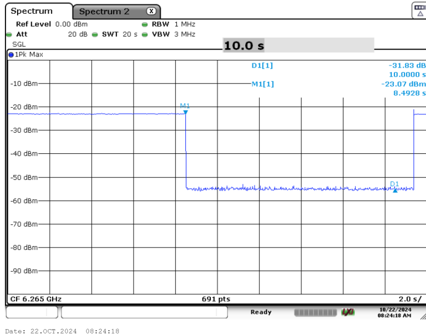
Plot 7-58. Contention Based Protocol Timing Plot (320MHz (UNII Band 5) – Ch. 63 Mid)
