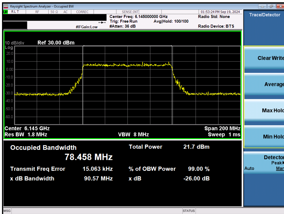
Plot 7-13. 26dB Bandwidth Plot MIMO ANT2 (80MHz 802.11ax/be (UNII Band 5) – Ch. 39) - LPI
