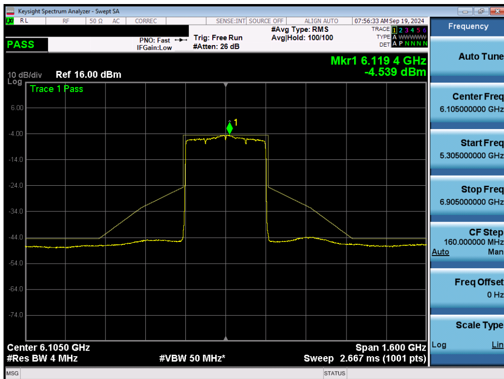
Plot 7-42. In Band Emissions Plot MIMO ANT1 (320MHz 802.11ax/be (UNII Band 5) – Ch. 31) - LPI
