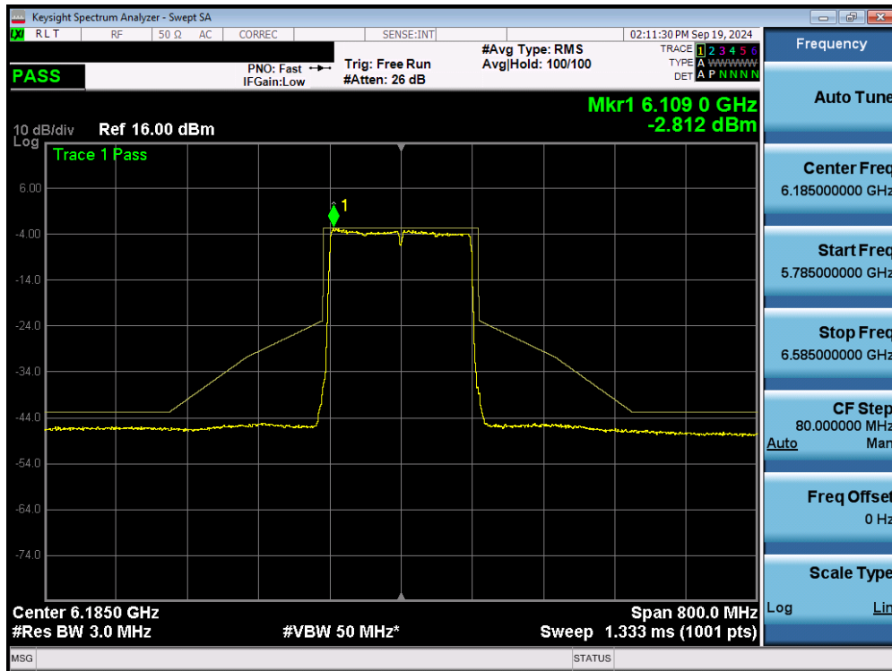
Plot 7-50. In Band Emissions Plot MIMO ANT2 (160MHz 802.11ax/be (UNII Band 5) – Ch. 47) - LPI
