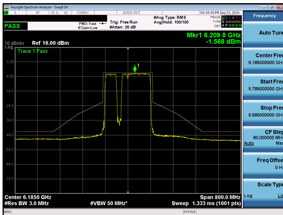
Plot 7-53. In Band Emissions Plot MIMO ANT2 (160MHz 802.11be (UNII Band 5) – Ch. 47) – 20MHz Punctured - LPI
