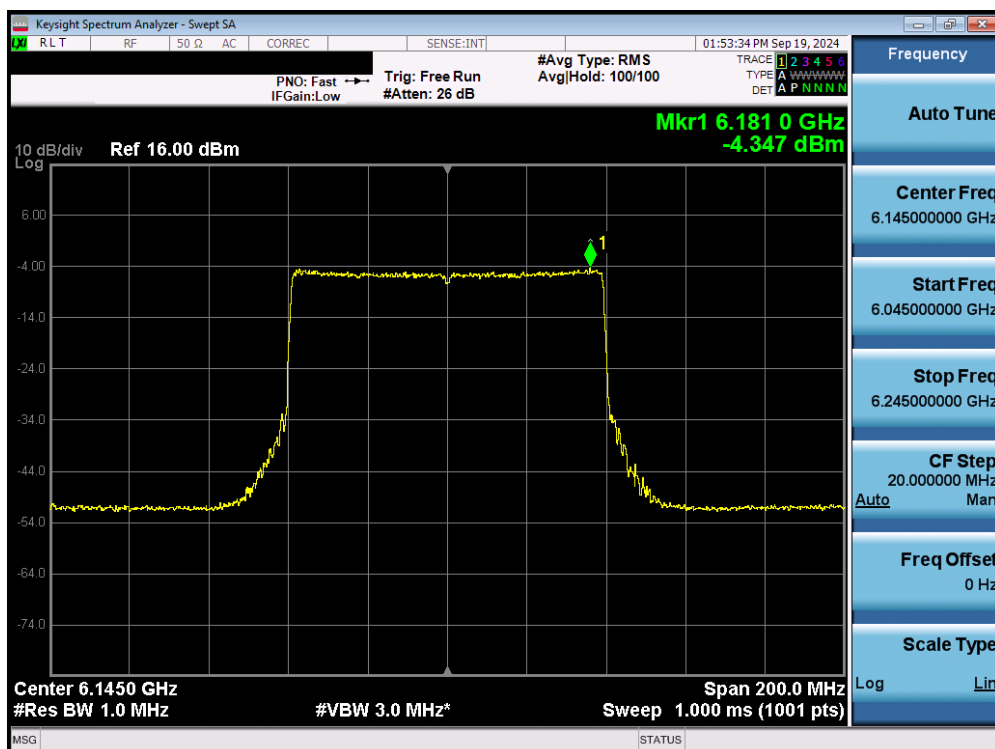
Plot 7-31. Power Spectral Density Plot MIMO ANT2 (80MHz 802.11ax/be (UNII Band 5) – Ch. 39) - LPI
