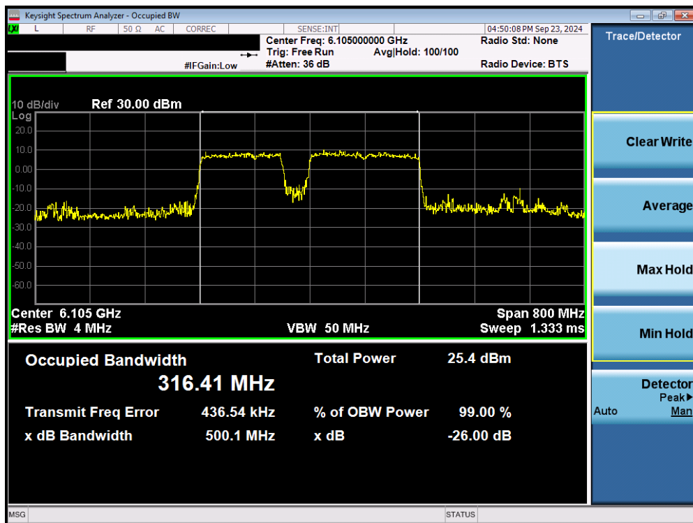
Plot 7-18. 26dB Bandwidth Plot MIMO ANT2 (320MHz 802.11be (UNII Band 5) – Ch. 31) – 40MHz Punctured – LPI
