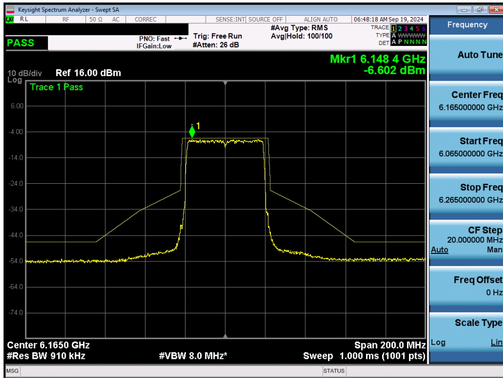
Plot 7-39. In Band Emissions Plot MIMO ANT1 (40MHz 802.11ax/be (UNII Band 5) – Ch. 43) - LPI
