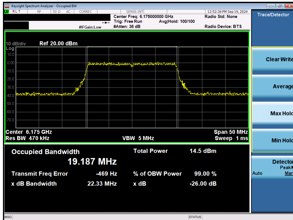
Plot 7-11. 26dB Bandwidth Plot MIMO ANT2 (20MHz 802.11ax/be (UNII Band 5) – Ch. 45) - LPI
