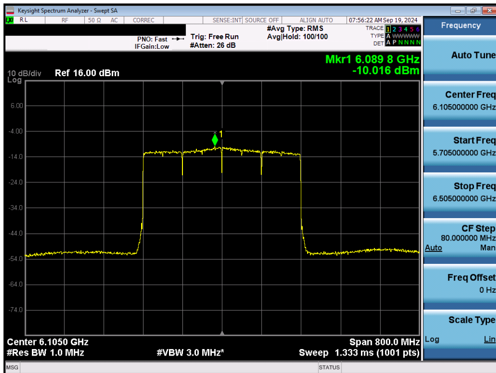
Plot 7-24. Power Spectral Density Plot MIMO ANT1 (320MHz 802.11ax/be (UNII Band 5) – Ch. 31) - LPI
