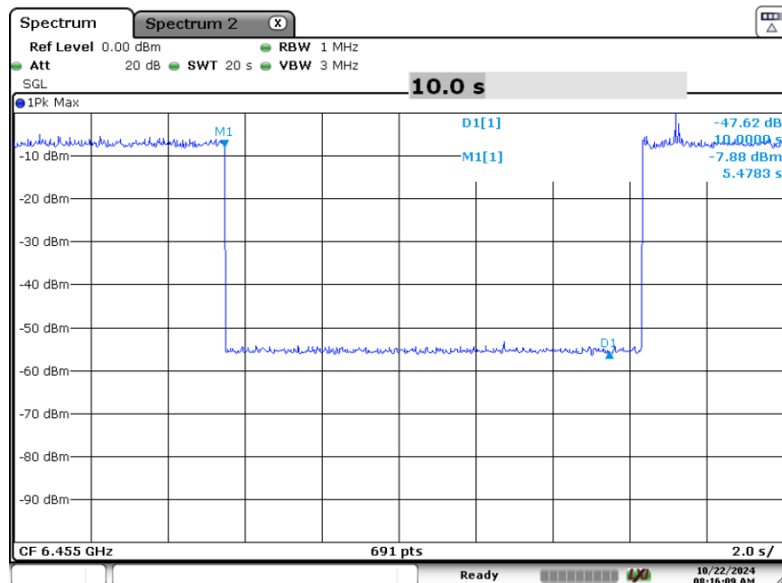
Plot 7-60. Contention Based Protocol Timing Plot (20MHz (UNII Band 6) – Ch. 101)
