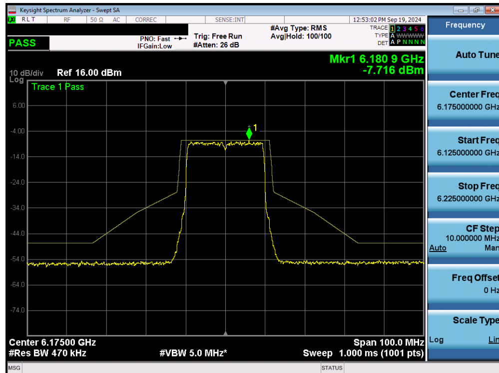
Plot 7-47. In Band Emissions Plot MIMO ANT2 (20MHz 802.11ax/be (UNII Band 5) – Ch. 45) - LPI
