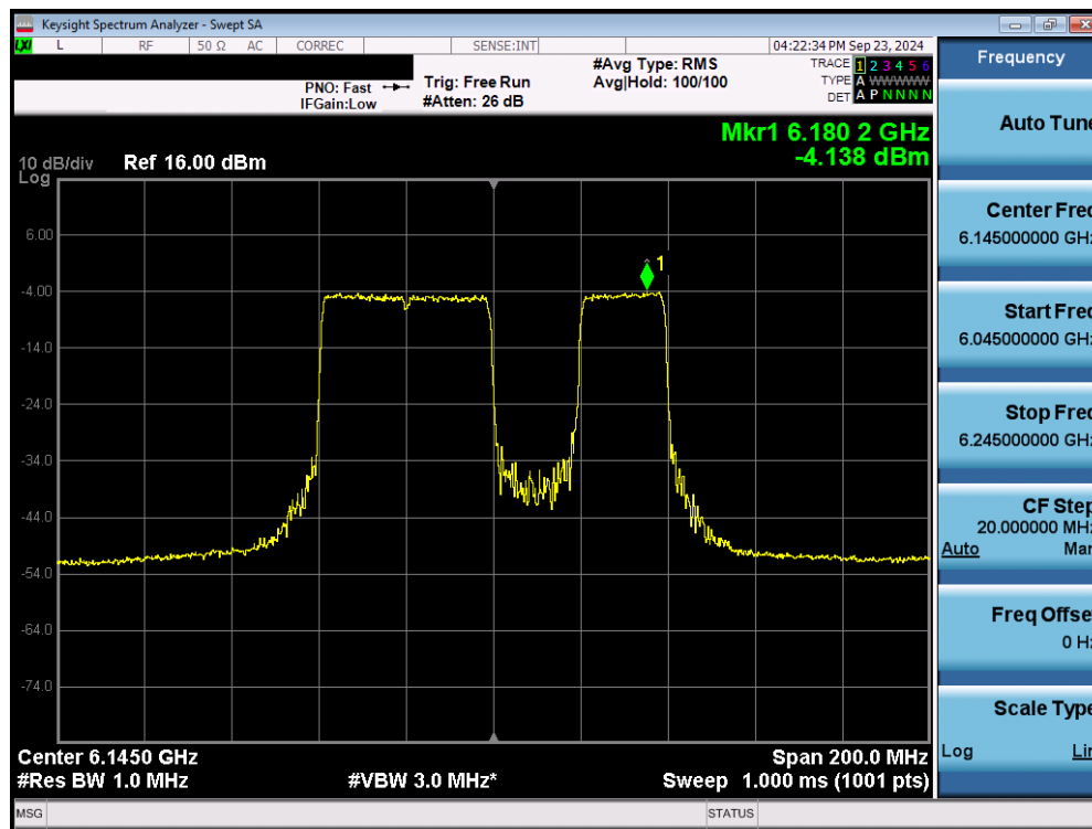
Plot 7-34. Power Spectral Density Plot MIMO ANT2 (80MHz 802.11be (UNII Band 5) – Ch. 39) – 20MHz Punctured - LPI
