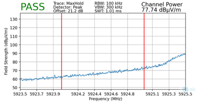
Plot 7-84. Radiated Lower Band Edge Plot MIMO (Peak – UNII Band 5)
