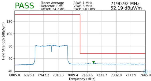
Plot 7-99. Radiated Upper Band Edge Plot MIMO (Average – UNII Band 8)
