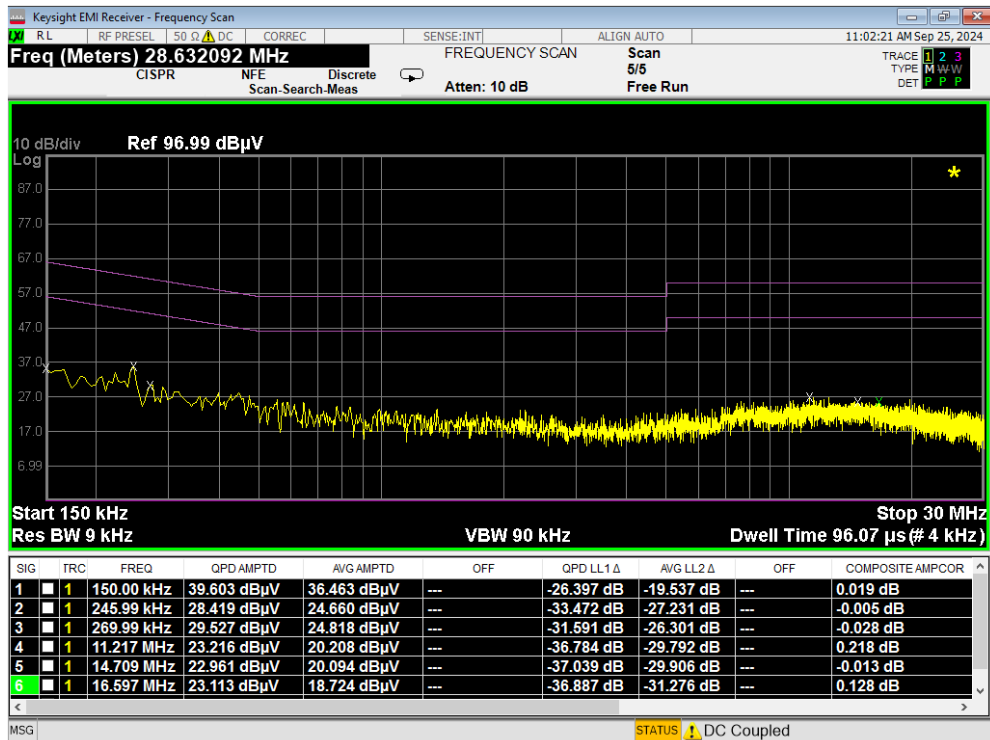
Plot 7-112. Line Conducted Plot with 802.11a UNII Band 6 (N)
