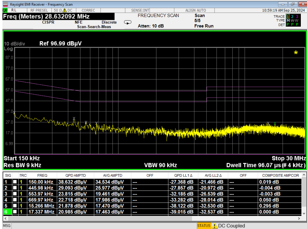
Plot 7-109. Line Conducted Plot with 802.11a UNII Band 5 (L1)
