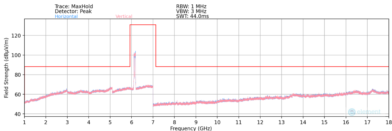
Plot 7-82. Radiated Spurious Plot 1GHz - 18GHz MIMO (802.11be (20MHz Puncture) - UNII Band 5 Ch. 39)
