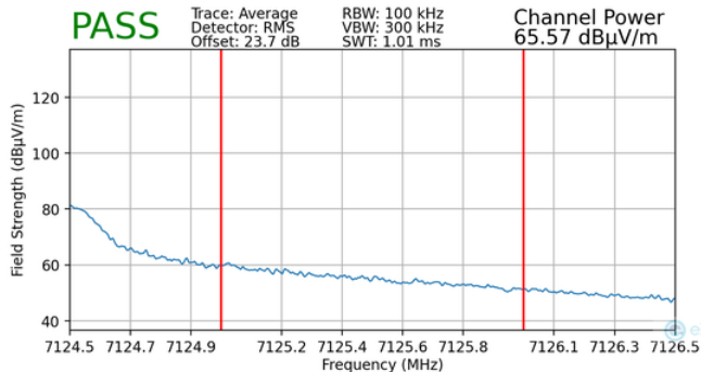
Plot 7-85. Radiated Upper Band Edge Plot MIMO (Average – UNII Band 8)
