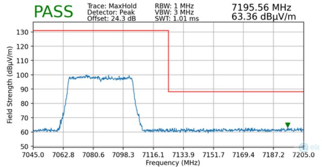
Plot 7-90. Radiated Upper Band Edge Plot MIMO (Peak – UNII Band 8)
