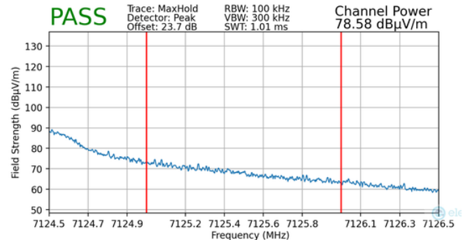
Plot 7-86. Radiated Upper Band Edge Plot MIMO (Peak – UNII Band 8)
