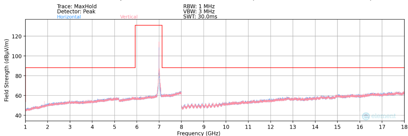
Plot 7-79. Radiated Spurious Plot 1GHz – 18GHz MIMO (802.11a – UNII Band 8 Ch. 209)
