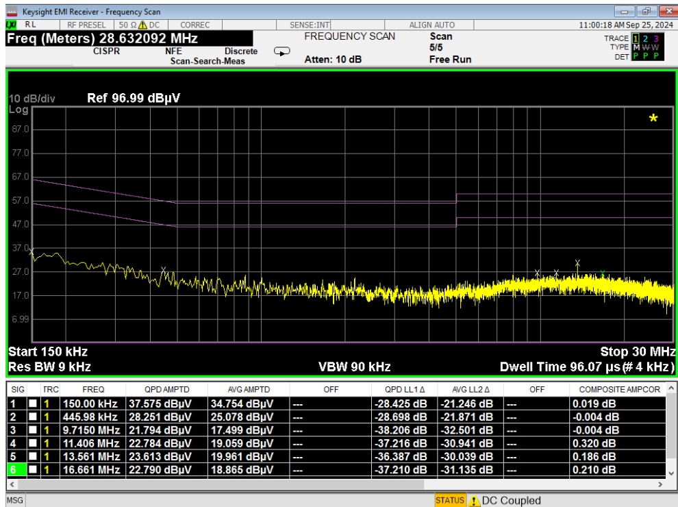
Plot 7-110. Line Conducted Plot with 802.11a UNII Band 5 (N)
