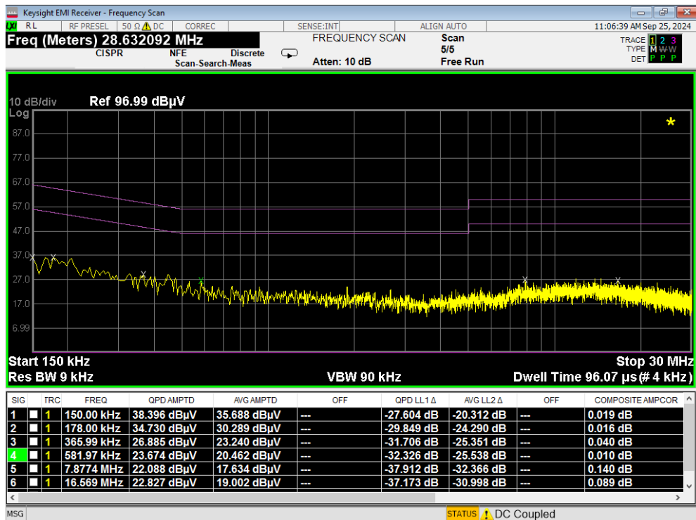
Plot 7-114. Line Conducted Plot with 802.11a UNII Band 7 (N)
