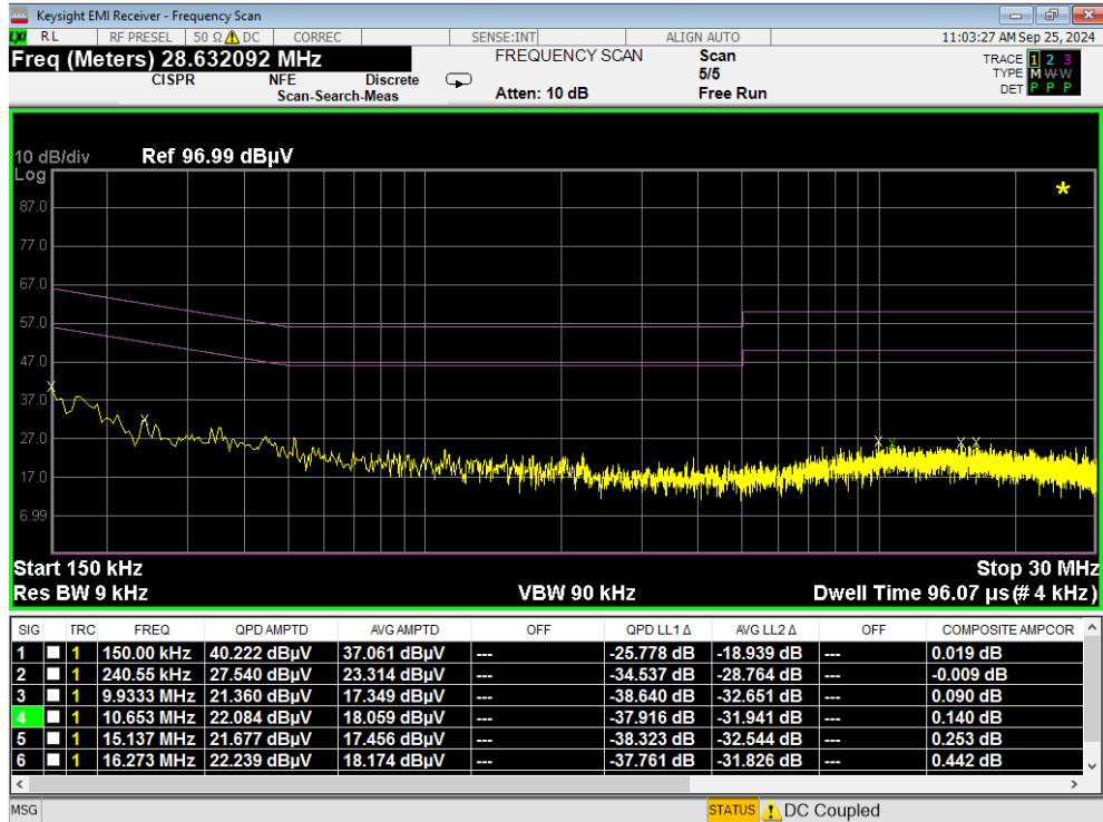
Plot 7-111. Line Conducted Plot with 802.11a UNII Band 6 (L1)
