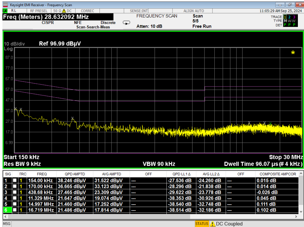
Plot 7-113. Line Conducted Plot with 802.11a UNII Band 7 (L1)
