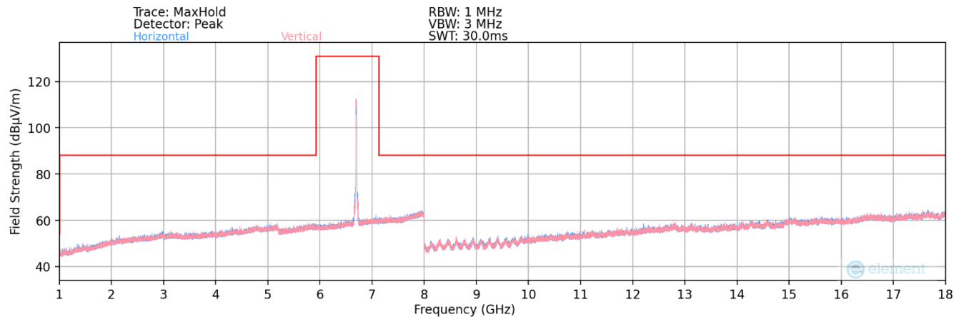
Plot 7-78. Radiated Spurious Plot 1GHz – 18GHz MIMO (802.11a – UNII Band 7 Ch. 149)
