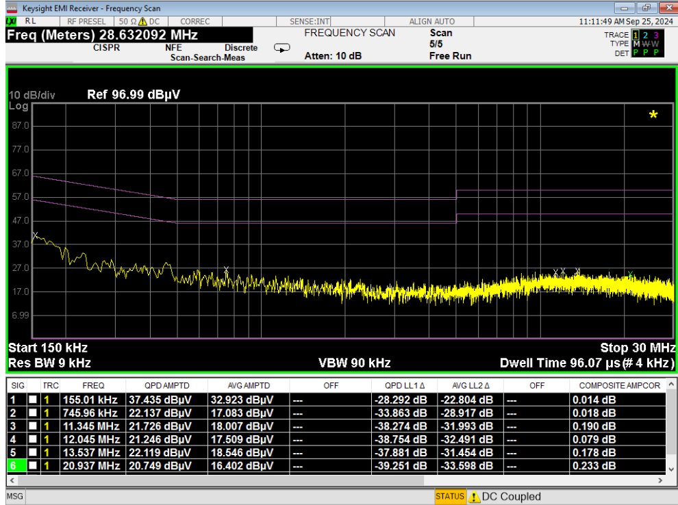
Plot 7-115. Line Conducted Plot with 802.11a UNII Band 8 (L1)
