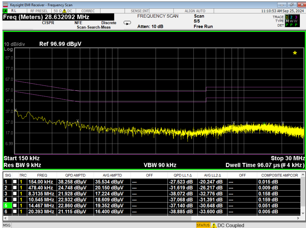
Plot 7-116. Line Conducted Plot with 802.11a UNII Band 8 (N)
