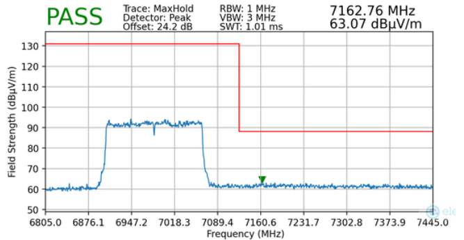
Plot 7-100. Radiated Upper Band Edge Plot MIMO (Peak – UNII Band 8)
