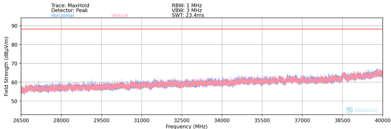
Plot 7-81. Radiated Spurious Plot 26.5GHz - 40GHz (802.11a)
