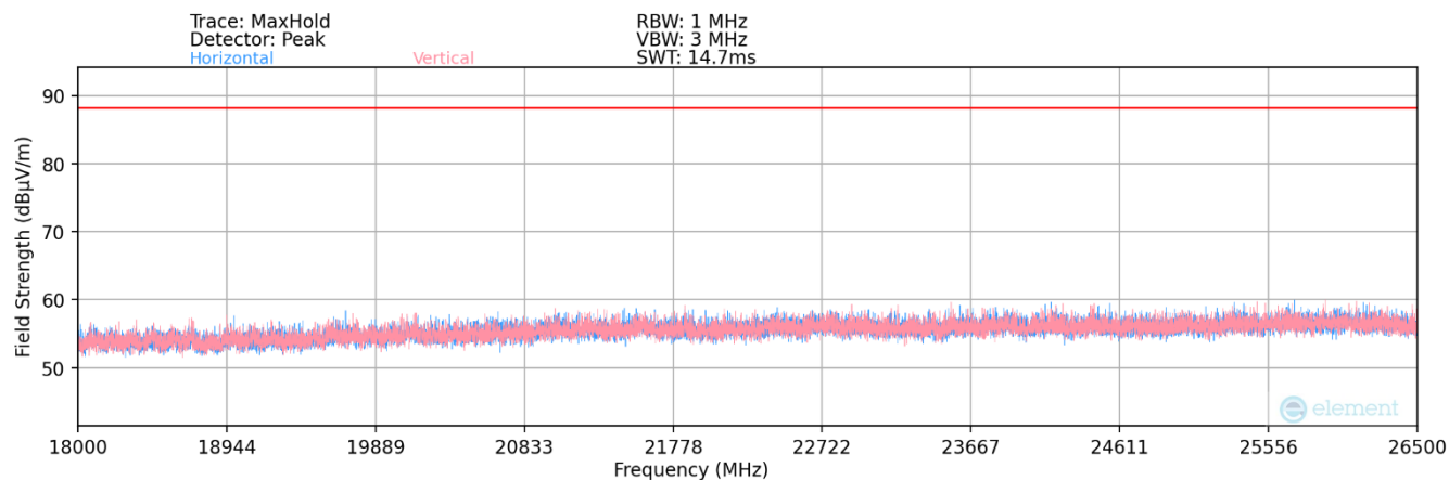
Plot 7-80. Radiated Spurious Plot 18GHz - 26.5GHz (802.11a)
