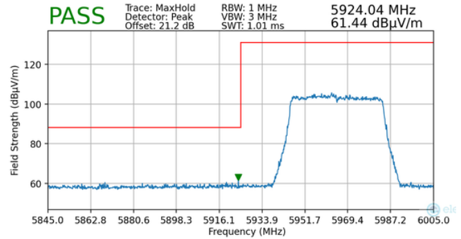
Plot 7-88. Radiated Lower Band Edge Plot MIMO (Peak – UNII Band 5)
