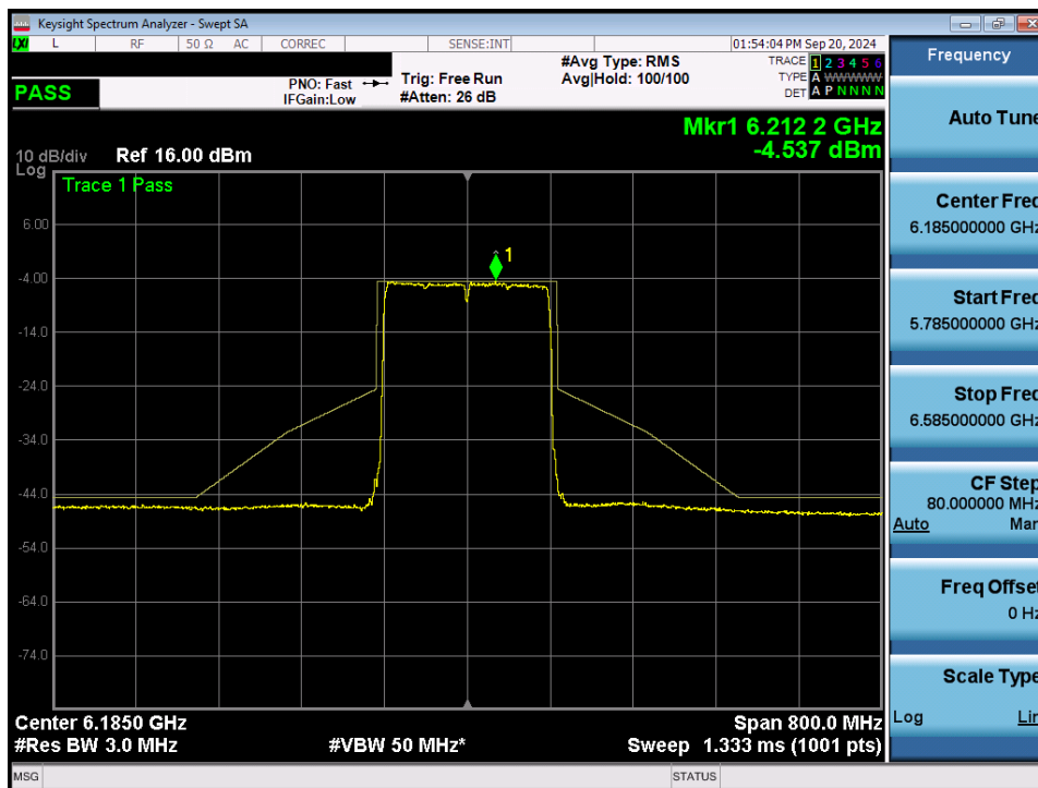
Plot 7-92. In Band Emissions Plot MIMO ANT2 (160MHz 802.11ax/be (Full Tones) (UNII Band 5) – Ch. 47) - LPI
