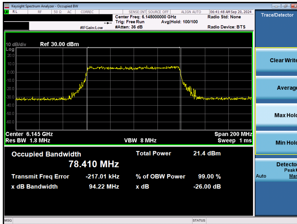
Plot 7-9. 26dB Bandwidth Plot MIMO ANT1 (80MHz 802.11ax/be (Full Tones) (UNII Band 5) – Ch. 39) - LPI
