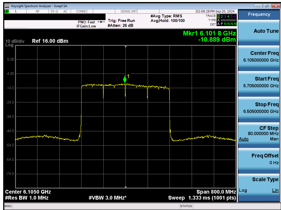
Plot 7-66. Power Spectral Density Plot MIMO ANT2 (320MHz 802.11ax/be (Full Tones) (UNII Band 5) – Ch. 31) - LPI
