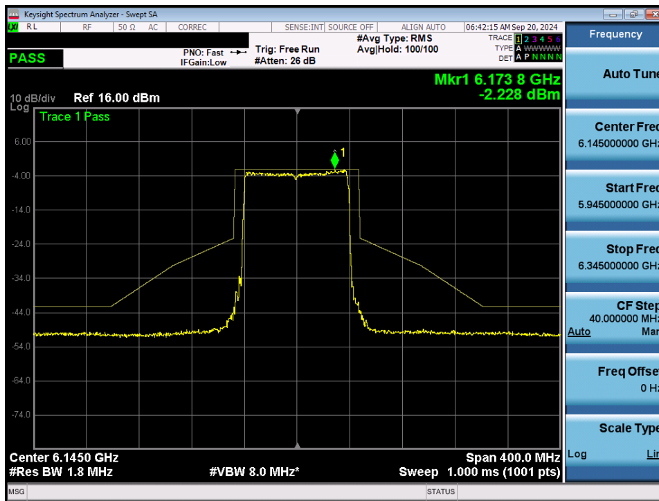
Plot 7-75. In Band Emissions Plot MIMO ANT1 (80MHz 802.11ax/be (Full Tones) (UNII Band 5) – Ch. 39) - LPI
