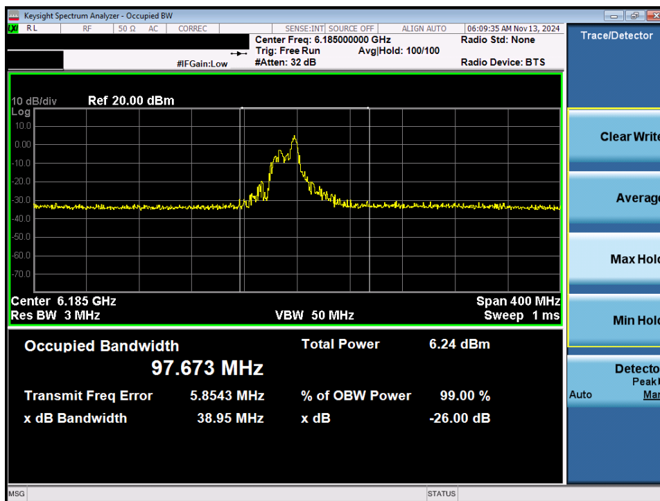
Plot 7-5. 26dB Bandwidth Plot MIMO ANT1 (160MHz 802.11ax/be (26 Tones) (UNII Band 5) – Ch. 47) - LPI
