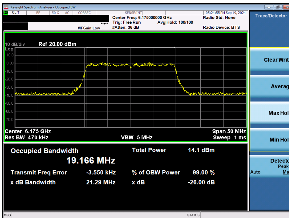
Plot 7-28. 26dB Bandwidth Plot MIMO ANT2 (20MHz 802.11ax/be (Full Tones) (UNII Band 5) – Ch. 45) - LPI
