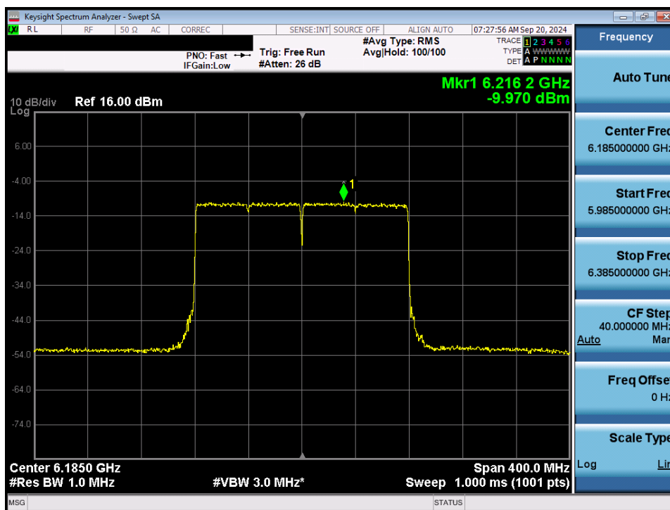
Plot 7-48. Power Spectral Density Plot MIMO ANT1 (160MHz 802.11ax/be (Full Tones) (UNII Band 5) – Ch. 47) - LPI
