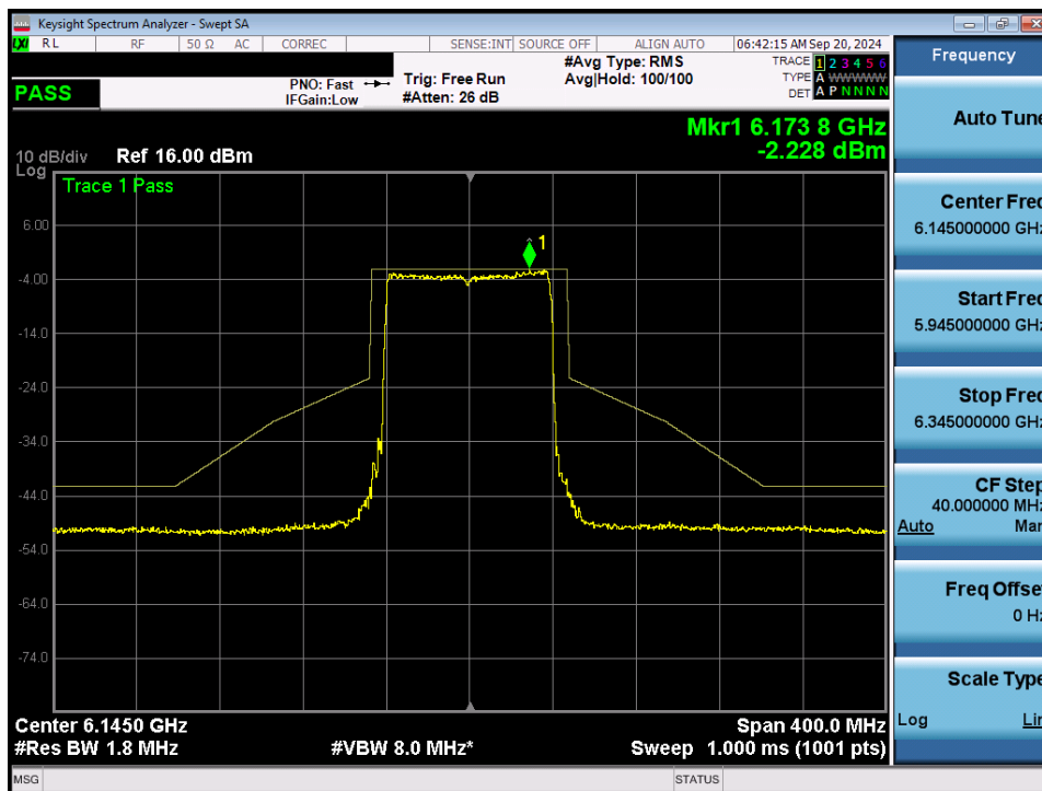
Plot 7-80. In Band Emissions Plot MIMO ANT1 (80MHz 802.11ax/be (Full Tones) (UNII Band 5) – Ch. 39) - LPI
