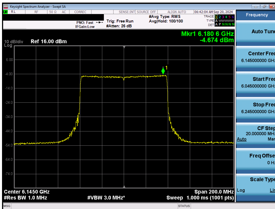
Plot 7-47. Power Spectral Density Plot MIMO ANT1 (80MHz 802.11ax/be (Full Tones) (UNII Band 5) – Ch. 39) - LPI
