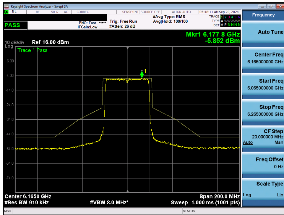
Plot 7-74. In Band Emissions Plot MIMO ANT1 (40MHz 802.11ax/be (Full Tones) (UNII Band 5) – Ch. 43) - LPI
