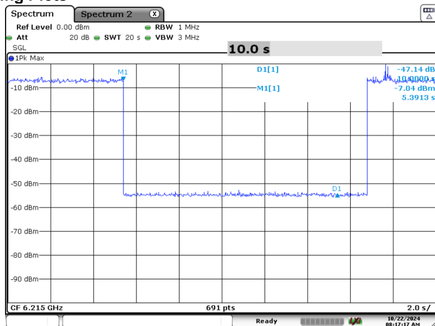
Plot 7-100. Contention Based Protocol Timing Plot (20MHz (UNII Band 5) – Ch. 53)
