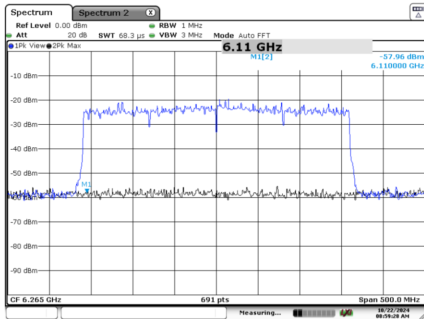
Plot 7-116. CBP 320MHz Channel - Injection Lower Edge – [6110 MHz]
