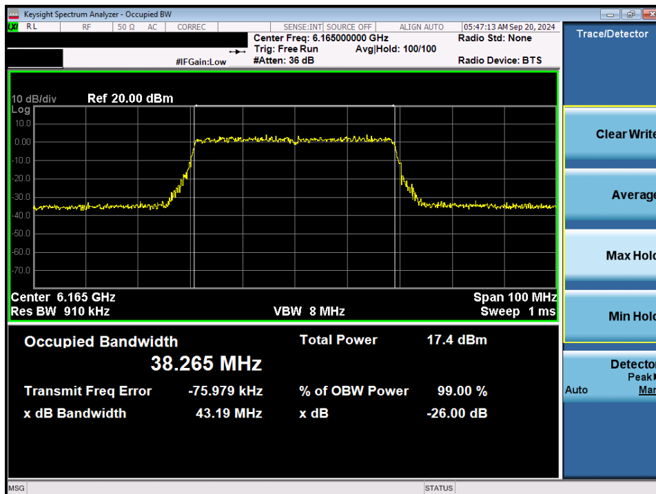
Plot 7-8. 26dB Bandwidth Plot MIMO ANT1 (40MHz 802.11ax/be (Full Tones) (UNII Band 5) – Ch. 43) - LPI
