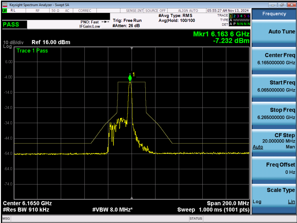
Plot 7-69. In Band Emissions Plot MIMO ANT1 (40MHz 802.11ax/be (26 Tones) (UNII Band 5) – Ch. 43) - LPI
