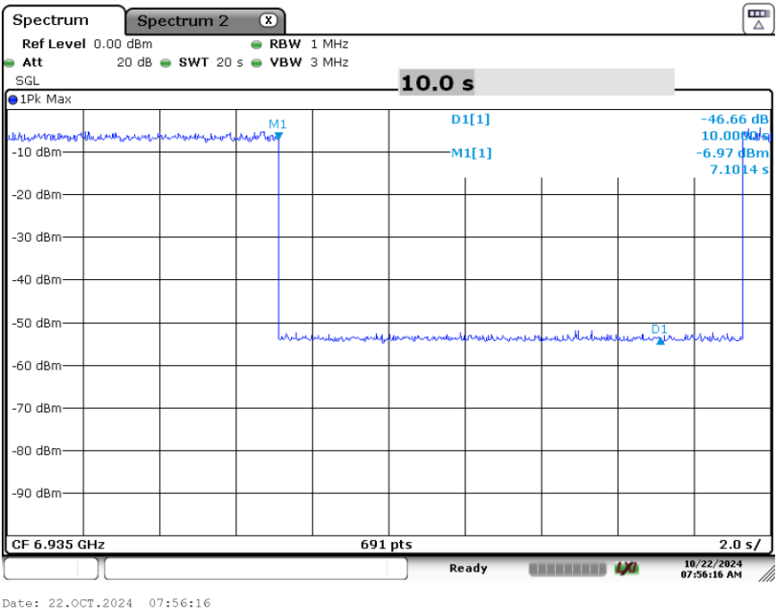
Plot 7-112. Contention Based Protocol Timing Plot (20MHz (UNII Band 8) – Ch. 197)
