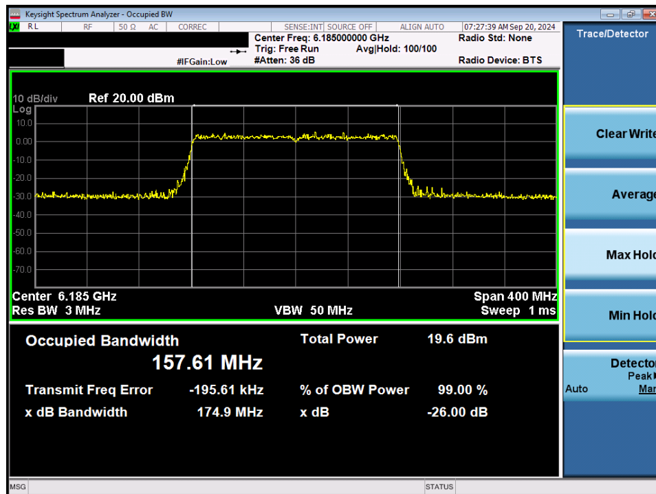
Plot 7-10. 26dB Bandwidth Plot MIMO ANT1 (160MHz 802.11ax/be (Full Tones) (UNII Band 5) – Ch. 47) - LPI
