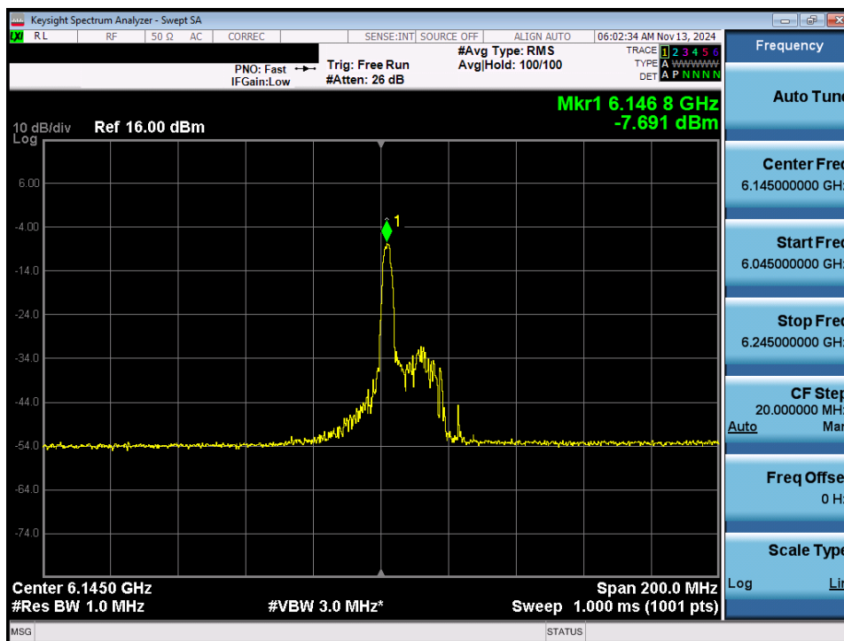
Plot 7-37. Power Spectral Density Plot MIMO ANT1 (80MHz 802.11ax/be (26 Tones) (UNII Band 5) – Ch. 39) - LPI
