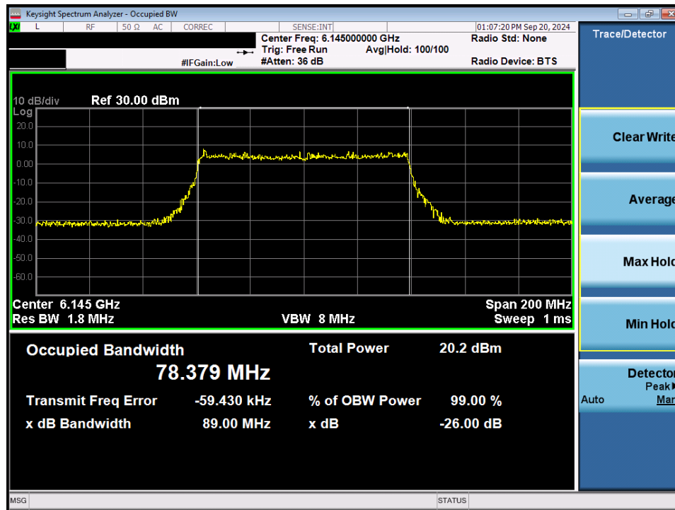
Plot 7-25. 26dB Bandwidth Plot MIMO ANT2 (80MHz 802.11ax/be (Full Tones) (UNII Band 5) – Ch. 39) - LPI
