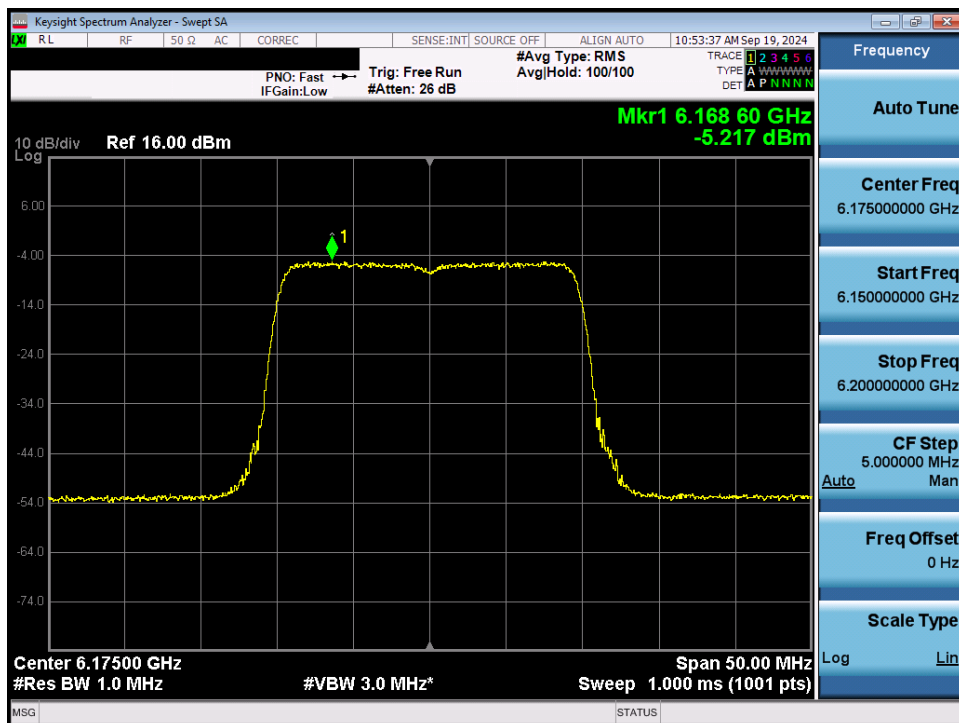
Plot 7-45. Power Spectral Density Plot MIMO ANT1 (20MHz 802.11ax/be (Full Tones) (UNII Band 5) – Ch. 45) - LPI
