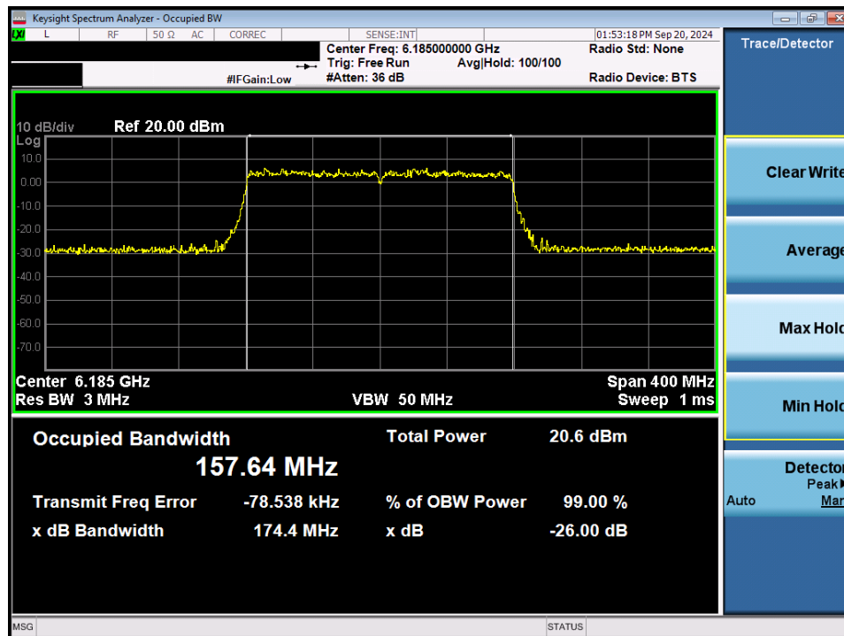
Plot 7-26. 26dB Bandwidth Plot MIMO ANT2 (160MHz 802.11ax/be (Full Tones) (UNII Band 5) – Ch. 47) - LPI
