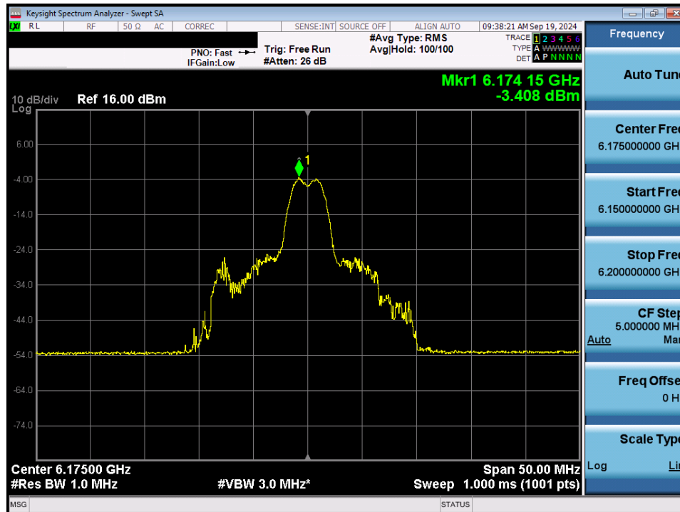
Plot 7-35. Power Spectral Density Plot MIMO ANT1 (20MHz 802.11ax/be (26 Tones) (UNII Band 5) – Ch. 45) - LPI
