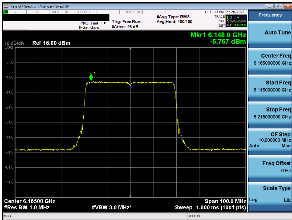
Plot 7-63. Power Spectral Density Plot MIMO ANT2 (40MHz 802.11ax/be (Full Tones) (UNII Band 5) – Ch. 43) - LPI
