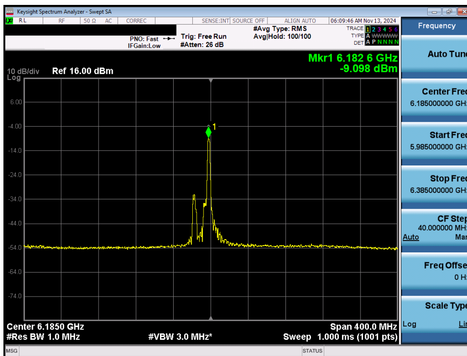
Plot 7-38. Power Spectral Density Plot MIMO ANT1 (160MHz 802.11ax/be (26 Tones) (UNII Band 5) – Ch. 47) - LPI
