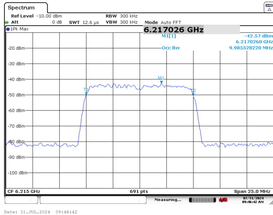
Plot 7-99. AWGN Signal (Demonstration)
