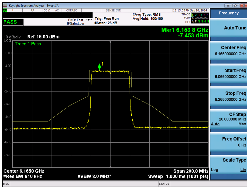
Plot 7-90. In Band Emissions Plot MIMO ANT2 (40MHz 802.11ax/be (Full Tones) (UNII Band 5) – Ch. 43) - LPI
