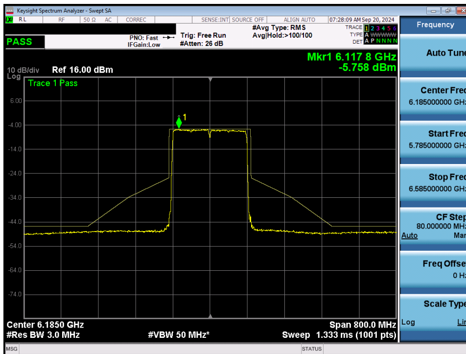
Plot 7-76. In Band Emissions Plot MIMO ANT1 (160MHz 802.11ax/be (Full Tones) (UNII Band 5) – Ch. 47) - LPI
