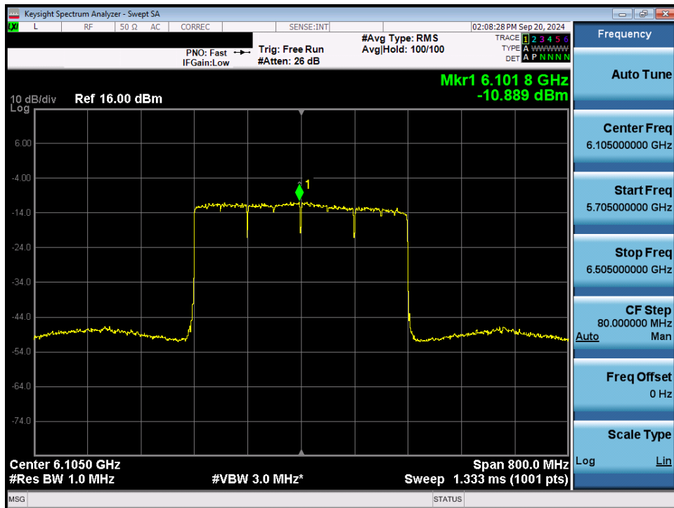
Plot 7-61. Power Spectral Density Plot MIMO ANT2 (320MHz 802.11ax/be (Full Tones) (UNII Band 5) – Ch. 31) - LPI
