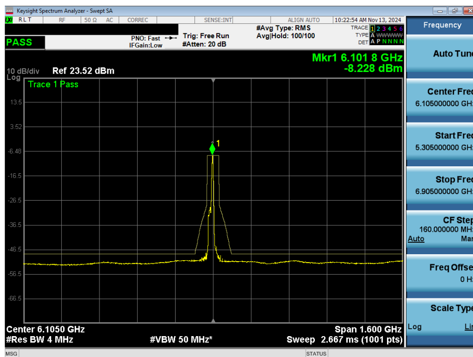
Plot 7-88. In Band Emissions Plot MIMO ANT2 (320MHz 802.11ax/be (26 Tones) (UNII Band 5) – Ch. 31) - LPI
