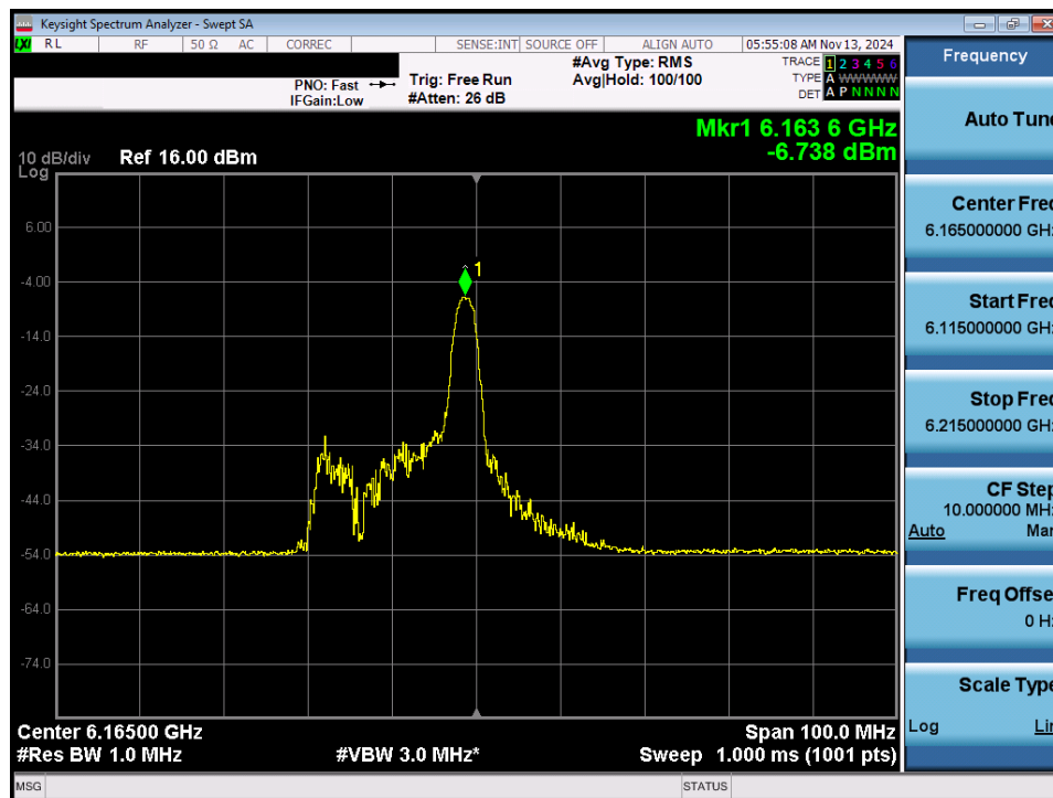
Plot 7-36. Power Spectral Density Plot MIMO ANT1 (40MHz 802.11ax/be (26 Tones) (UNII Band 5) – Ch. 43) - LPI
