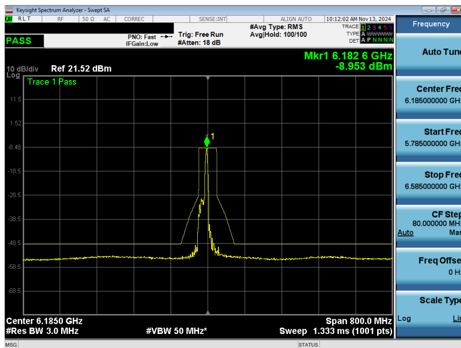
Plot 7-87. In Band Emissions Plot MIMO ANT2 (160MHz 802.11ax/be (26 Tones) (UNII Band 5) – Ch. 47) - LPI
