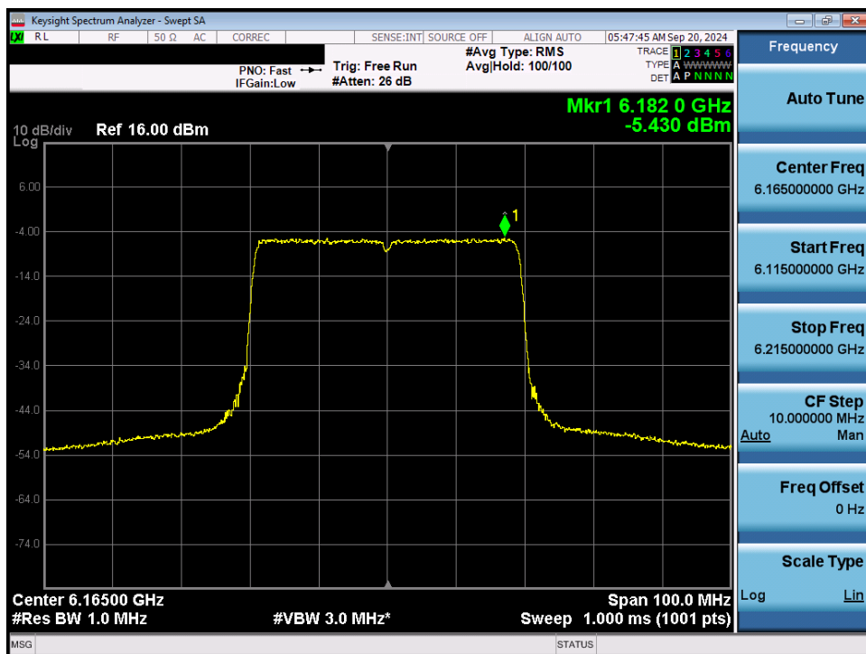
Plot 7-46. Power Spectral Density Plot MIMO ANT1 (40MHz 802.11ax/be (Full Tones) (UNII Band 5) – Ch. 43) - LPI
