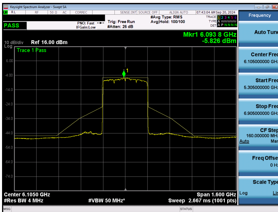
Plot 7-82. In Band Emissions Plot MIMO ANT1 (320MHz 802.11ax/be (Full Tones) (UNII Band 5) – Ch. 31) - LPI
