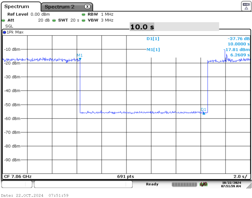
Plot 7-115. Contention Based Protocol Timing Plot (320MHz (UNII Band 8) – Ch. 191 High)
