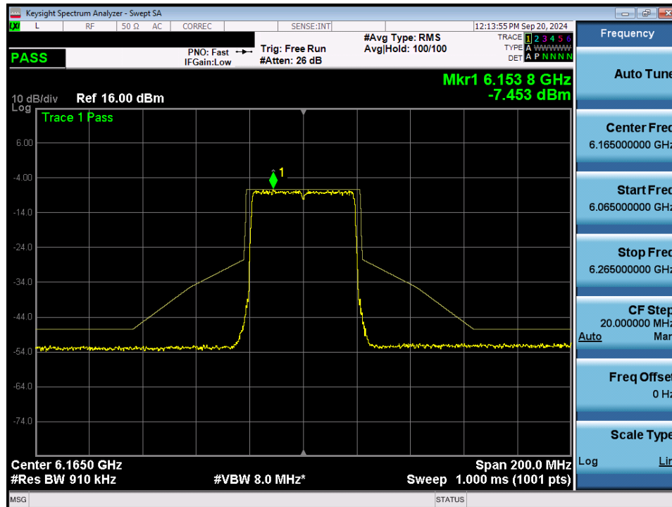
Plot 7-95. In Band Emissions Plot MIMO ANT2 (40MHz 802.11ax/be (Full Tones) (UNII Band 5) – Ch. 43) - LPI
