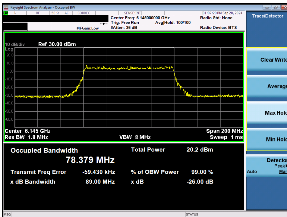
Plot 7-30. 26dB Bandwidth Plot MIMO ANT2 (80MHz 802.11ax/be (Full Tones) (UNII Band 5) – Ch. 39) - LPI
