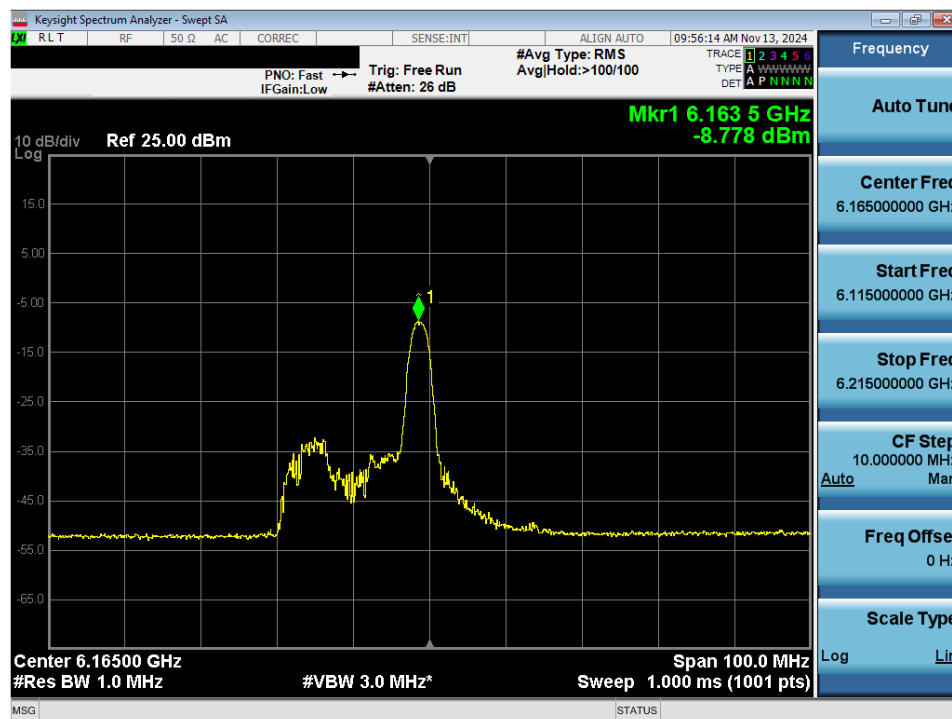
Plot 7-53. Power Spectral Density Plot MIMO ANT2 (40MHz 802.11ax/be (26 Tones) (UNII Band 5) – Ch. 43) - LPI
