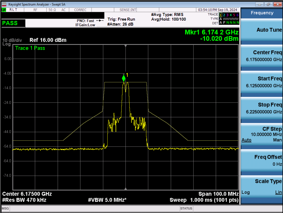
Plot 7-83. In Band Emissions Plot MIMO ANT2 (20MHz 802.11ax/be (26 Tones) (UNII Band 5) – Ch. 45) - LPI
