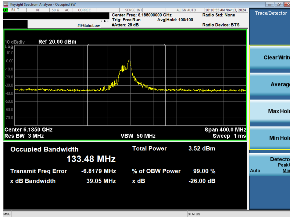
Plot 7-21. 26dB Bandwidth Plot MIMO ANT2 (160MHz 802.11ax/be (26 Tones) (UNII Band 5) – Ch. 47) - LPI
