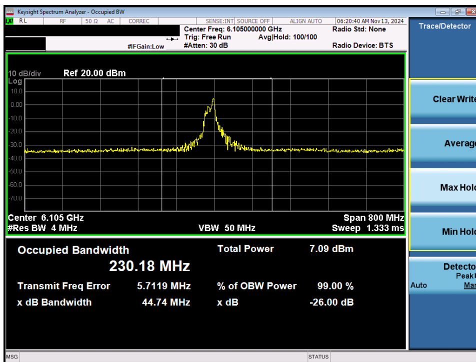
Plot 7-6. 26dB Bandwidth Plot MIMO ANT1 (320MHz 802.11ax/be (26 Tones) (UNII Band 5) – Ch. 31) - LPI
