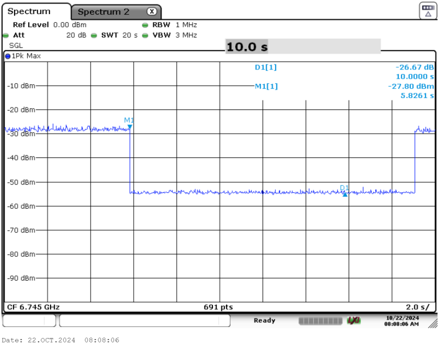
Plot 7-110. Contention Based Protocol Timing Plot (320MHz (UNII Band 7) – Ch. 159 Mid)
