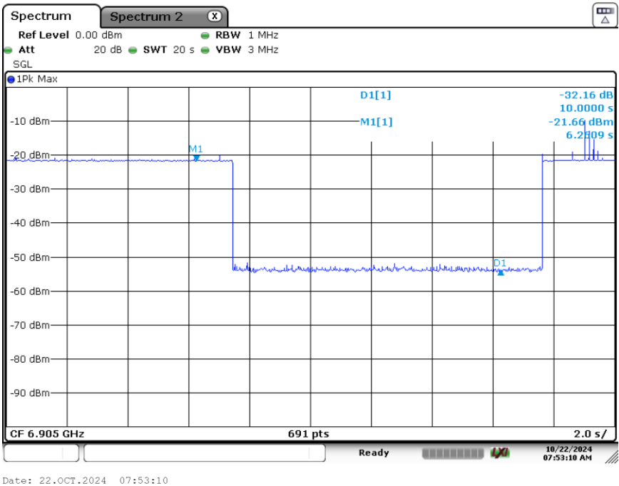
Plot 7-114. Contention Based Protocol Timing Plot (320MHz (UNII Band 8) – Ch. 191 Mid)
