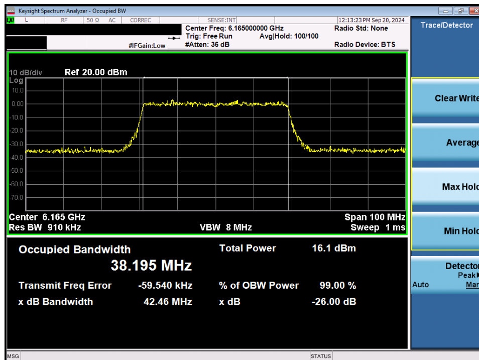
Plot 7-24. 26dB Bandwidth Plot MIMO ANT2 (40MHz 802.11ax/be (Full Tones) (UNII Band 5) – Ch. 43) - LPI
