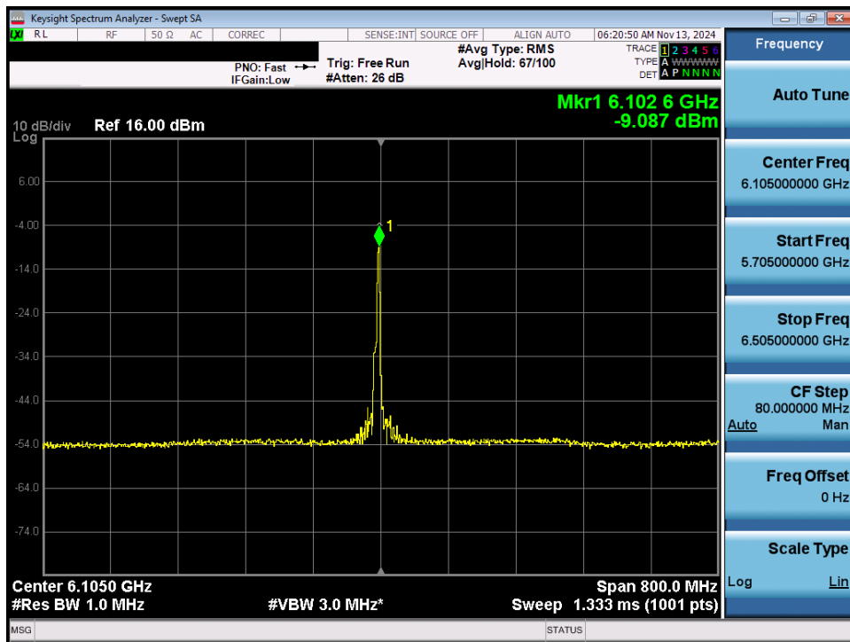
Plot 7-39. Power Spectral Density Plot MIMO ANT1 (320MHz 802.11ax/be (26 Tones) (UNII Band 5) – Ch. 31) – LPI
