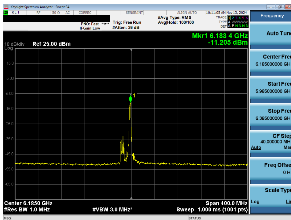
Plot 7-51. Power Spectral Density Plot MIMO ANT2 (160MHz 802.11ax/be (26 Tones) (UNII Band 5) – Ch. 47) - LPI
