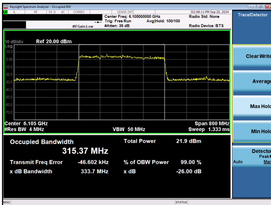
Plot 7-27. 26dB Bandwidth Plot MIMO ANT2 (320MHz 802.11ax/be (Full Tones) (UNII Band 5) – Ch. 31) - LPI
