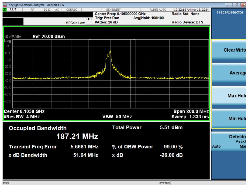
Plot 7-22. 26dB Bandwidth Plot MIMO ANT2 (320MHz 802.11ax/be (26 Tones) (UNII Band 5) – Ch. 31) - LPI
