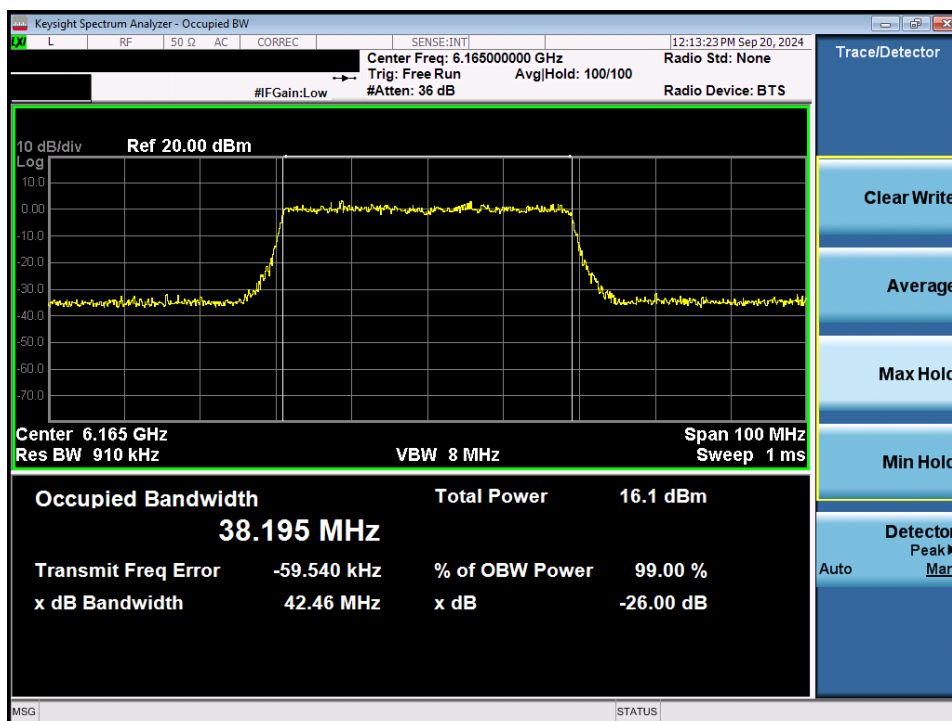
Plot 7-29. 26dB Bandwidth Plot MIMO ANT2 (40MHz 802.11ax/be (Full Tones) (UNII Band 5) – Ch. 43) - LPI
