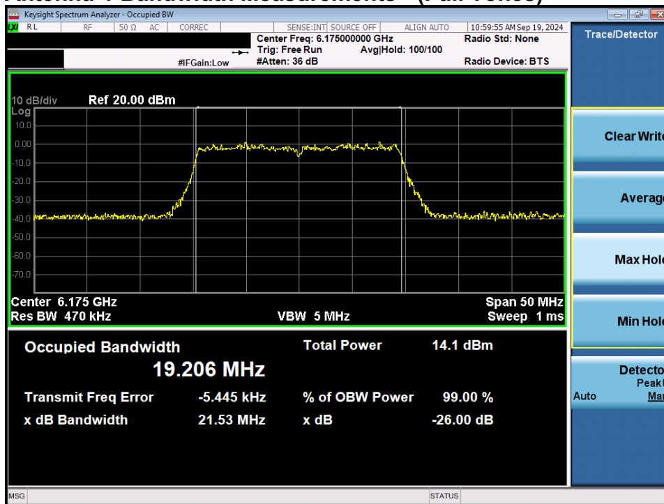
Plot 7-7. 26dB Bandwidth Plot MIMO ANT1 (20MHz 802.11ax/be (Full Tones) (UNII Band 5) – Ch. 45) - LPI
