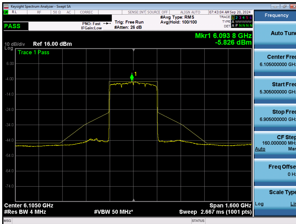
Plot 7-77. In Band Emissions Plot MIMO ANT1 (320MHz 802.11ax/be (Full Tones) (UNII Band 5) – Ch. 31) - LPI
