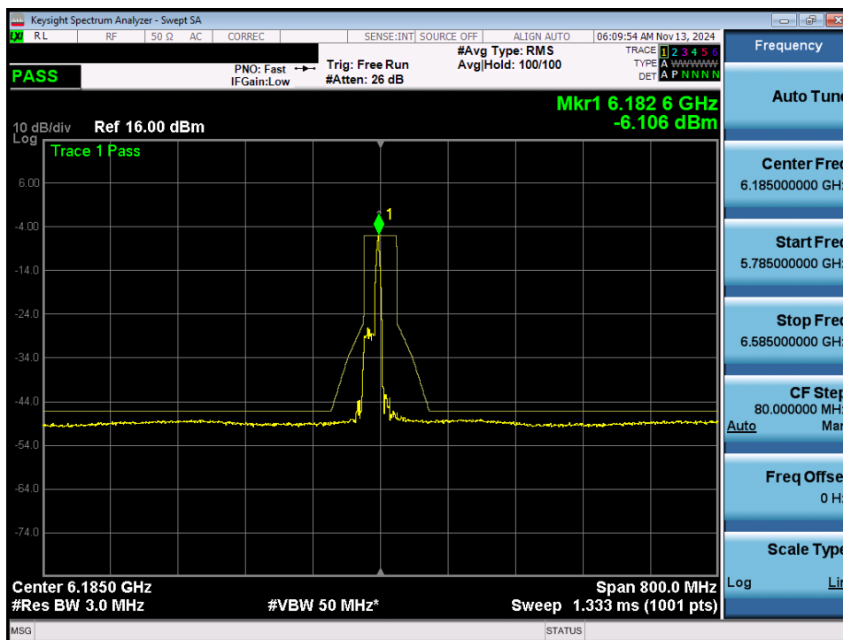
Plot 7-71. In Band Emissions Plot MIMO ANT1 (160MHz 802.11ax/be (26 Tones) (UNII Band 5) – Ch. 47) - LPI
