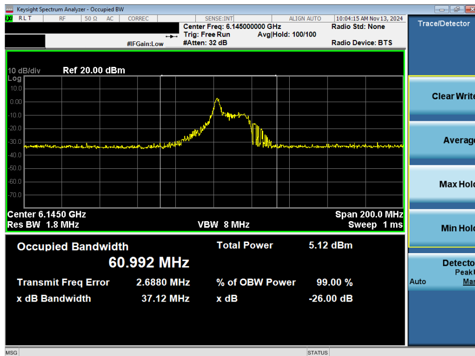
Plot 7-20. 26dB Bandwidth Plot MIMO ANT2 (80MHz 802.11ax/be (26 Tones) (UNII Band 5) – Ch. 39) - LPI
