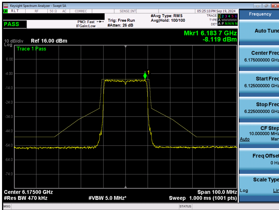
Plot 7-94. In Band Emissions Plot MIMO ANT2 (20MHz 802.11ax/be (Full Tones) (UNII Band 5) – Ch. 45) - LPI
