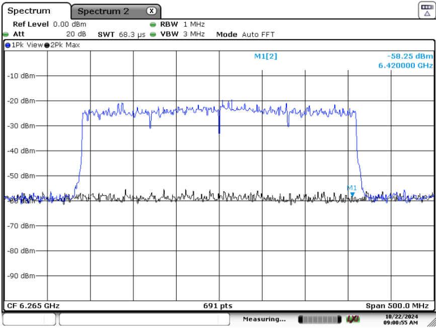
Plot 7-118. CBP 320MHz Channel - Injection Upper Edge – [6420 MHz]
