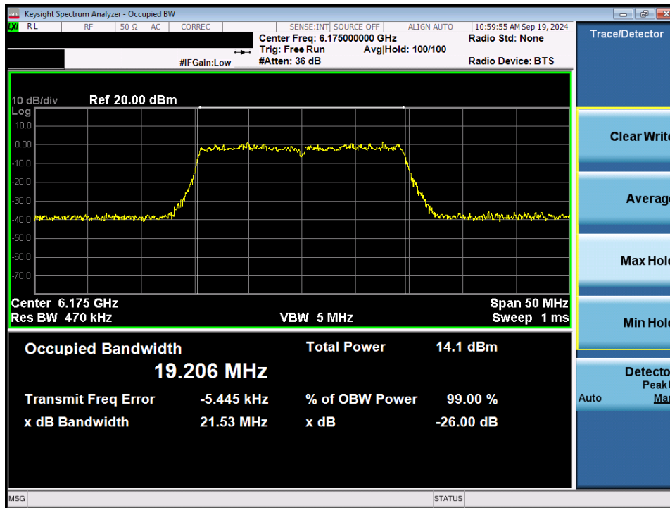
Plot 7-12. 26dB Bandwidth Plot MIMO ANT1 (20MHz 802.11ax/be (Full Tones) (UNII Band 5) – Ch. 45) - LPI
