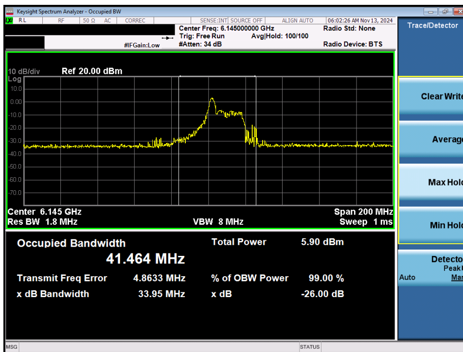
Plot 7-4. 26dB Bandwidth Plot MIMO ANT1 (80MHz 802.11ax/be (26 Tones) (UNII Band 5) – Ch. 39) - LPI
