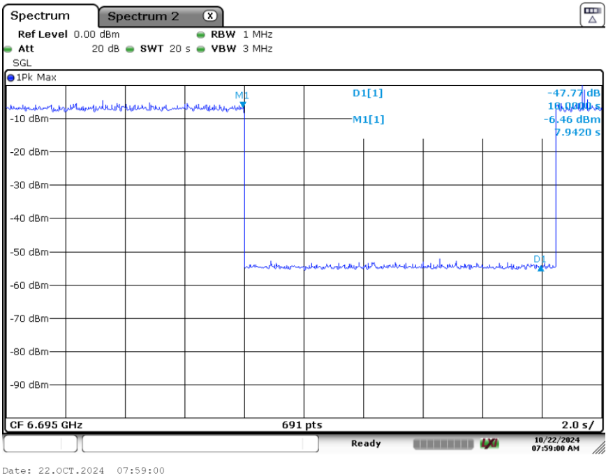
Plot 7-108. Contention Based Protocol Timing Plot (20MHz (UNII Band 7) – Ch. 149)
