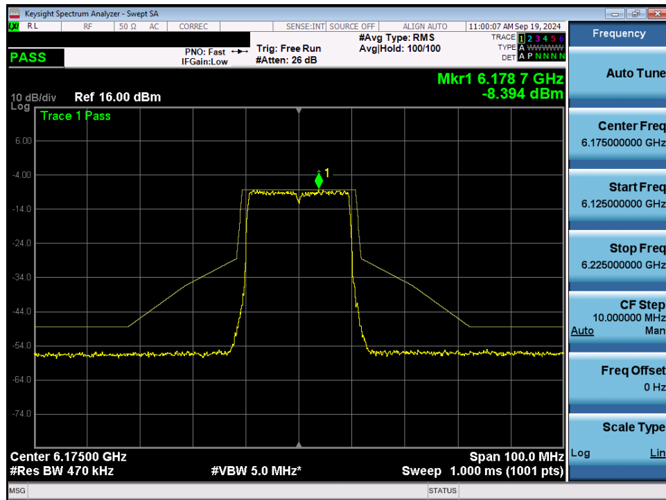
Plot 7-73. In Band Emissions Plot MIMO ANT1 (20MHz 802.11ax/be (Full Tones) (UNII Band 5) – Ch. 45) - LPI
