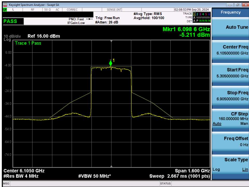
Plot 7-93. In Band Emissions Plot MIMO ANT2 (320MHz 802.11ax/be (Full Tones) (UNII Band 5) – Ch. 31) - LPI
