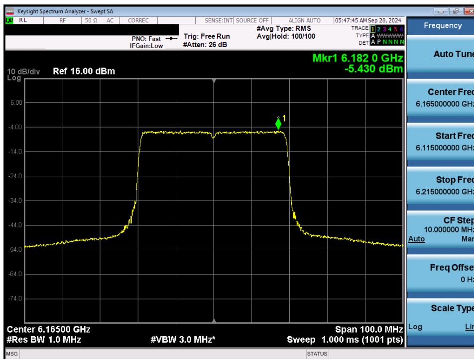
Plot 7-41. Power Spectral Density Plot MIMO ANT1 (40MHz 802.11ax/be (Full Tones) (UNII Band 5) – Ch. 43) - LPI
