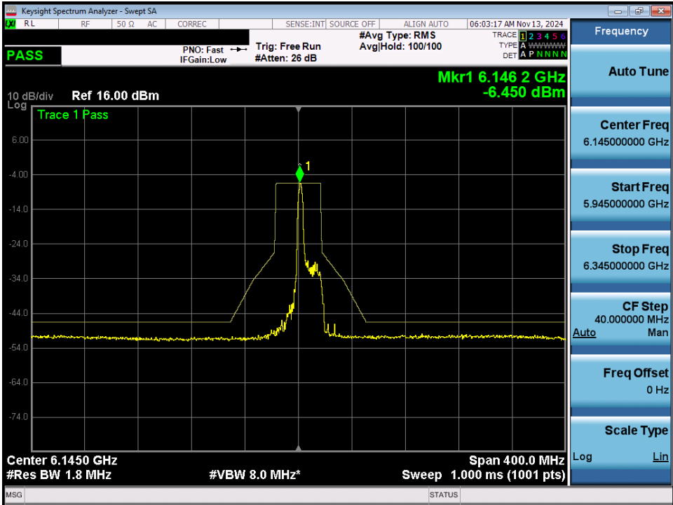
Plot 7-70. In Band Emissions Plot MIMO ANT1 (80MHz 802.11ax/be (26 Tones) (UNII Band 5) – Ch. 39) - LPI
