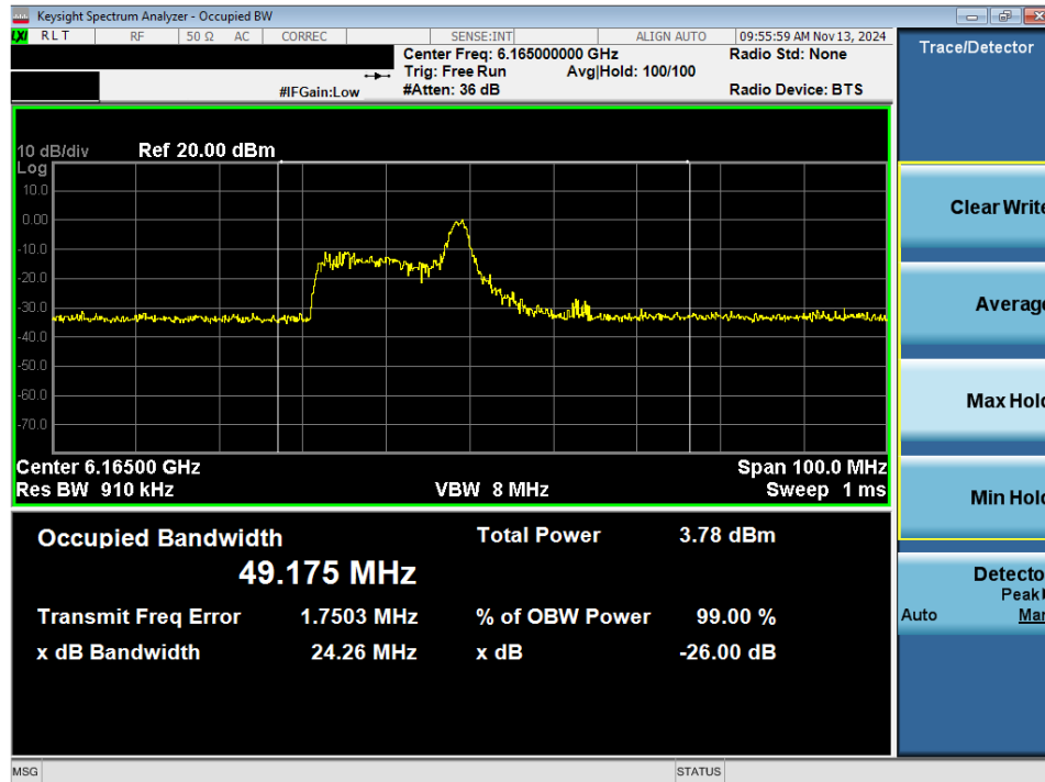
Plot 7-19. 26dB Bandwidth Plot MIMO ANT2 (40MHz 802.11ax/be (26 Tones) (UNII Band 5) – Ch. 43) - LPI
