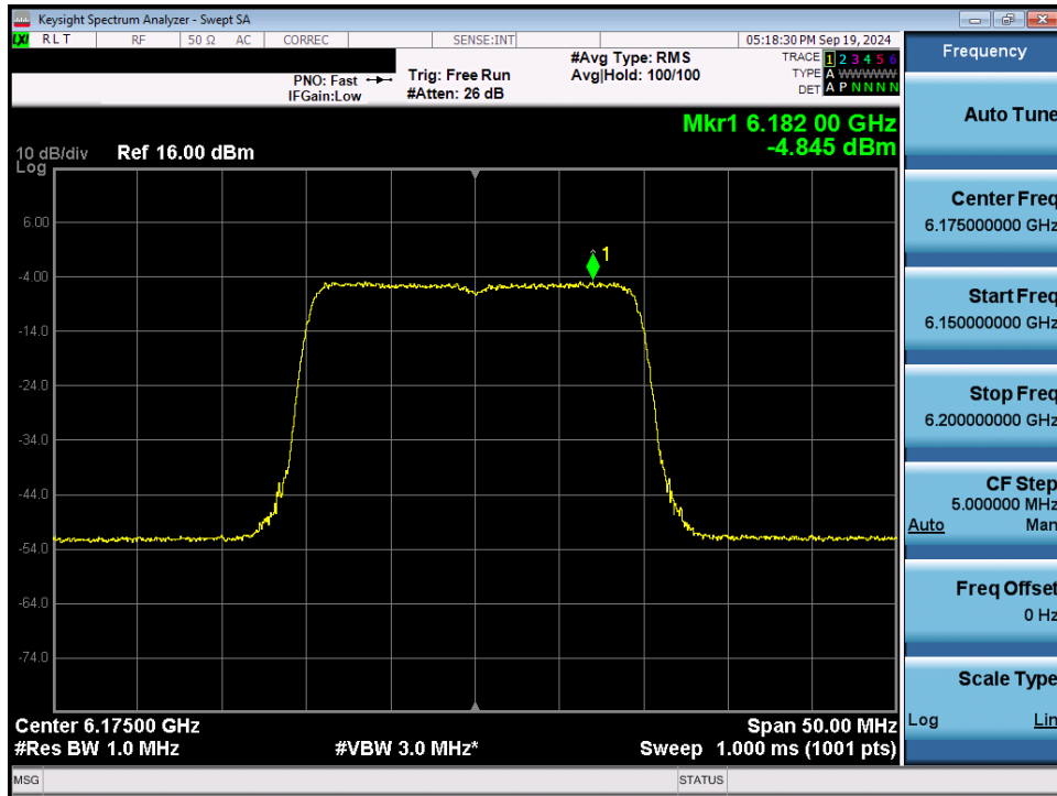
Plot 7-62. Power Spectral Density Plot MIMO ANT2 (20MHz 802.11ax/be (Full Tones) (UNII Band 5) – Ch. 45) - LPI
