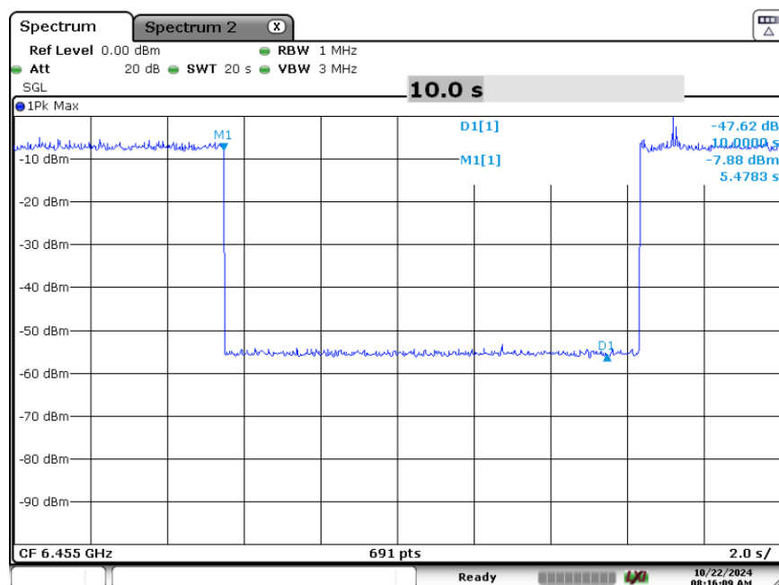
Plot 7-104. Contention Based Protocol Timing Plot (20MHz (UNII Band 6) – Ch. 101)
