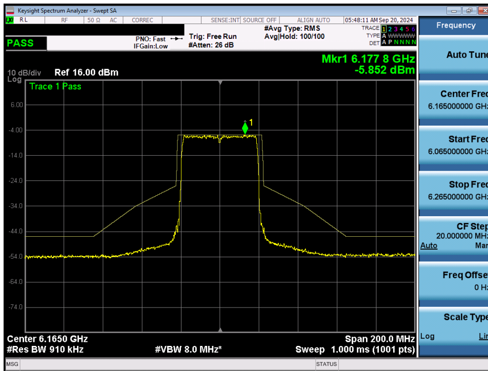
Plot 7-79. In Band Emissions Plot MIMO ANT1 (40MHz 802.11ax/be (Full Tones) (UNII Band 5) – Ch. 43) - LPI
