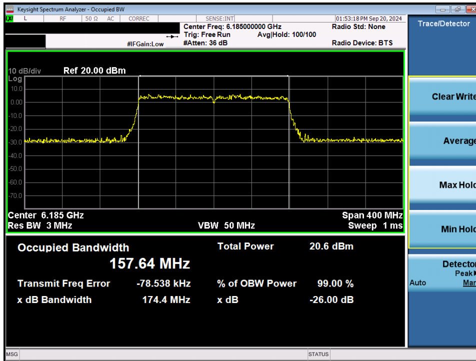
Plot 7-31. 26dB Bandwidth Plot MIMO ANT2 (160MHz 802.11ax/be (Full Tones) (UNII Band 5) – Ch. 47) - LPI
