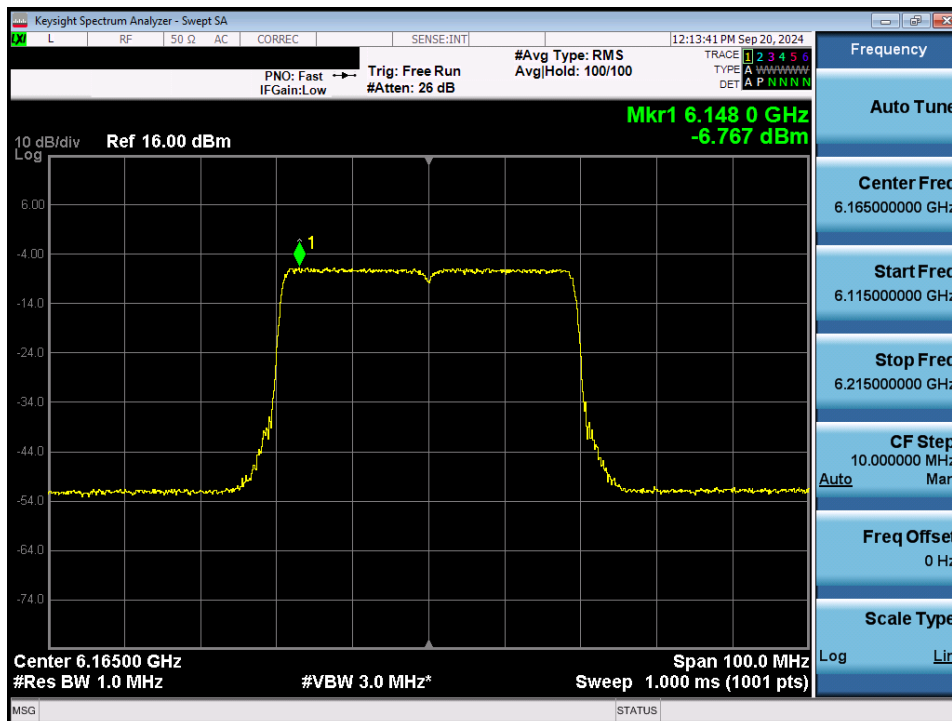
Plot 7-58. Power Spectral Density Plot MIMO ANT2 (40MHz 802.11ax/be (Full Tones) (UNII Band 5) – Ch. 43) - LPI
