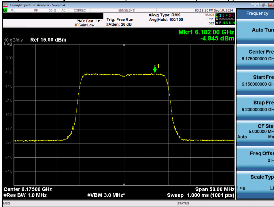
Plot 7-57. Power Spectral Density Plot MIMO ANT2 (20MHz 802.11ax/be (Full Tones) (UNII Band 5) – Ch. 45) - LPI
