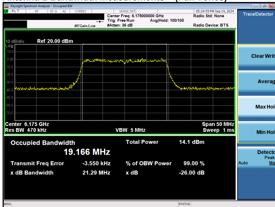
Plot 7-23. 26dB Bandwidth Plot MIMO ANT2 (20MHz 802.11ax/be (Full Tones) (UNII Band 5) – Ch. 45) - LPI
