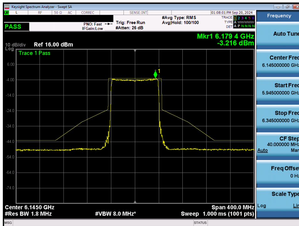
Plot 7-96. In Band Emissions Plot MIMO ANT2 (80MHz 802.11ax/be (Full Tones) (UNII Band 5) – Ch. 39) - LPI
