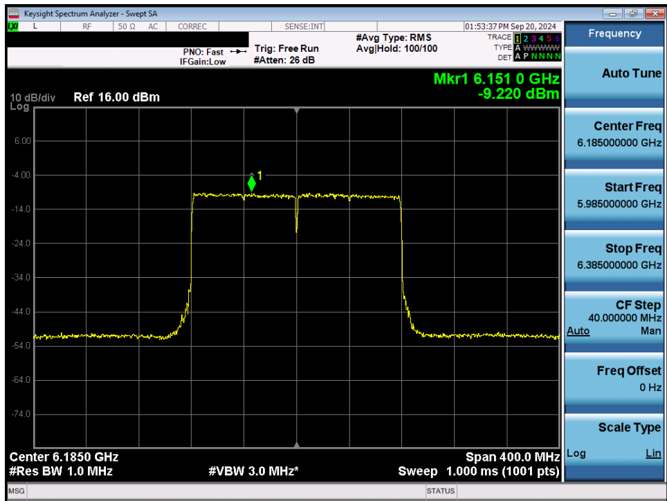
Plot 7-65. Power Spectral Density Plot MIMO ANT2 (160MHz 802.11ax/be (Full Tones) (UNII Band 5) – Ch. 47) - LPI
