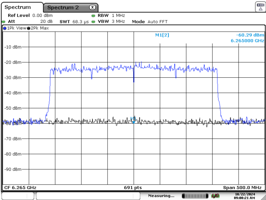
Plot 7-117. CBP 320MHz Channel - Injection Center – [6265 MHz]
