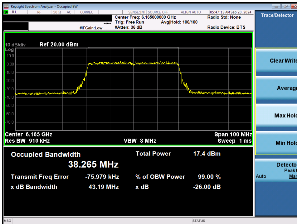
Plot 7-13. 26dB Bandwidth Plot MIMO ANT1 (40MHz 802.11ax/be (Full Tones) (UNII Band 5) – Ch. 43) - LPI
