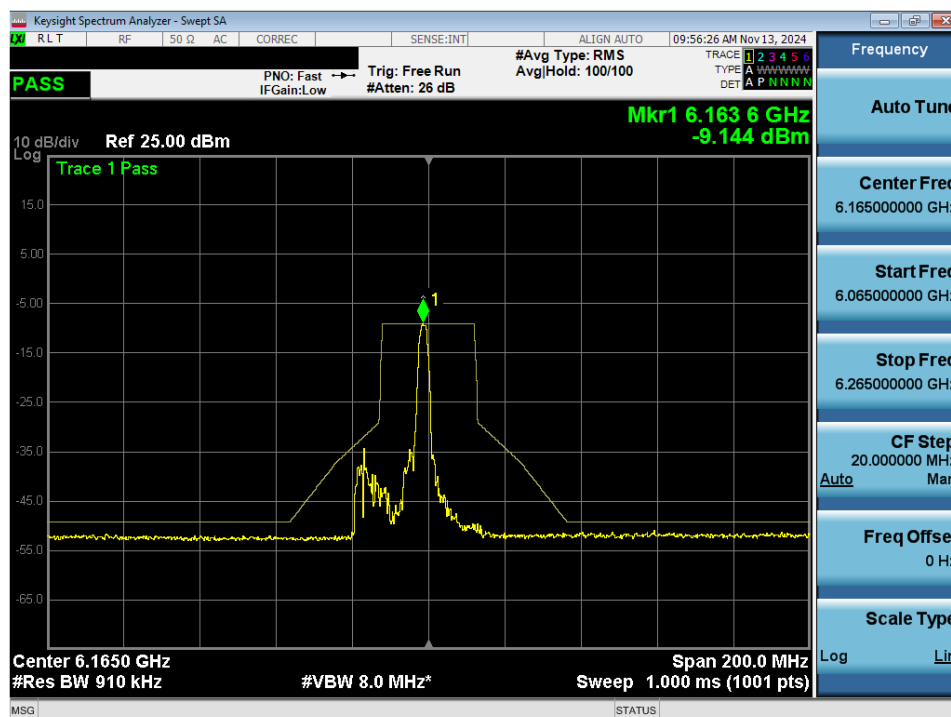
Plot 7-85. In Band Emissions Plot MIMO ANT2 (40MHz 802.11ax/be (26 Tones) (UNII Band 5) – Ch. 43) - LPI
