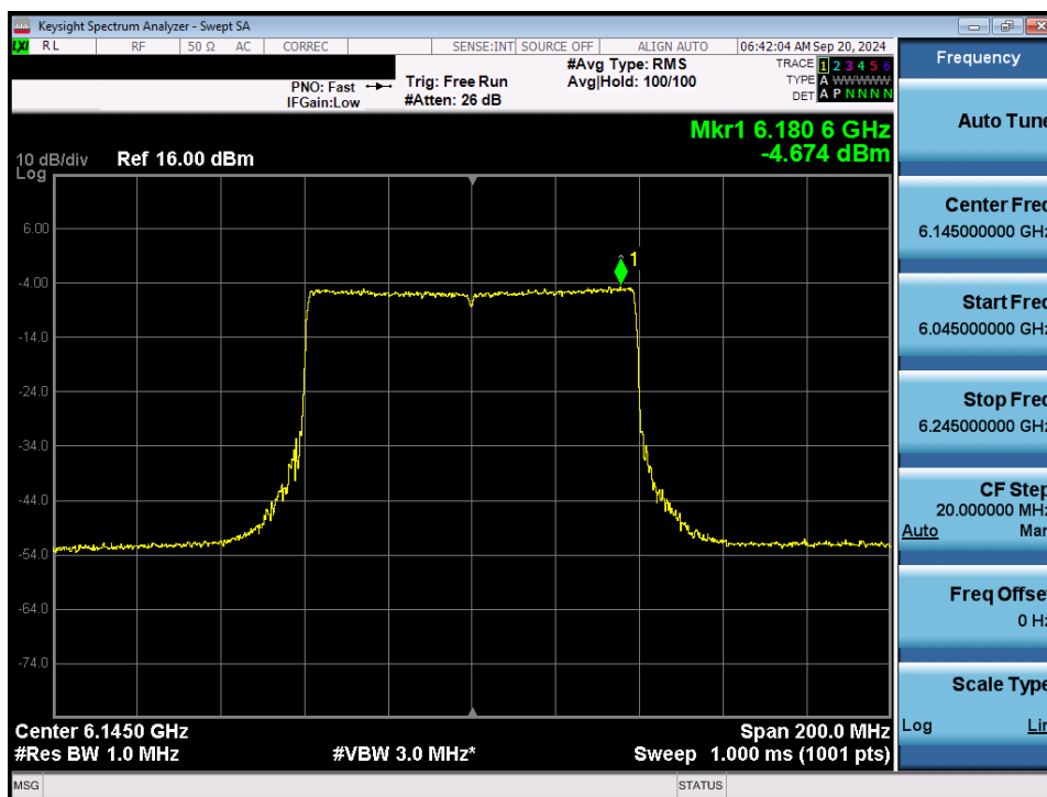
Plot 7-42. Power Spectral Density Plot MIMO ANT1 (80MHz 802.11ax/be (Full Tones) (UNII Band 5) – Ch. 39) - LPI
