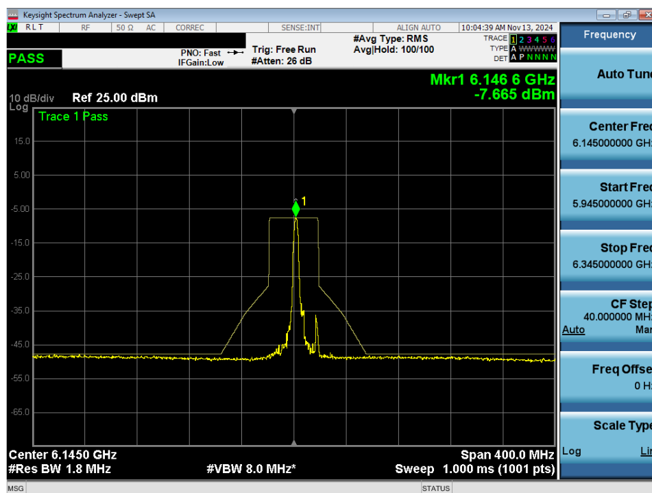
Plot 7-86. In Band Emissions Plot MIMO ANT2 (80MHz 802.11ax/be (26 Tones) (UNII Band 5) – Ch. 39) - LPI
