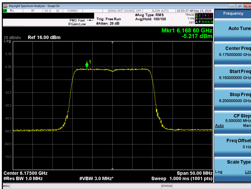
Plot 7-40. Power Spectral Density Plot MIMO ANT1 (20MHz 802.11ax/be (Full Tones) (UNII Band 5) – Ch. 45) - LPI
