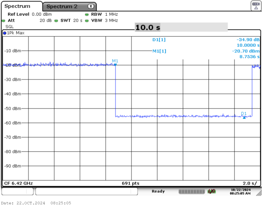
Plot 7-103. Contention Based Protocol Timing Plot (320MHz (UNII Band 5) – Ch. 31 High)
