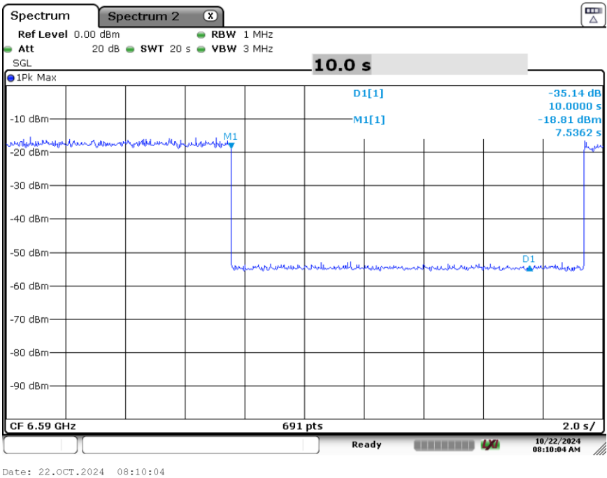
Plot 7-109. Contention Based Protocol Timing Plot (320MHz (UNII Band 7) – Ch. 159 Low)
