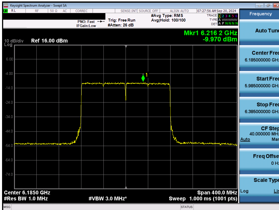
Plot 7-43. Power Spectral Density Plot MIMO ANT1 (160MHz 802.11ax/be (Full Tones) (UNII Band 5) – Ch. 47) - LPI
