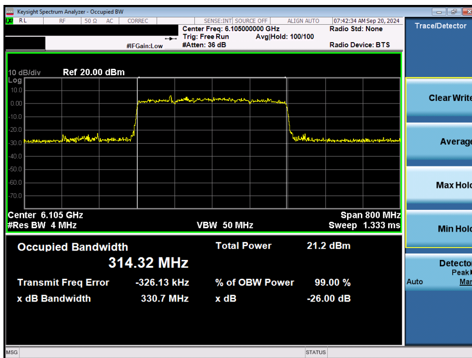
Plot 7-16. 26dB Bandwidth Plot MIMO ANT1 (320MHz 802.11ax/be (Full Tones) (UNII Band 5) – Ch. 31) - LPI
