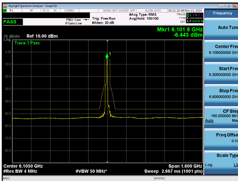
Plot 7-72. In Band Emissions Plot MIMO ANT1 (320MHz 802.11ax/be (26 Tones) (UNII Band 5) – Ch. 31) - LPI
