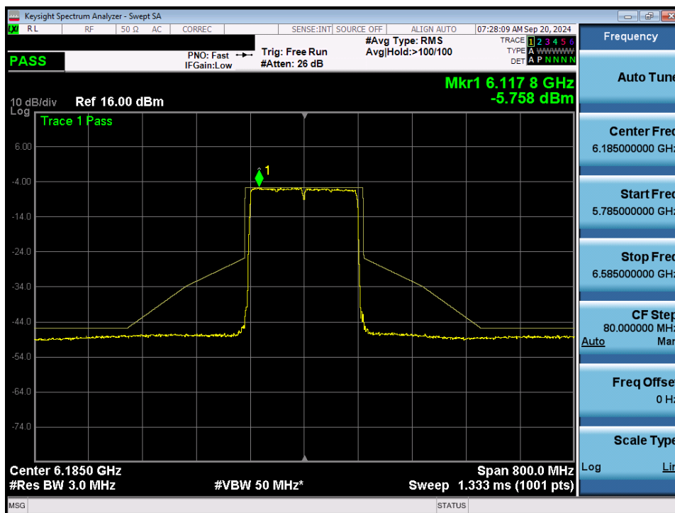
Plot 7-81. In Band Emissions Plot MIMO ANT1 (160MHz 802.11ax/be (Full Tones) (UNII Band 5) – Ch. 47) - LPI
