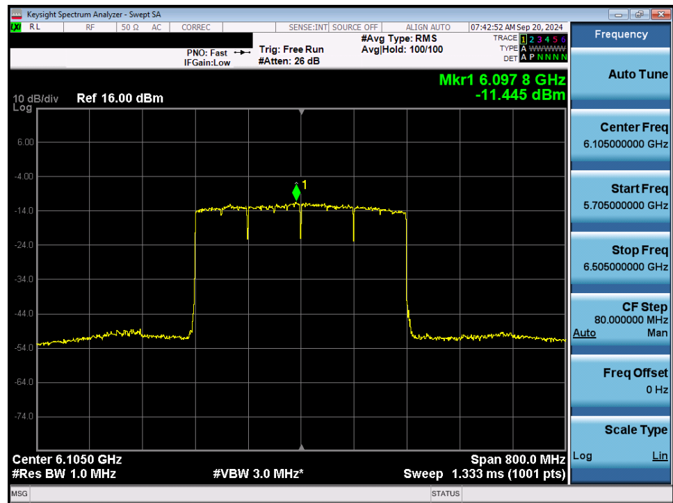
Plot 7-49. Power Spectral Density Plot MIMO ANT1 (320MHz 802.11ax/be (Full Tones) (UNII Band 5) – Ch. 31) - LPI
