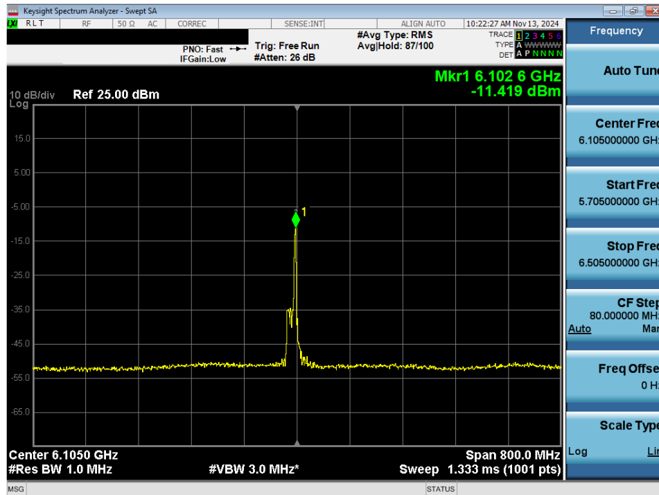
Plot 7-56. Power Spectral Density Plot MIMO ANT2 (320MHz 802.11ax/be (26 Tones) (UNII Band 5) – Ch. 31) - LPI
