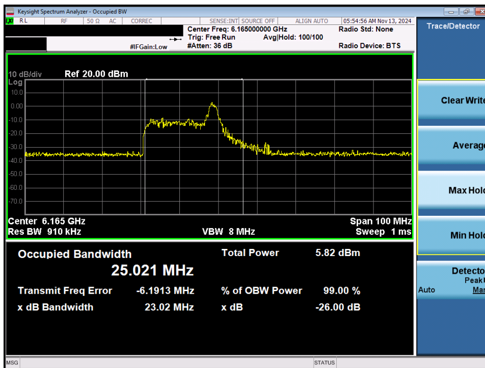
Plot 7-3. 26dB Bandwidth Plot MIMO ANT1 (40MHz 802.11ax/be (26 Tones) (UNII Band 5) – Ch. 43) - LPI
