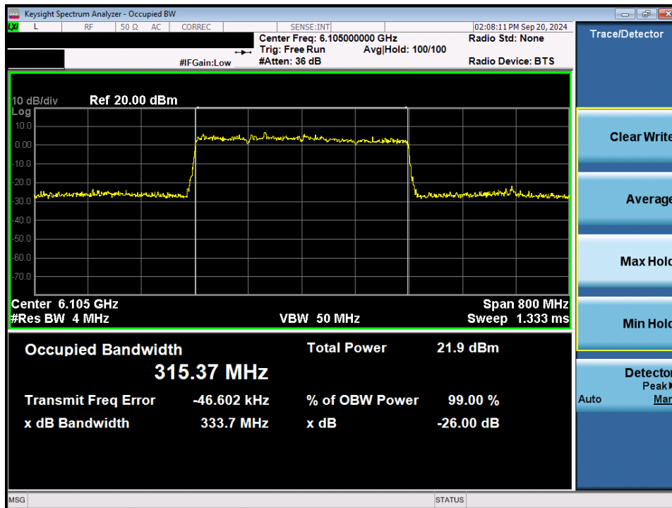
Plot 7-32. 26dB Bandwidth Plot MIMO ANT2 (320MHz 802.11ax/be (Full Tones) (UNII Band 5) – Ch. 31) - LPI
