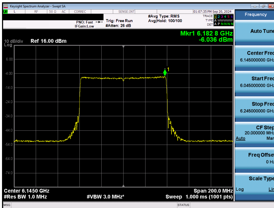
Plot 7-59. Power Spectral Density Plot MIMO ANT2 (80MHz 802.11ax/be (Full Tones) (UNII Band 5) – Ch. 39) - LPI
