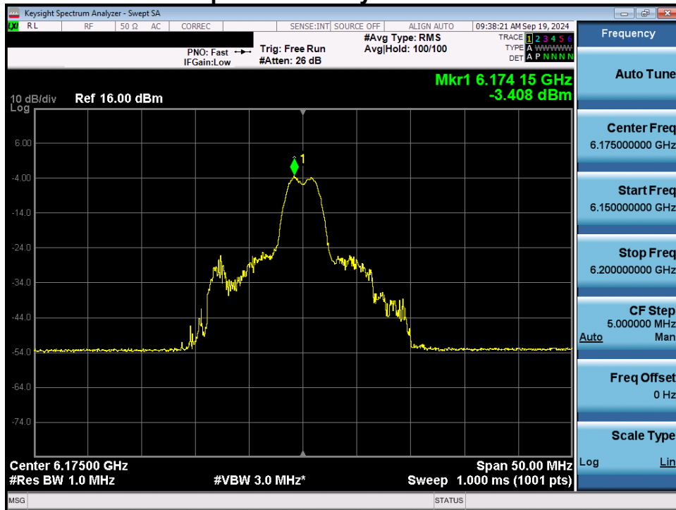
Plot 7-33. Power Spectral Density Plot MIMO ANT1 (20MHz 802.11ax/be (26 Tones) (UNII Band 5) – Ch. 45) - LPI
