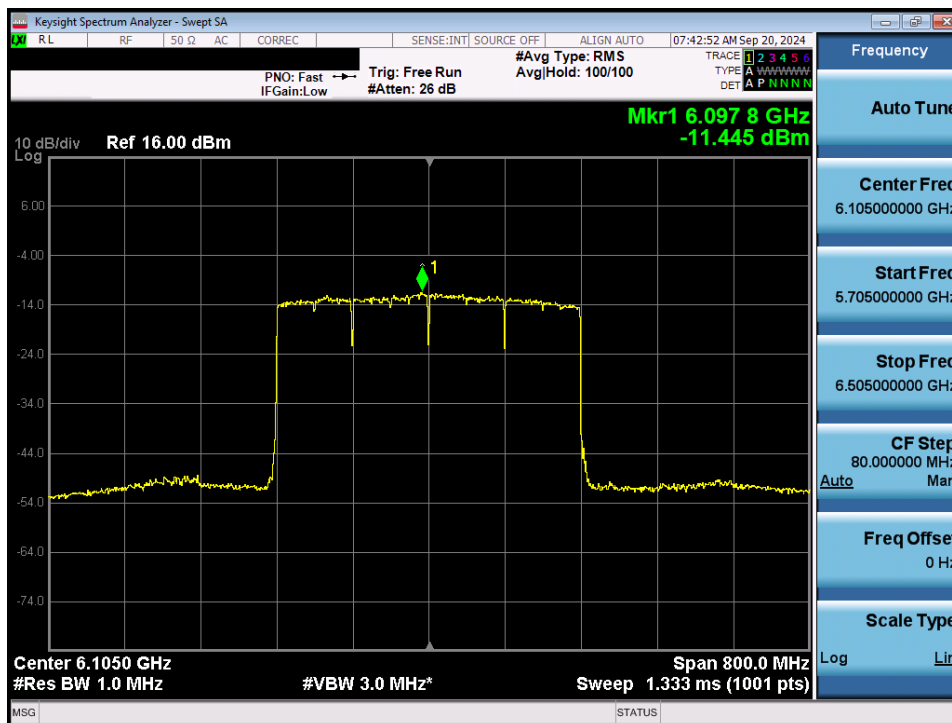
Plot 7-44. Power Spectral Density Plot MIMO ANT1 (320MHz 802.11ax/be (Full Tones) (UNII Band 5) – Ch. 31) - LPI
