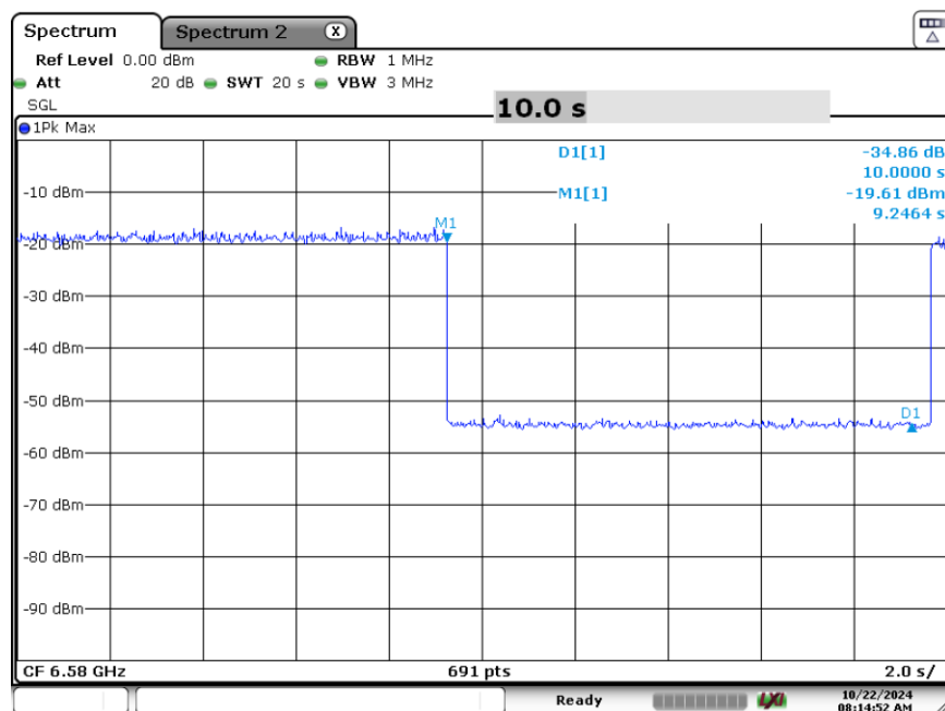
Plot 7-106. Contention Based Protocol Timing Plot (320MHz (UNII Band 6) – Ch. 95 Mid)
