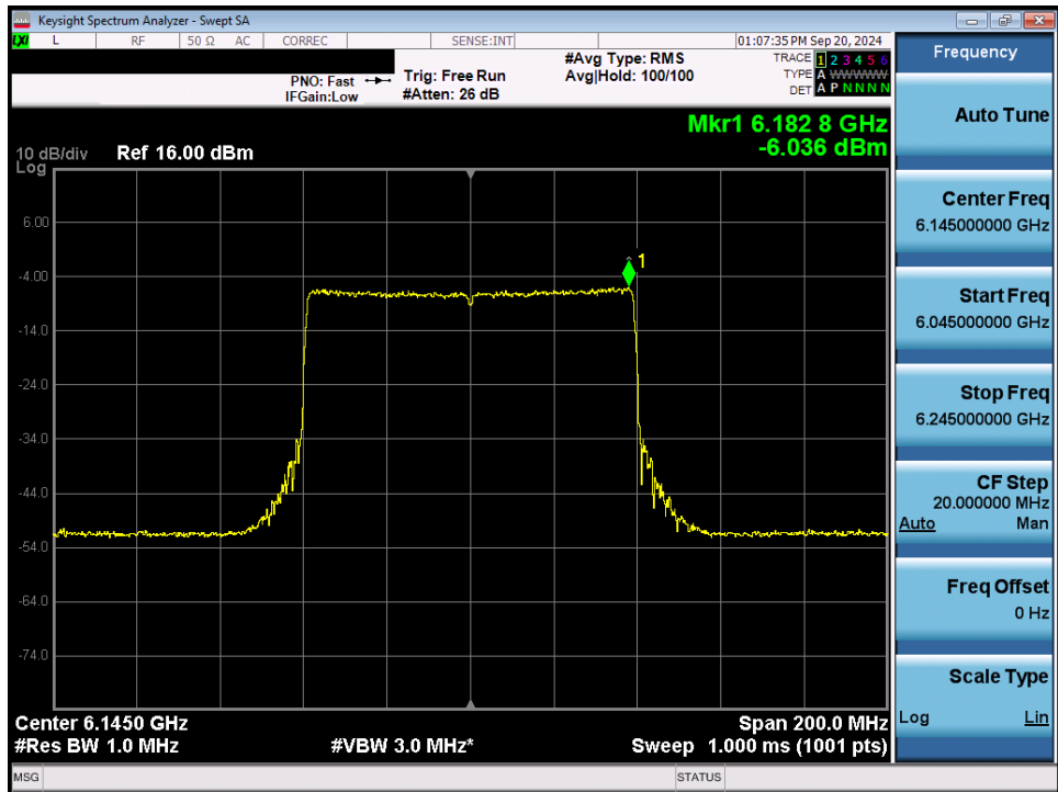
Plot 7-64. Power Spectral Density Plot MIMO ANT2 (80MHz 802.11ax/be (Full Tones) (UNII Band 5) – Ch. 39) - LPI
