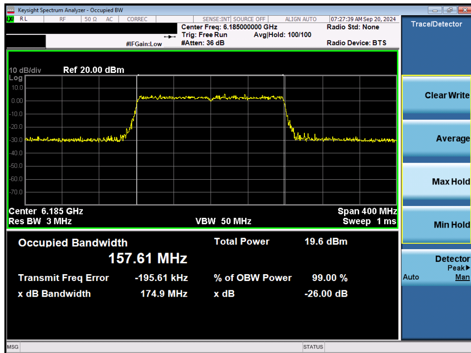
Plot 7-15. 26dB Bandwidth Plot MIMO ANT1 (160MHz 802.11ax/be (Full Tones) (UNII Band 5) – Ch. 47) - LPI
