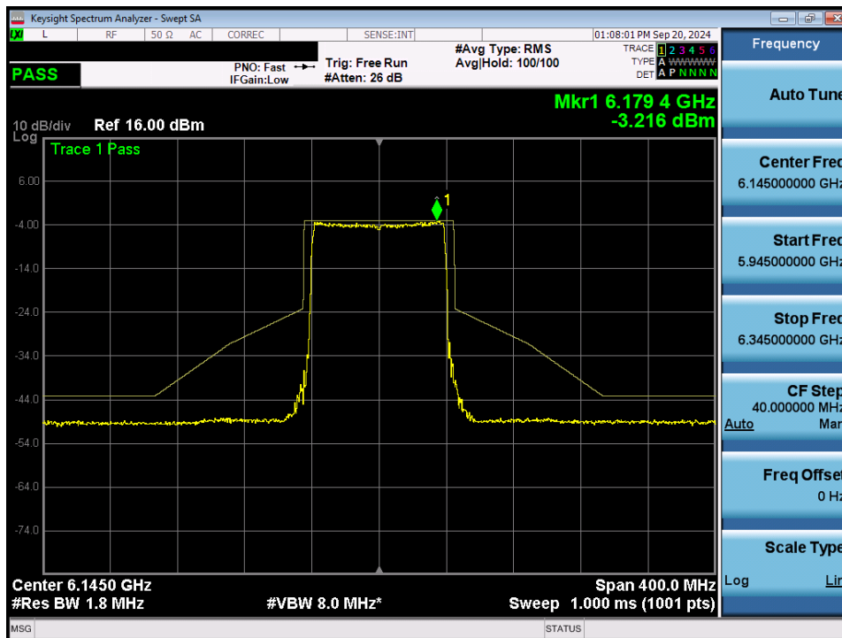
Plot 7-91. In Band Emissions Plot MIMO ANT2 (80MHz 802.11ax/be (Full Tones) (UNII Band 5) – Ch. 39) - LPI
