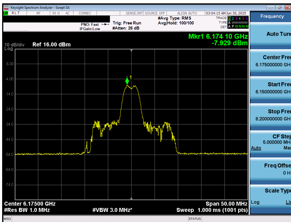
Plot 7-50. Power Spectral Density Plot MIMO ANT2 (20MHz 802.11ax/be (26 Tones) (UNII Band 5) – Ch. 45) - LPI
