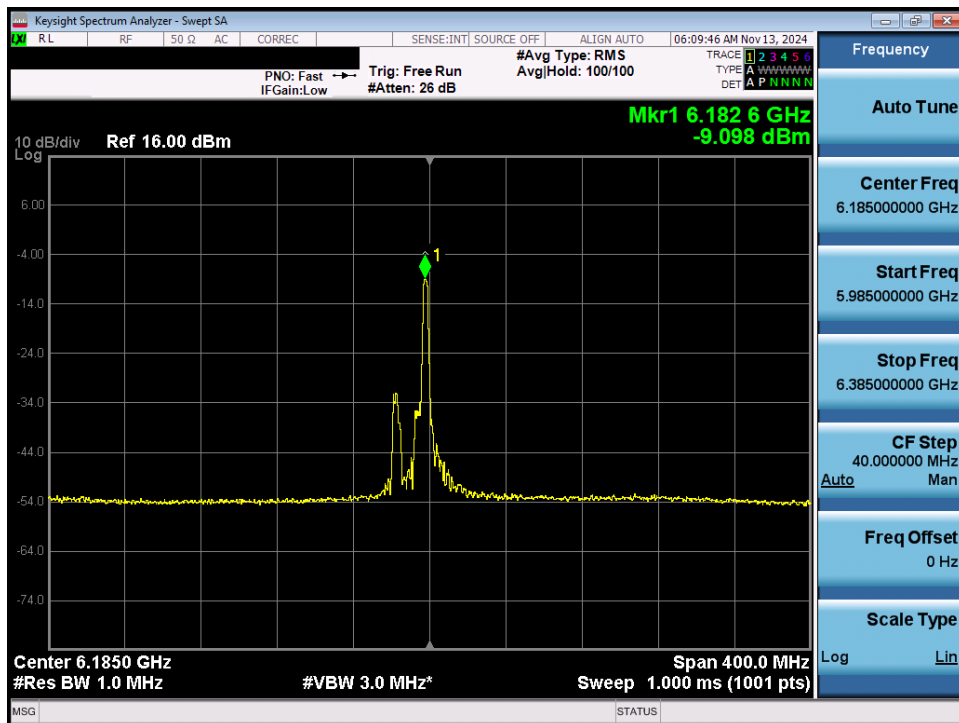
Plot 7-34. Power Spectral Density Plot MIMO ANT1 (160MHz 802.11ax/be (26 Tones) (UNII Band 5) – Ch. 47) - LPI
