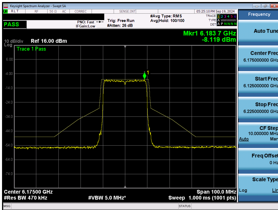
Plot 7-89. In Band Emissions Plot MIMO ANT2 (20MHz 802.11ax/be (Full Tones) (UNII Band 5) – Ch. 45) - LPI
