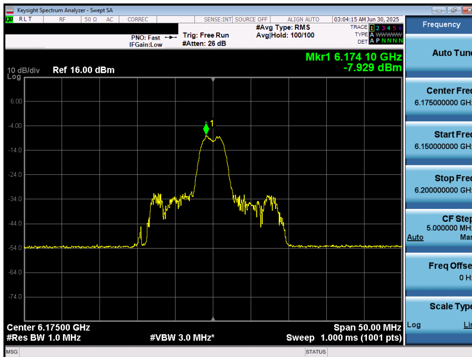
Plot 7-52. Power Spectral Density Plot MIMO ANT2 (20MHz 802.11ax/be (26 Tones) (UNII Band 5) – Ch. 45) - LPI
