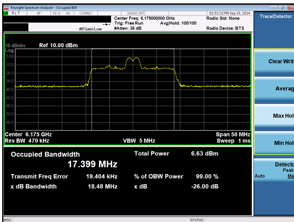
Plot 7-18. 26dB Bandwidth Plot MIMO ANT2 (20MHz 802.11ax/be (26 Tones) (UNII Band 5) – Ch. 45) - LPI
