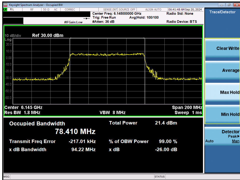
Plot 7-14. 26dB Bandwidth Plot MIMO ANT1 (80MHz 802.11ax/be (Full Tones) (UNII Band 5) – Ch. 39) - LPI
