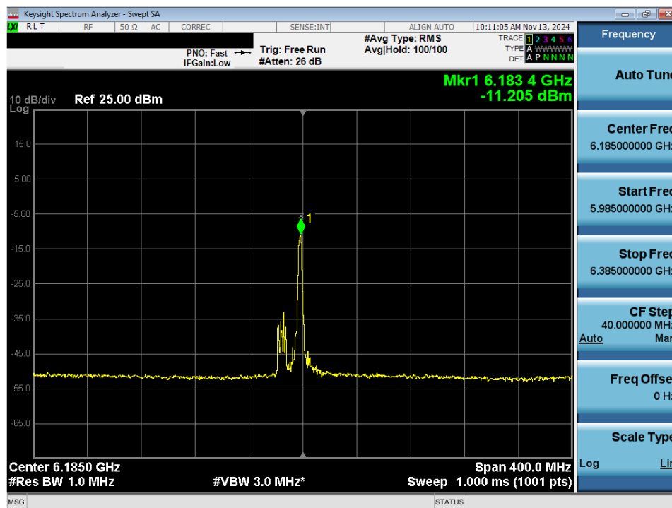
Plot 7-55. Power Spectral Density Plot MIMO ANT2 (160MHz 802.11ax/be (26 Tones) (UNII Band 5) – Ch. 47) - LPI
