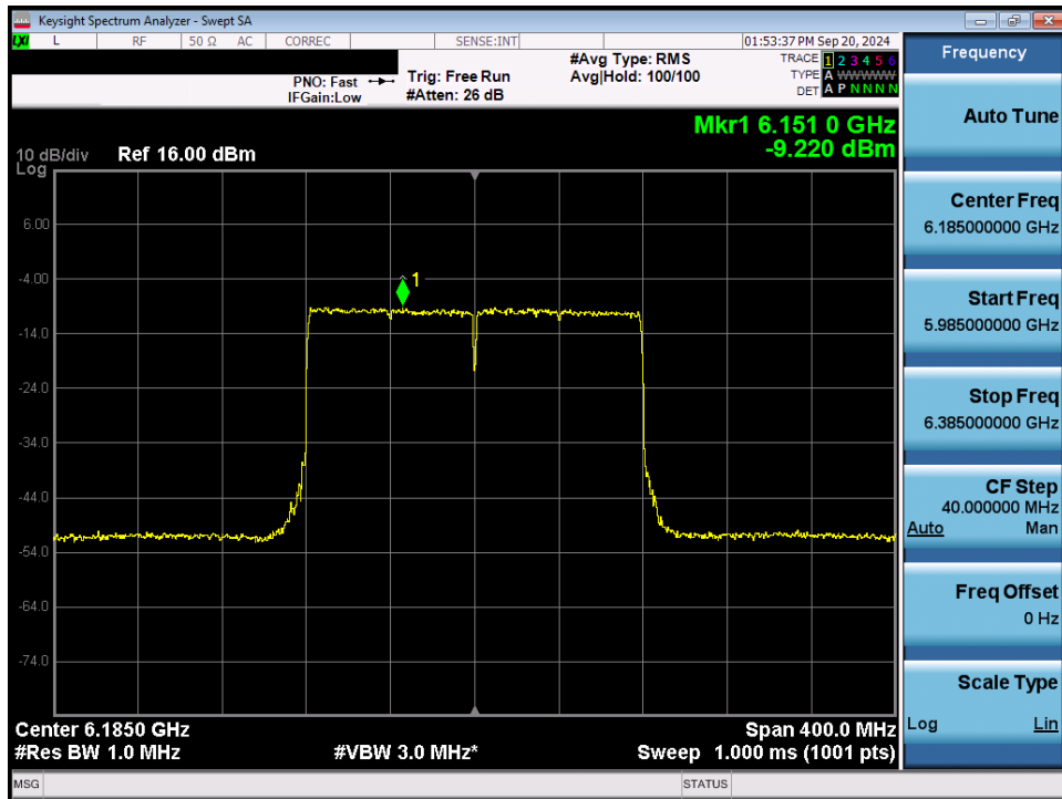
Plot 7-60. Power Spectral Density Plot MIMO ANT2 (160MHz 802.11ax/be (Full Tones) (UNII Band 5) – Ch. 47) - LPI
