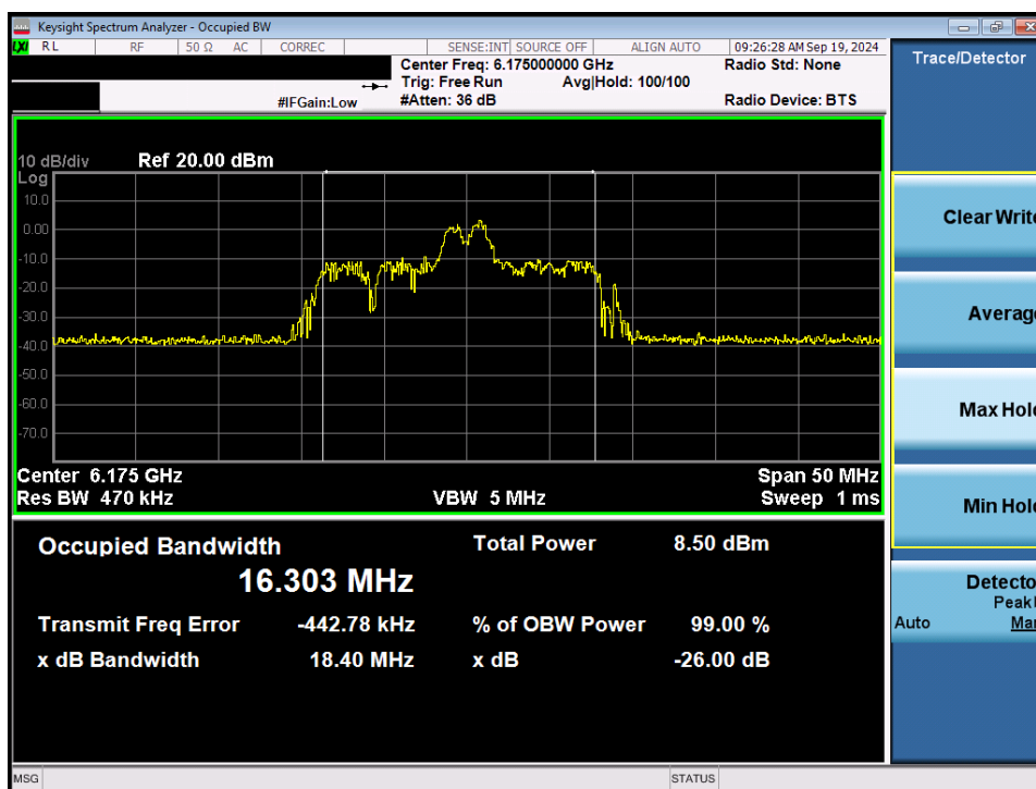
Plot 7-2. 26dB Bandwidth Plot MIMO ANT1 (20MHz 802.11ax/be (26 Tones) (UNII Band 5) – Ch. 45) - LPI
