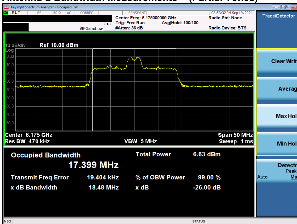
Plot 7-17. 26dB Bandwidth Plot MIMO ANT2 (20MHz 802.11ax/be (26 Tones) (UNII Band 5) – Ch. 45) - LPI
