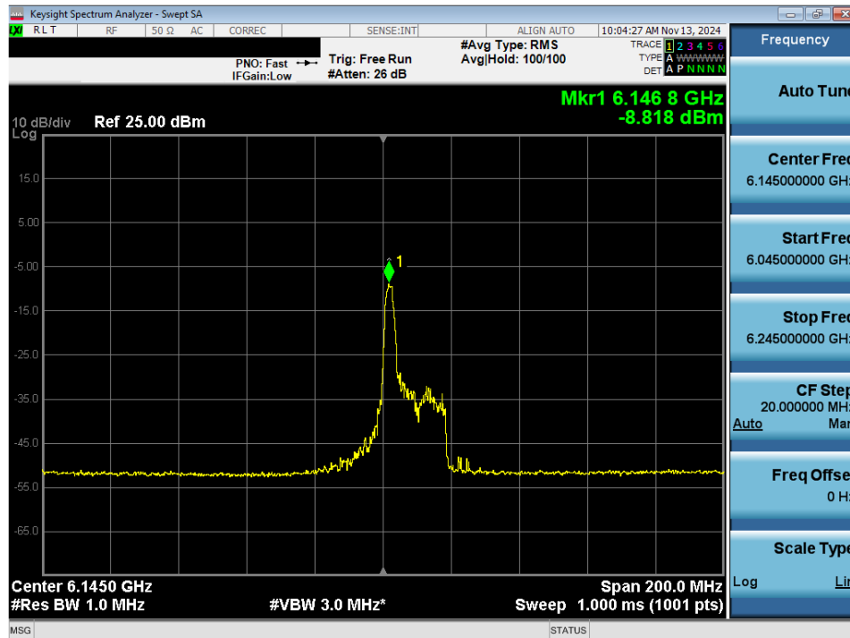
Plot 7-54. Power Spectral Density Plot MIMO ANT2 (80MHz 802.11ax/be (26 Tones) (UNII Band 5) – Ch. 39) - LPI
