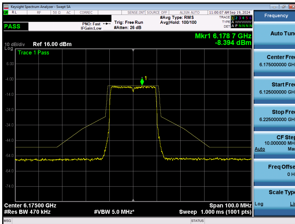
Plot 7-78. In Band Emissions Plot MIMO ANT1 (20MHz 802.11ax/be (Full Tones) (UNII Band 5) – Ch. 45) - LPI
