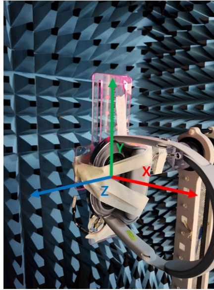
Figure 1: Geometry for SM-I610 for Radiation patterns.
