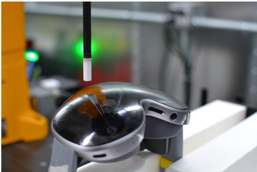
PD Test Setup Photo 8 – PD, Front Side at 8.58mm
