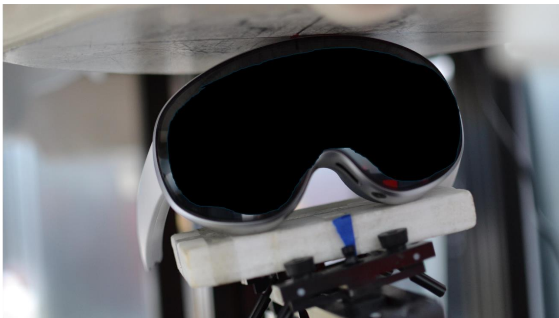
SAR Test Setup Photo 3 – Extremity, Top Edge WIFI/BT Antenna 2
