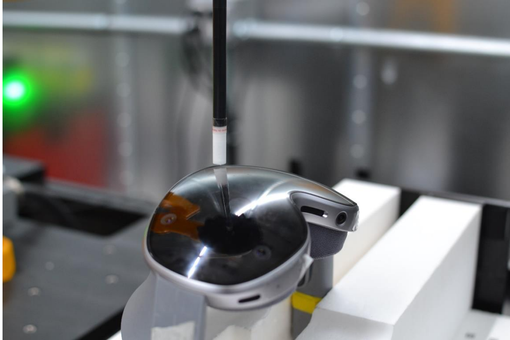
PD Test Setup Photo 7 – PD, Ant 2 Front Side at 2mm
