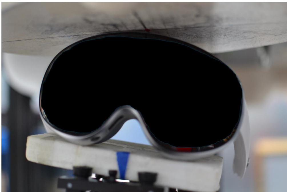
SAR Test Setup Photo 2 – Extremity, Top Edge, WIFI/BT Antenna 1
