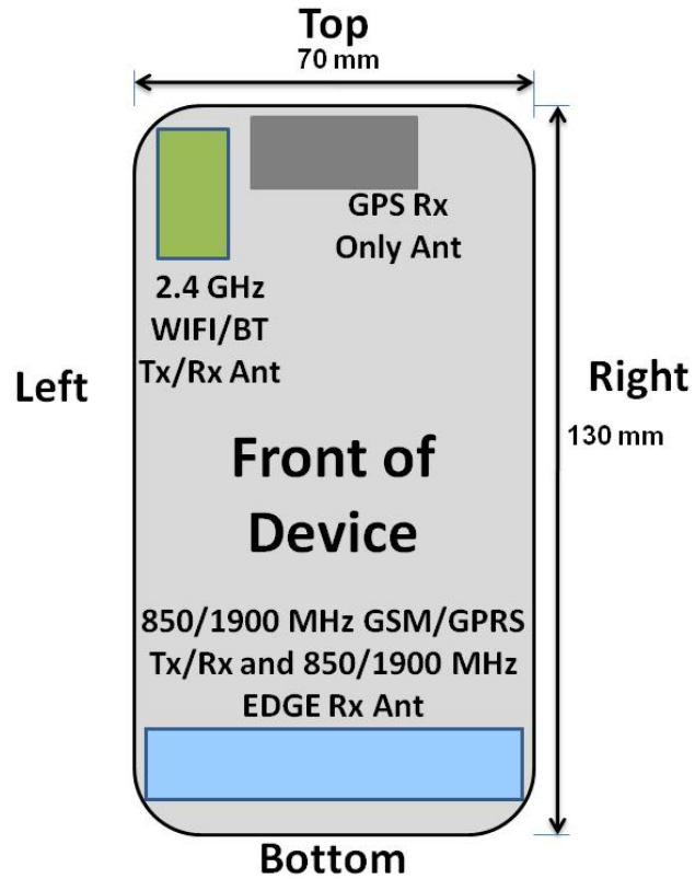
SAR Test Setup Photo 11: DUT Antenna Locations
