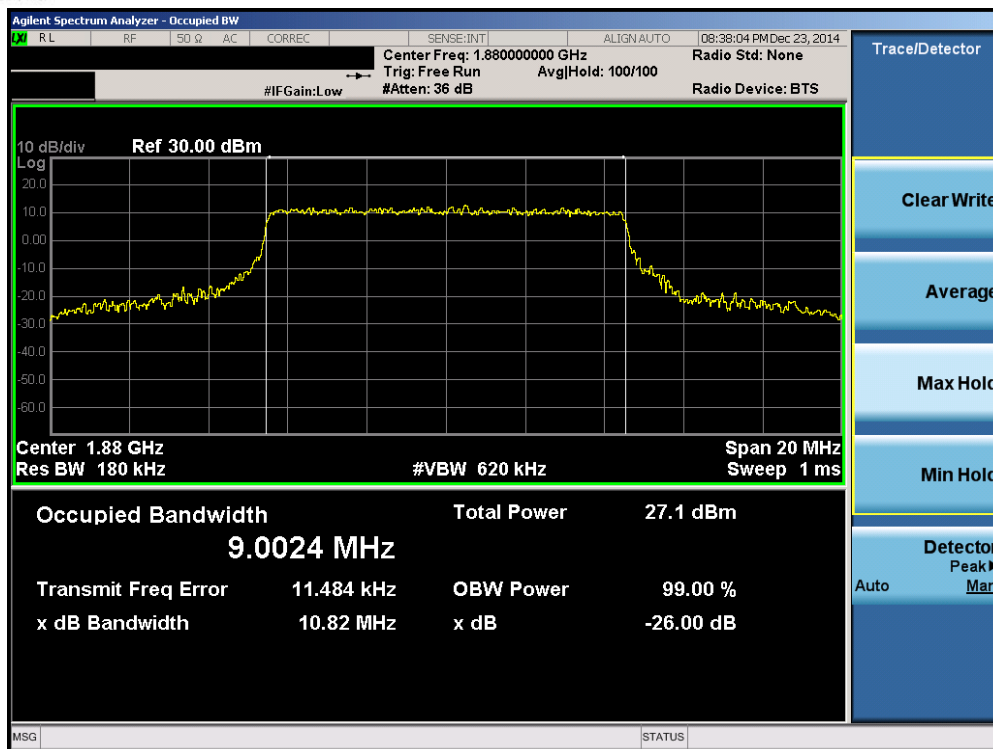
Plot 6-19. Occupied Bandwidth Plot (Band 2 – 10.0MHz QPSK – RB Size 50)
