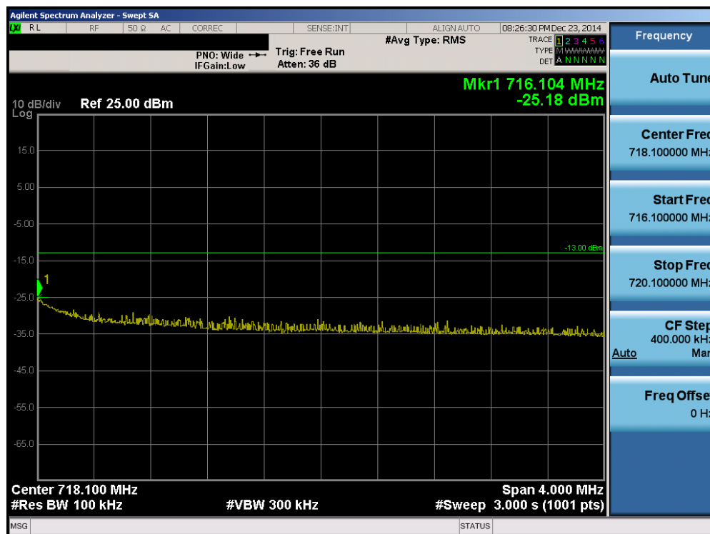
Plot 6-52. Upper Extended Band Edge Plot (Band 17 – 5.0MHz QPSK – RB Size 25)
