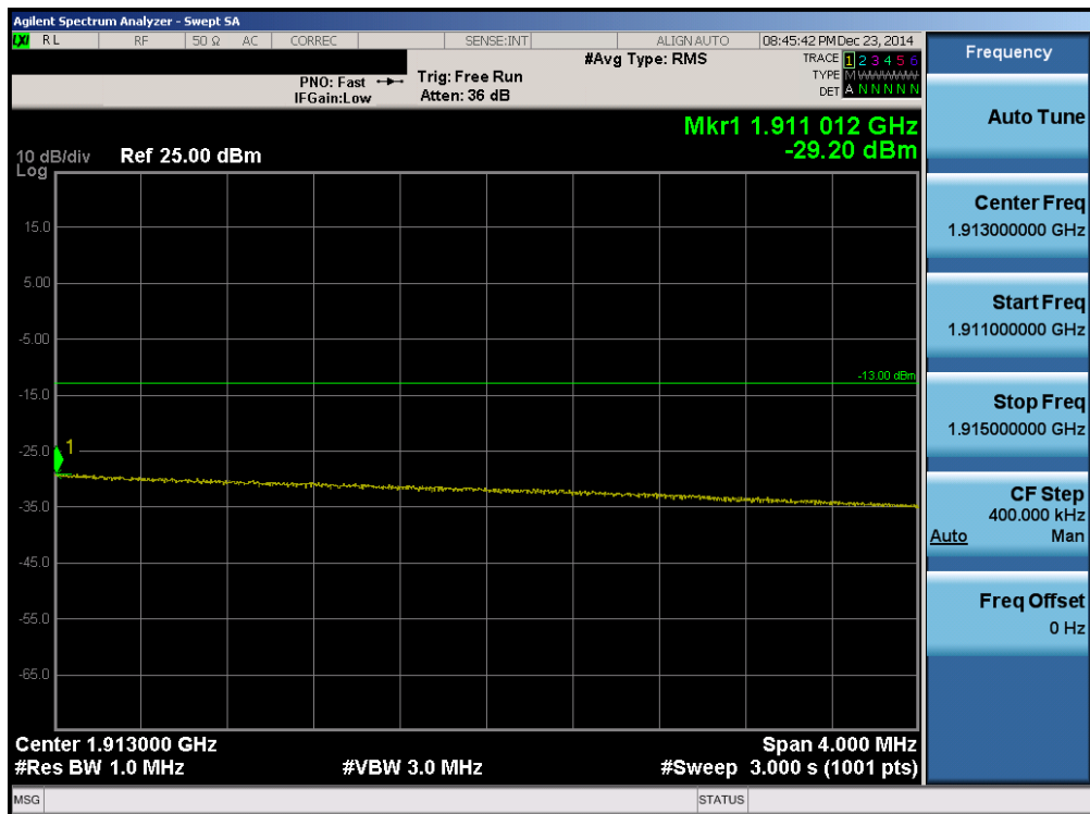
Plot 6-88. Upper Extended Band Edge Plot (Band 2 – 15.0MHz QPSK – RB Size 75)
