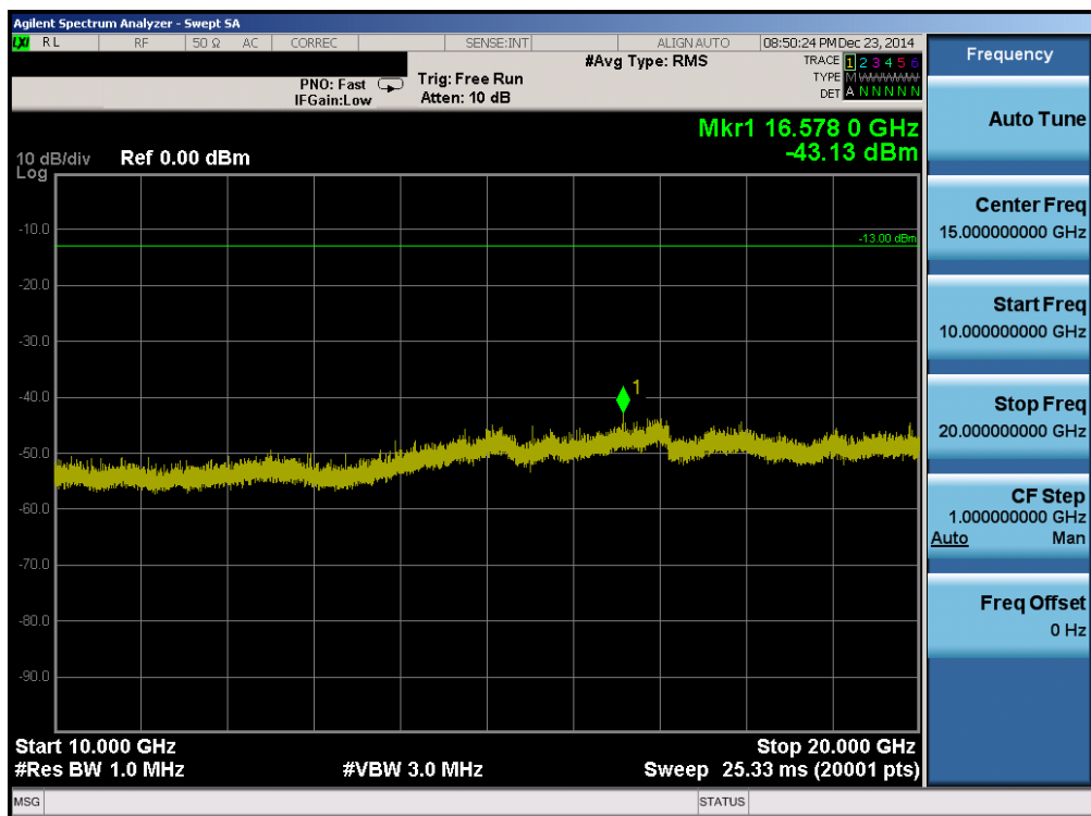
Plot 6-44. Conducted Spurious Plot (Band 2 – 20.0MHz QPSK – RB Size 1, RB Offset 0 – Low Channel)
