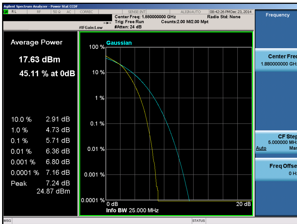
Plot 6-98. PAR Plot (Band 2 – 15.0MHz 16-QAM – RB Size 75)
