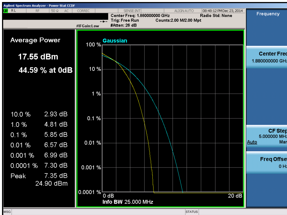
Plot 6-100. PAR Plot (Band 2 – 20.0MHz 16-QAM – RB Size 100)
