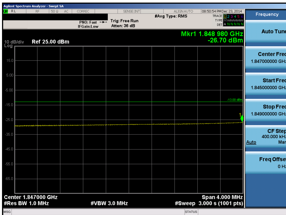
Plot 6-90. Lower Extended Band Edge Plot (Band 2 – 20.0MHz QPSK – RB Size 100)
