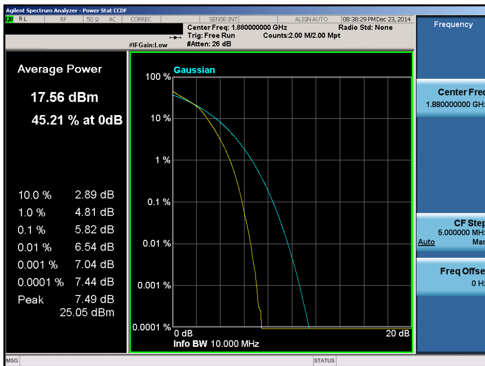
Plot 6-96. PAR Plot (Band 2 – 10.0MHz 16-QAM – RB Size 50)
