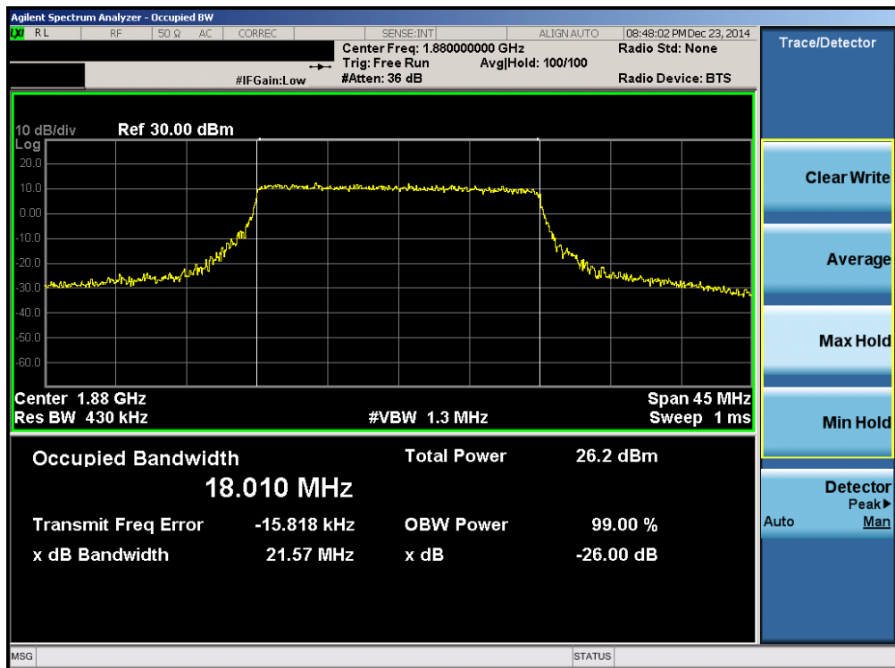
Plot 6-24. Occupied Bandwidth Plot (Band 2 – 20.0MHz 16-QAM – RB Size 100)
