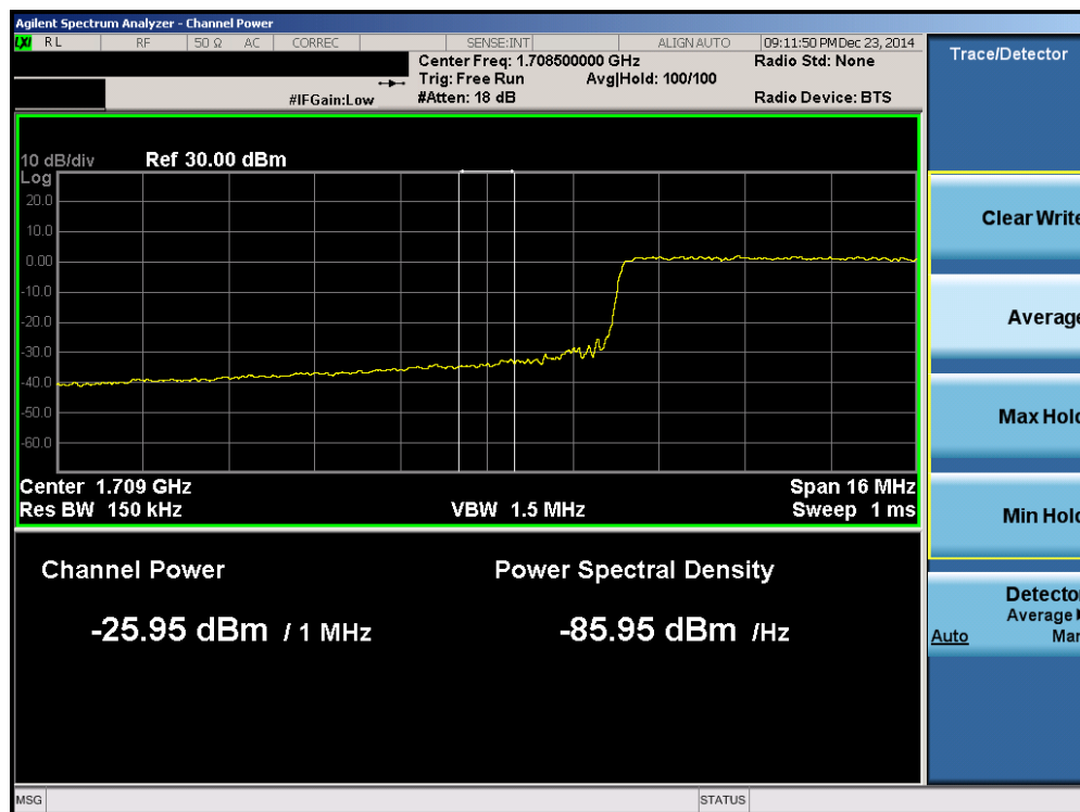
Plot 6-74. Lower Extended Band Edge Plot (Band 4 – 20.0MHz QPSK – RB Size 100)
