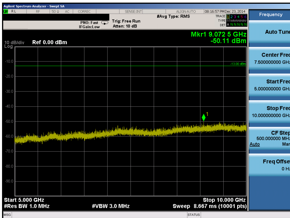
Plot 6-32. Conducted Spurious Plot (Band 5 – 10.0MHz QPSK – RB Size 1, RB Offset 0 – Low Channel)
