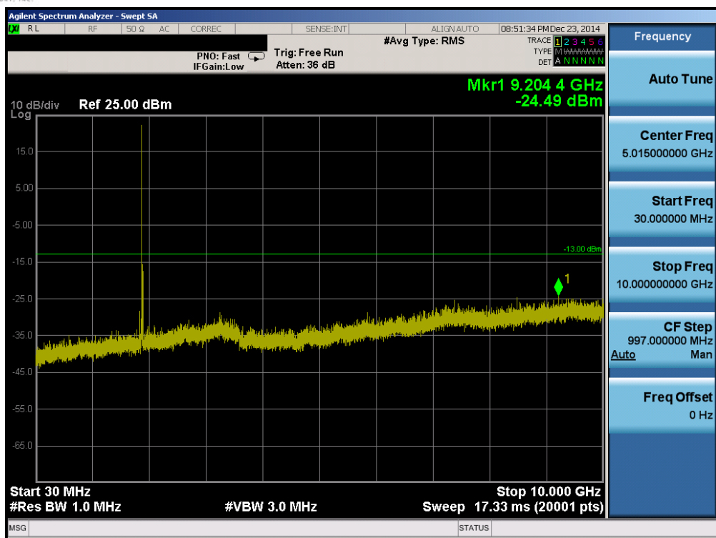
Plot 6-47. Conducted Spurious Plot (Band 2 – 20.0MHz QPSK – RB Size 1, RB Offset 0 – High Channel)
