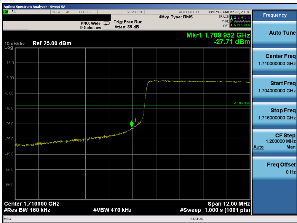
Plot 6-69. Lower Band Edge Plot (Band 4 – 15.0MHz QPSK – RB Size 75)
