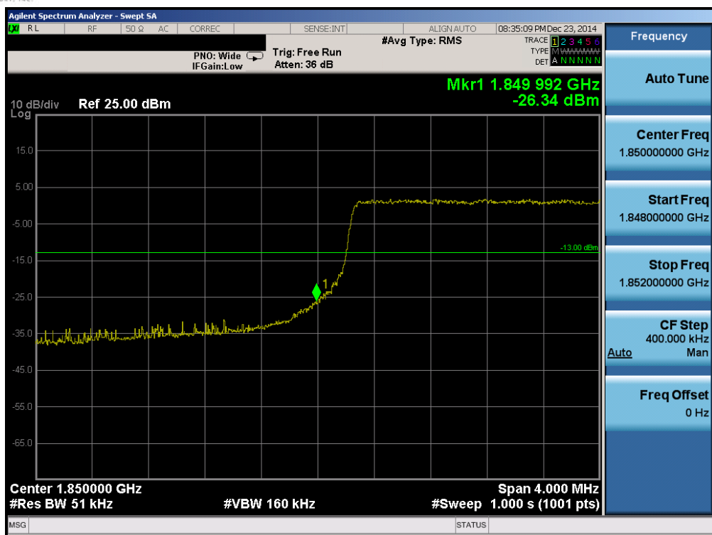
Plot 6-77. Lower Band Edge Plot (Band 2 – 5.0MHz QPSK – RB Size 25)
