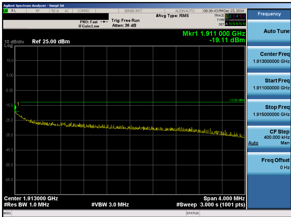
Plot 6-80. Upper Extended Band Edge Plot (Band 2 – 5.0MHz QPSK – RB Size 25)
