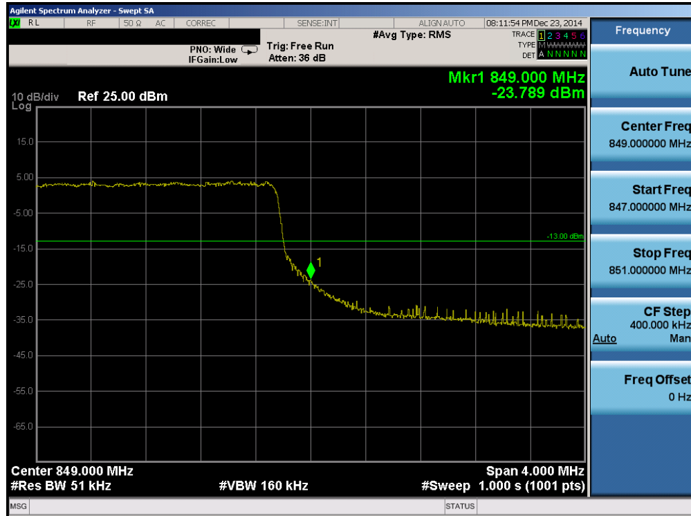
Plot 6-57. Upper Band Edge Plot (Band 5 - 5.0MHz QPSK - RB Size 25)
