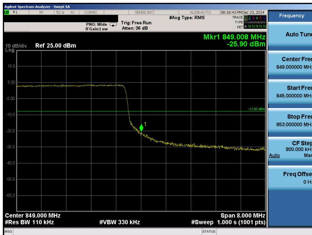
Plot 6-60. Upper Band Edge Plot (Band 5 – 10.0MHz QPSK – RB Size 50)
