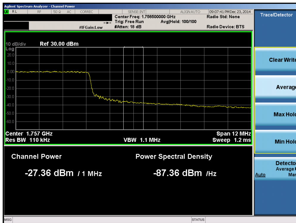
Plot 6-72. Upper Extended Band Edge Plot (Band 4 – 15.0MHz QPSK – RB Size 75)
