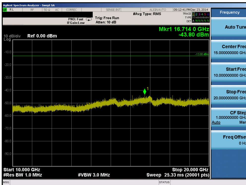
Plot 6-42. Conducted Spurious Plot (Band 4 – 20.0MHz QPSK – RB Size 1, RB Offset 0 – High Channel)
