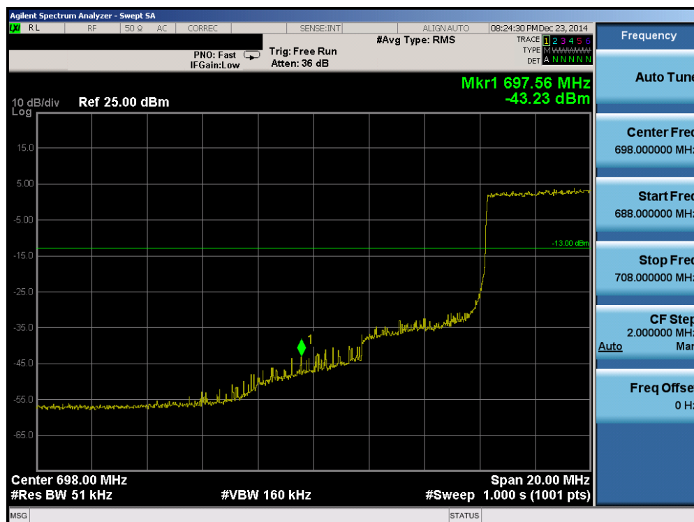
Plot 6-49. Lower Band Edge Plot (Band 17 – 5.0MHz QPSK – RB Size 25)
