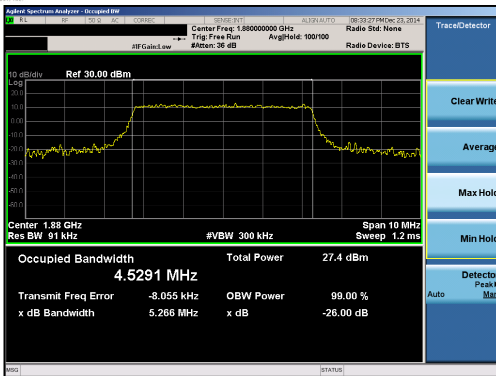
Plot 6-17. Occupied Bandwidth Plot (Band 2 – 5.0MHz QPSK – RB Size 25)
