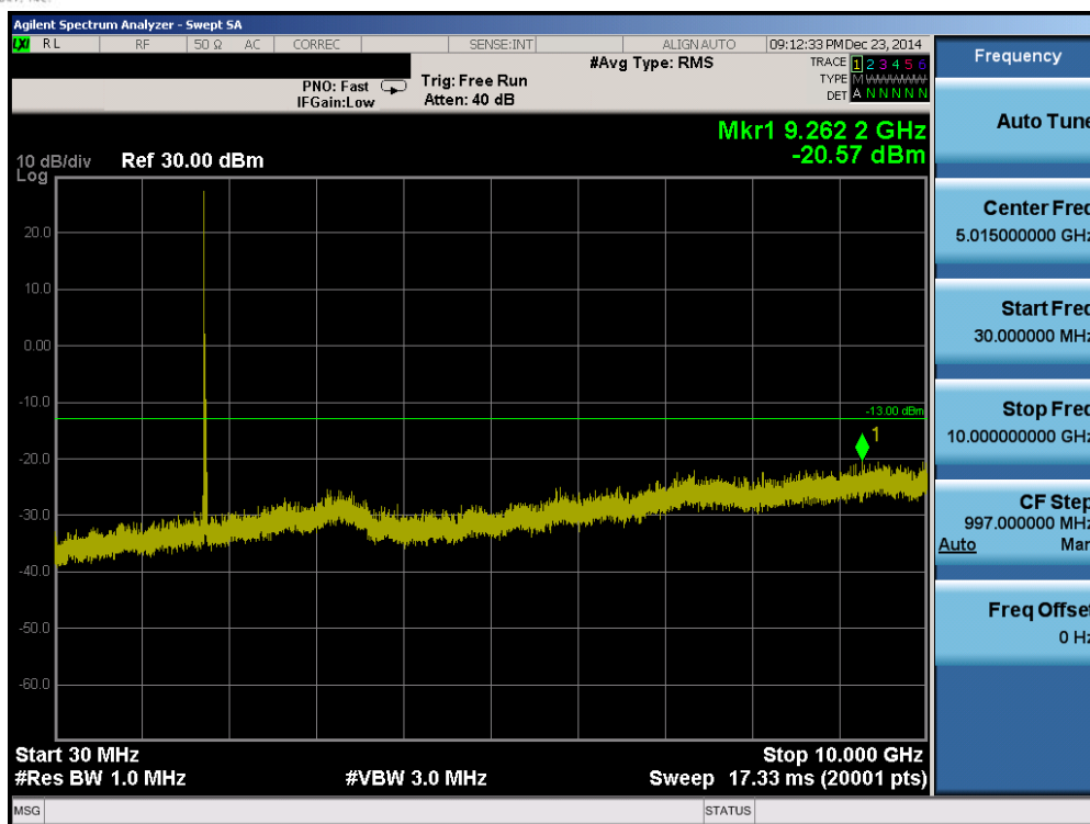
Plot 6-41. Conducted Spurious Plot (Band 4 – 20.0MHz QPSK – RB Size 1, RB Offset 0 – High Channel)
