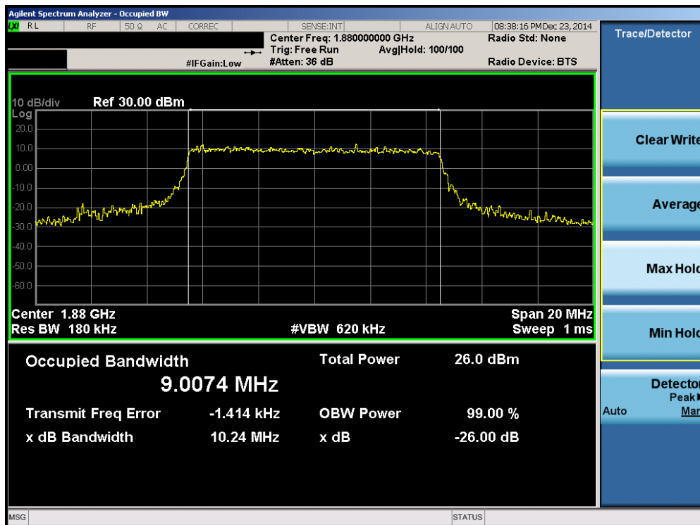
Plot 6-20. Occupied Bandwidth Plot (Band 2 – 10.0MHz 16-QAM – RB Size 50)
