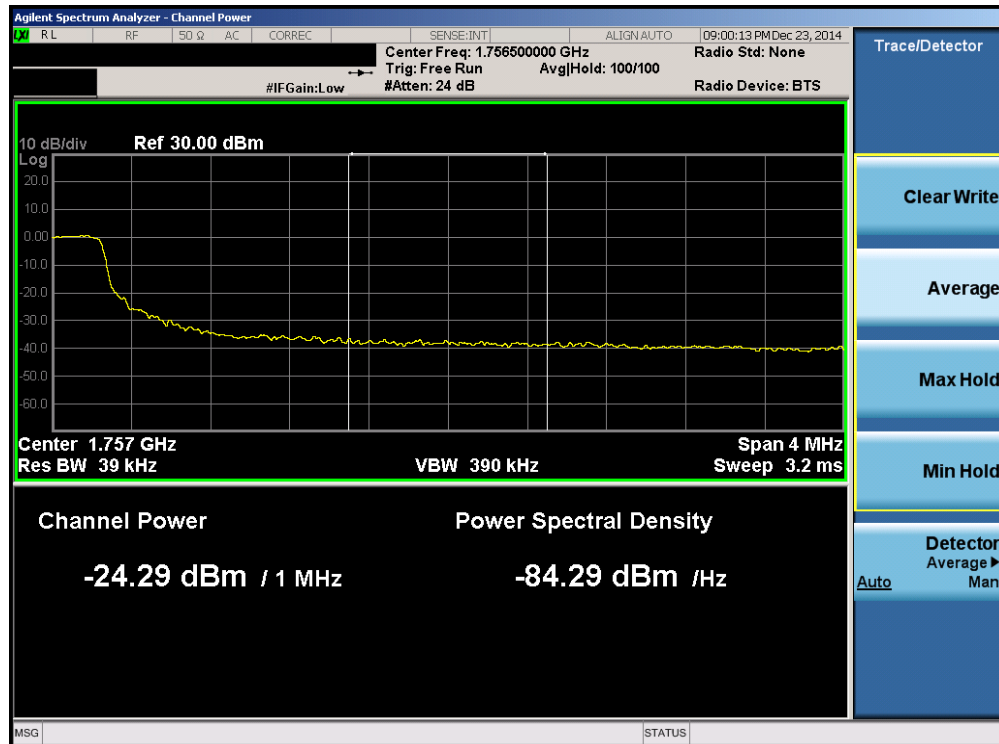
Plot 6-64. Upper Extended Band Edge Plot (Band 4 – 5.0MHz QPSK – RB Size 25)
