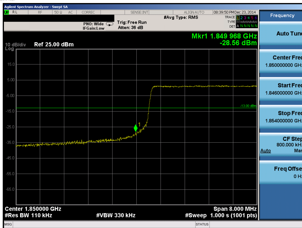
Plot 6-81. Lower Band Edge Plot (Band 2 – 10.0MHz QPSK – RB Size 50)
