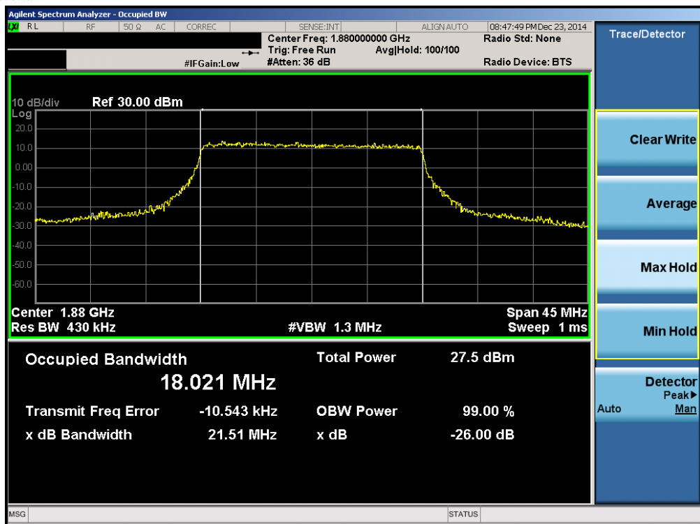
Plot 6-23. Occupied Bandwidth Plot (Band 2 – 20.0MHz QPSK – RB Size 100)
