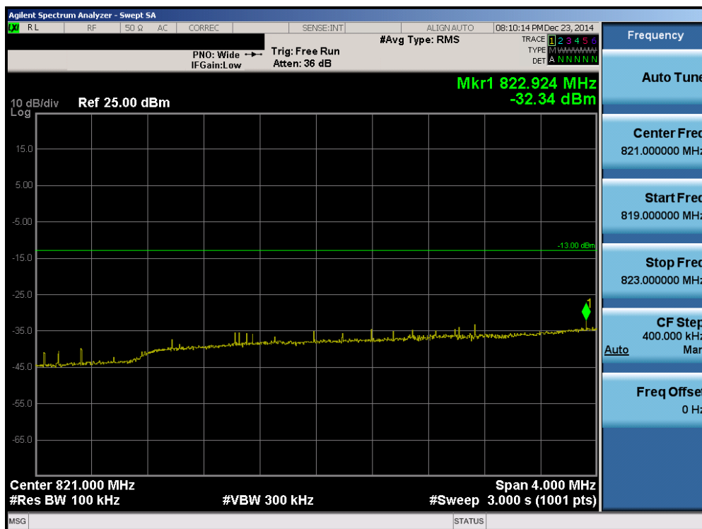
Plot 6-56. Lower Extended Band Edge Plot (Band 5 – 5.0MHz QPSK – RB Size 25)
