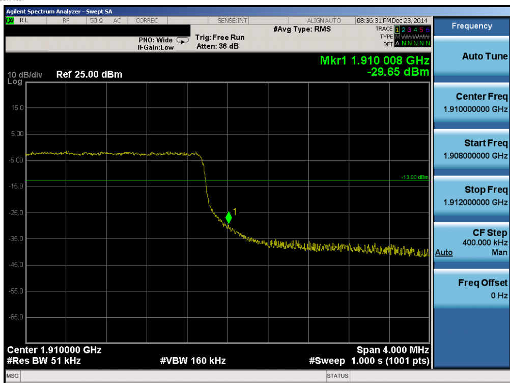
Plot 6-79. Upper Band Edge Plot (Band 2 – 5.0MHz QPSK – RB Size 25)
