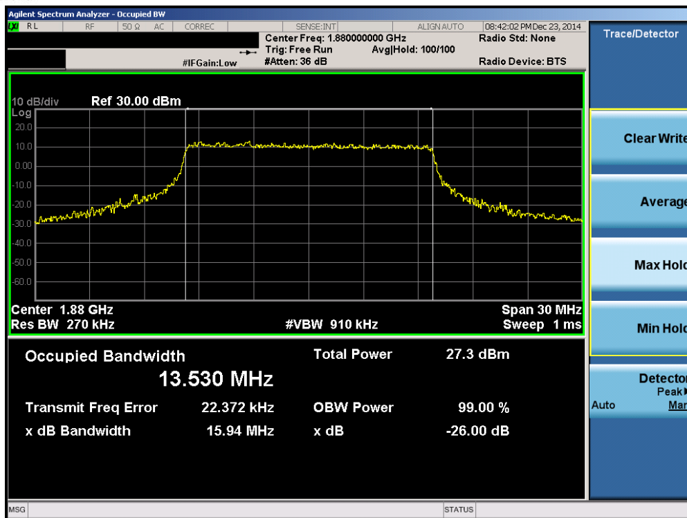
Plot 6-21. Occupied Bandwidth Plot (Band 2 – 15.0MHz QPSK – RB Size 75)
