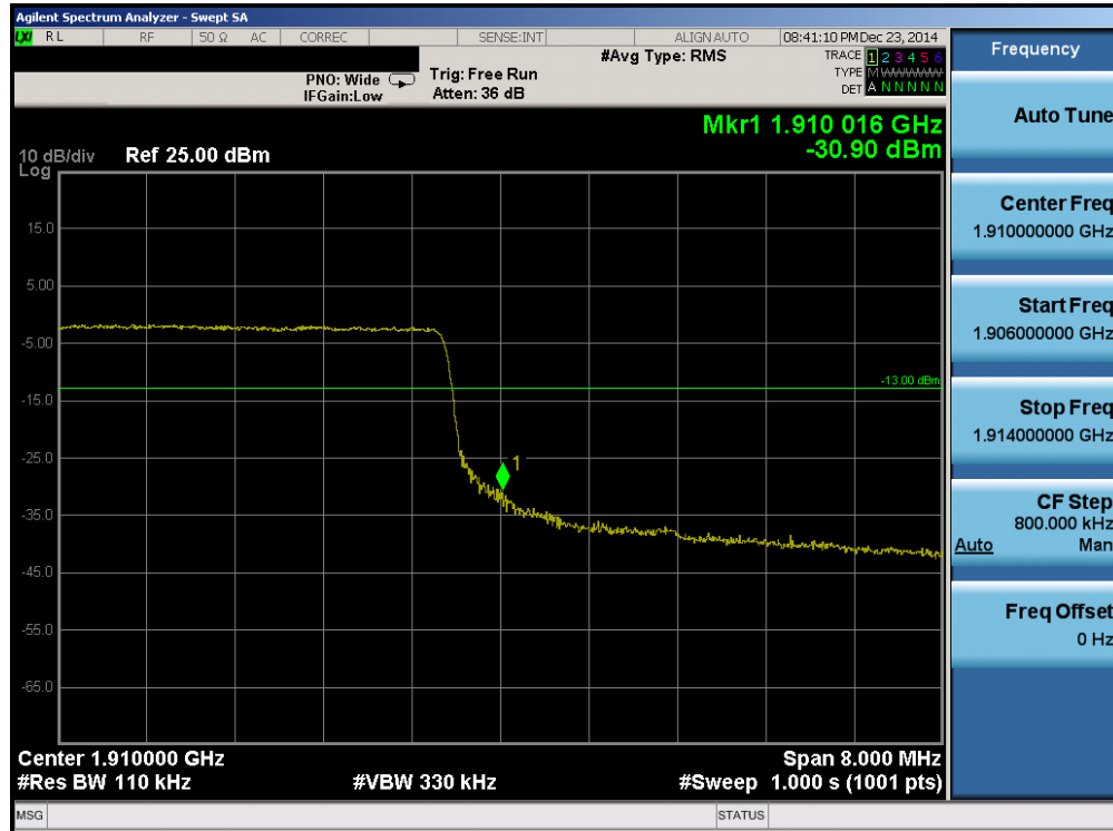
Plot 6-83. Upper Band Edge Plot (Band 2 – 10.0MHz QPSK – RB Size 50)
