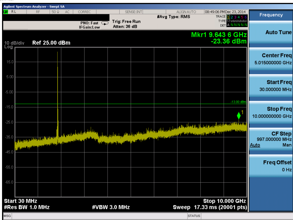
Plot 6-45. Conducted Spurious Plot (Band 2 – 20.0MHz QPSK – RB Size 1, RB Offset 0 – Mid Channel)
