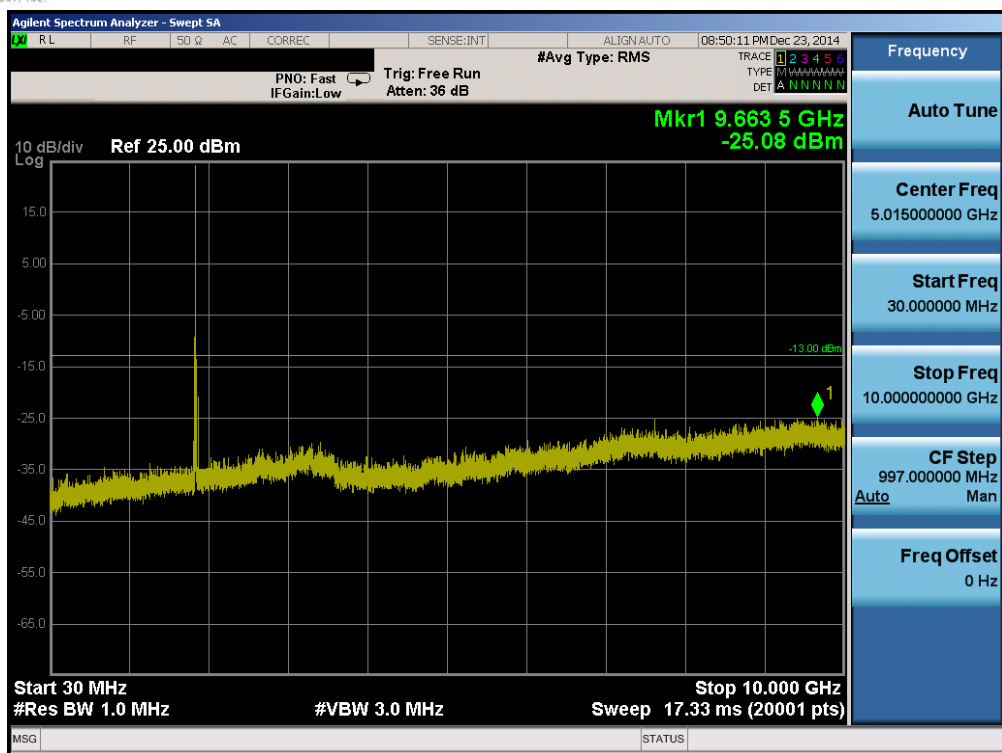
Plot 6-43. Conducted Spurious Plot (Band 2 – 20.0MHz QPSK – RB Size 1, RB Offset 0– Low Channel)
