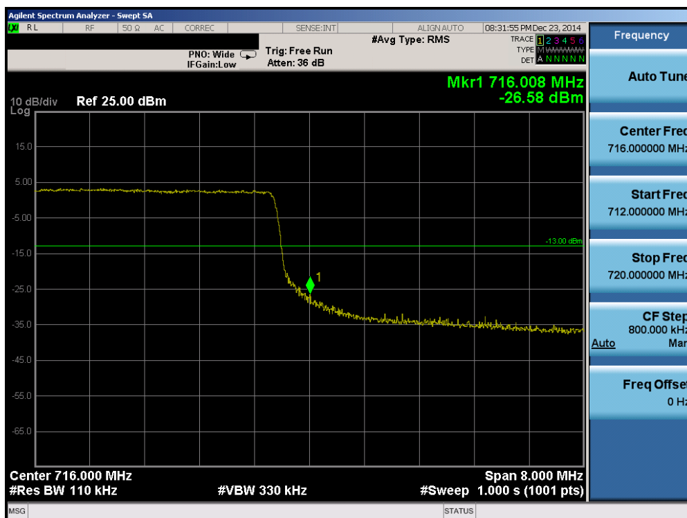
Plot 6-54. Upper Band Edge Plot (Band 17 – 10.0MHz QPSK – RB Size 50)
