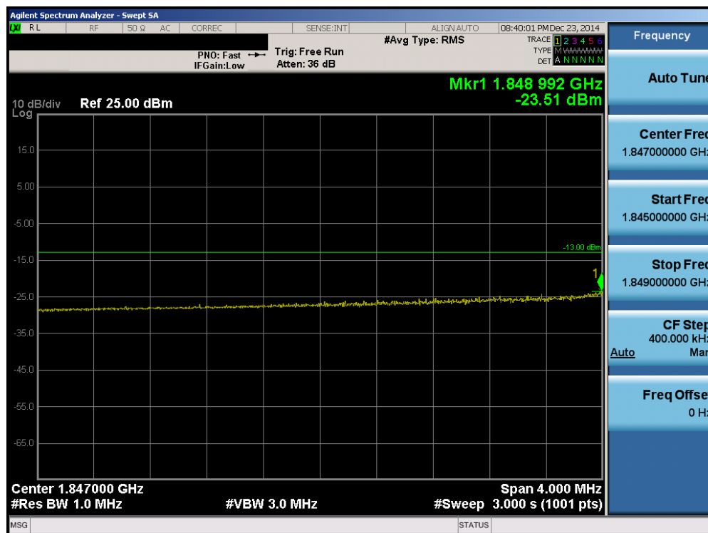
Plot 6-82. Lower Extended Band Edge Plot (Band 2 – 10.0MHz QPSK – RB Size 50)
