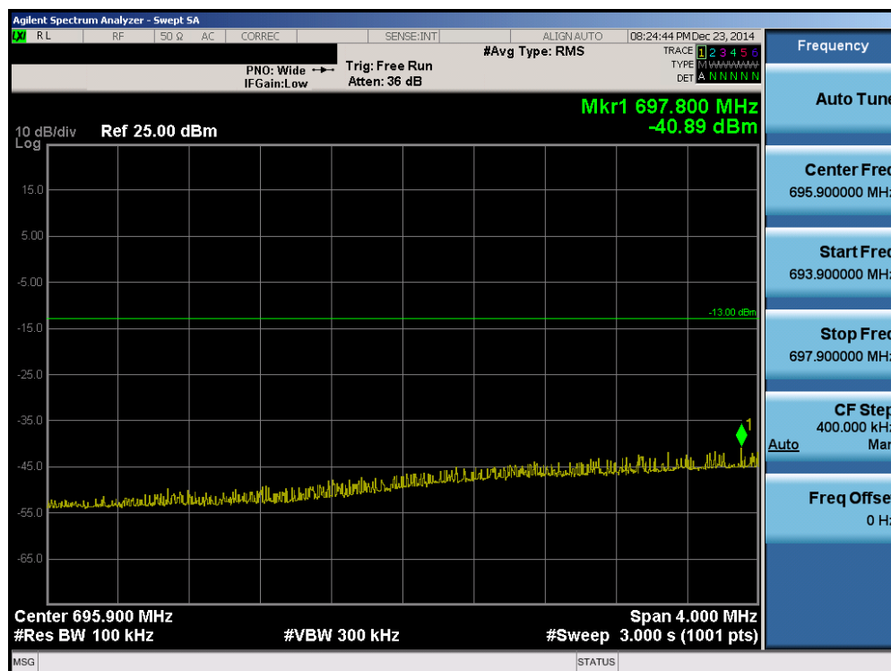
Plot 6-50. Lower Extended Band Edge Plot (Band 17 – 5.0MHz QPSK – RB Size 25)
