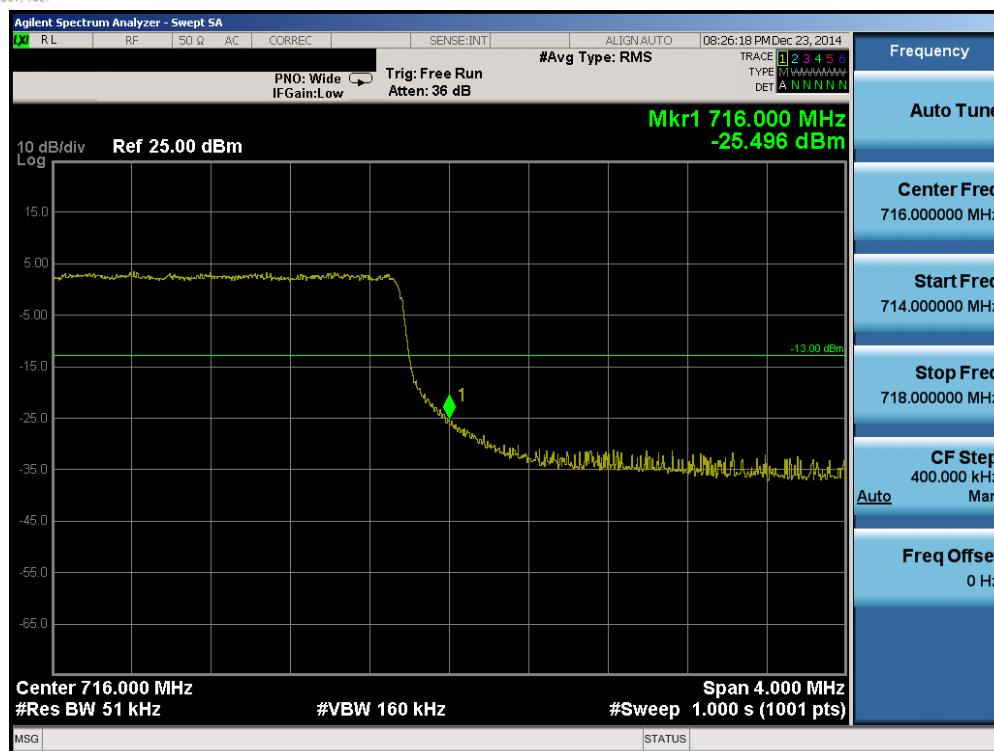
Plot 6-51. Upper Band Edge Plot (Band 17 – 5.0MHz QPSK – RB Size 25)
