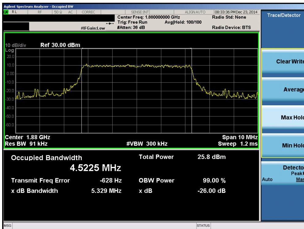
Plot 6-18. Occupied Bandwidth Plot (Band 2 – 5.0MHz 16-QAM – RB Size 25)
