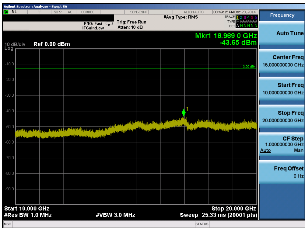
Plot 6-46. Conducted Spurious Plot (Band 2 – 20.0MHz QPSK – RB Size 1, RB Offset 0 – Mid Channel)
