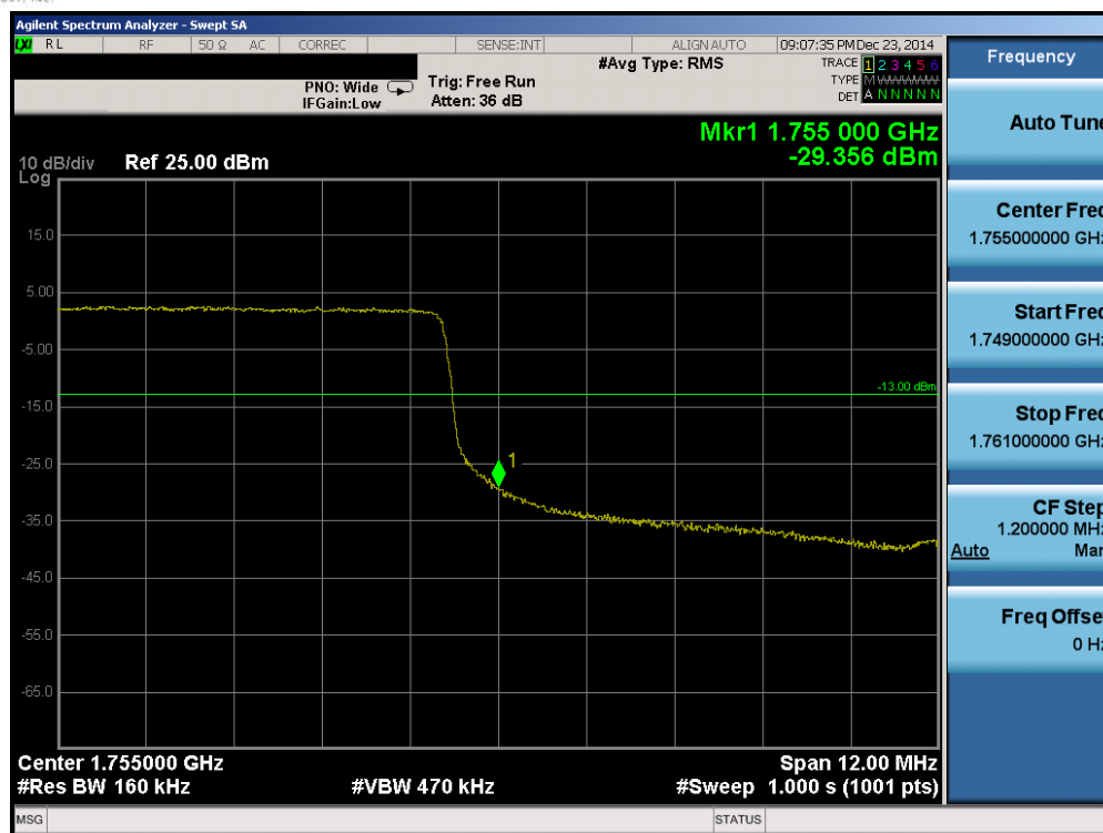
Plot 6-71. Upper Band Edge Plot (Band 4 – 15.0MHz QPSK – RB Size 75)
