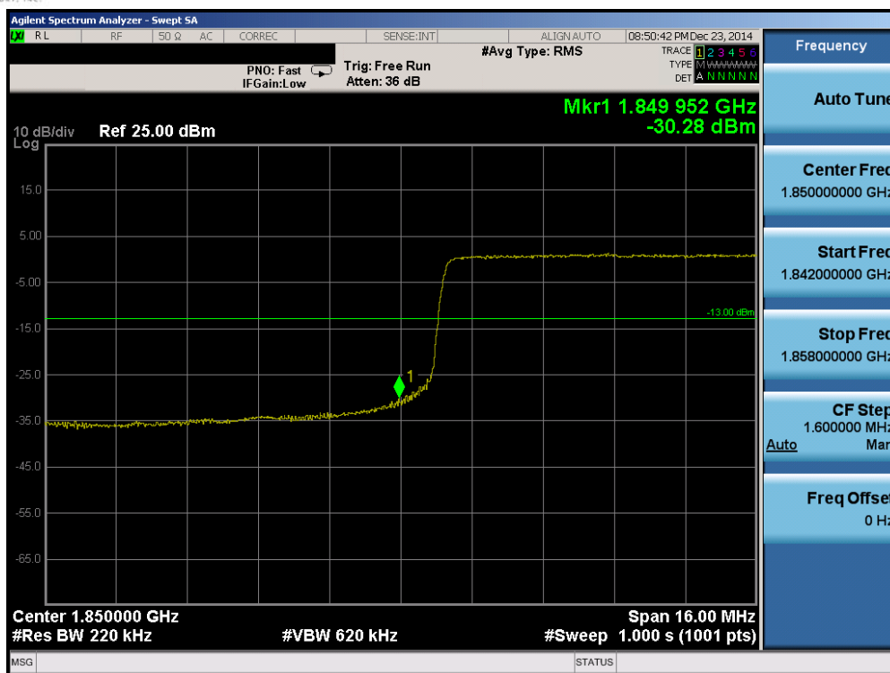
Plot 6-89. Lower Band Edge Plot (Band 2 – 20.0MHz QPSK – RB Size 100)
