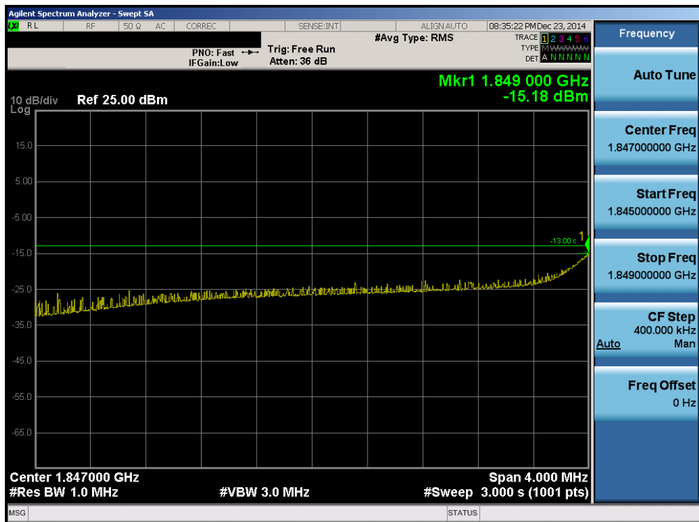
Plot 6-78. Lower Extended Band Edge Plot (Band 2 – 5.0MHz QPSK – RB Size 25)
