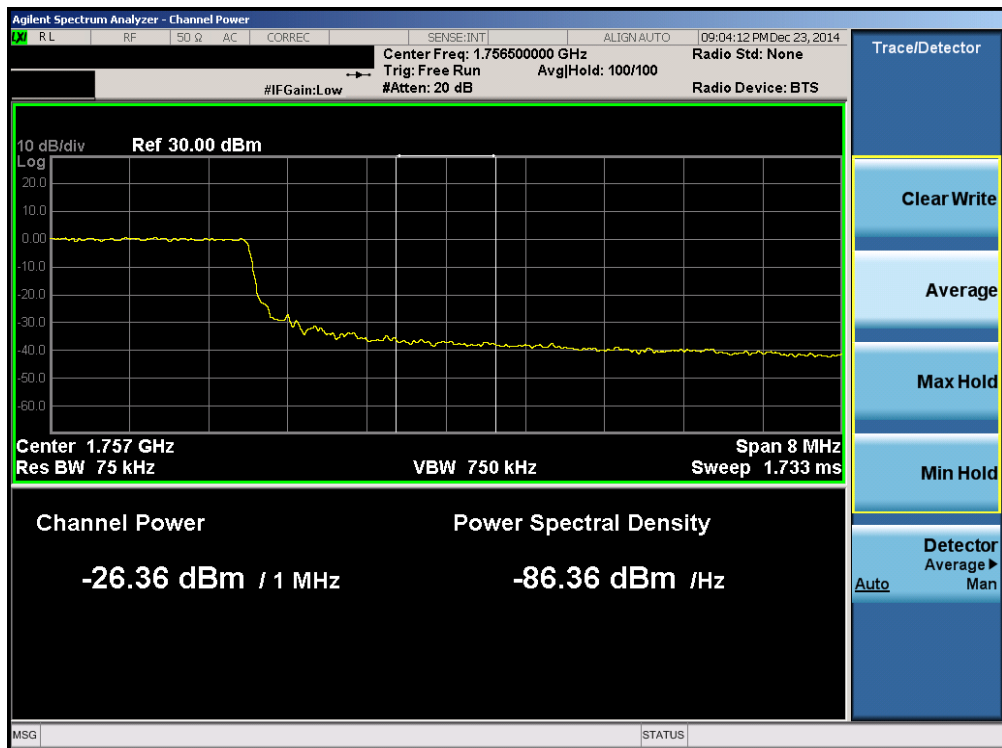
Plot 6-68. Upper Extended Band Edge Plot (Band 4 – 10.0MHz QPSK – RB Size 50)
