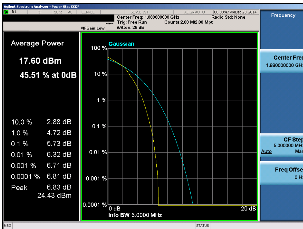
Plot 6-94. PAR Plot (Band 2 – 5.0MHz 16-QAM – RB Size 25)
