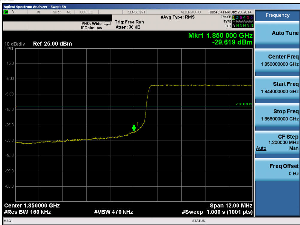
Plot 6-85. Lower Band Edge Plot (Band 2 – 15.0MHz QPSK – RB Size 75)
