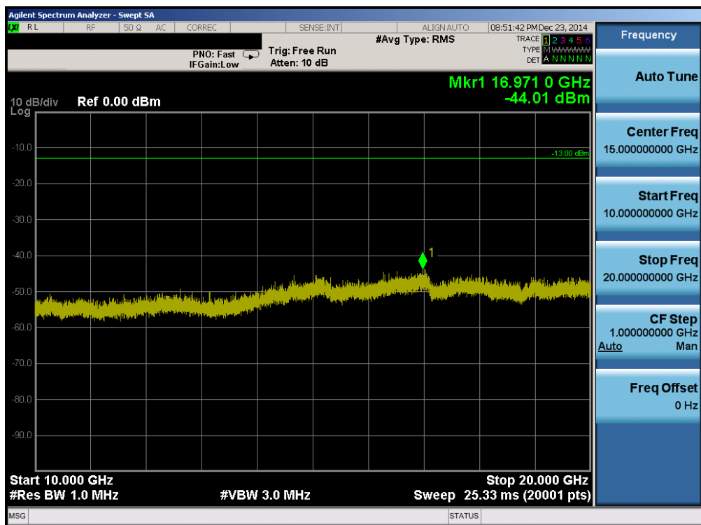
Plot 6-48. Conducted Spurious Plot (Band 2 – 20.0MHz QPSK – RB Size 1, RB Offset 0 – High Channel)
