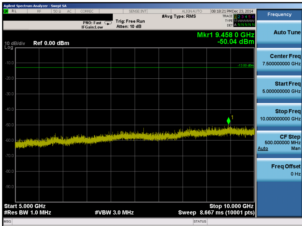
Plot 6-36. Conducted Spurious Plot (Band 5 – 10.0MHz QPSK – RB Size 1, RB Offset 0 – High Channel)
