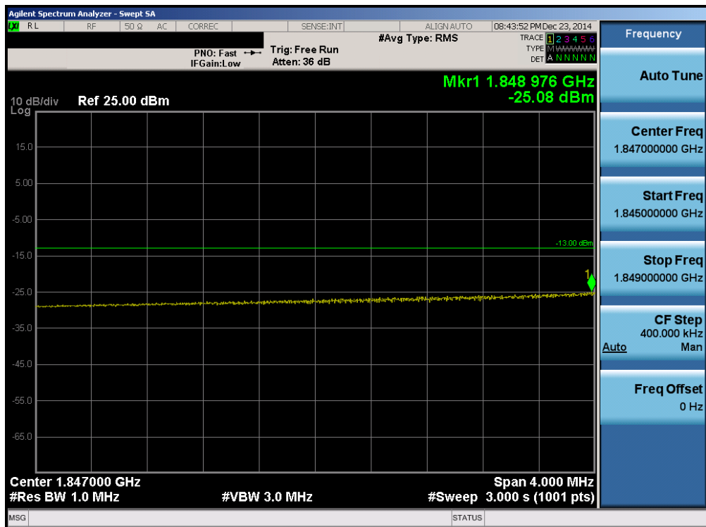
Plot 6-86. Lower Extended Band Edge Plot (Band 2 – 15.0MHz QPSK – RB Size 75)
