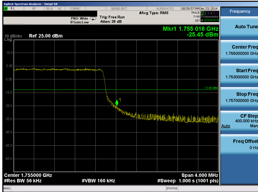
Plot 6-63. Upper Band Edge Plot (Band 4 – 5.0MHz QPSK – RB Size 25)
