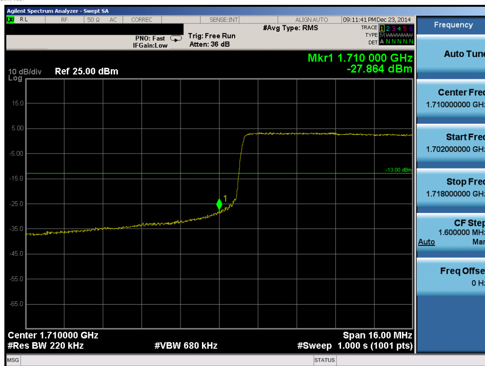
Plot 6-73. Lower Band Edge Plot (Band 4 – 20.0MHz QPSK – RB Size 100)
