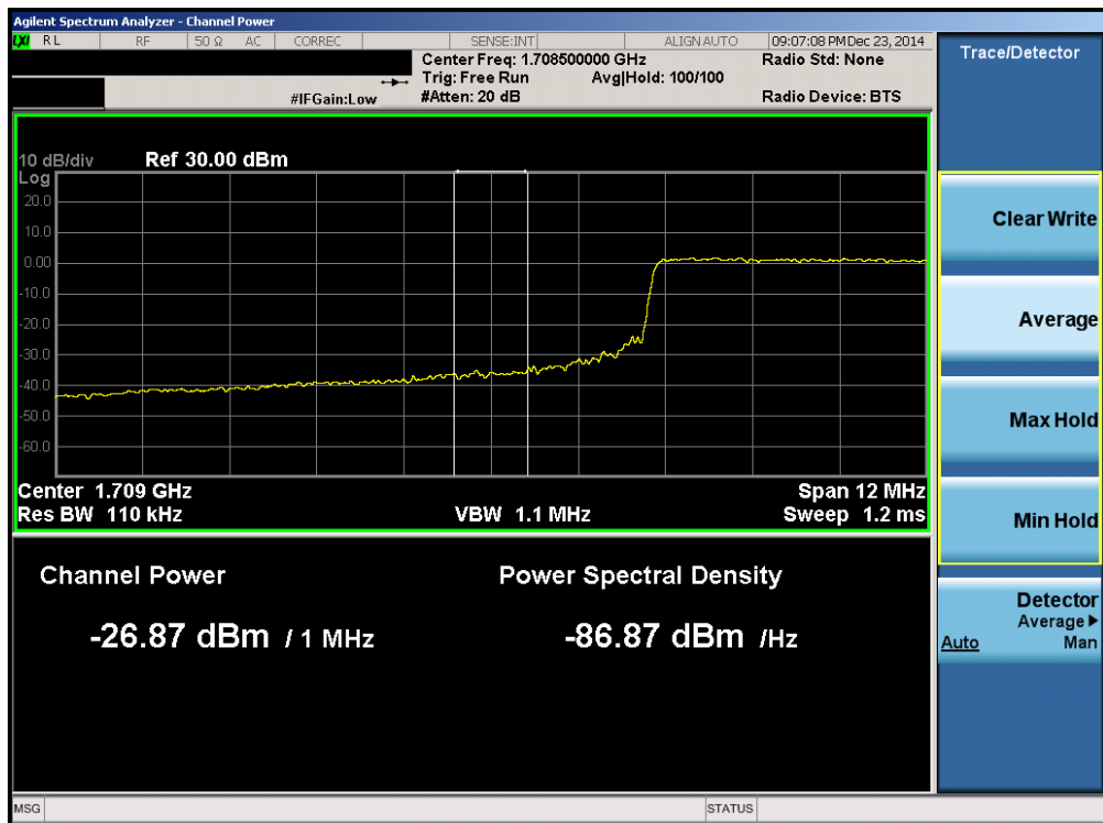
Plot 6-70. Lower Extended Band Edge Plot (Band 4 – 15.0MHz QPSK – RB Size 75)
