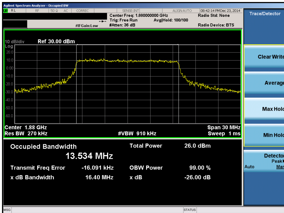
Plot 6-22. Occupied Bandwidth Plot (Band 2 – 15.0MHz 16-QAM – RB Size 75)
