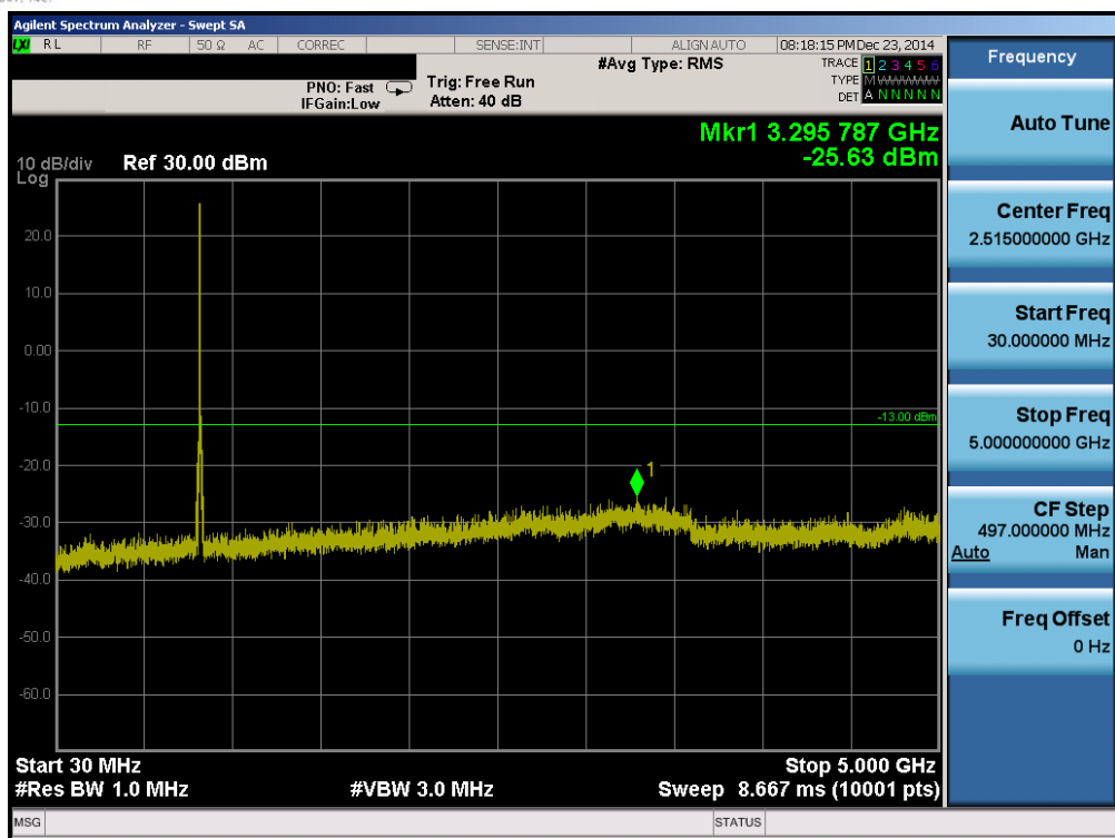
Plot 6-35. Conducted Spurious Plot (Band 5 – 10.0MHz QPSK – RB Size 1, RB Offset 0 – High Channel)
