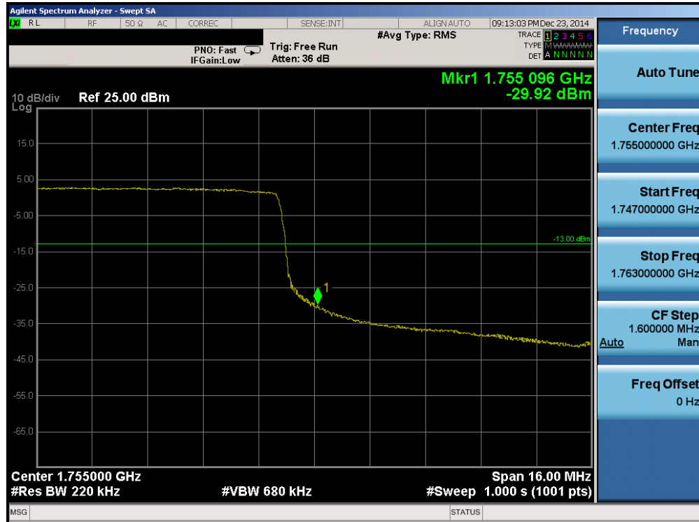
Plot 6-75. Upper Band Edge Plot (Band 4 – 20.0MHz QPSK – RB Size 100)
