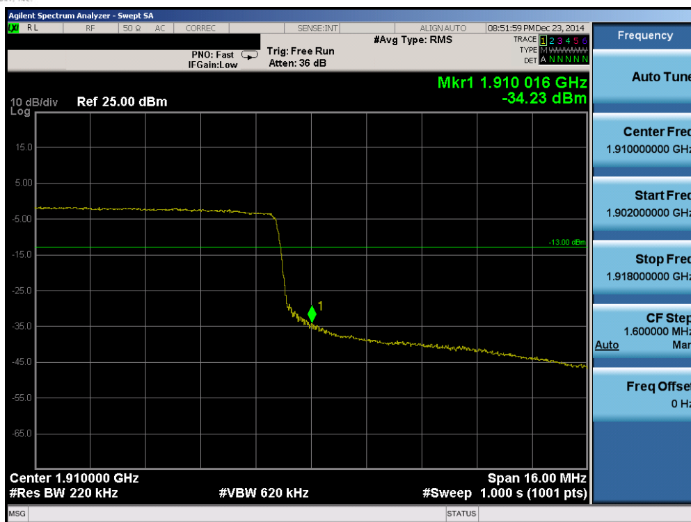
Plot 6-91. Upper Band Edge Plot (Band 2 – 20.0MHz QPSK – RB Size 100)
