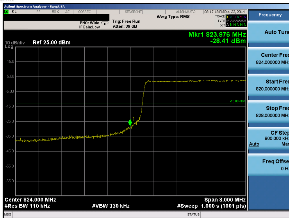
Plot 6-59. Lower Band Edge Plot (Band 5 – 10.0MHz QPSK – RB Size 50)
