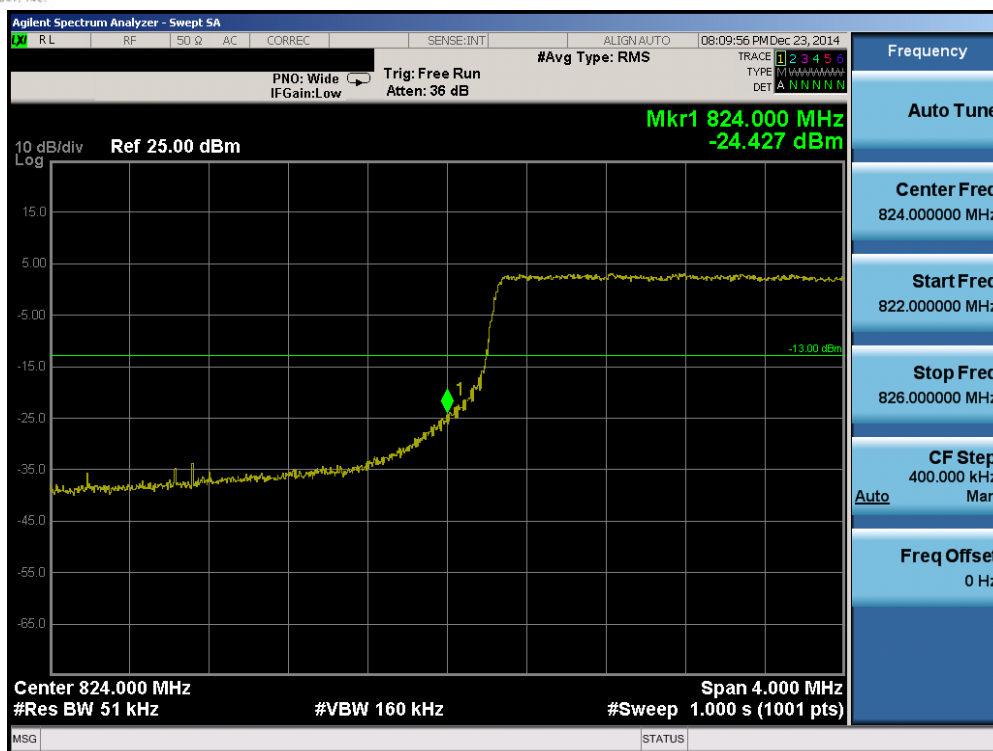
Plot 6-55. Lower Band Edge Plot (Band 5 – 5.0MHz QPSK – RB Size 25)
