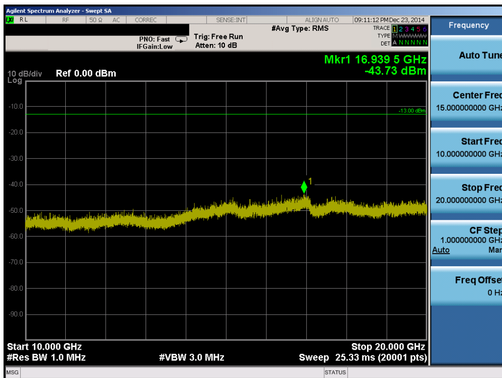
Plot 6-38. Conducted Spurious Plot (Band 4 – 20.0MHz QPSK – RB Size 1, RB Offset 0 – Low Channel)
