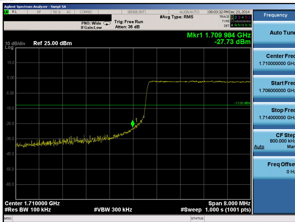
Plot 6-65. Lower Band Edge Plot (Band 4 – 10.0MHz QPSK – RB Size 50)
