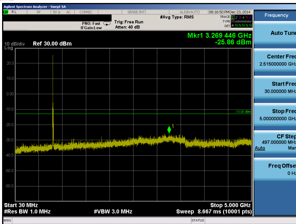
Plot 6-31. Conducted Spurious Plot (Band 5 – 10.0MHz QPSK – RB Size 1, RB Offset 0– Low Channel)
