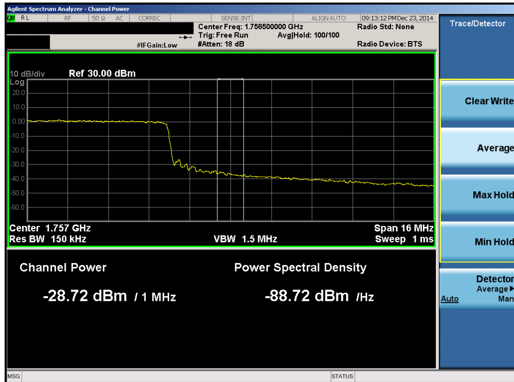
Plot 6-76. Upper Extended Band Edge Plot (Band 4 – 20.0MHz QPSK – RB Size 100)
