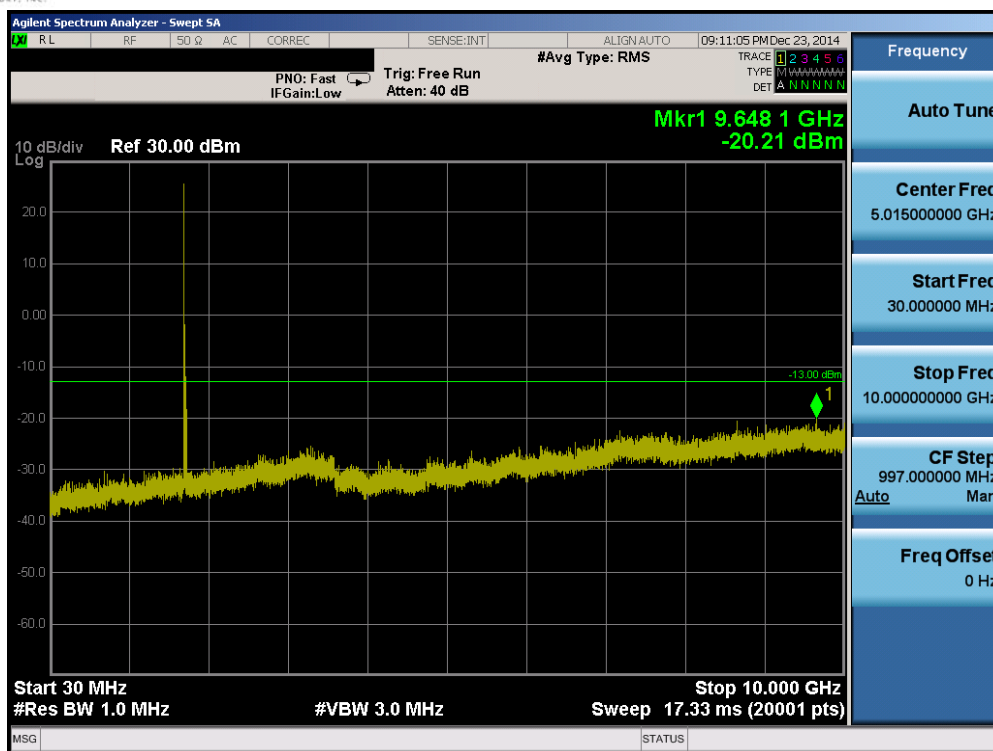
Plot 6-37. Conducted Spurious Plot (Band 4 – 20.0MHz QPSK – RB Size 1, RB Offset 0– Low Channel)
