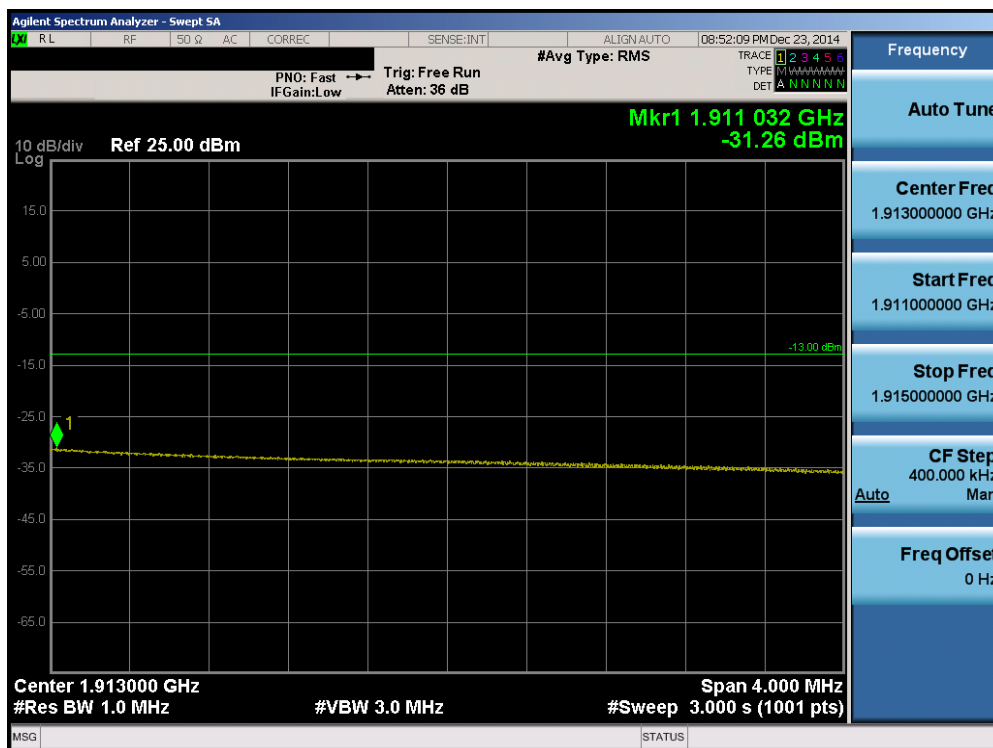
Plot 6-92. Upper Extended Band Edge Plot (Band 2 – 20.0MHz QPSK – RB Size 100)
