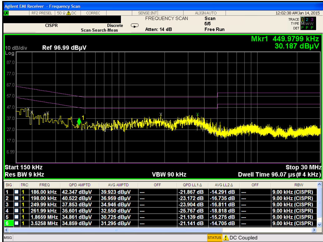
Plot 6-36. Line Conducted Plot with 802.11b (N)
