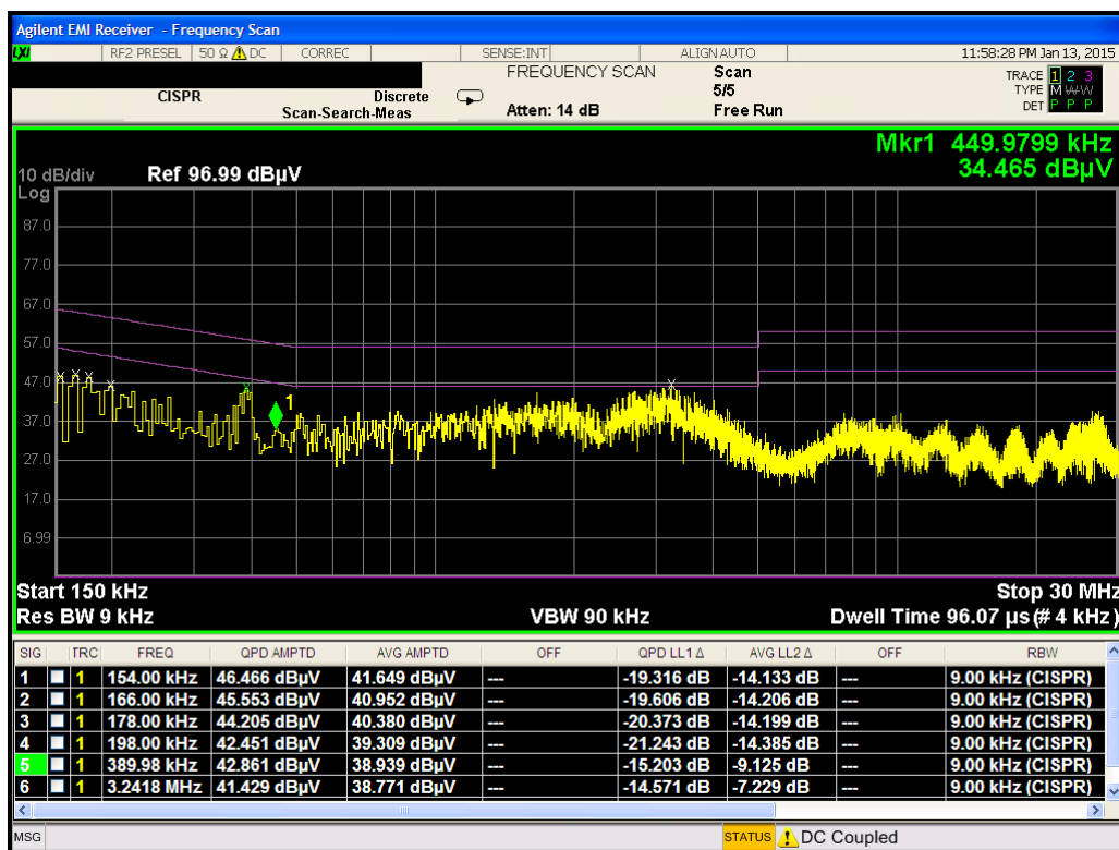
Plot 6-35. Line Conducted Plot with 802.11b (L1)
