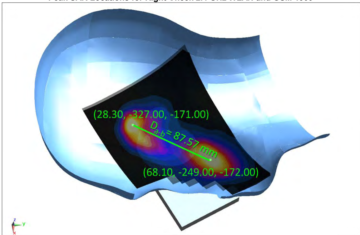
Figure 11-1 Peak SAR Locations for Right Cheek 2.4 GHz WLAN and GSM 1900
