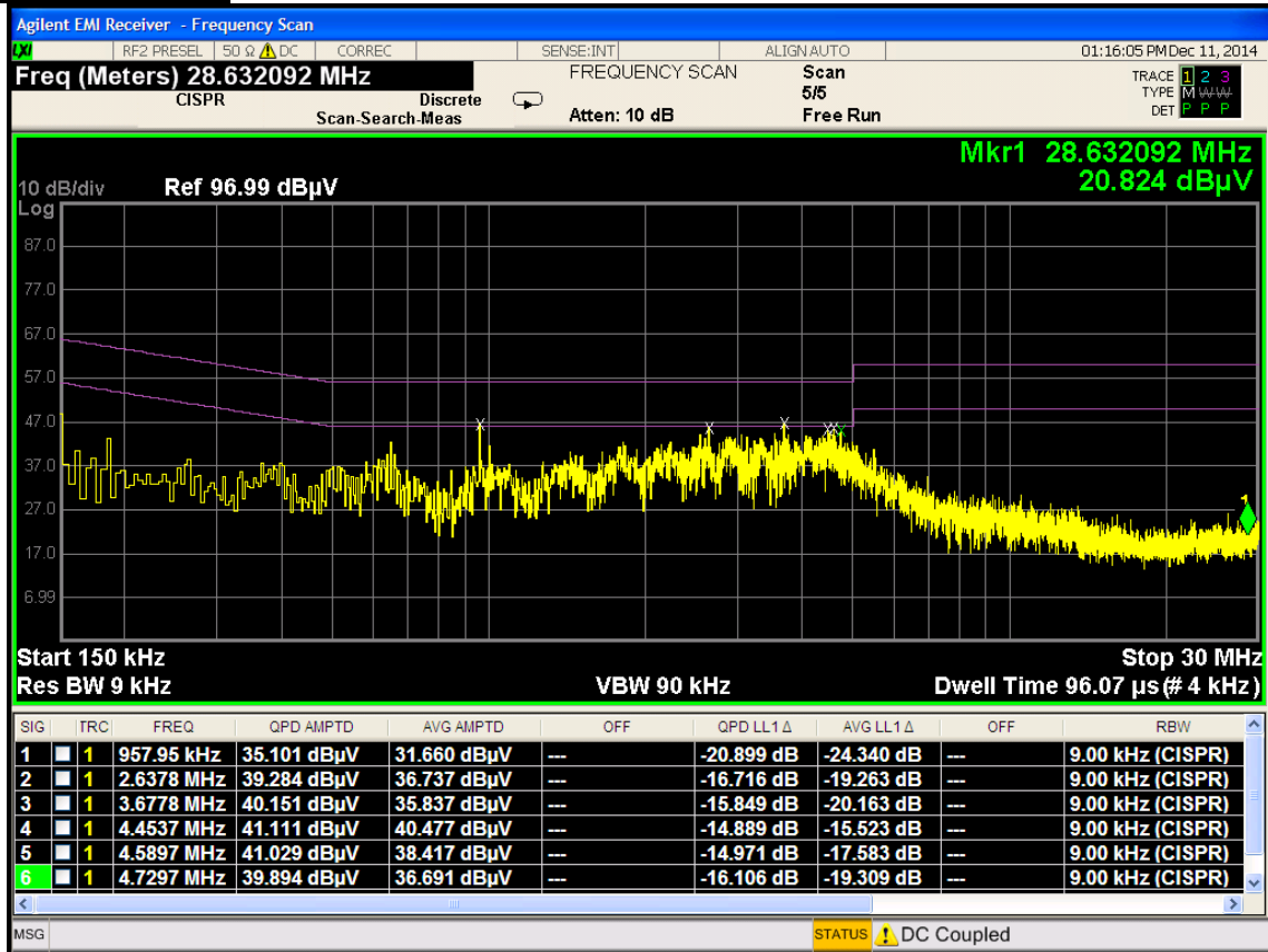
Plot 6-20. Line Conducted Plot and Data with Bluetooth LE (N)
