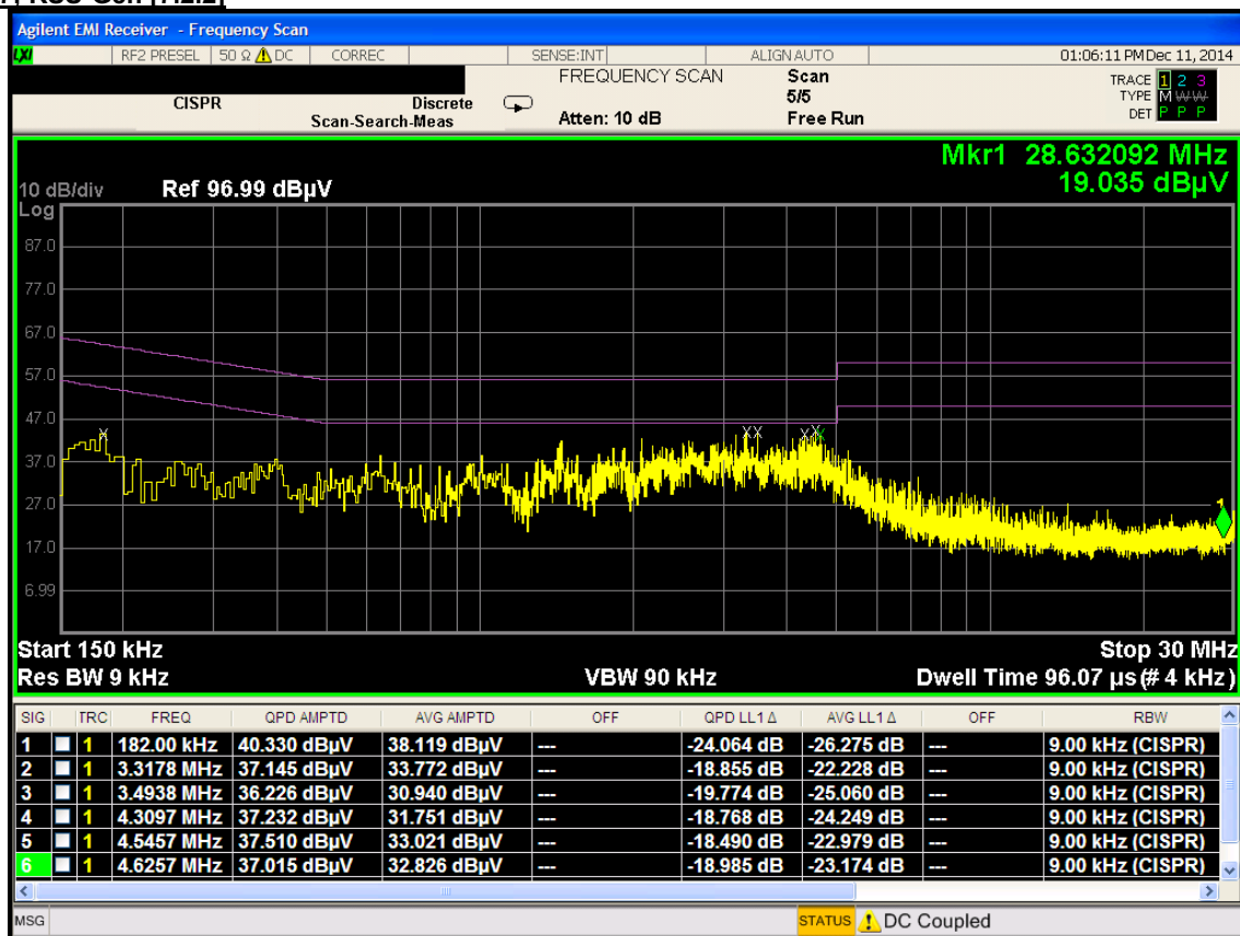
Plot 6-19. Line Conducted Plot and Data with Bluetooth LE (L1)
