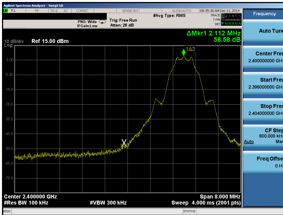
Plot 6-10. Band Edge Plot (Bluetooth (LE) – Ch. 0)
