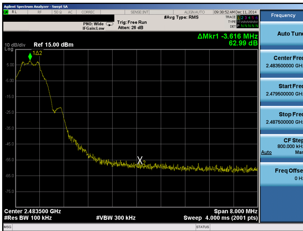
Plot 6-11. Band Edge Plot (Bluetooth (LE) – Ch. 39)
