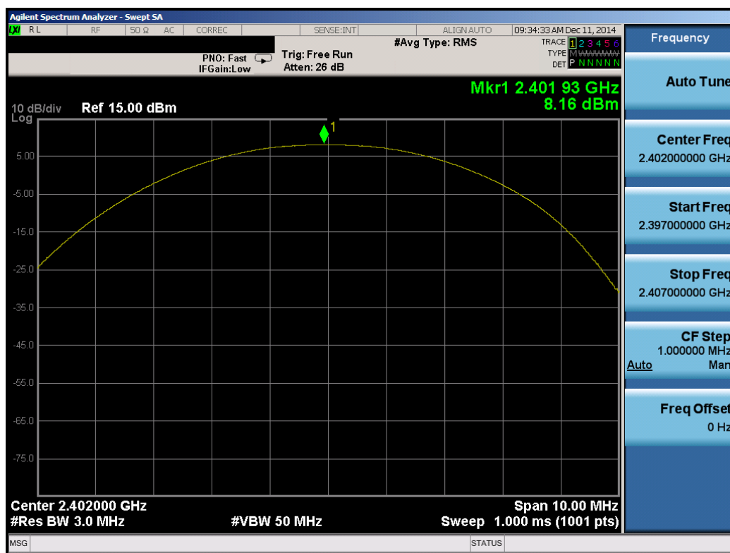
Plot 6-4. Peak Power Plot (Bluetooth (LE) – Ch. 0)
