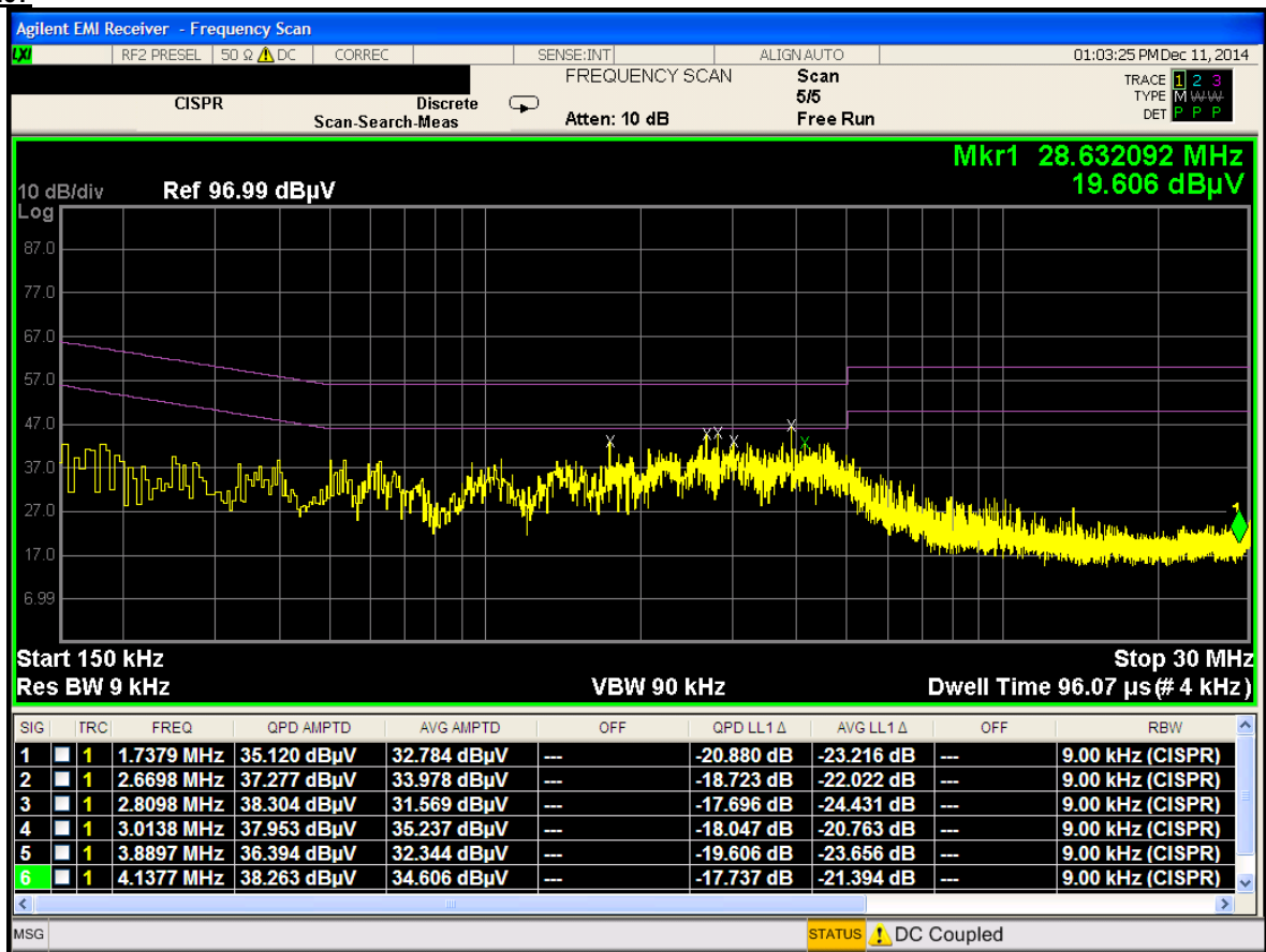
Plot 6-43. Line-Conducted Test Plot and Data (L1)
