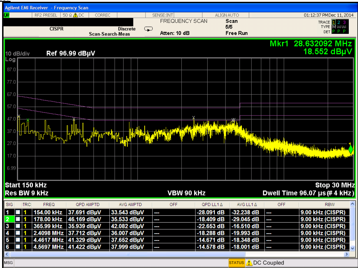
Plot 6-44. Line-Conducted Test Plot and Data (N)
