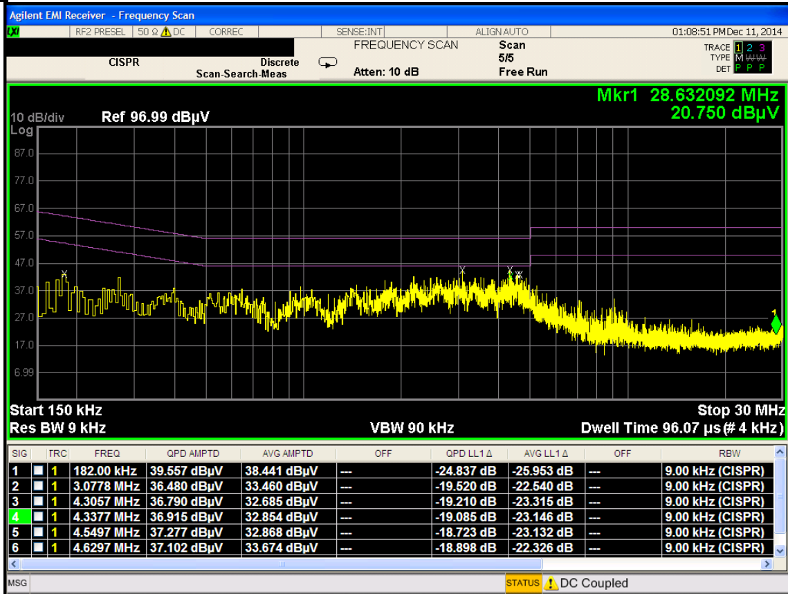
Plot 6-33. Line Conducted Plot and Data with 802.11b (L1)
