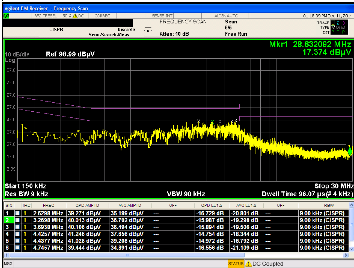
Plot 6-34. Line Conducted Plot and Data with 802.11b (N)
