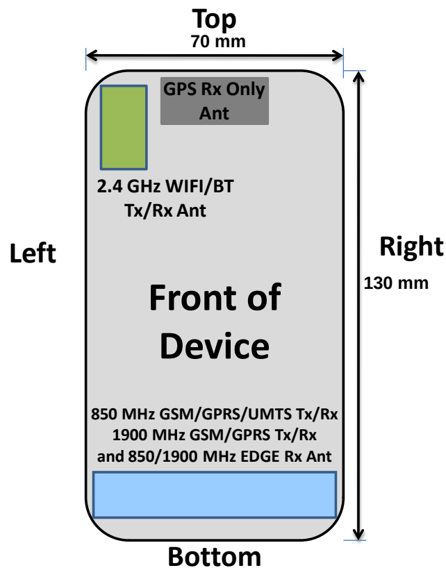
Figure F-1: DUT Antenna Locations
