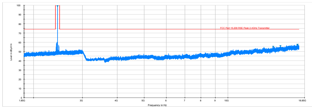
Plot 6-44. Radiated Spurious Plot above 1GHz (BT – Ch. 39, Ant. Pol. H)
