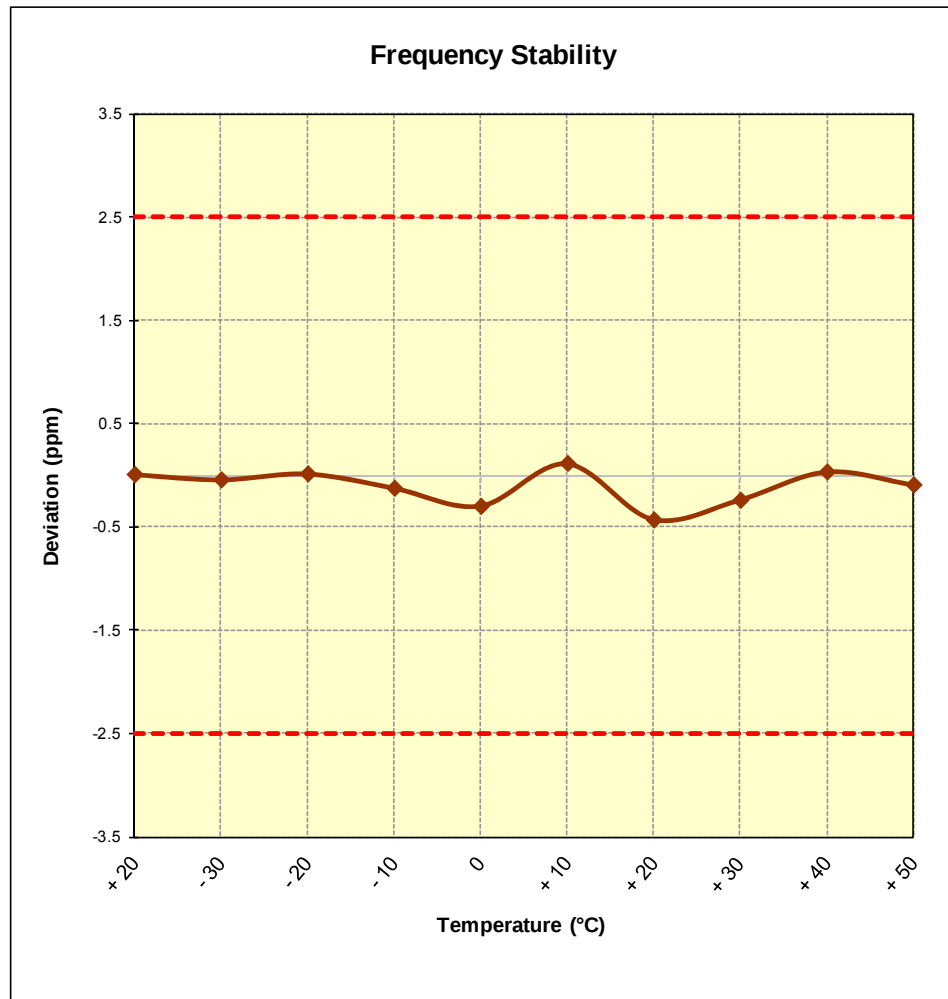
Figure 6-7. Frequency Stability Graph (Cellular CDMA Mode – Ch. 384)
