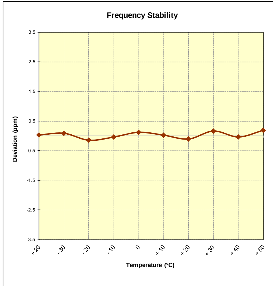
Figure 6-8. Frequency Stability Graph (PCS CDMA Mode – Ch. 600)
