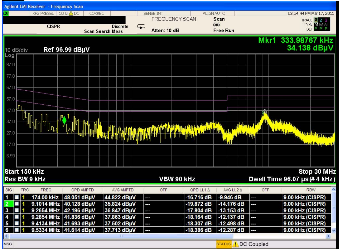
Plot 7-1. Line Conducted Plot (L1)
