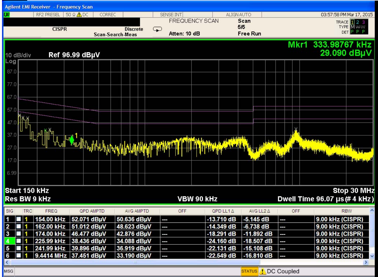
Plot 7-2. Line Conducted Plot (LN)
