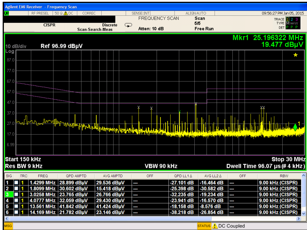
Plot 7-1. Line-Conducted Test Plot (L1)
