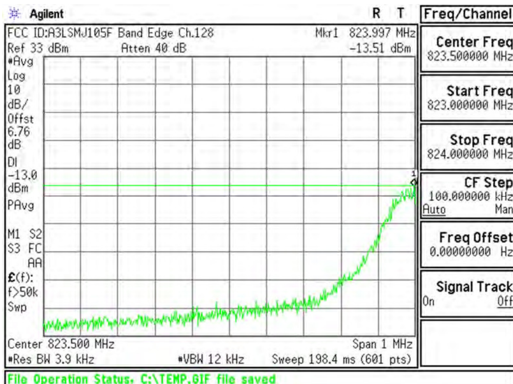
Plot 6-40. Lower Band Edge Plot (Cellular GSM Mode – Ch.128)
