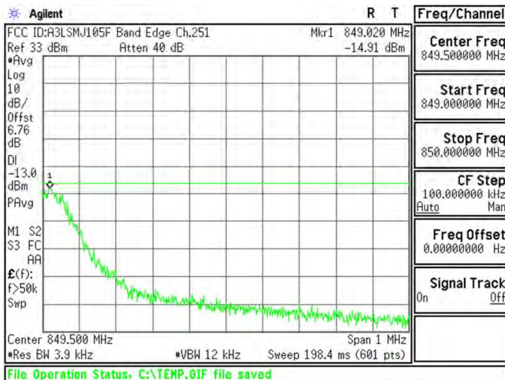
Plot 6-42. Upper Band Edge Plot (Cellular GSM Mode – Ch.251)
