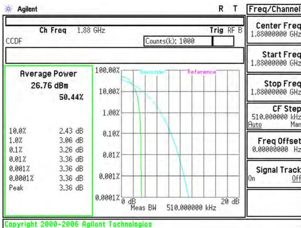
Plot 6-52. Peak-Average Ratio Plot (EDGE1900 Mode - Ch.661)
