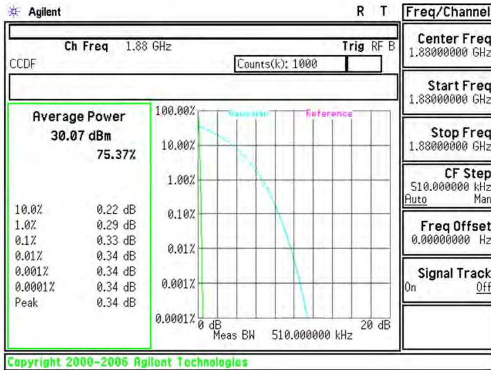
Plot 6-51. Peak-Average Ratio Plot (PCS GSM Mode - Ch.661)
