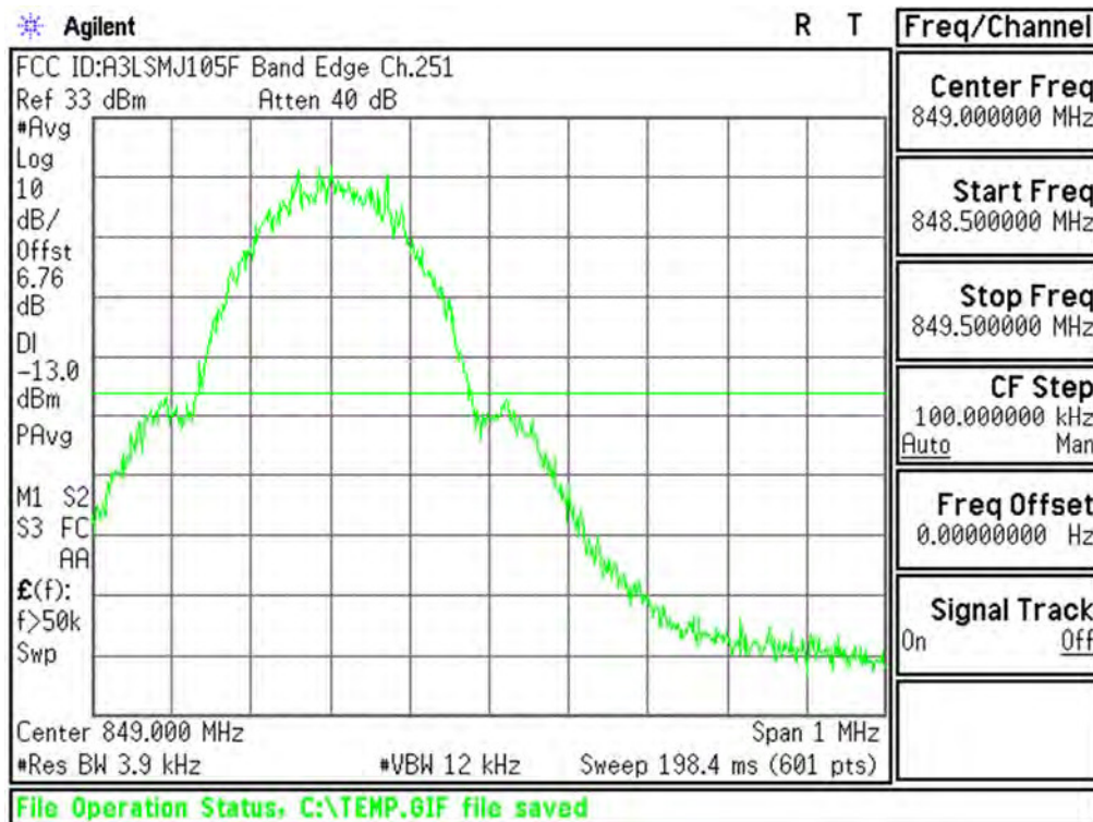
Plot 6-41. Upper Band Edge Plot (Cellular GSM Mode – Ch.251)
