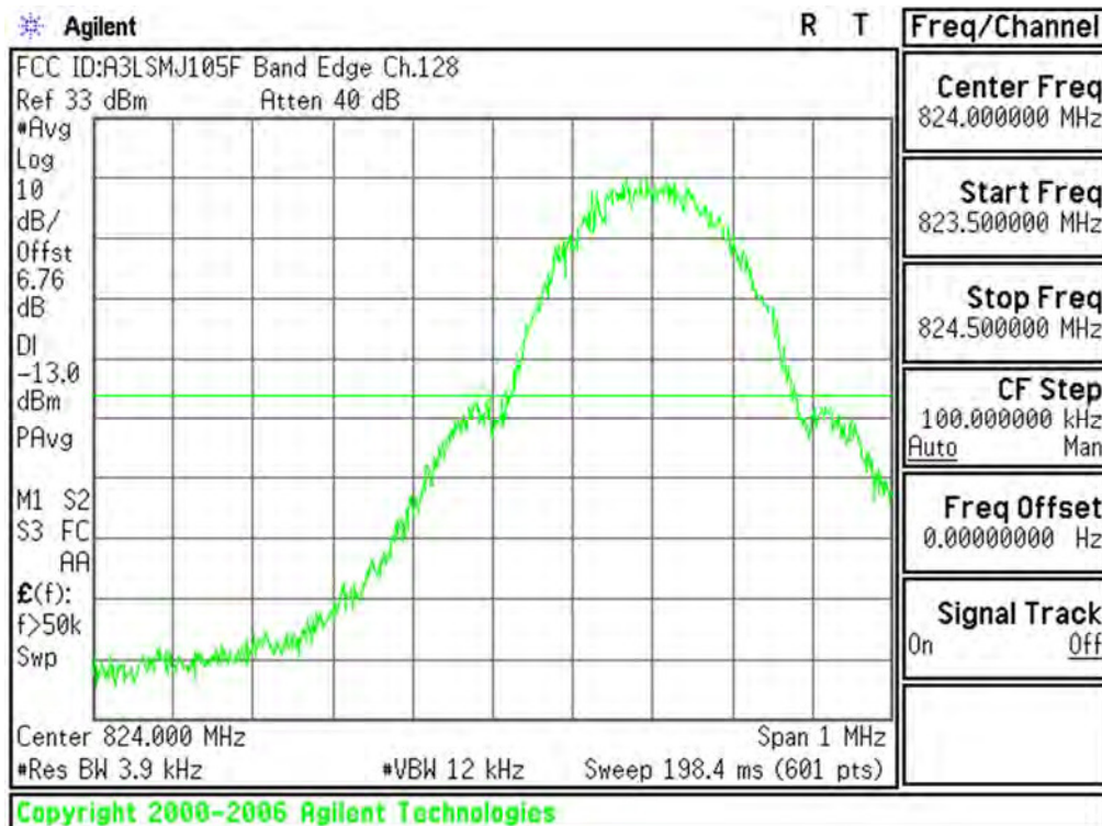
Plot 6-39. Lower Band Edge Plot (Cellular GSM Mode – Ch.128)
