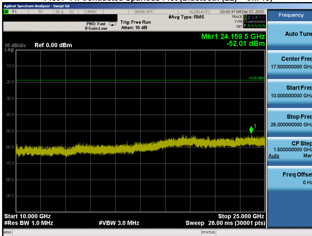
Plot 7-15. Conducted Spurious Plot (Bluetooth (LE) – Ch. 19)
