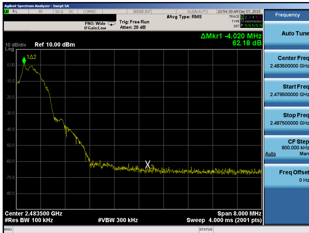
Plot 7-11. Band Edge Plot (Bluetooth (LE) – Ch. 39)
