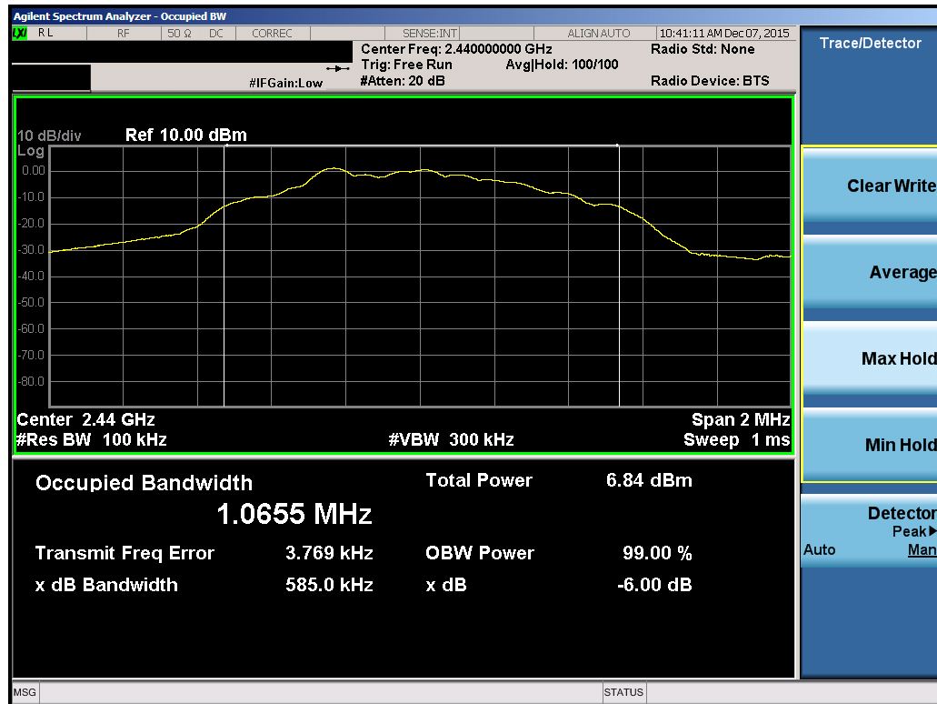
Plot 7-2. 6dB Bandwidth Plot (Bluetooth (LE) – Ch. 19)
