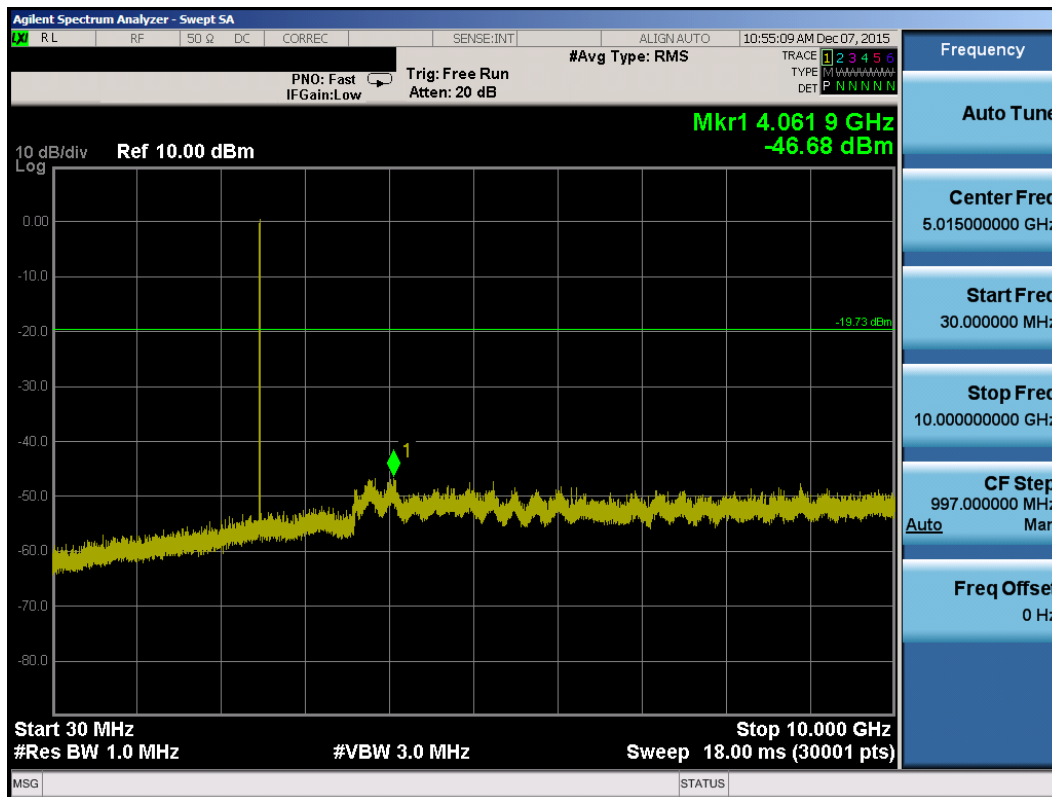
Plot 7-16. Conducted Spurious Plot (Bluetooth (LE) – Ch. 39)
