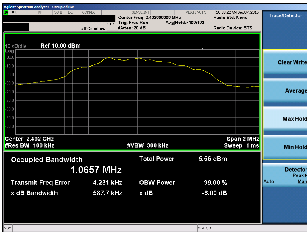
Plot 7-1. 6dB Bandwidth Plot (Bluetooth (LE) – Ch. 0)
