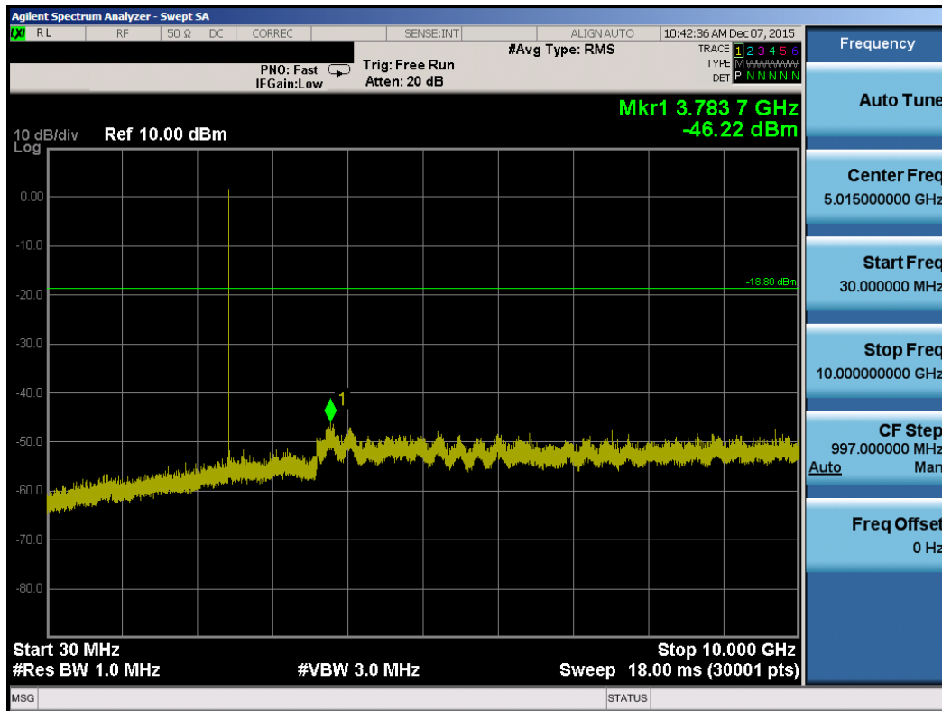
Plot 7-14. Conducted Spurious Plot (Bluetooth (LE) – Ch. 19)
