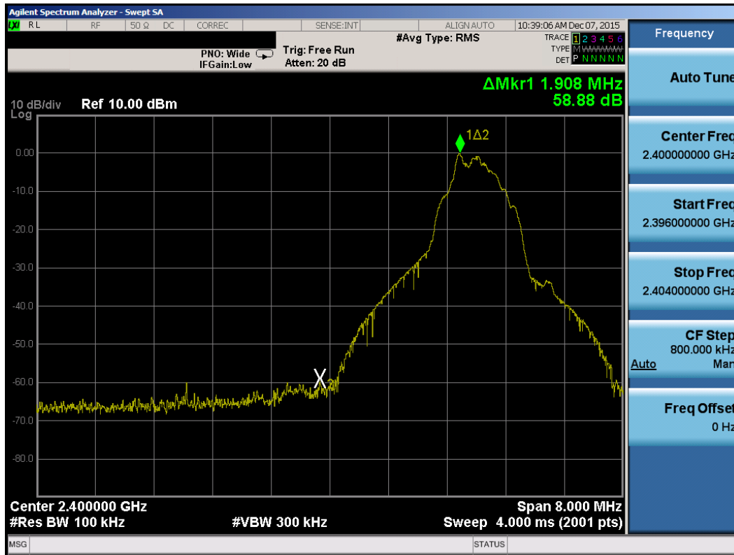
Plot 7-10. Band Edge Plot (Bluetooth (LE) – Ch. 0)
