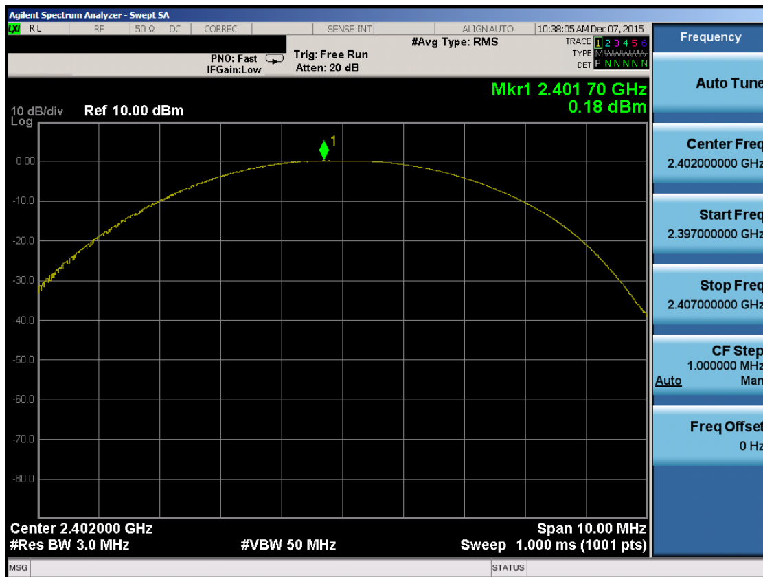
Plot 7-4. Peak Power Plot (Bluetooth (LE) – Ch. 0)
