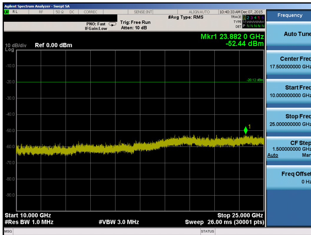
Plot 7-13. Conducted Spurious Plot (Bluetooth (LE) – Ch. 0)
