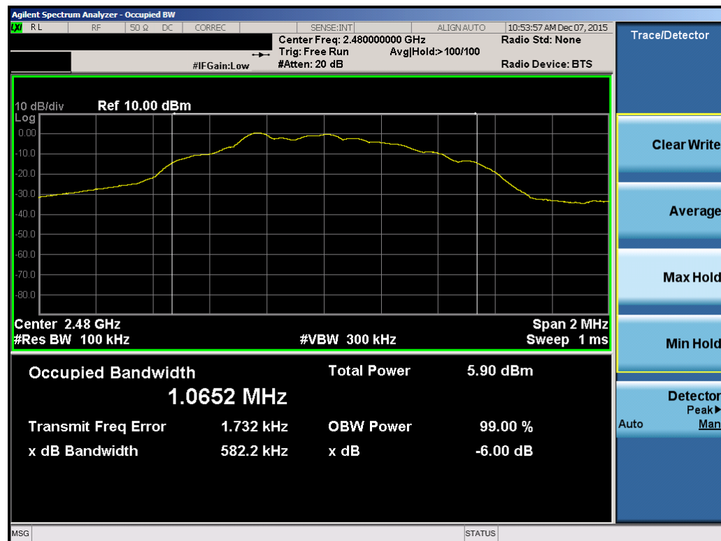
Plot 7-3. 6dB Bandwidth Plot (Bluetooth (LE) – Ch. 39)
