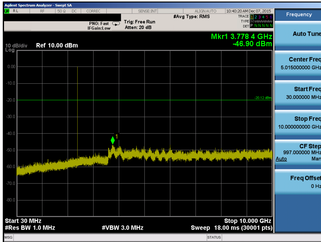
Plot 7-12. Conducted Spurious Plot (Bluetooth (LE) – Ch. 0)
