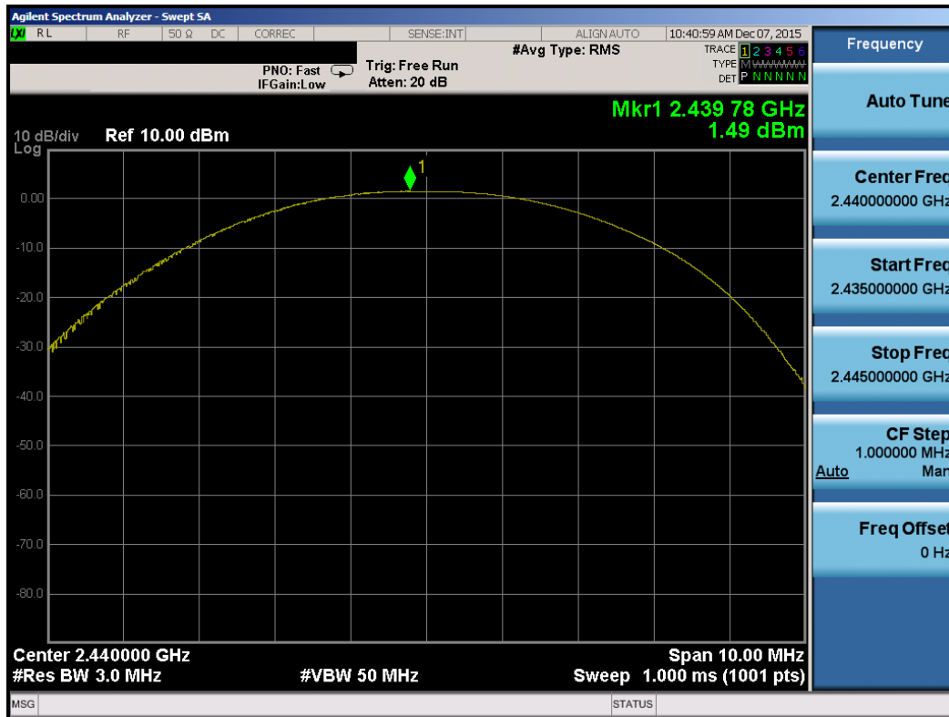
Plot 7-5. Peak Power Plot (Bluetooth (LE) – Ch. 19)
