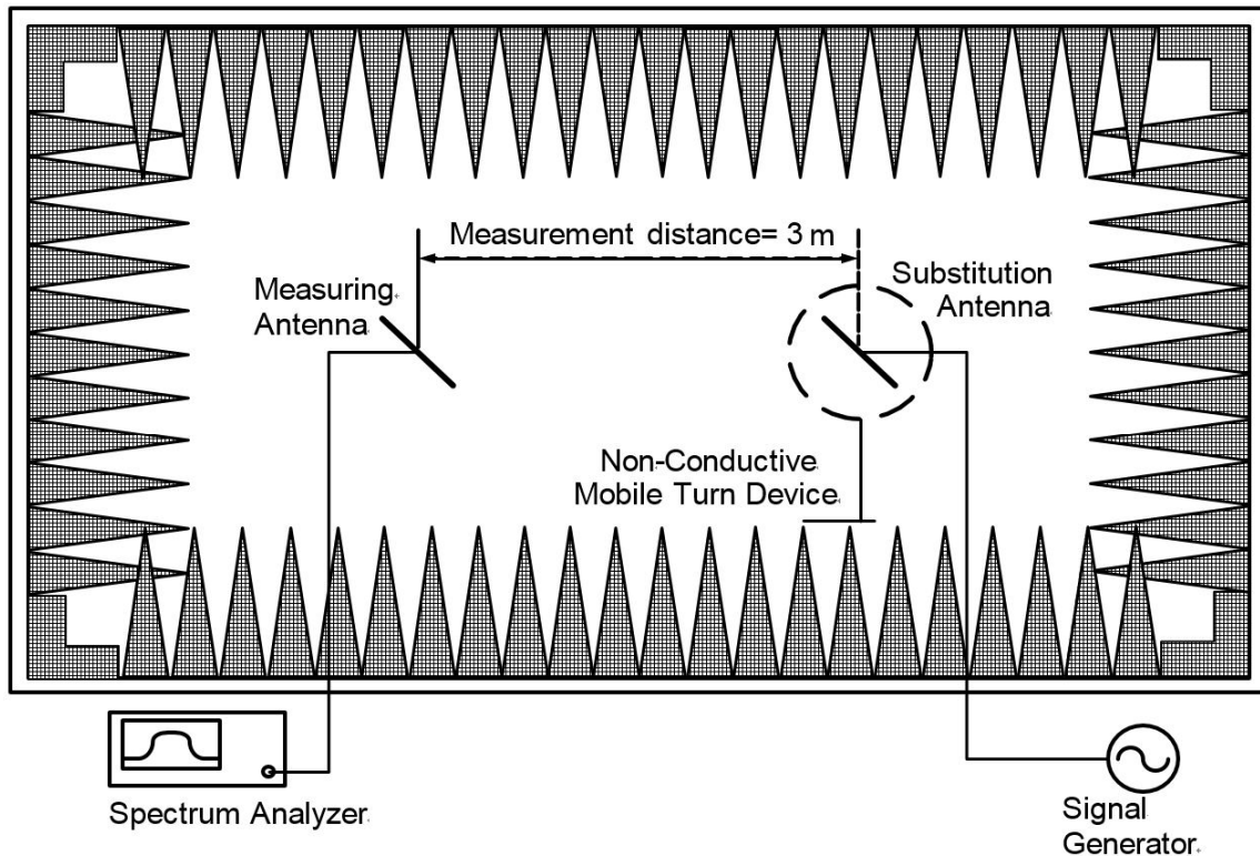
Figure 6-6. Test Instruments & Measurement Setup
