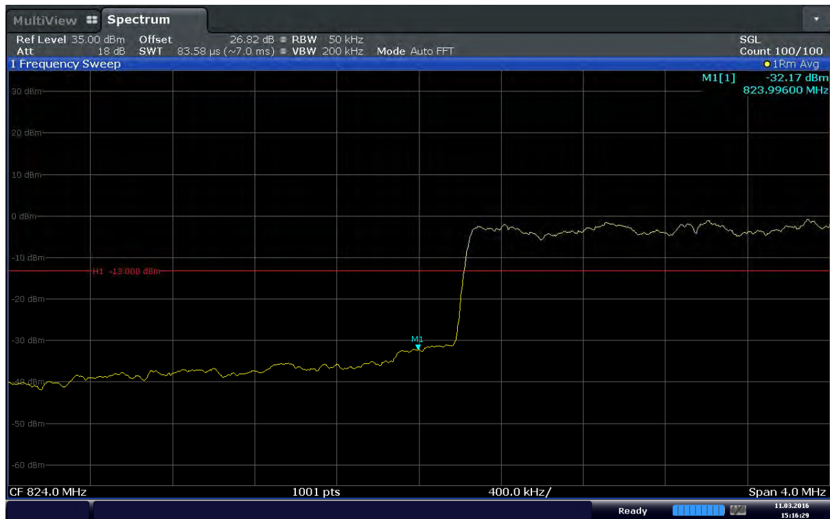
Plot 6-29. Lower Band Edge Plot (Band 5 – 5.0MHz – 16QAM – RB Size 25)
