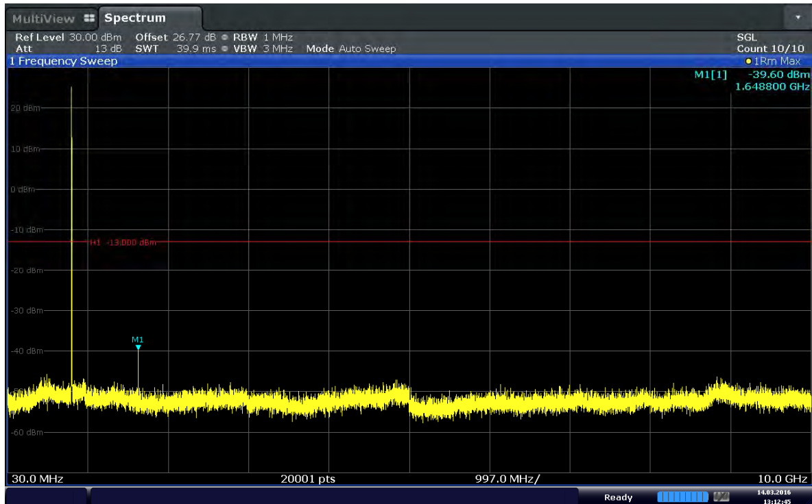
Plot 6-9. Conducted Spurious Plot (Band 5–1.4MHz–QPSK–RB Size 1–RB Offset 0–Ch.20407)
