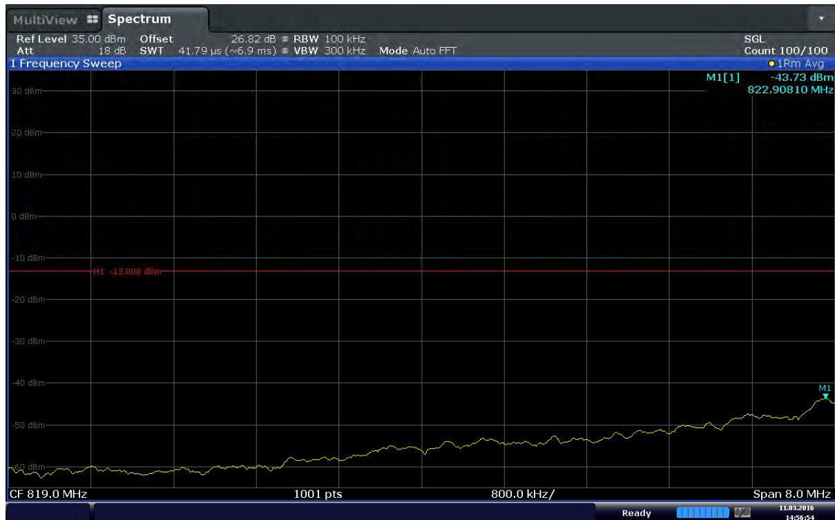
Plot 6-22. Extended Lower Band Edge Plot (Band5 – 1.4MHz – QPSK – RB Size 6)
