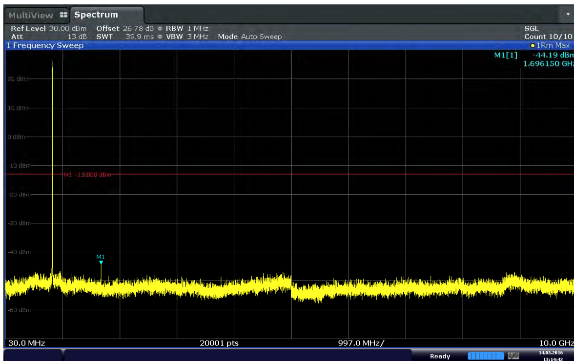
Plot 6-11. Conducted Spurious Plot (Band 5–1.4MHz–QPSK–RB Size 1–RB Offset 2– Ch.20643)
