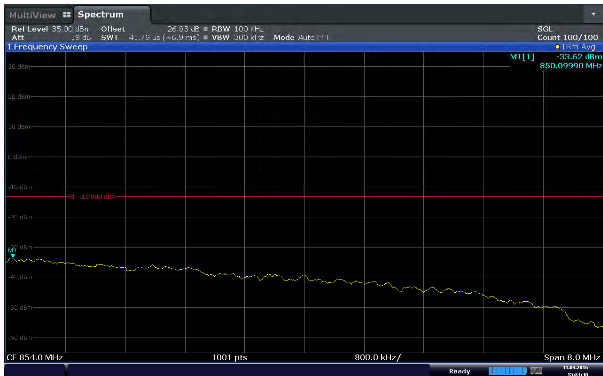
Plot 6-36. Upper Band Edge Plot (Band 5 – 10.0MHz – QPSK – RB Size 1 – RB Offset 50)
