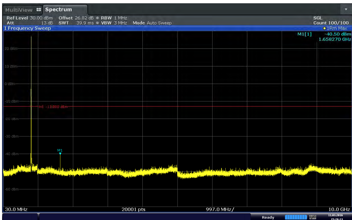
Plot 6-18. Conducted Spurious Plot (Band 5–10.0MHz–QPSK–RB Size 1–RB Offset 25– Ch.20450)
