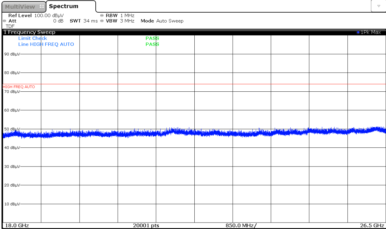
Plot 7-38. Radiated Spurious Plot above 18GHz (Pol. V)
