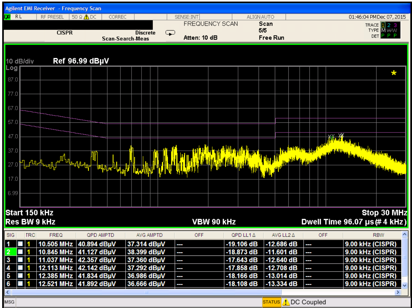
Plot 7-45. Line Conducted Plot with 802.11b (L1)
