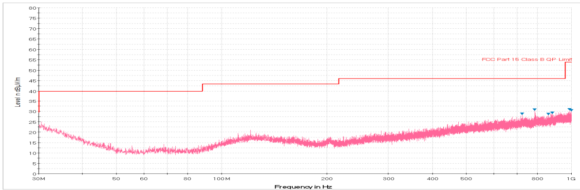
Plot 7-43. Radiated Spurious Plot below 1GHz (Pol. H)
