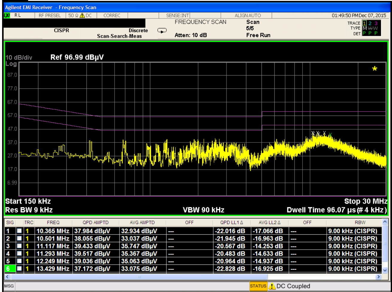
Plot 7-46. Line Conducted Plot with 802.11b (N)
