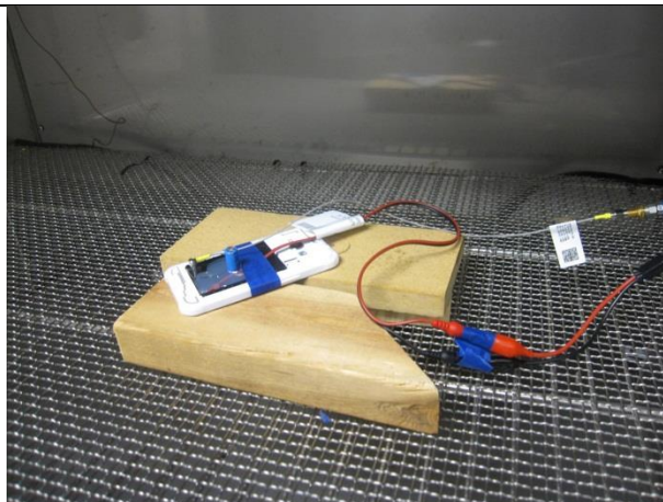
FREQUENCY STABILITY
