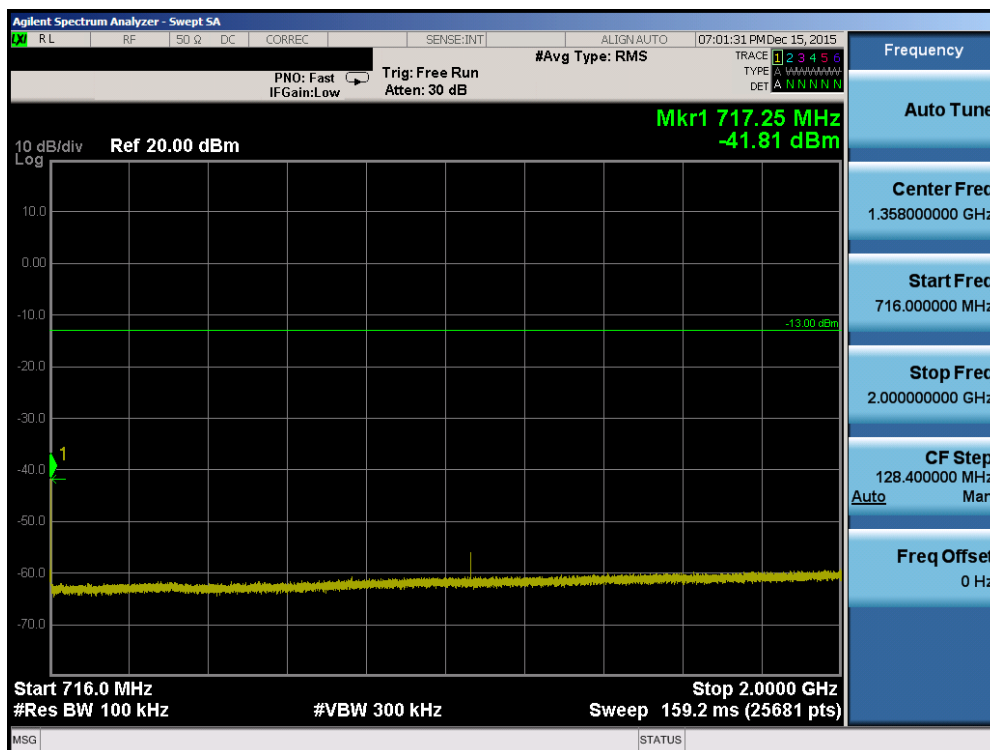
Plot 7-42. Conducted Spurious Plot (Band 12/17 – 10MHz QPSK – RB Size 1, RB Offset 0 – Low Channel)
