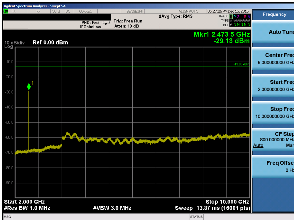
Plot 7-52. Conducted Spurious Plot (Band 5 – 1.4MHz QPSK – RB Size 1, RB Offset 0 – Low Channel)
