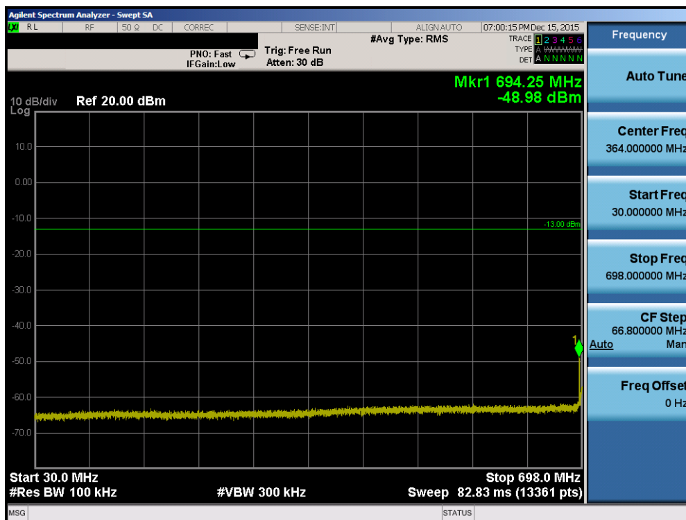
Plot 7-44. Conducted Spurious Plot (Band 12/17 – 10MHz QPSK – RB Size 1, RB Offset 0 – Mid Channel)
