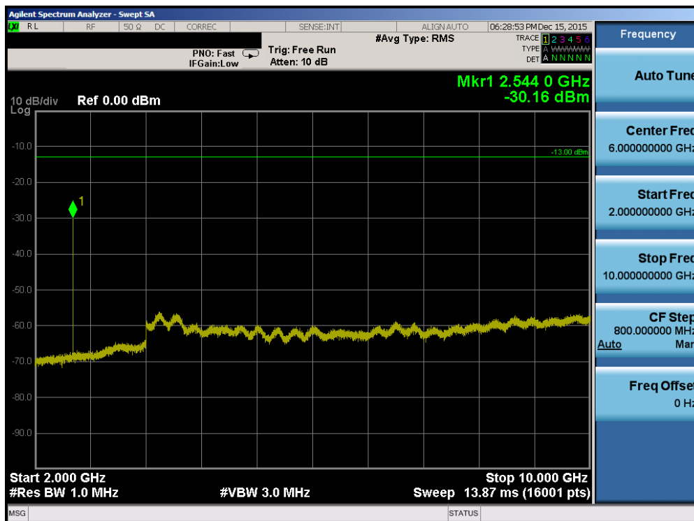
Plot 7-58. Conducted Spurious Plot (Band 5 – 1.4MHz QPSK – RB Size 1, RB Offset 0 – High Channel)
