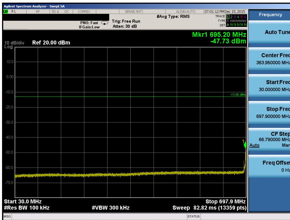
Plot 7-41. Conducted Spurious Plot (Band 12/17 – 10MHz QPSK – RB Size 1, RB Offset 0 – Low Channel)
