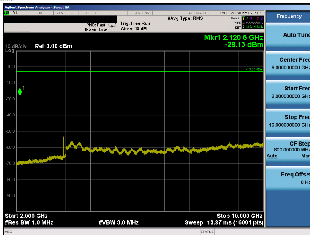
Plot 7-49. Conducted Spurious Plot (Band 12/17 – 10MHz QPSK – RB Size 1, RB Offset 0 – High Channel)
