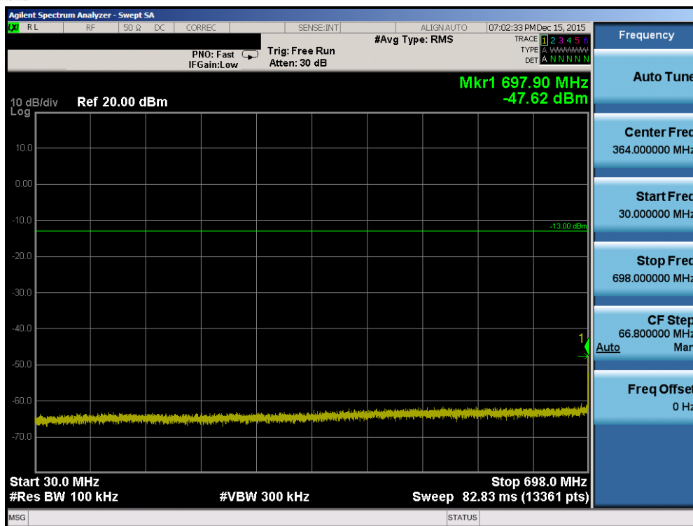
Plot 7-47. Conducted Spurious Plot (Band 12/17 – 10MHz QPSK – RB Size 1, RB Offset 0 – High Channel)
