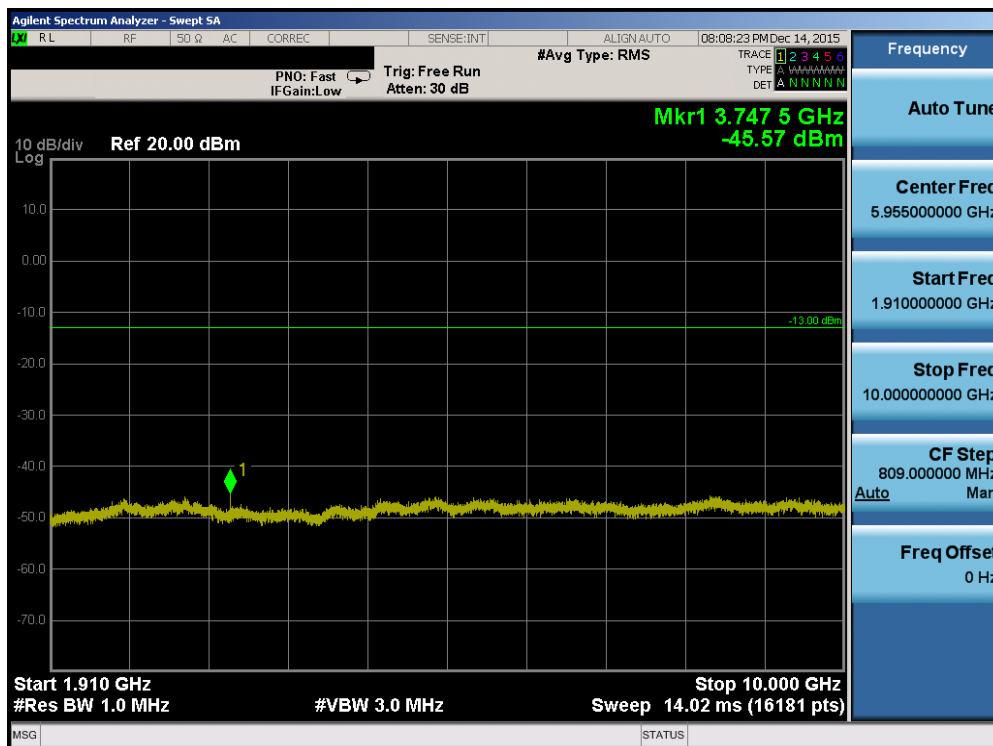
Plot 7-72. Conducted Spurious Plot (Band 2 – 15.0MHz QPSK – RB Size 1, RB Offset 0 – Mid Channel)
