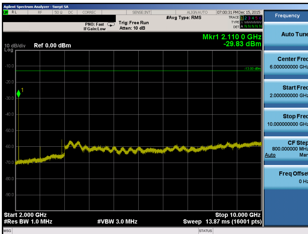
Plot 7-46. Conducted Spurious Plot (Band 12/17 – 10MHz QPSK – RB Size 1, RB Offset 0 – Mid Channel)
