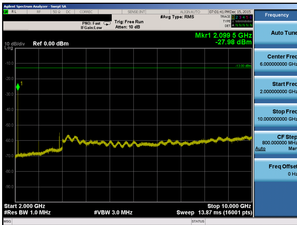
Plot 7-43. Conducted Spurious Plot (Band 12/17 – 10MHz QPSK – RB Size 1, RB Offset 0 – Low Channel)
