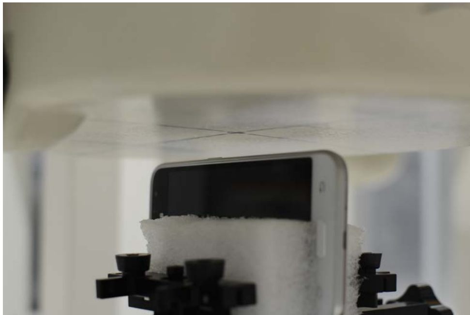
SAR Test Setup Photo 10 – Right Edge (10 mm)
