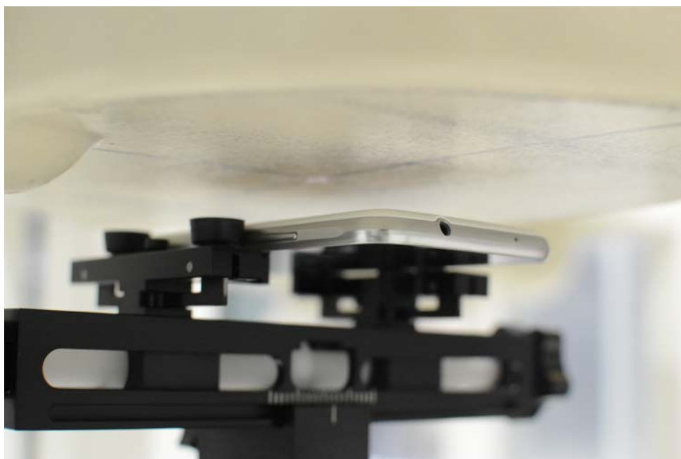
SAR Test Setup Photo 6 – Back Side (15 mm)
