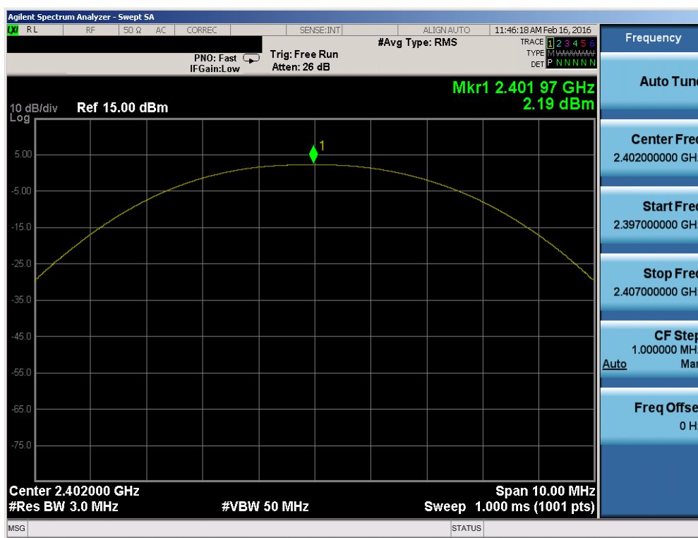
Plot 7-4. Peak Power Plot (Bluetooth (LE) – Ch. 0)
