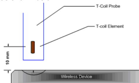
Figure 5-10 Measurement Distance
