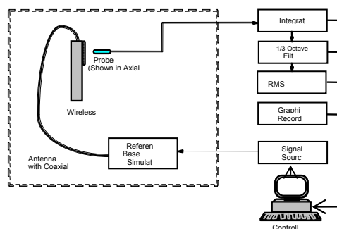
Figure 5-12 Audio Magnetic Field Test Setup
