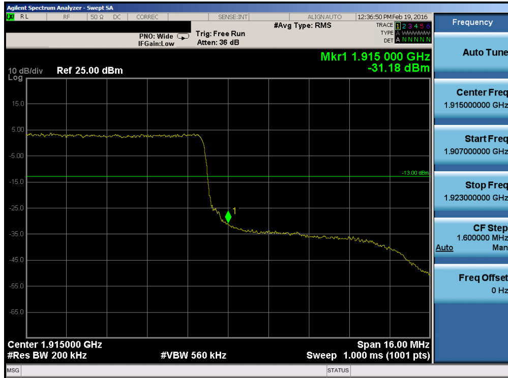
Plot 7-90. Upper Band Edge Plot (Band 25 – 20.0MHz QPSK – RB Size 100)
