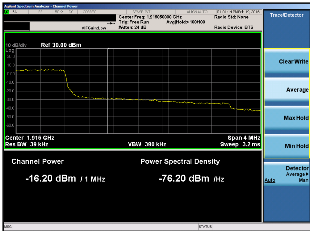
Plot 7-75. Upper Extended Band Edge Plot (Band 25 – 3.0MHz QPSK – RB Size 15)
