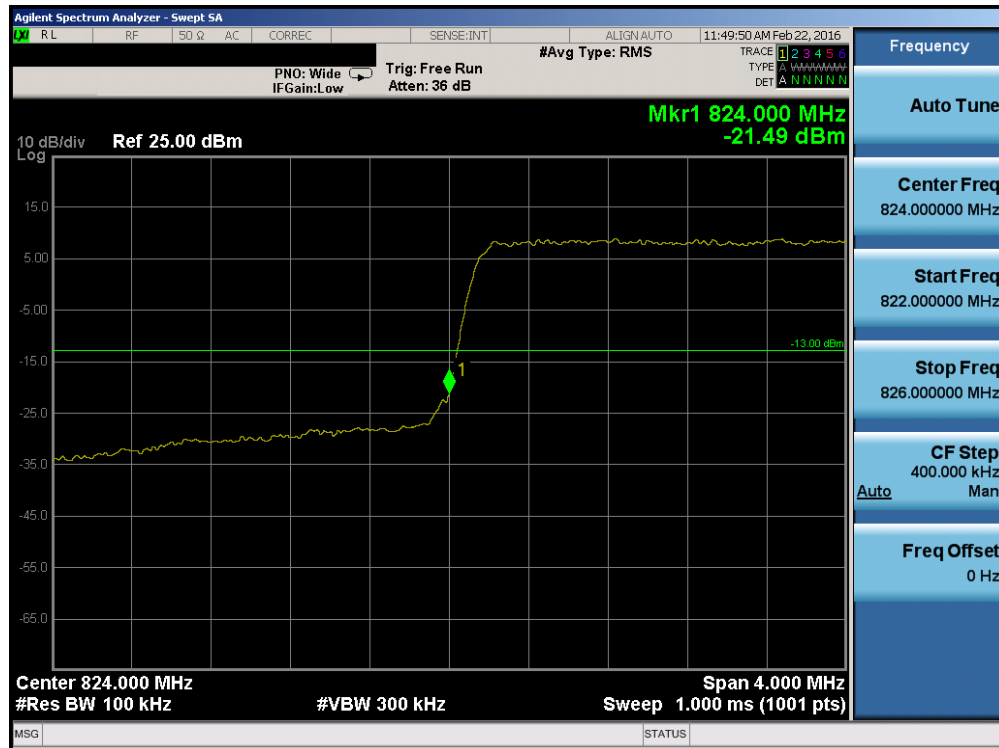
Plot 7-60. Lower Band Edge Plot (Band 26 – 3.0MHz QPSK – RB Size 15)
