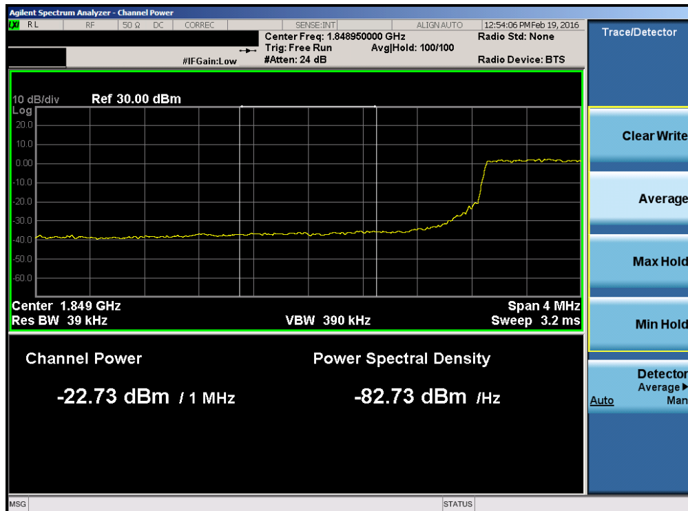
Plot 7-77. Lower Extended Band Edge Plot (Band 25 – 5.0MHz QPSK – RB Size 25)
