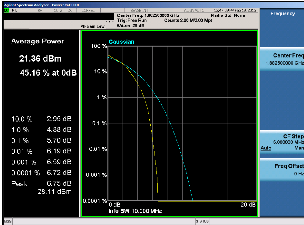
Plot 7-107. PAR Plot (Band 25 – 10.0MHz 16-QAM – RB Size 50)
