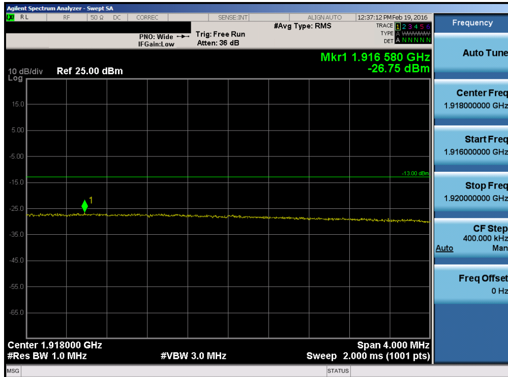
Plot 7-91. Upper Extended Band Edge Plot (Band 25 – 20.0MHz QPSK – RB Size 100)
