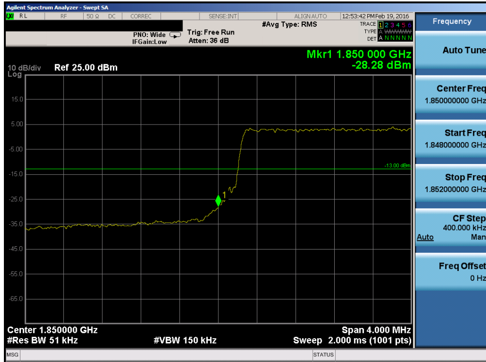
Plot 7-76. Lower Band Edge Plot (Band 25 – 5.0MHz QPSK – RB Size 25)
