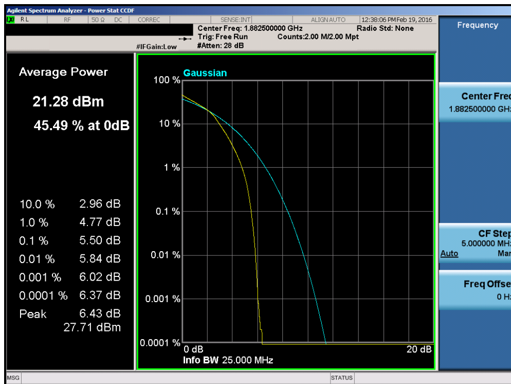
Plot 7-109. PAR Plot (Band 25 – 15.0MHz 16-QAM – RB Size 75)
