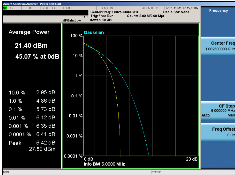
Plot 7-105. PAR Plot (Band 25 – 5.0MHz 16-QAM – RB Size 25)
