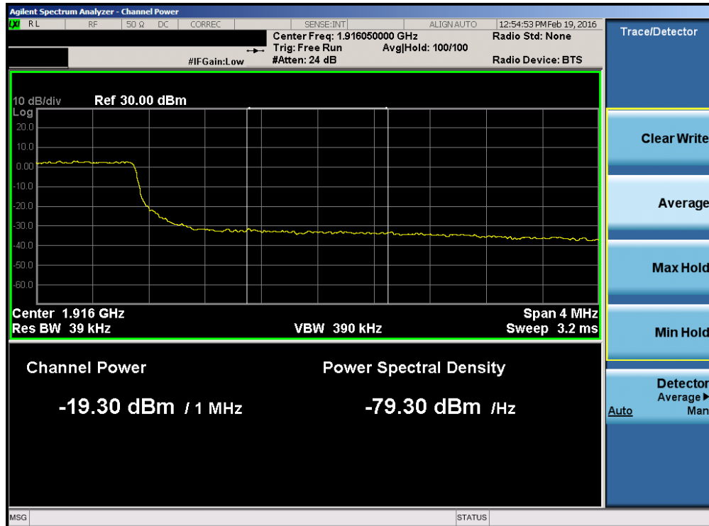
Plot 7-79. Upper Extended Band Edge Plot (Band 25 – 5.0MHz QPSK – RB Size 25)
