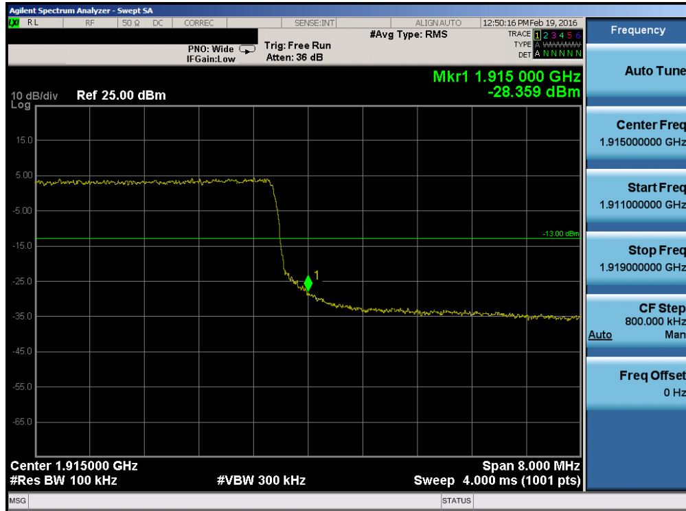
Plot 7-82. Upper Band Edge Plot (Band 25 – 10.0MHz QPSK – RB Size 50)
