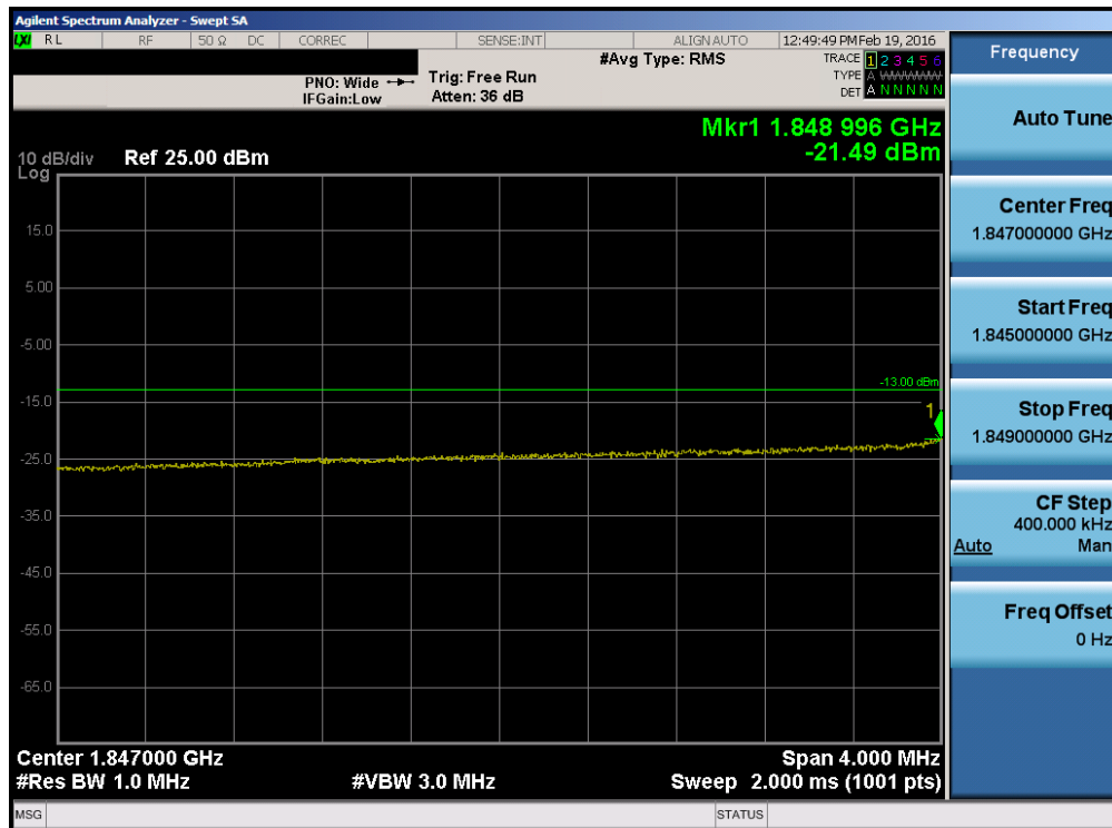
Plot 7-81. Lower Extended Band Edge Plot (Band 25 – 10.0MHz QPSK – RB Size 50)
