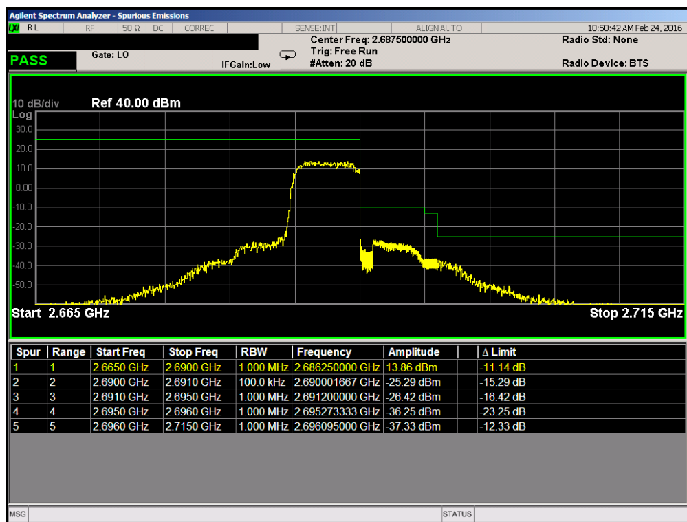
Plot 7-93. Upper ACP Plot (Band 41 – 5.0MHz QPSK – RB Size 25)
