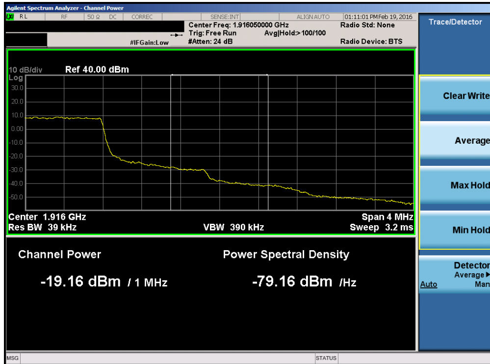
Plot 7-71. Upper Extended Band Edge Plot (Band 25 – 1.4MHz QPSK – RB Size 6)
