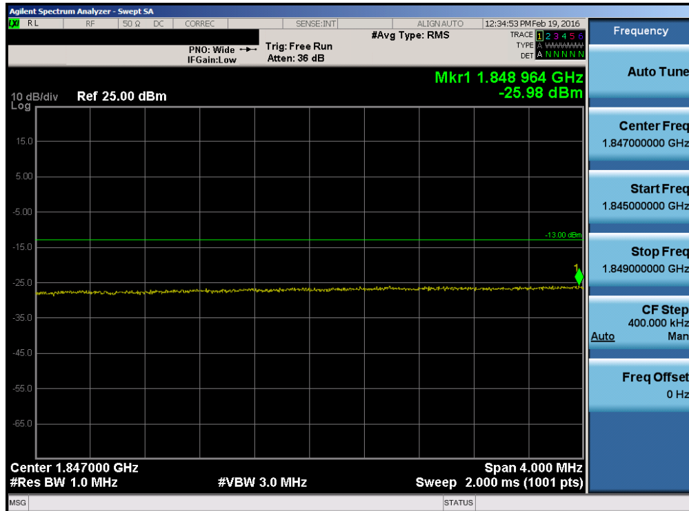
Plot 7-89. Lower Extended Band Edge Plot (Band 25 – 20.0MHz QPSK – RB Size 100)
