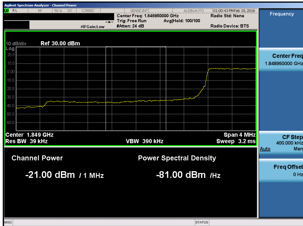
Plot 7-73. Lower Extended Band Edge Plot (Band 25 – 3.0MHz QPSK – RB Size 15)
