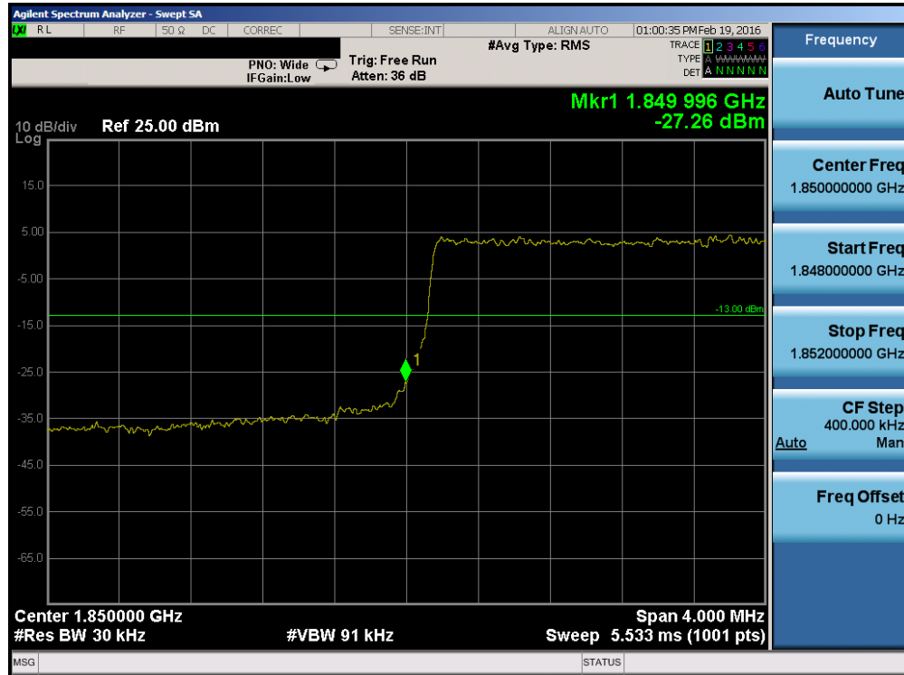
Plot 7-72. Lower Band Edge Plot (Band 25 – 3.0MHz QPSK – RB Size 15)
