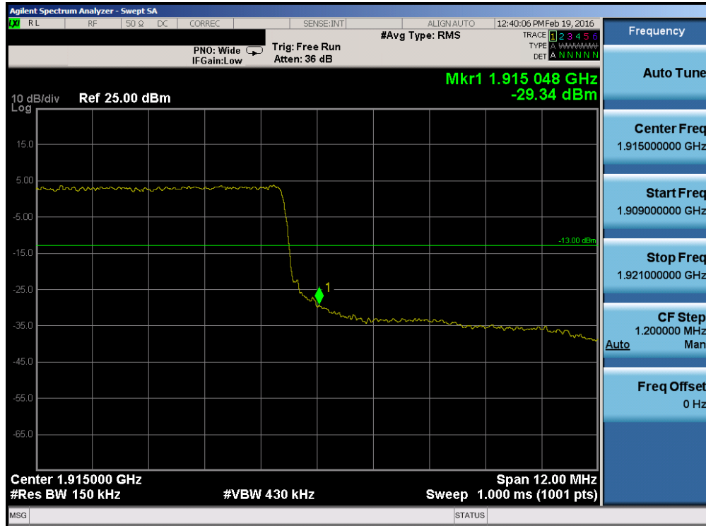
Plot 7-86. Upper Band Edge Plot (Band 25 – 15.0MHz QPSK – RB Size 75)
