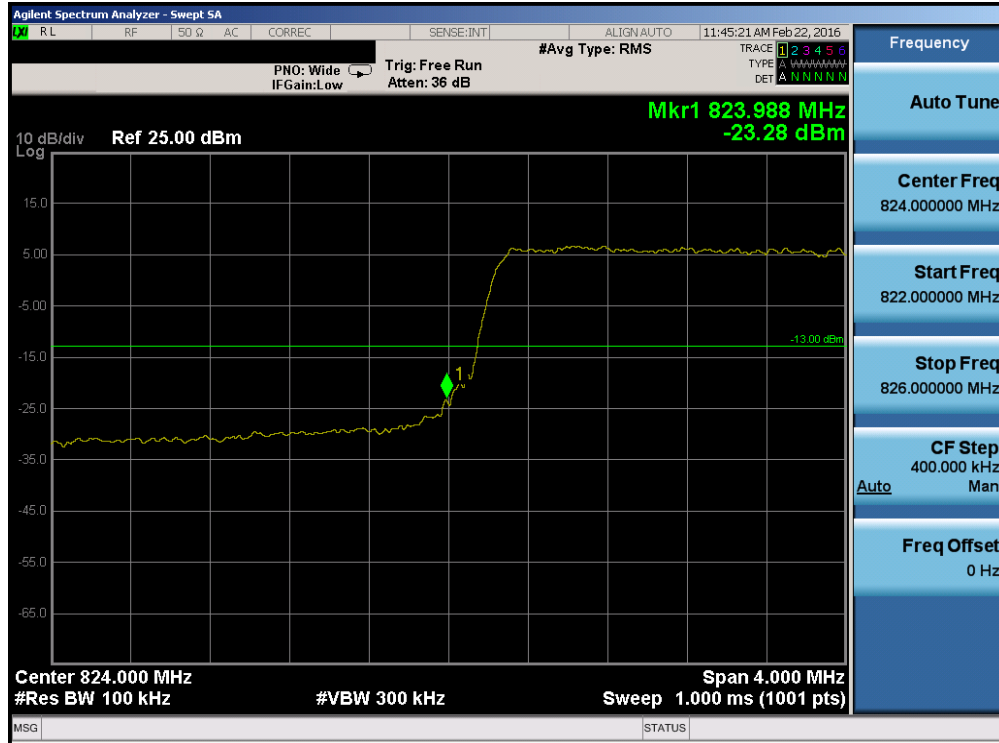
Plot 7-62. Lower Band Edge Plot (Band 26 – 5.0MHz QPSK – RB Size 25)
