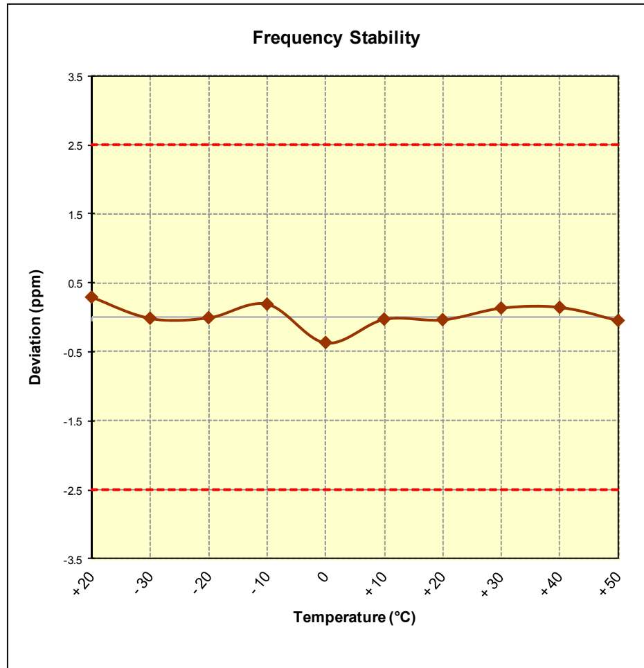
Figure 7-8. Frequency Stability Graph (Band 26)
