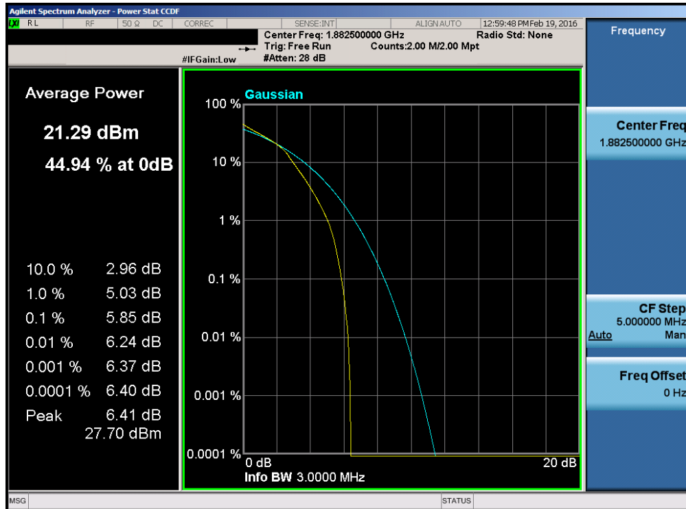
Plot 7-103. PAR Plot (Band 25 – 3.0MHz 16-QAM – RB Size 15)
