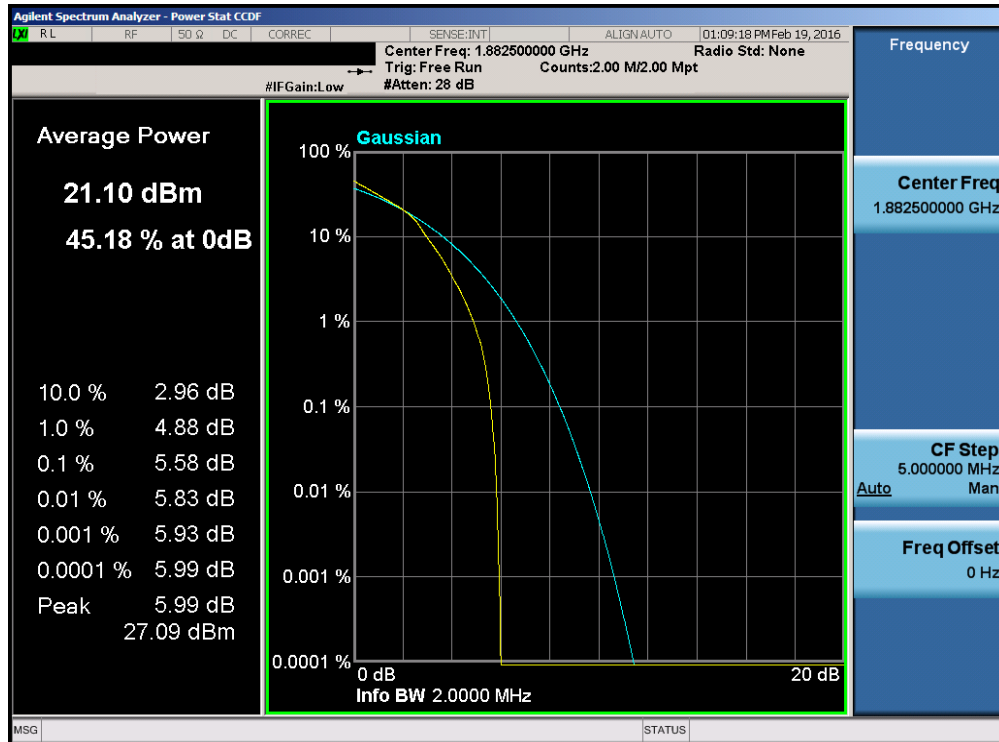
Plot 7-101. PAR Plot (Band 25 – 1.4MHz 16-QAM – RB Size 6)
