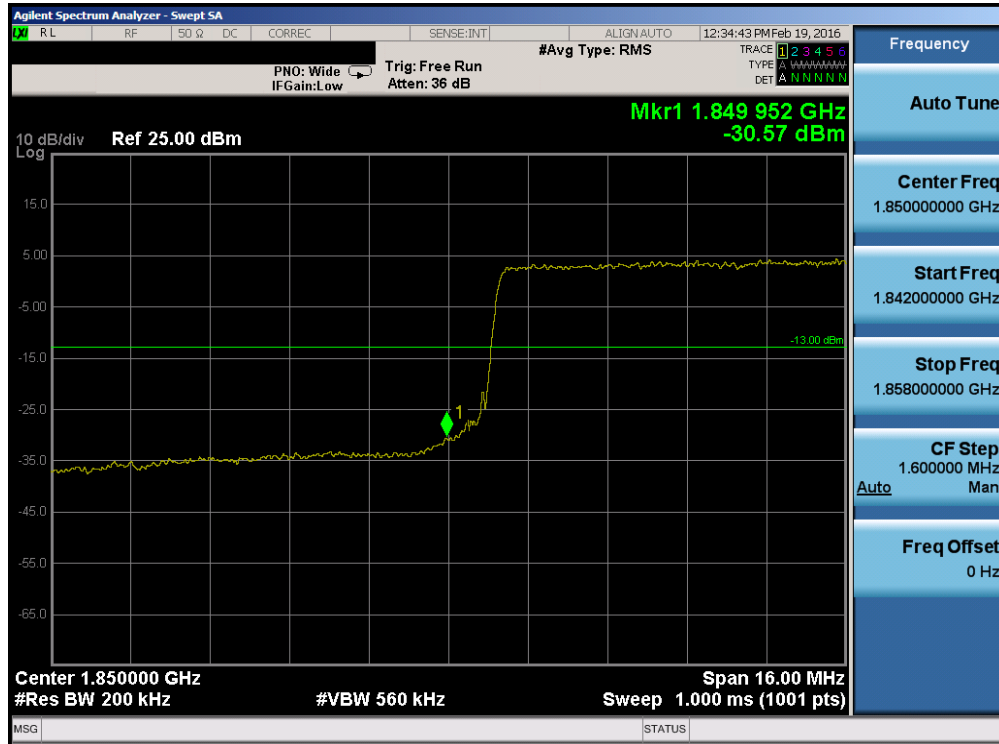
Plot 7-88. Lower Band Edge Plot (Band 25 – 20.0MHz QPSK – RB Size 100)
