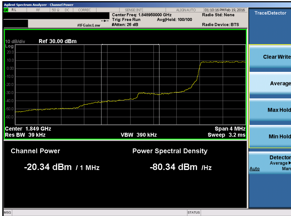
Plot 7-69. Lower Extended Band Edge Plot (Band 25 – 1.4MHz QPSK – RB Size 6)
