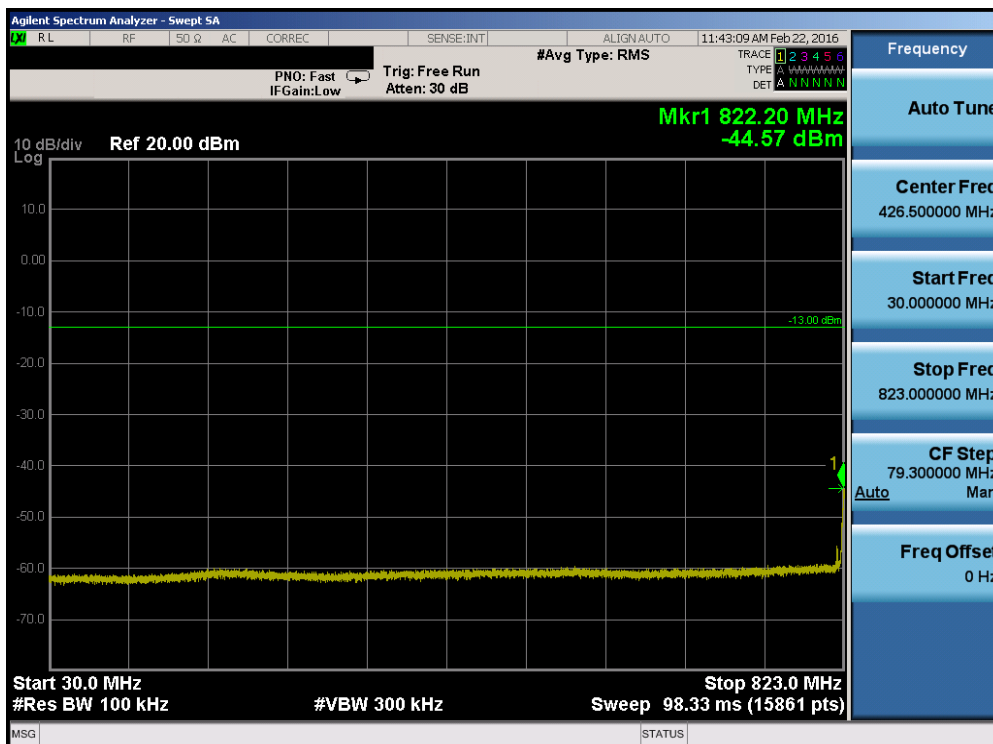
Plot 7-31. Conducted Spurious Plot (Band 26 – 5.0MHz QPSK – RB Size 1, RB Offset 0 – Low Channel)
