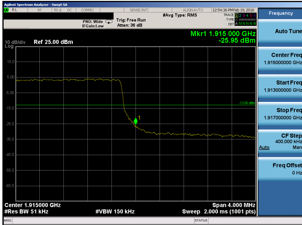
Plot 7-78. Upper Band Edge Plot (Band 25 – 5.0MHz QPSK – RB Size 25)
