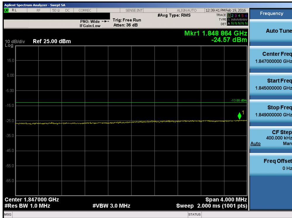
Plot 7-85. Lower Extended Band Edge Plot (Band 25 – 15.0MHz QPSK – RB Size 75)
