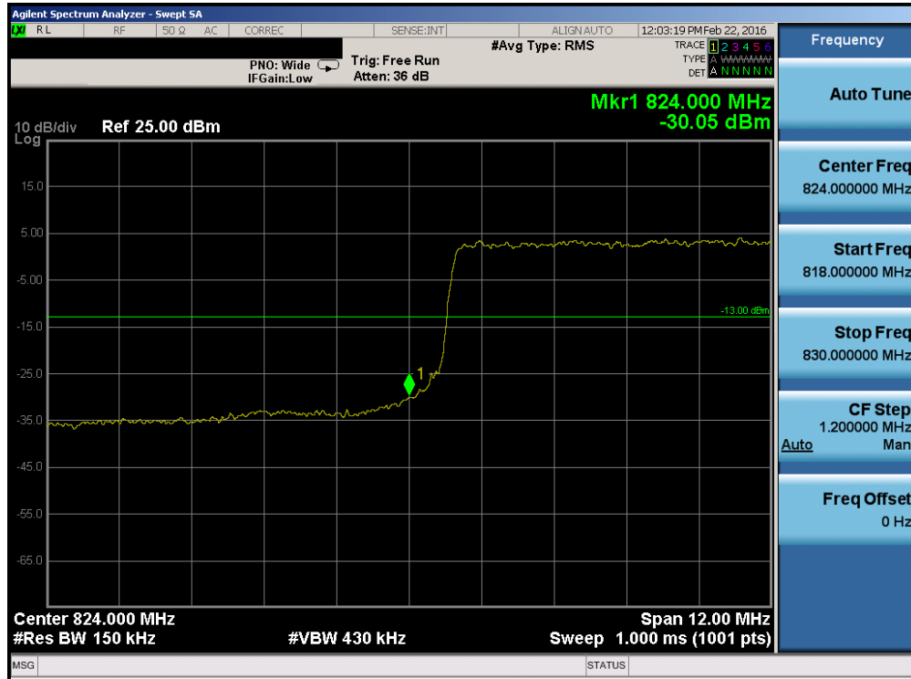
Plot 7-66. Lower Band Edge Plot (Band 26 – 15.0MHz QPSK – RB Size 75)
