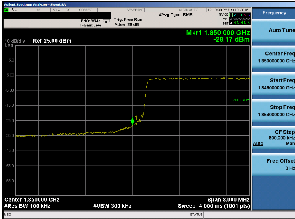
Plot 7-80. Lower Band Edge Plot (Band 25 – 10.0MHz QPSK – RB Size 50)
