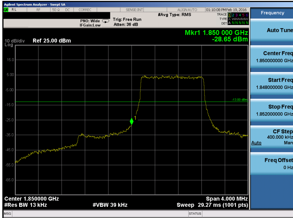
Plot 7-68. Lower Band Edge Plot (Band 25 – 1.4MHz QPSK – RB Size 6)
