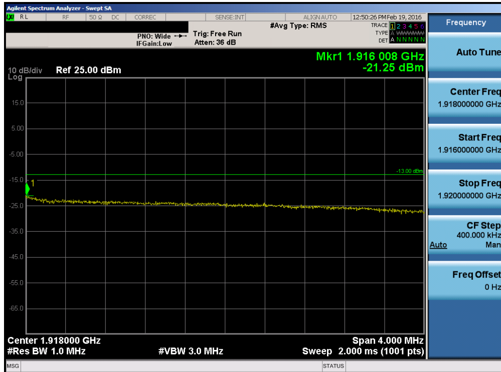
Plot 7-83. Upper Extended Band Edge Plot (Band 25 – 10.0MHz QPSK – RB Size 50)
