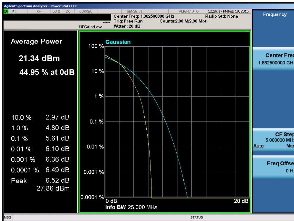
Plot 7-111. PAR Plot (Band 25 – 20.0MHz 16-QAM – RB Size 100)
