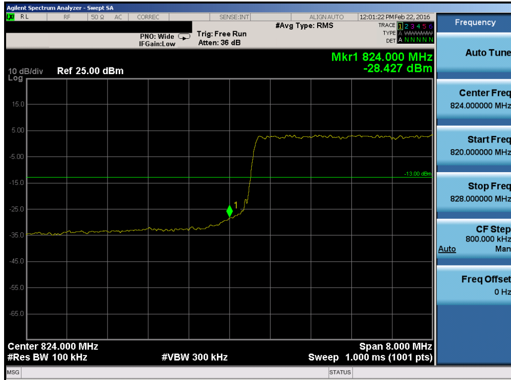
Plot 7-64. Lower Band Edge Plot (Band 26 – 10.0MHz QPSK – RB Size 50)
