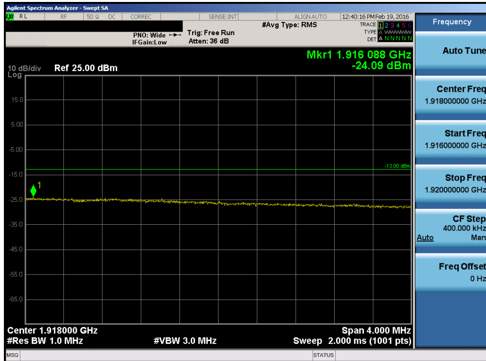
Plot 7-87. Upper Extended Band Edge Plot (Band 25 – 15.0MHz QPSK – RB Size 75)
