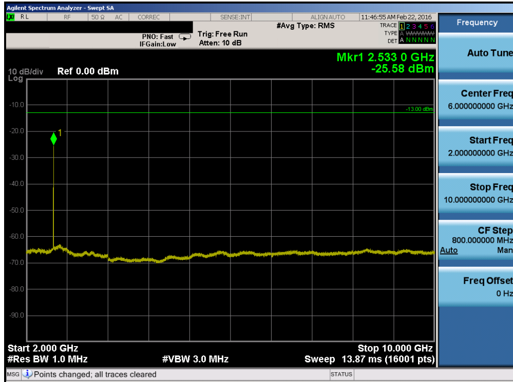
Plot 7-39. Conducted Spurious Plot (Band 26 – 5.0MHz QPSK – RB Size 1, RB Offset 0 – High Channel)
