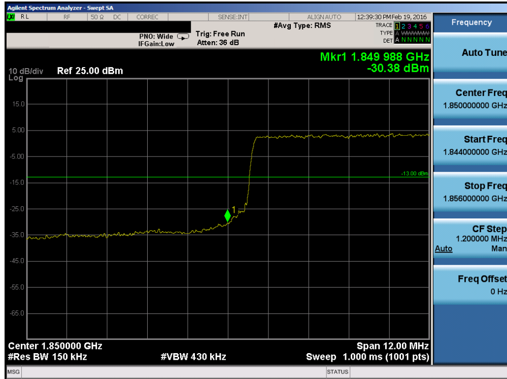
Plot 7-84. Lower Band Edge Plot (Band 25 – 15.0MHz QPSK – RB Size 75)
