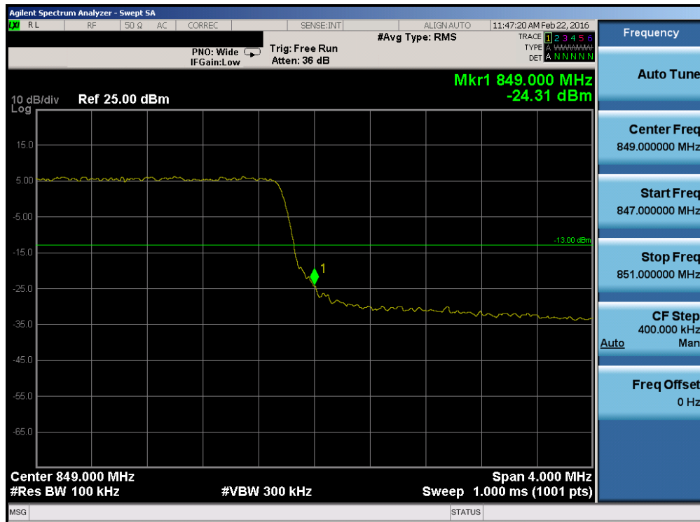
Plot 7-63. Upper Band Edge Plot (Band 26 – 5.0MHz QPSK – RB Size 25)
