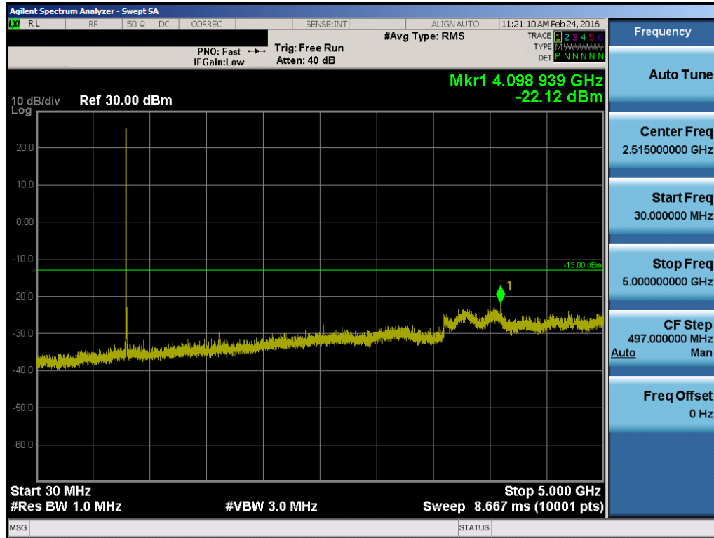
Plot 7-15. Conducted Spurious Plot (10 MHz QPSK – RB Size 1, RB Offset 0)
