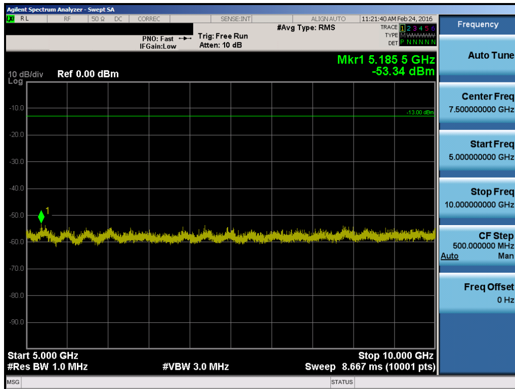
Plot 7-16. Conducted Spurious Plot (10 MHz QPSK – RB Size 1, RB Offset 0)
