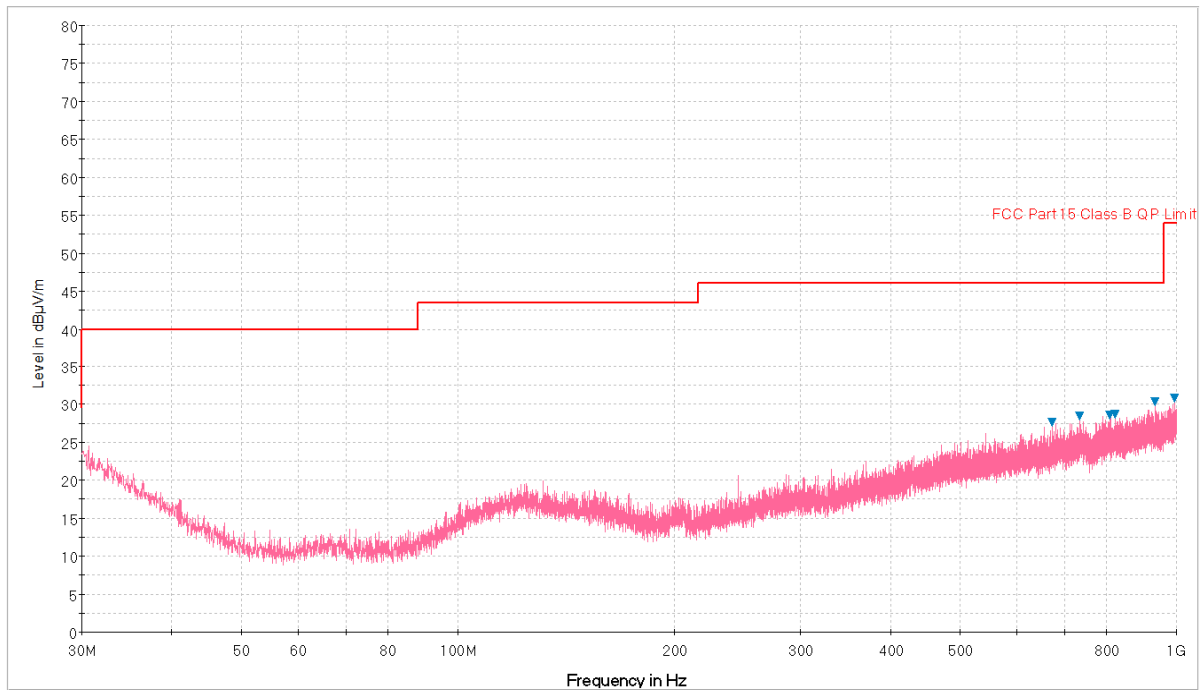
Plot 7-46. Radiated Spurious Plot below 1GHz (Pol. V)
