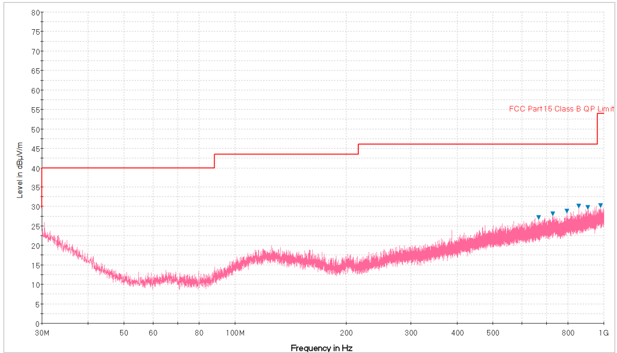
Plot 7-45. Radiated Spurious Plot below 1GHz (Pol. H)
