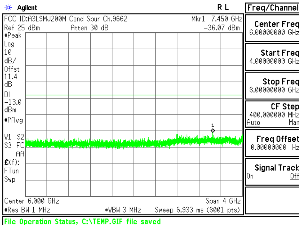
Plot 6-55. Conducted Spurious Plot (PCS WCDMA Mode - Ch.9262(DL9662))
