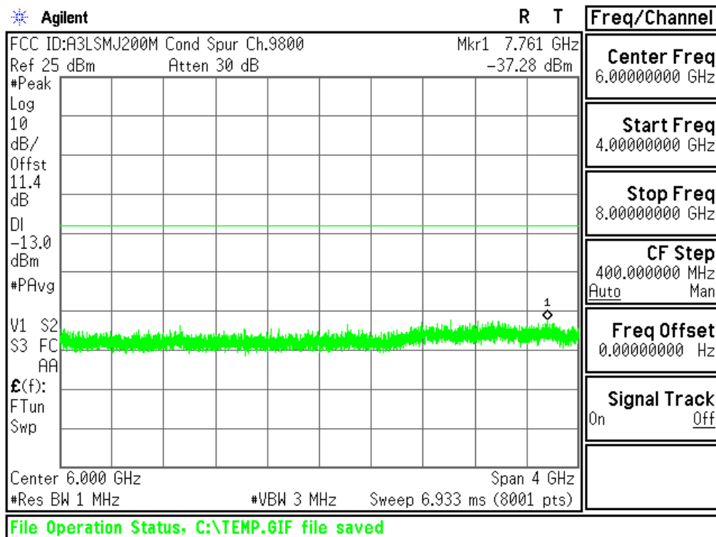
Plot 6-60. Conducted Spurious Plot (PCS WCDMA Mode - Ch.9400(DL9800))
