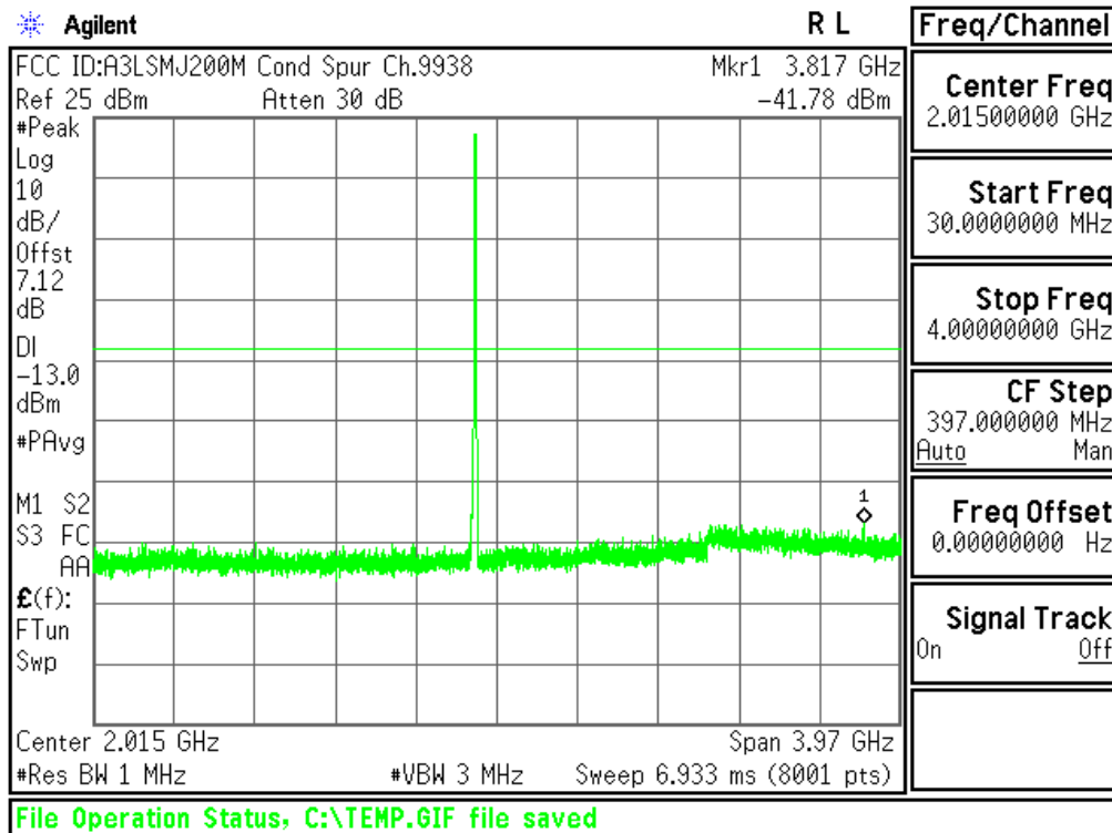
Plot 6-64. Conducted Spurious Plot (PCS WCDMA Mode - Ch.9538(DL9938))
