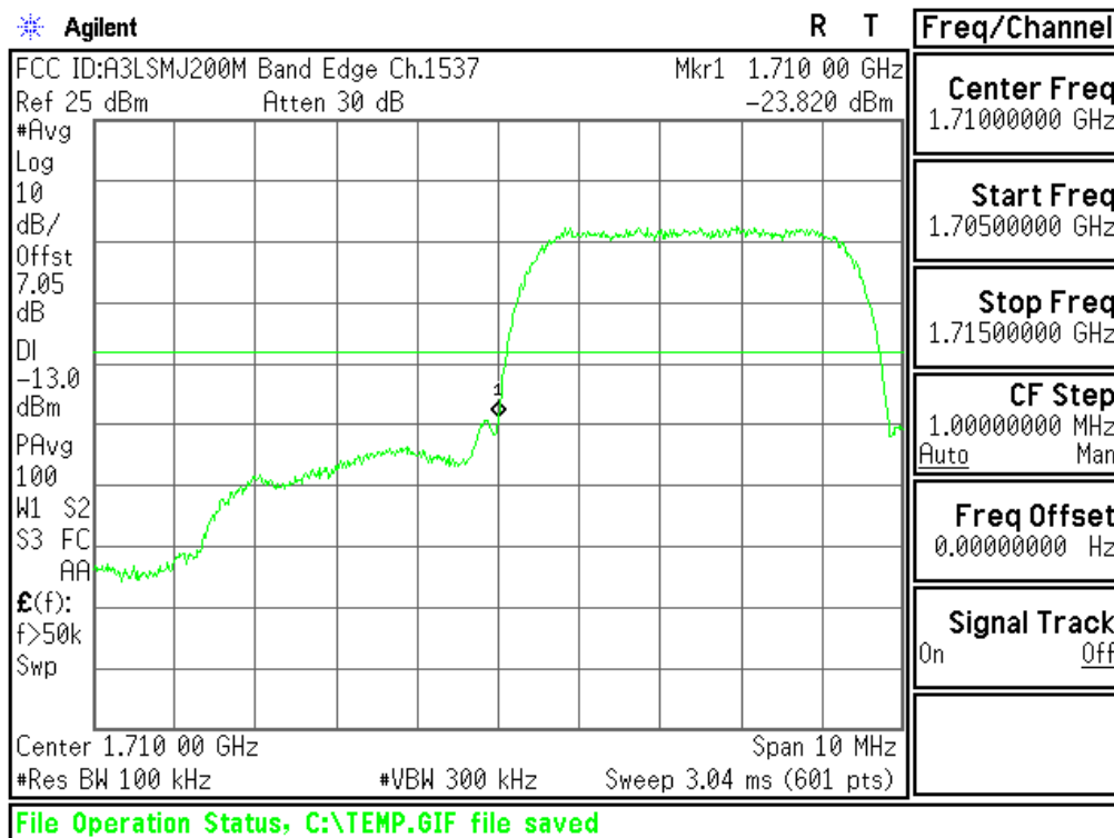
Plot 6-81. Lower Band Edge Plot (AWS WCDMA Mode - Ch.1312(DL1537))
