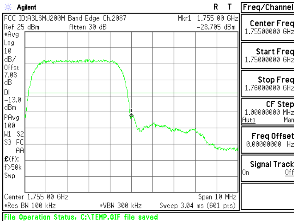
Plot 6-83. Upper Band Edge Plot (AWS WCDMA Mode - Ch.1862(DL2087))
