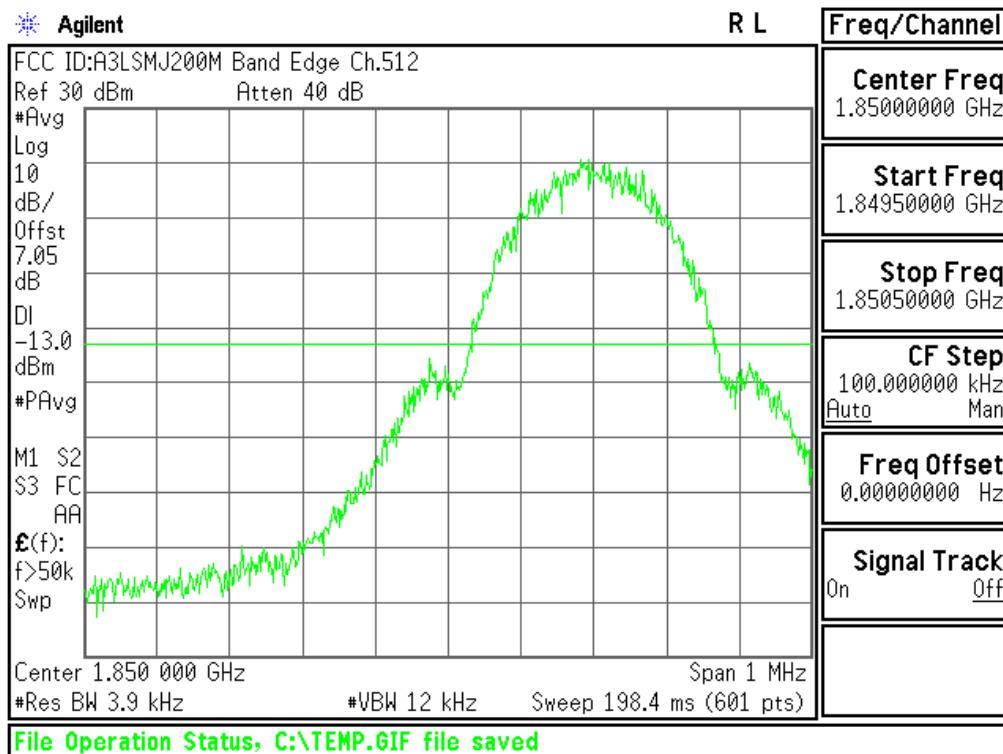
Plot 6-73. Lower Band Edge Plot (PCS GSM Mode – Ch.512)
