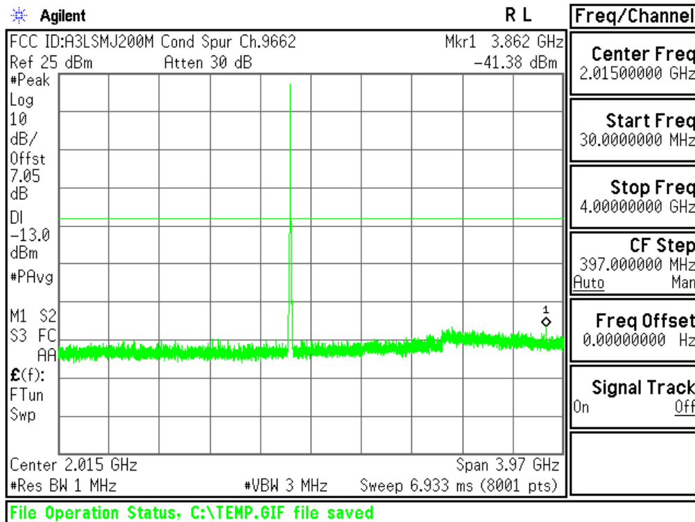
Plot 6-54. Conducted Spurious Plot (PCS WCDMA Mode - Ch.9262(DL9662))
