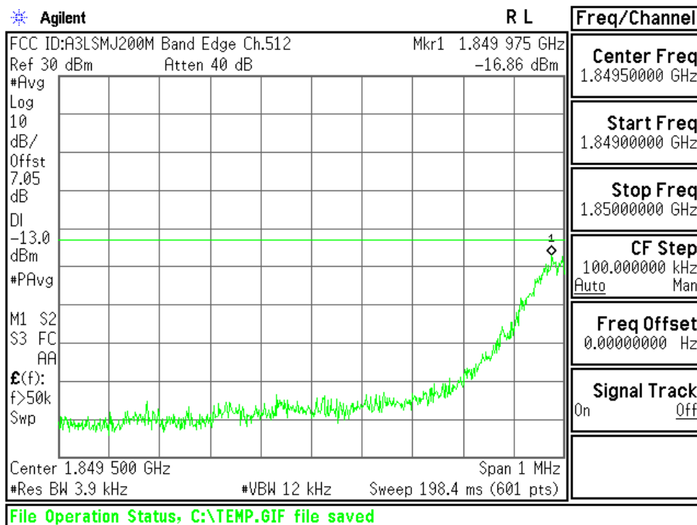
Plot 6-74. Lower Band Edge Plot (PCS GSM Mode – Ch.512)
