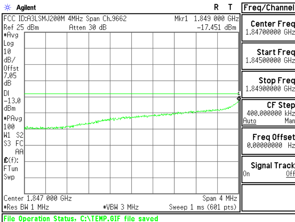
Plot 6-86. Extended Lower Band Edge Plot (PCS WCDMA Mode - Ch.9262(DL9662))
