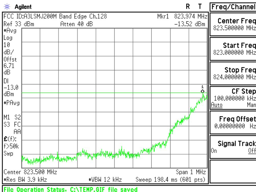
Plot 6-70. Lower Band Edge Plot (Cellular GSM Mode – Ch.128)
