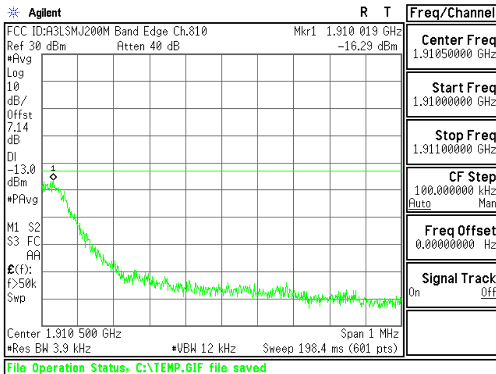
Plot 6-76. Upper Band Edge Plot (PCS GSM Mode – Ch.810)
