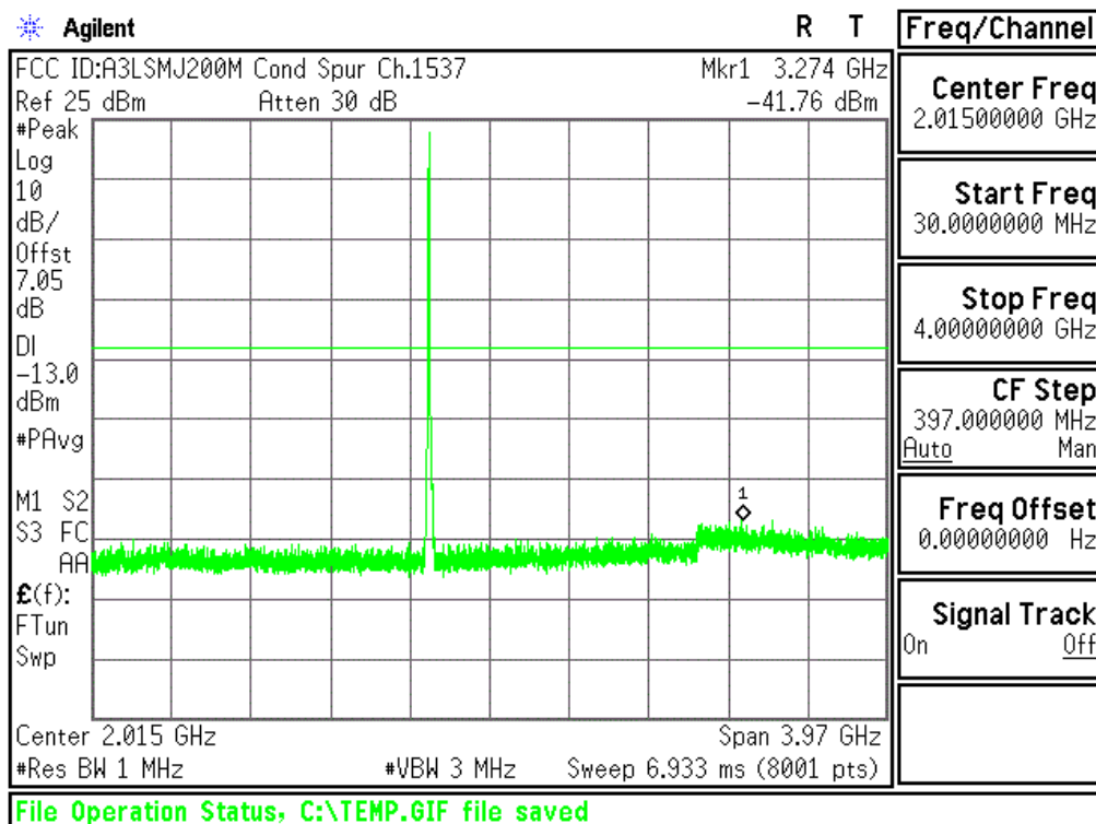
Plot 6-39. Conducted Spurious Plot (AWS WCDMA Mode - Ch.1312(DL1537))
