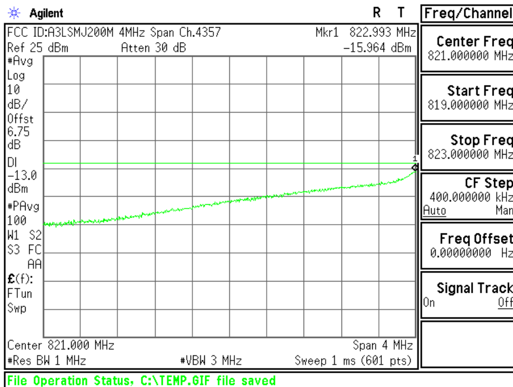
Plot 6-78. Extended Lower Band Edge Plot (Cellular WCDMA Mode - Ch.4132(DL4357))
