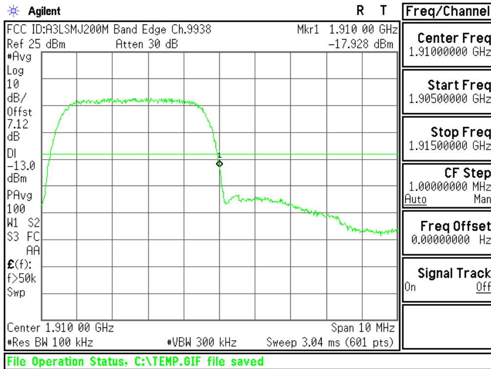
Plot 6-87. Upper Band Edge Plot (PCS WCDMA Mode - Ch.9538(DL9938))
