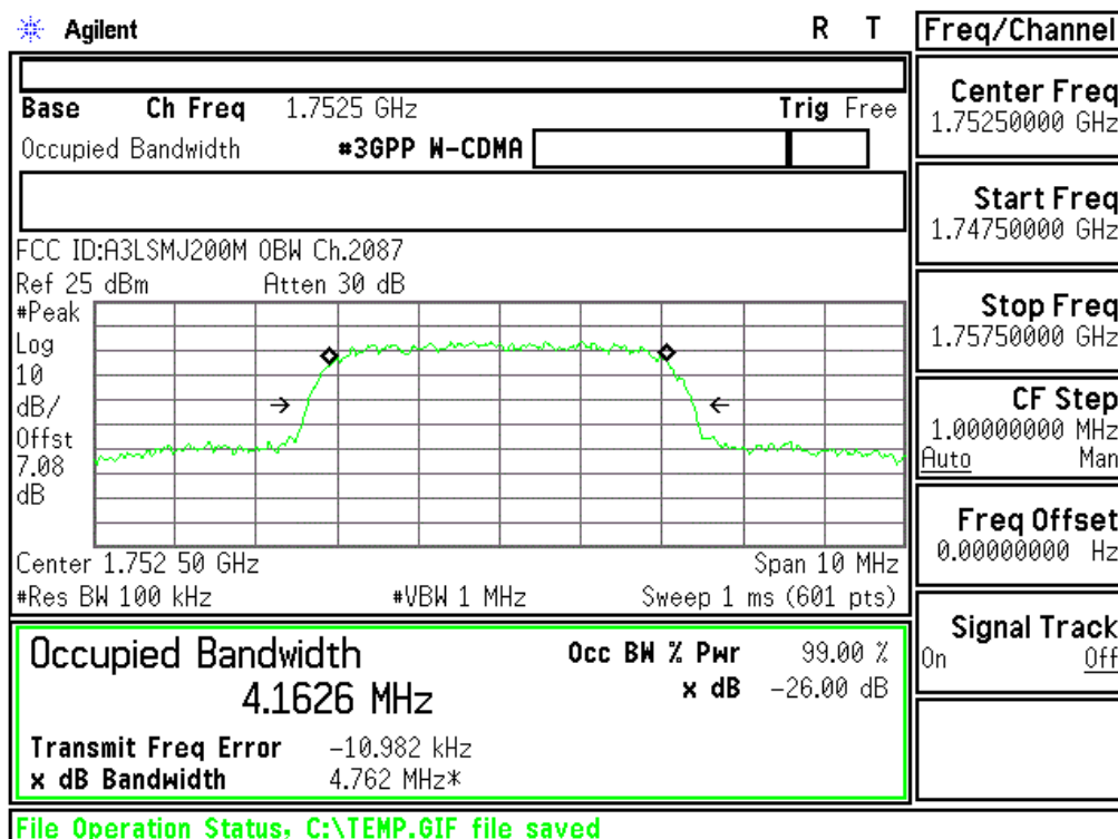
Plot 6-4. Occupied Bandwidth Plot (AWS WCDMA Mode - Ch.1862(DL2087))
