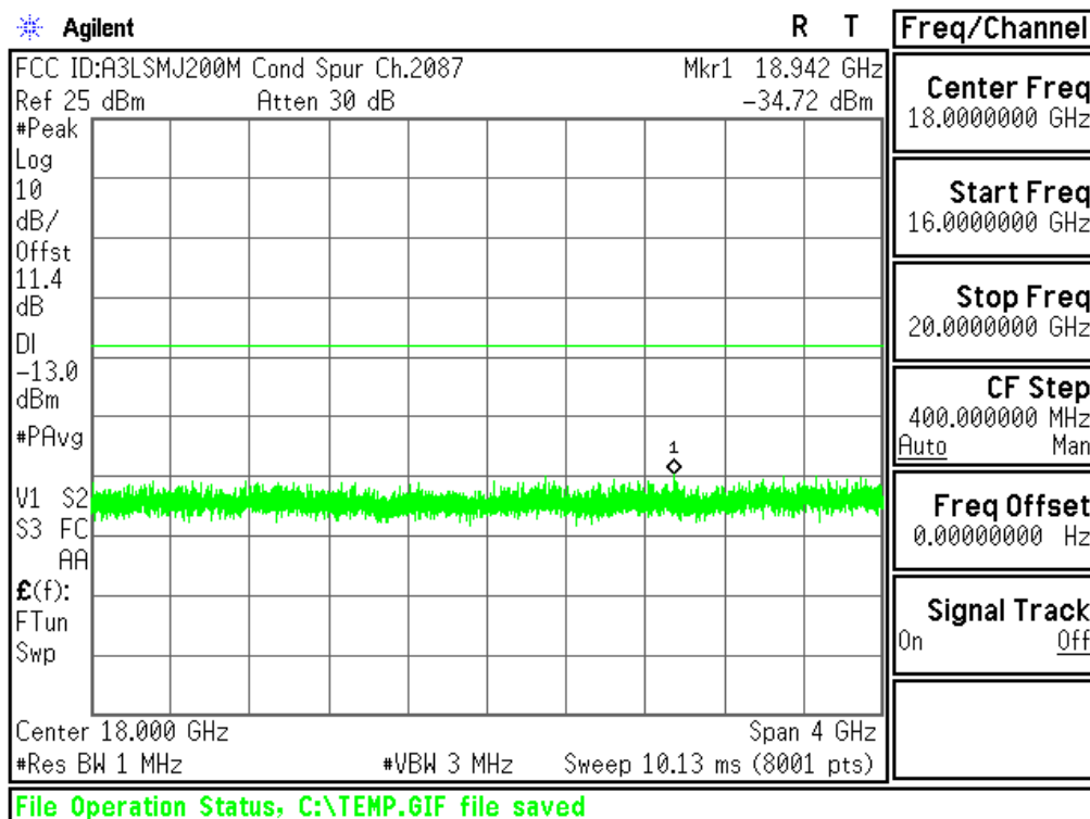
Plot 6-53. Conducted Spurious Plot (AWS WCDMA Mode - Ch.1862(DL2087))
