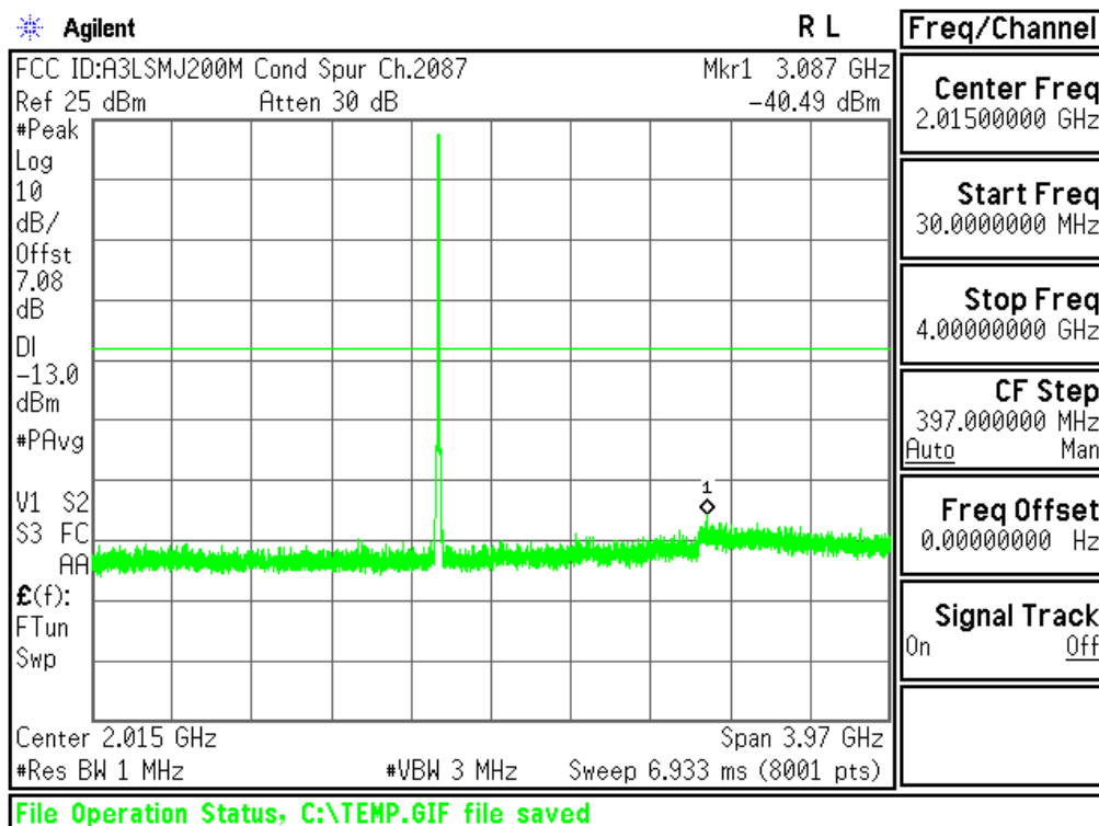
Plot 6-49. Conducted Spurious Plot (AWS WCDMA Mode - Ch.1862(DL2087))
