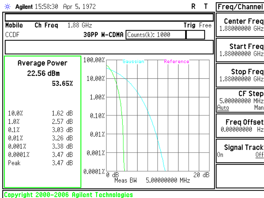
Plot 6-90. Peak-Average Ratio Plot (PCS WCDMA Mode - Ch.9400(DL9800))
