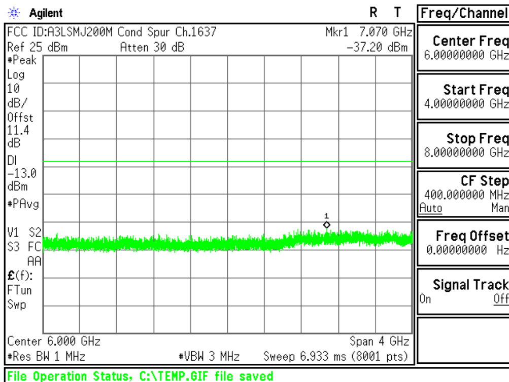
Plot 6-45. Conducted Spurious Plot (AWS WCDMA Mode - Ch.1412(DL1637))
