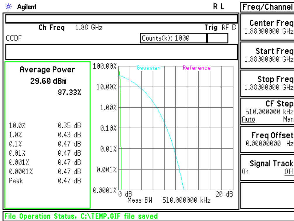
Plot 6-89. Peak-Average Ratio Plot (PCS GSM Mode - Ch.661)
