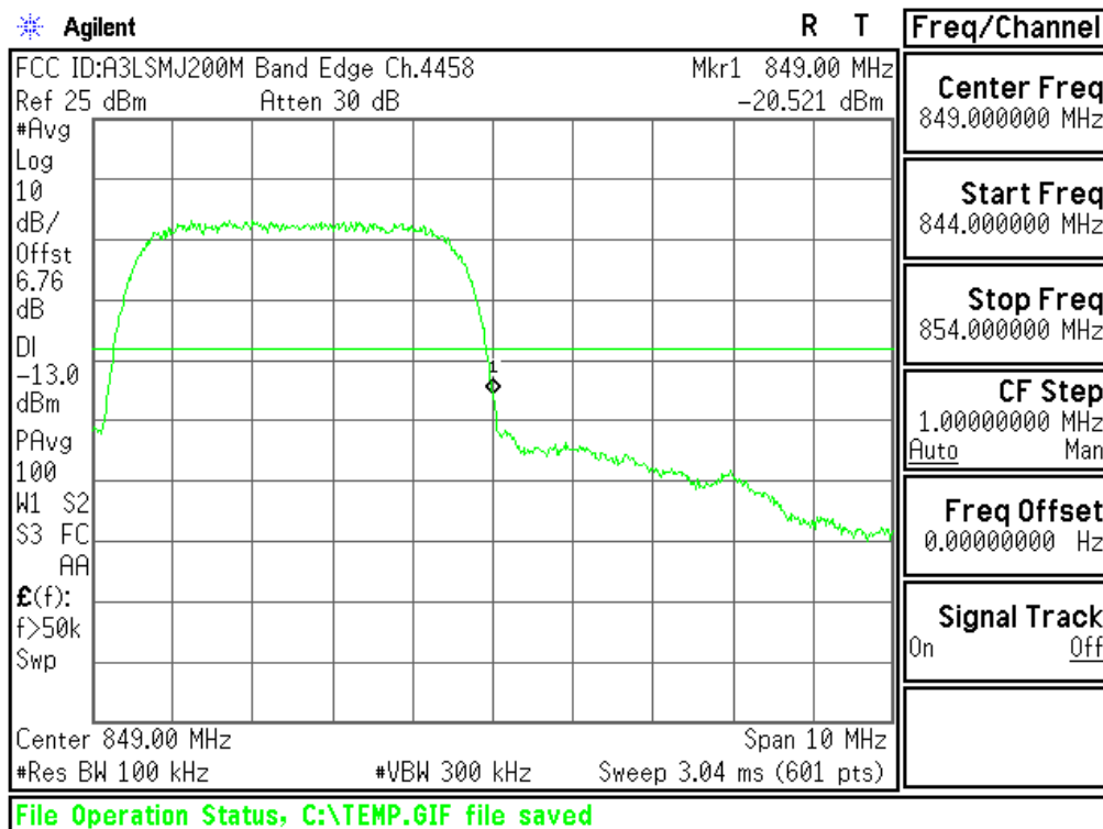
Plot 6-79. Upper Band Edge Plot (Cellular WCDMA Mode - Ch.4233(DL4458))
