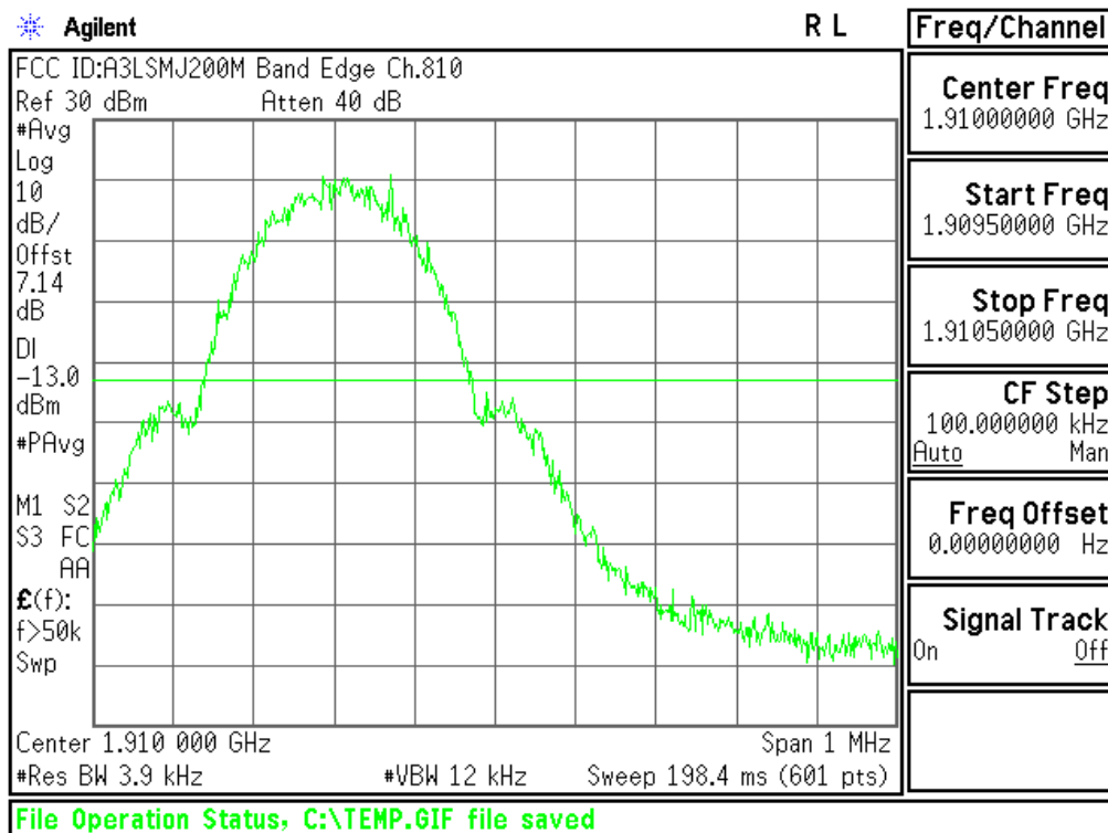
Plot 6-75. Upper Band Edge Plot (PCS GSM Mode – Ch.810)
