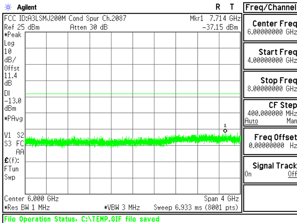
Plot 6-50. Conducted Spurious Plot (AWS WCDMA Mode - Ch. 1862(DL2087))
