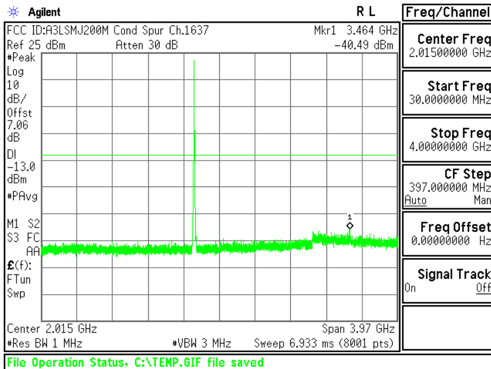
Plot 6-44. Conducted Spurious Plot (AWS WCDMA Mode - Ch.1412(DL1637))
