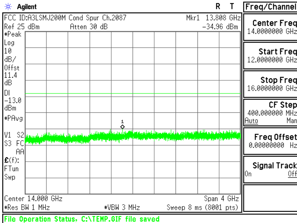
Plot 6-52. Conducted Spurious Plot (AWS WCDMA Mode - Ch.1862(DL2087))
