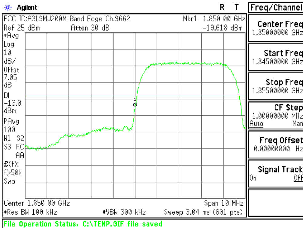
Plot 6-85. Lower Band Edge Plot (PCS WCDMA Mode - Ch.9262(DL9662))
