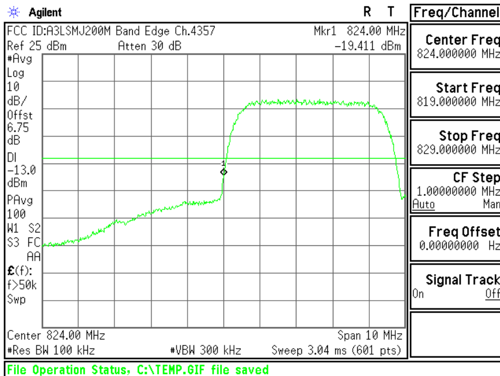
Plot 6-77. Lower Band Edge Plot (Cellular WCDMA Mode - Ch.4132(DL4357))
