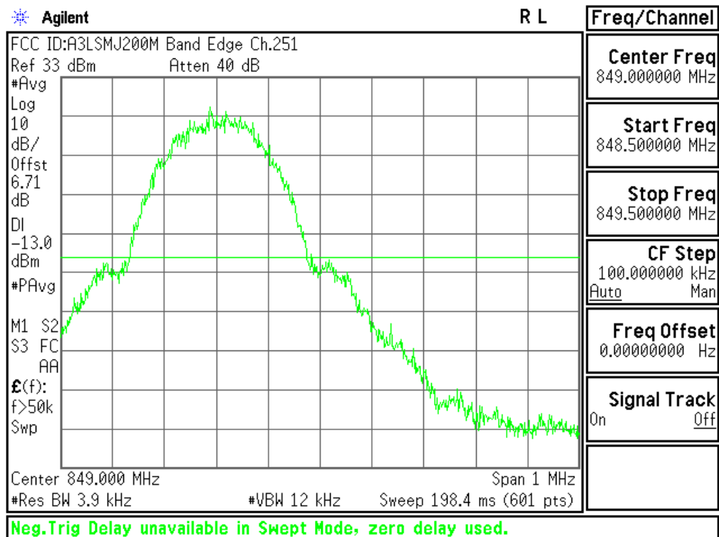
Plot 6-71. Upper Band Edge Plot (Cellular GSM Mode – Ch.251)
