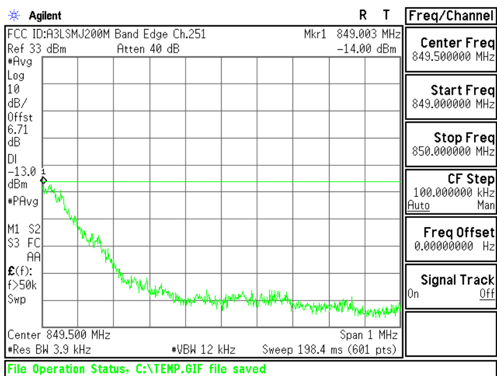
Plot 6-72. Upper Band Edge Plot (Cellular GSM Mode – Ch.251)
