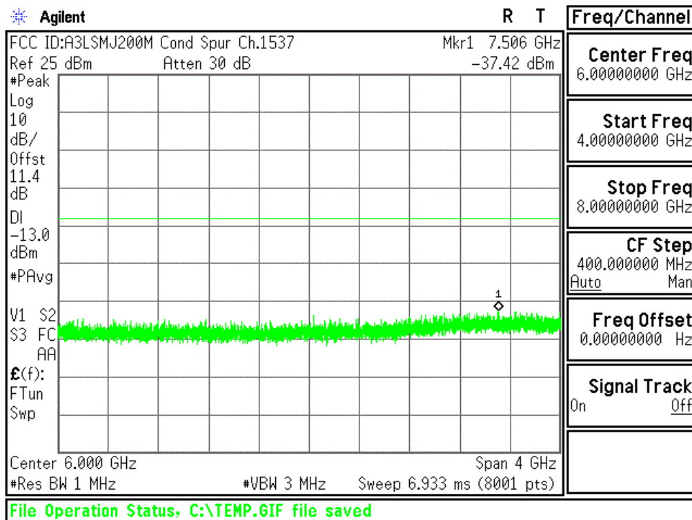
Plot 6-40. Conducted Spurious Plot (AWS WCDMA Mode - Ch.1312(DL1537))
