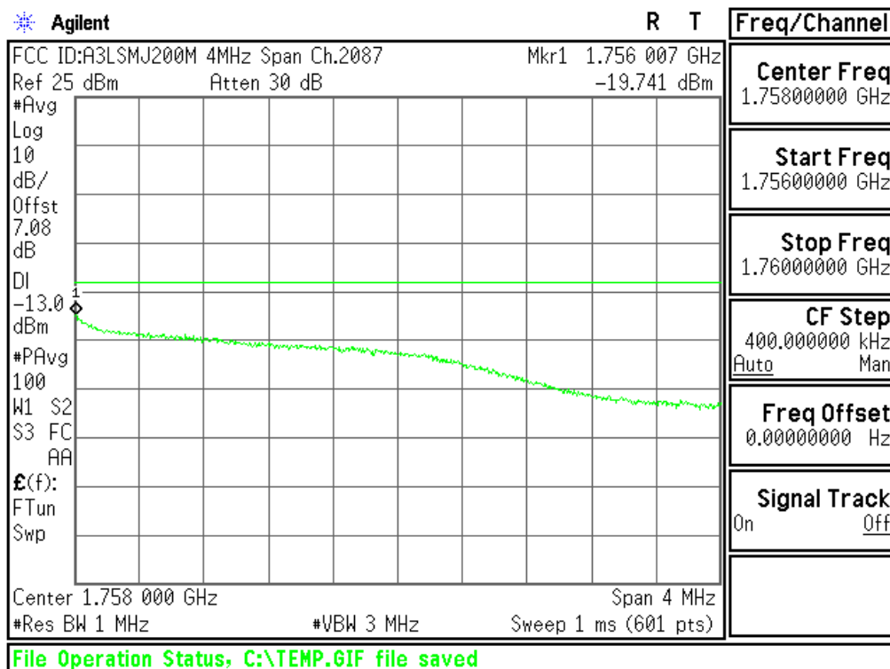
Plot 6-84. Extended Upper Band Edge Plot (AWS WCDMA Mode - Ch.1862(DL2087))
