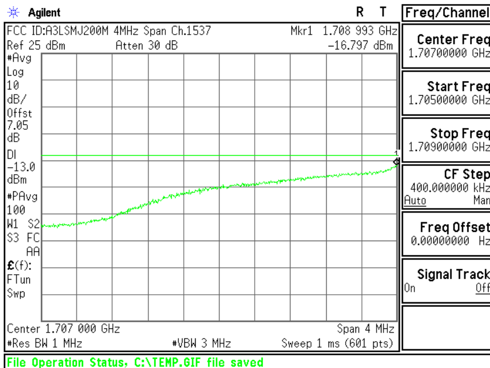
Plot 6-82. Extended Lower Band Edge Plot (AWS WCDMA Mode - Ch.1312(DL1537))
