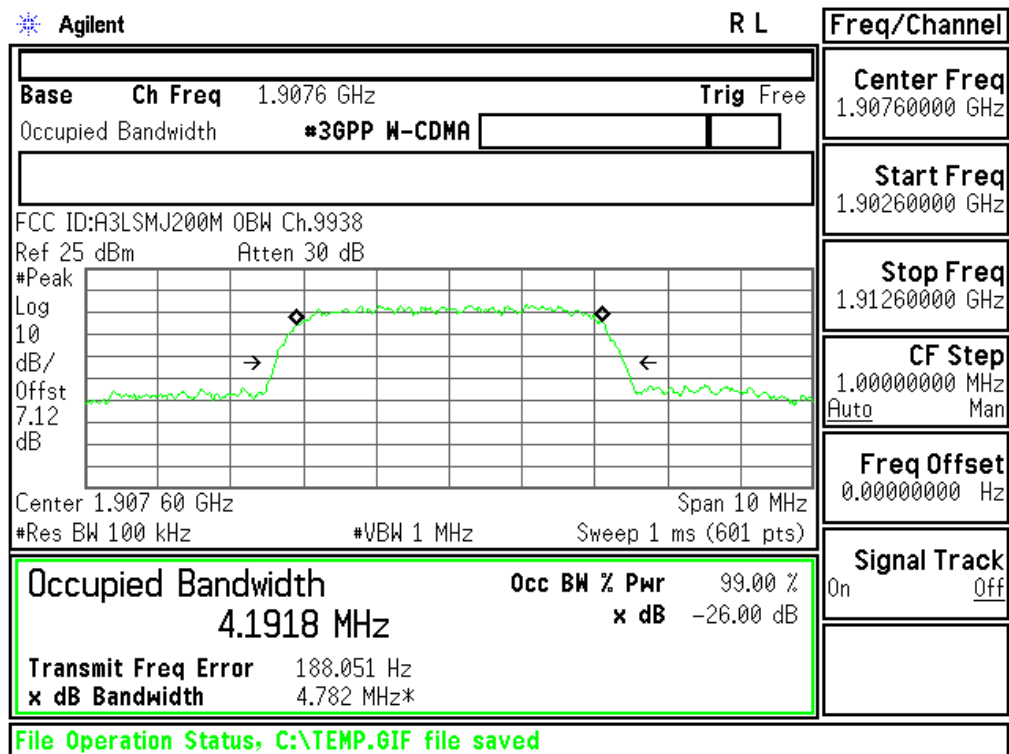
Plot 6-5. Occupied Bandwidth Plot (PCS WCDMA Mode - Ch.9538(DL9938))
