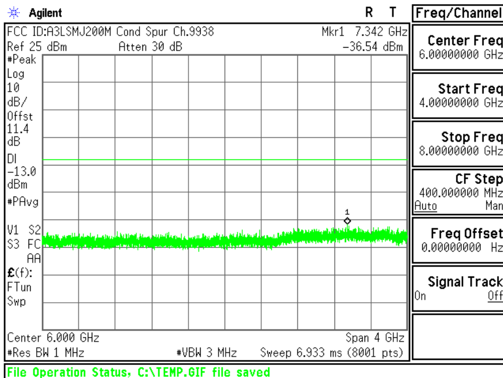
Plot 6-65. Conducted Spurious Plot (PCS WCDMA Mode - Ch.9538(DL9938))
