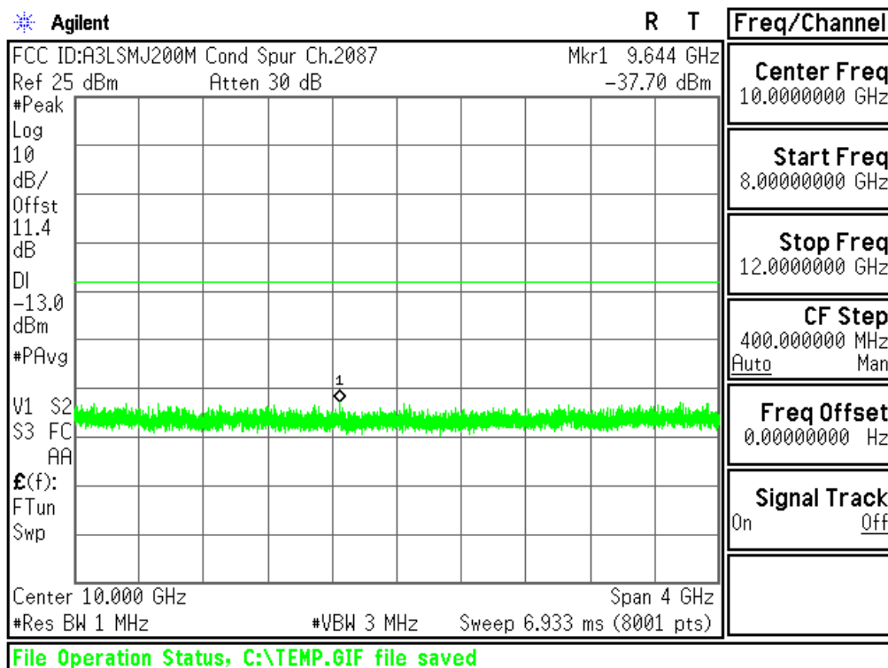
Plot 6-51. Conducted Spurious Plot (AWS WCDMA Mode - Ch. 1862(DL2087))
