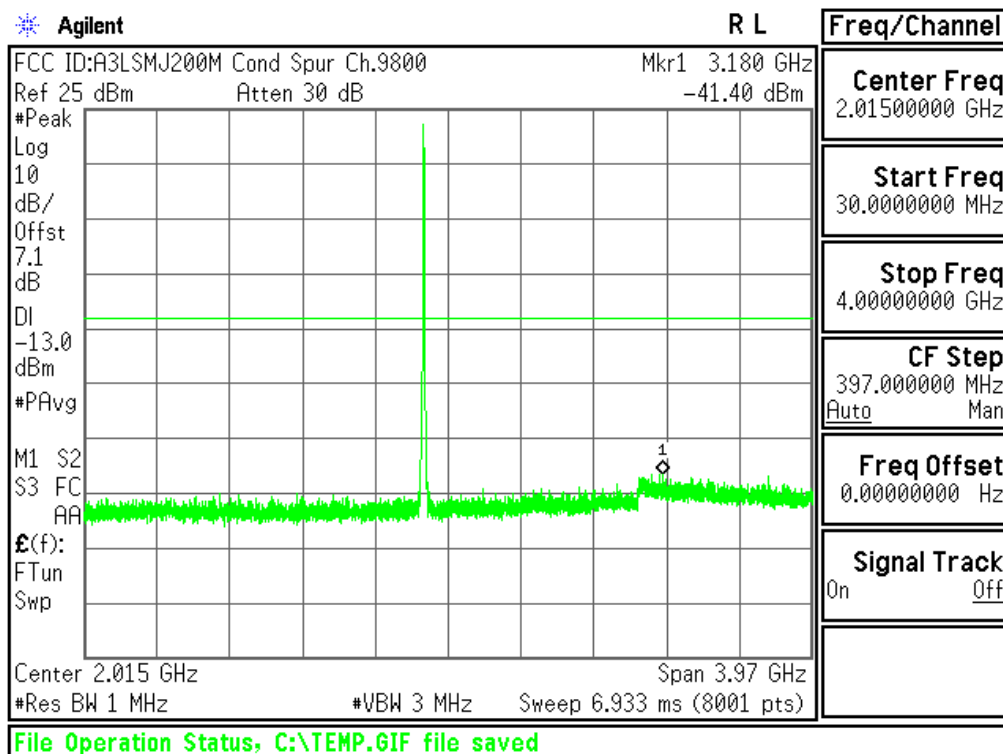
Plot 6-59. Conducted Spurious Plot (PCS WCDMA Mode - Ch.9400(DL9800))
