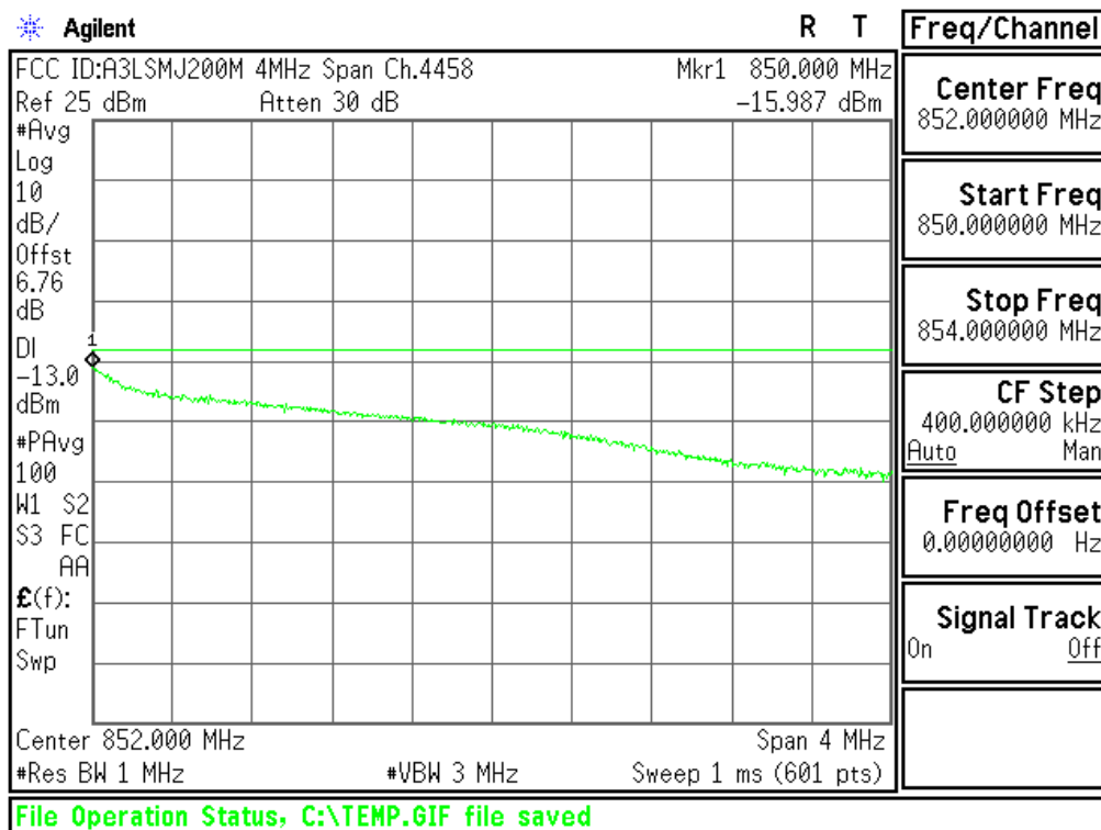
Plot 6-80. Extended Upper Band Edge Plot (Cellular WCDMA Mode - Ch.4233(DL4458))
