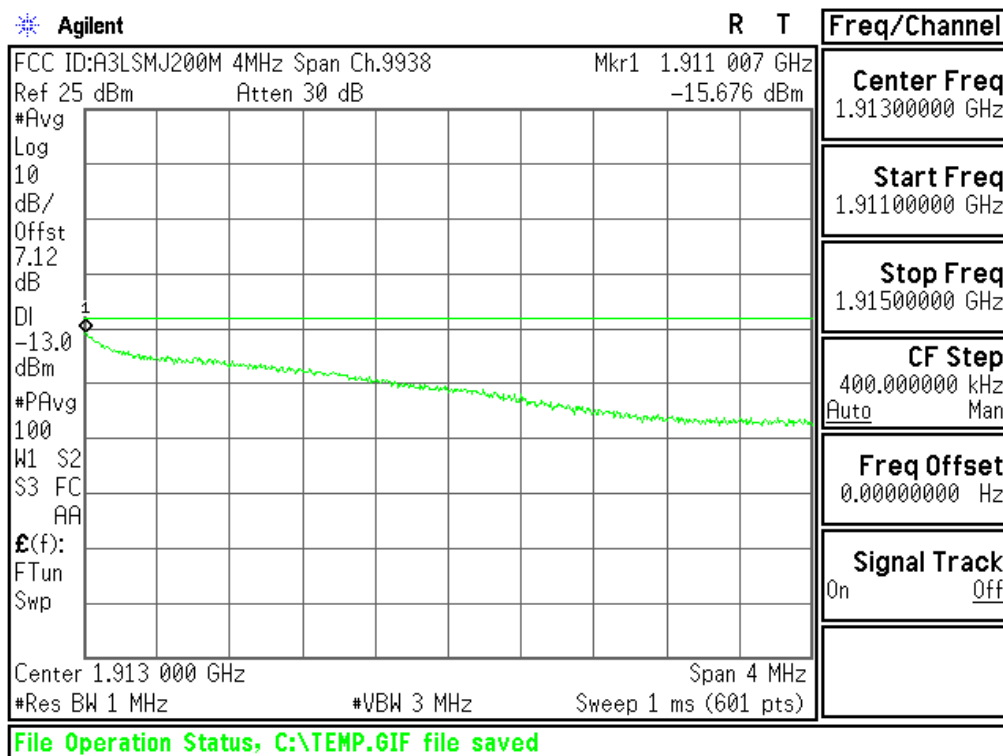
Plot 6-88. Extended Upper Band Edge Plot (PCS WCDMA Mode - Ch.9538(DL9938))
