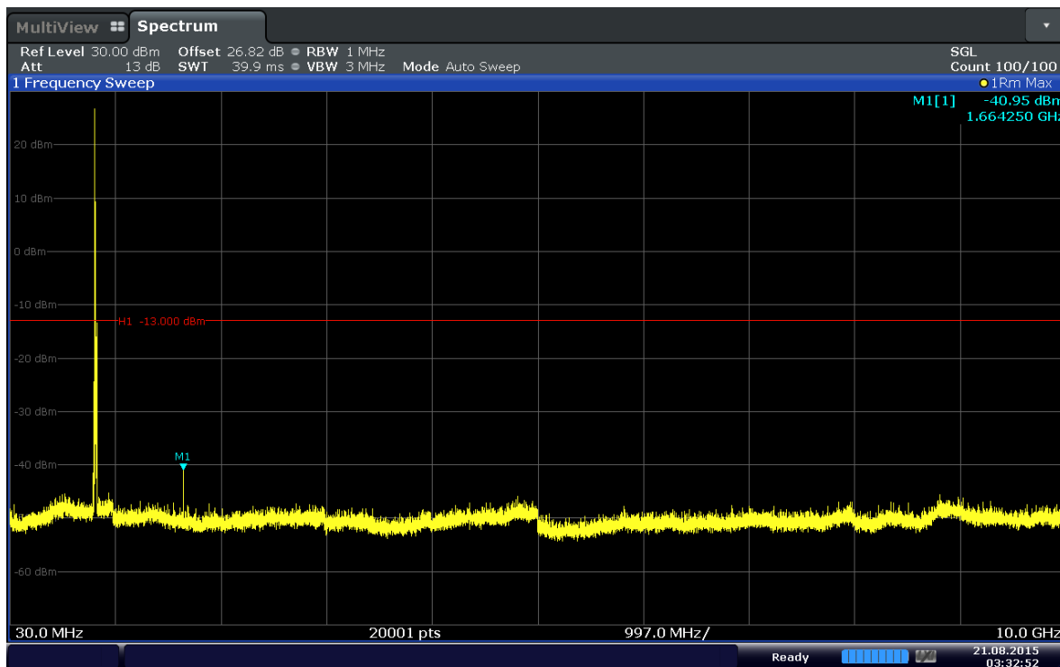
Plot 6-67. Conducted Spurious Plot (Band 5–10.0MHz–QPSK–RB Size 1–RB Offset 0–Ch.20525)
