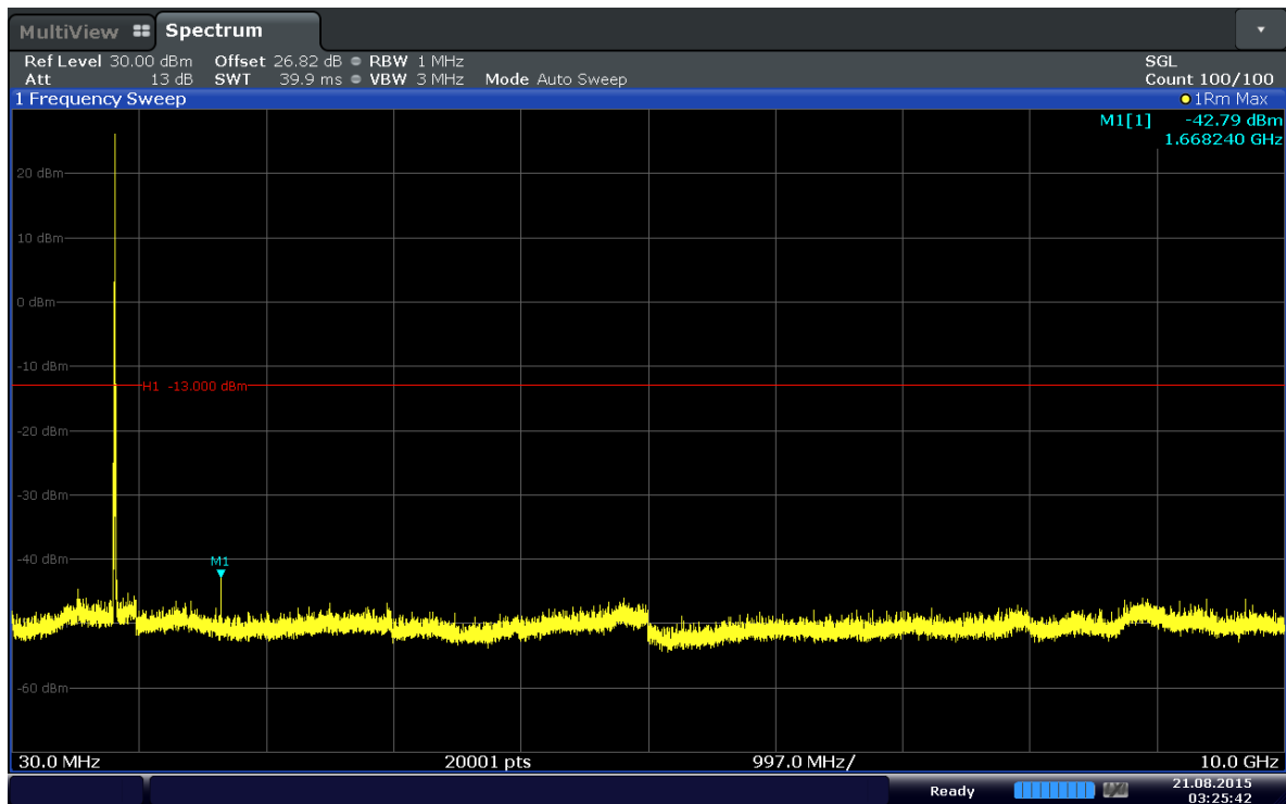
Plot 6-64. Conducted Spurious Plot (Band 5–5.0MHz–QPSK–RB Size 1–RB Offset 0–Ch.20525)
