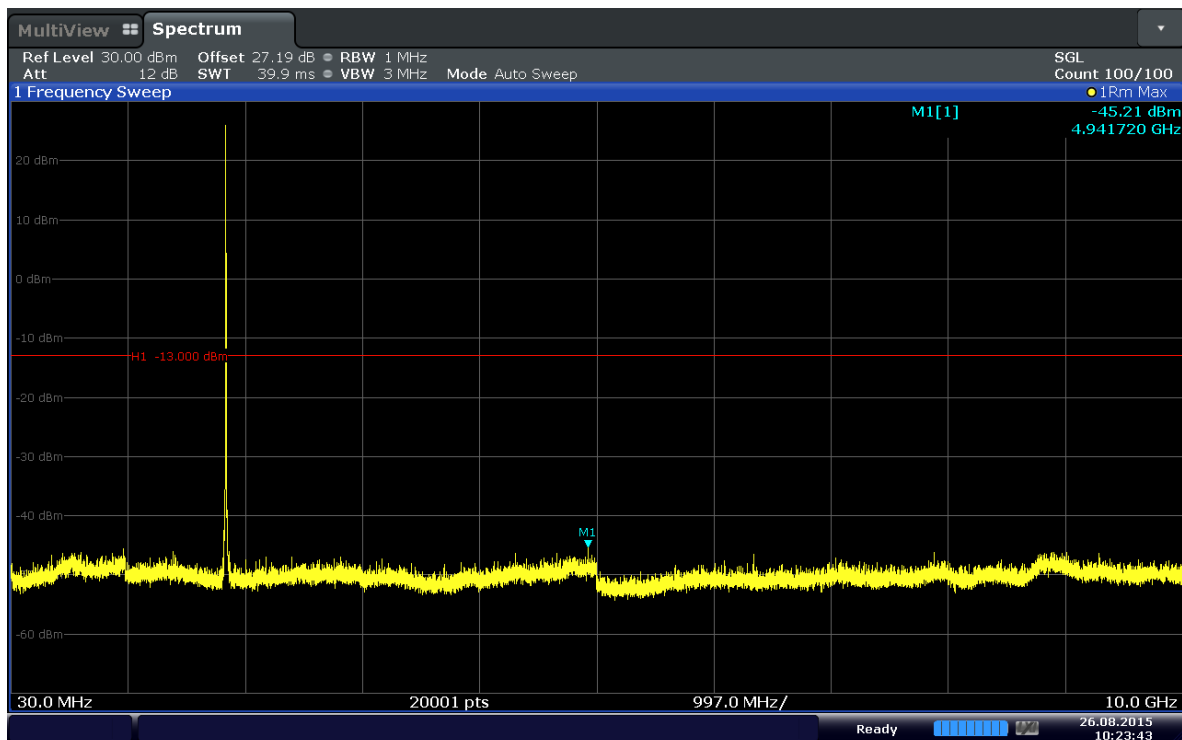
Plot 6-45. Conducted Spurious Plot (Band 2–15.0MHz–QPSK–RB Size 1–RB Offset 37–Ch.18675)
