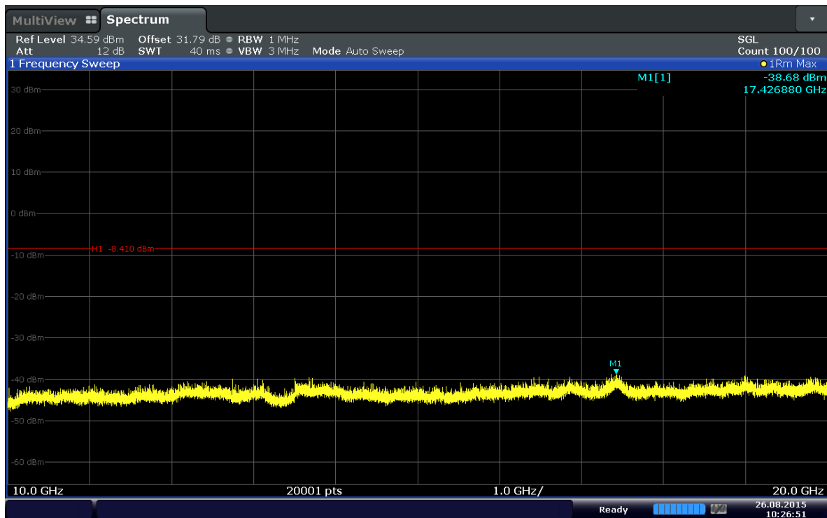
Plot 6-50. Conducted Spurious Plot (Band 2–15.0MHz–QPSK–RB Size 1–RB Offset 74–Ch.19125)
