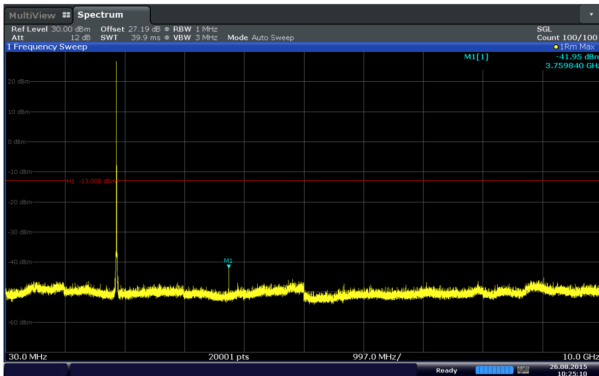
Plot 6-47. Conducted Spurious Plot (Band 2–15.0MHz–QPSK–RB Size 1–RB Offset 37–Ch.18900)
