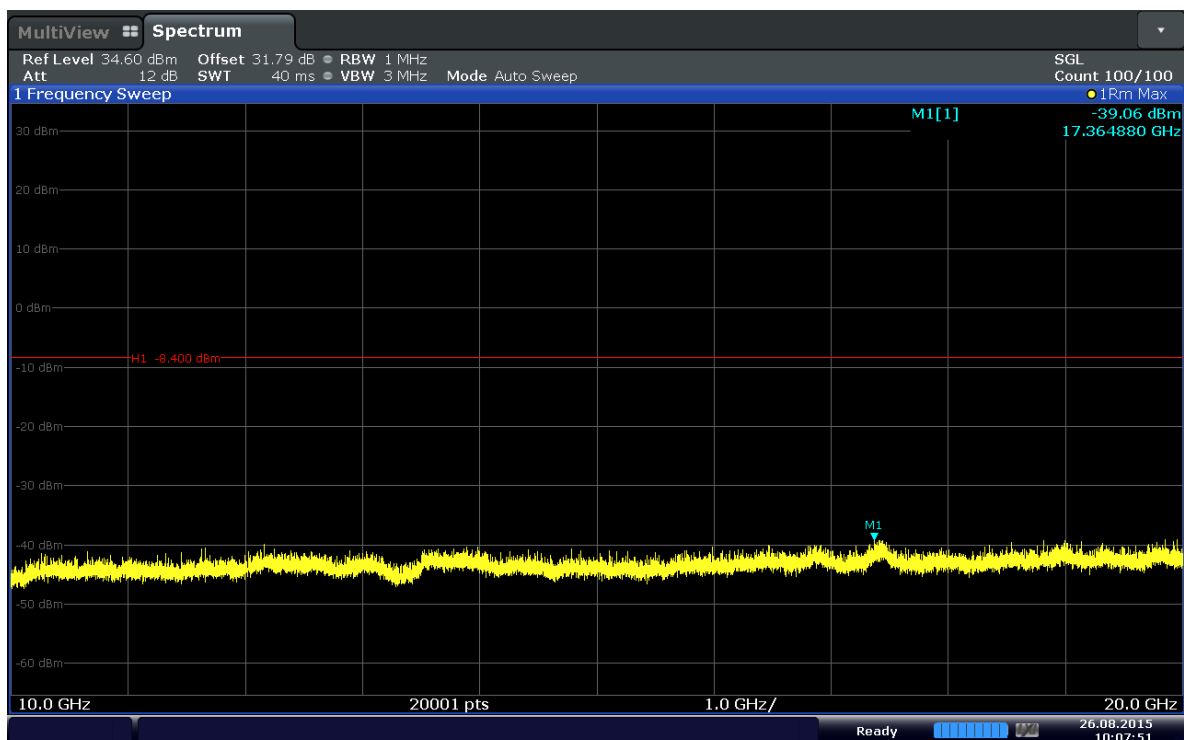
Plot 6-21. Conducted Spurious Plot (Band 2–1.4MHz–QPSK–RB Size 1–RB Offset 2–Ch.18607)
