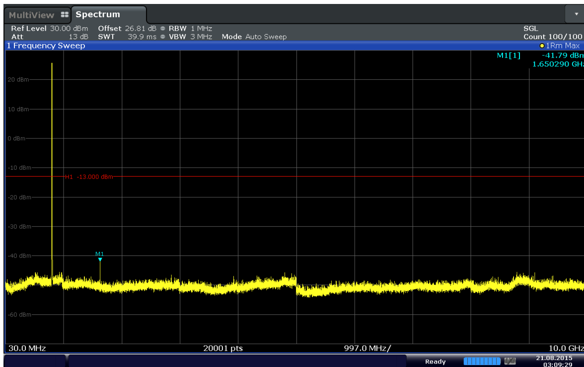
Plot 6-57. Conducted Spurious Plot (Band 5–1.4MHz–QPSK–RB Size 1–RB Offset 5–Ch.20407)
