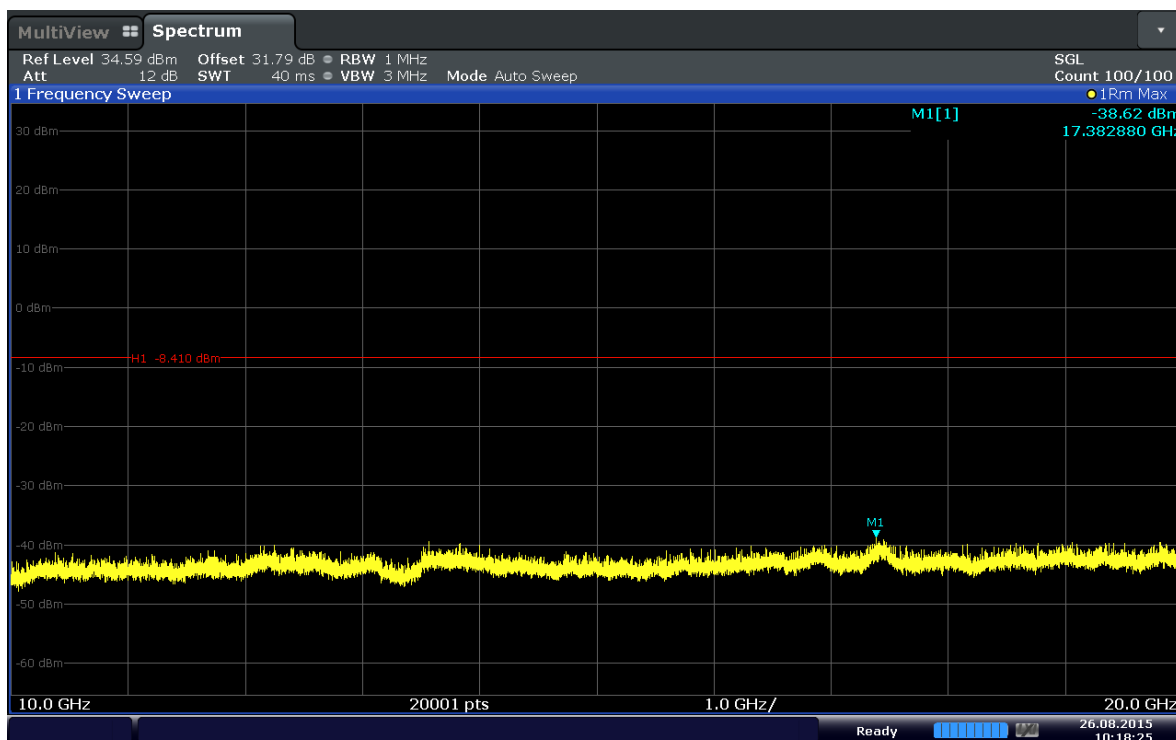
Plot 6-38. Conducted Spurious Plot (Band 2–5.0MHz–QPSK–RB Size 1–RB Offset 24–Ch.19175)
