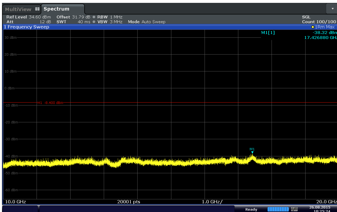
Plot 6-48. Conducted Spurious Plot (Band 2–15.0MHz–QPSK–RB Size 1–RB Offset 37–Ch.18900)
