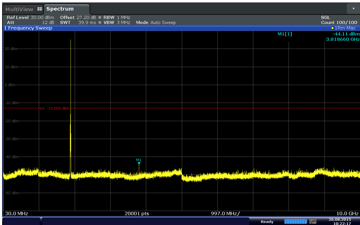
Plot 6-43. Conducted Spurious Plot (Band 2–10.0MHz–QPSK–RB Size 1–RB Offset 49–Ch.19150)
