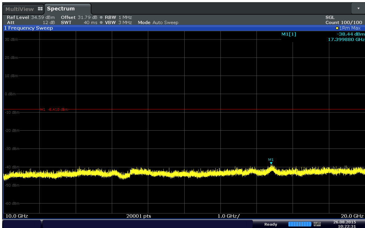
Plot 6-44. Conducted Spurious Plot (Band 2–10.0MHz–QPSK–RB Size 1–RB Offset 49–Ch.19150)
