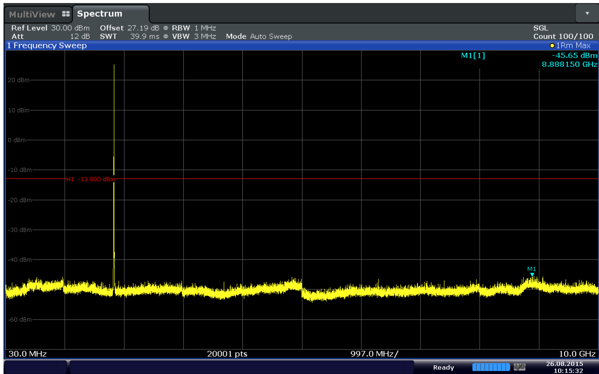
Plot 6-33. Conducted Spurious Plot (Band 2–5.0MHz–QPSK–RB Size 1–RB Offset 12–Ch.18625)
