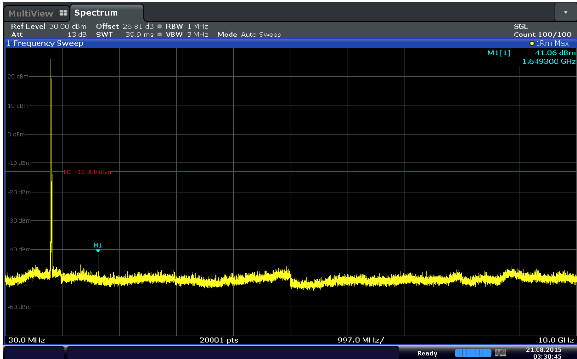
Plot 6-66. Conducted Spurious Plot (Band 5–10.0MHz–QPSK–RB Size 1–RB Offset 0–Ch.20450)
