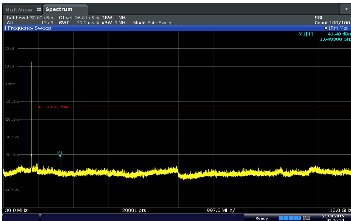
Plot 6-60. Conducted Spurious Plot (Band 5–3.0MHz–QPSK–RB Size 1–RB Offset 0–Ch.20415)
