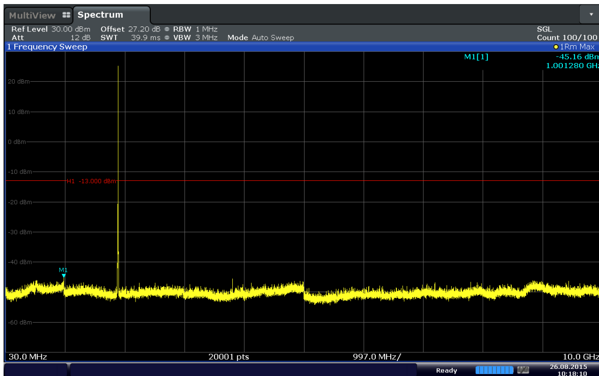
Plot 6-37. Conducted Spurious Plot (Band 2–5.0MHz–QPSK–RB Size 1–RB Offset 24–Ch.19175)
