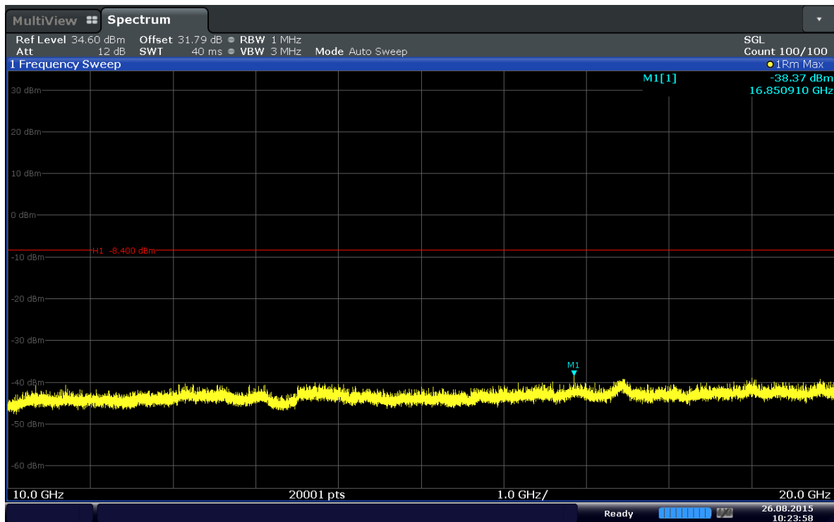
Plot 6-46. Conducted Spurious Plot (Band 2–15.0MHz–QPSK–RB Size 1–RB Offset 37–Ch.18675)
