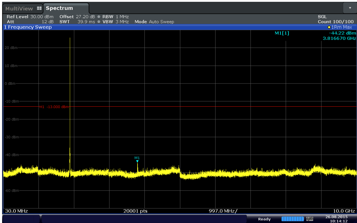
Plot 6-31. Conducted Spurious Plot (Band 2–3.0MHz–QPSK–RB Size 1–RB Offset 7–Ch.19185)
