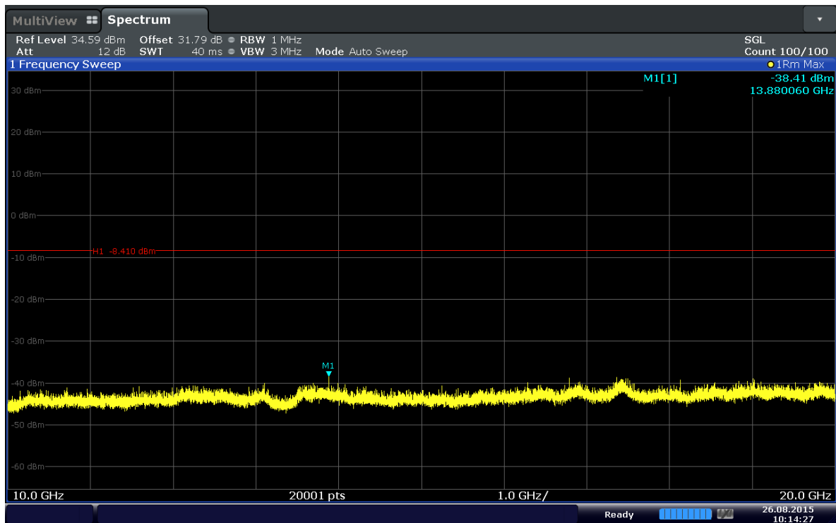
Plot 6-32. Conducted Spurious Plot (Band 2–3.0MHz–QPSK–RB Size 1–RB Offset 7–Ch.19185)
