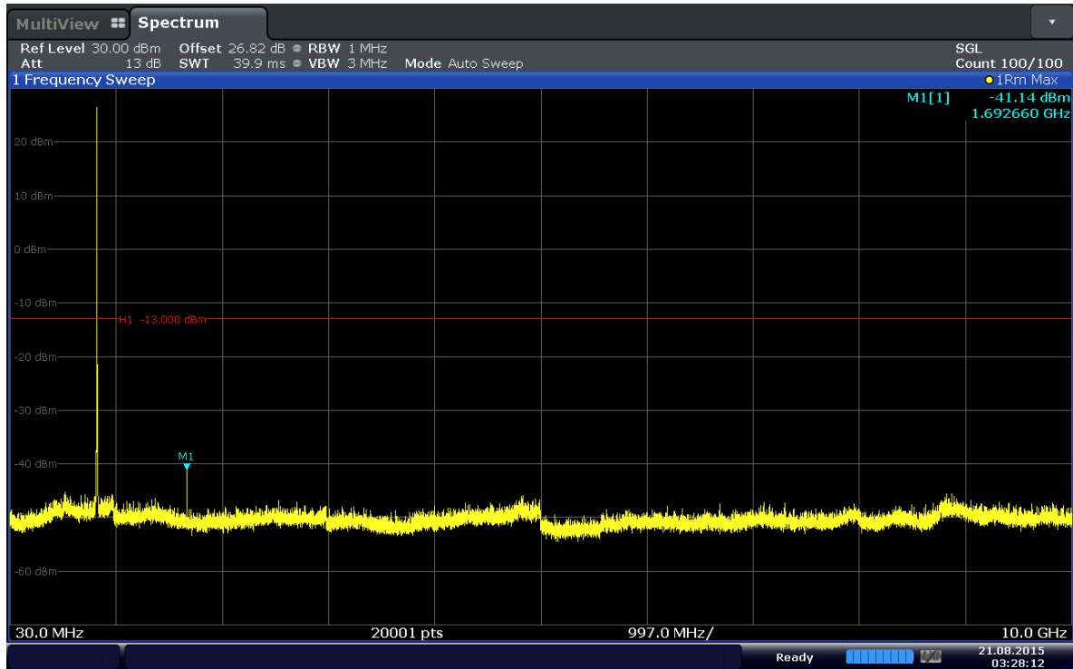
Plot 6-65. Conducted Spurious Plot (Band 5–5.0MHz–QPSK–RB Size 1–RB Offset 12–Ch.20625)
