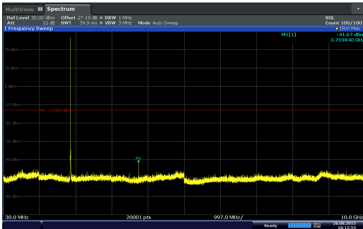
Plot 6-29. Conducted Spurious Plot (Band 2–3.0MHz–QPSK–RB Size 1–RB Offset 7–Ch.18900)
