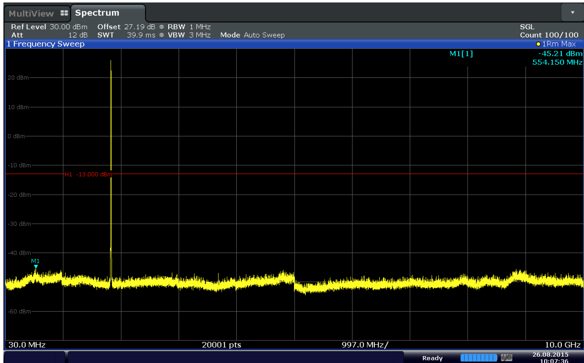
Plot 6-21. Conducted Spurious Plot (Band 2–1.4MHz–QPSK–RB Size 1–RB Offset 2–Ch.18607)
