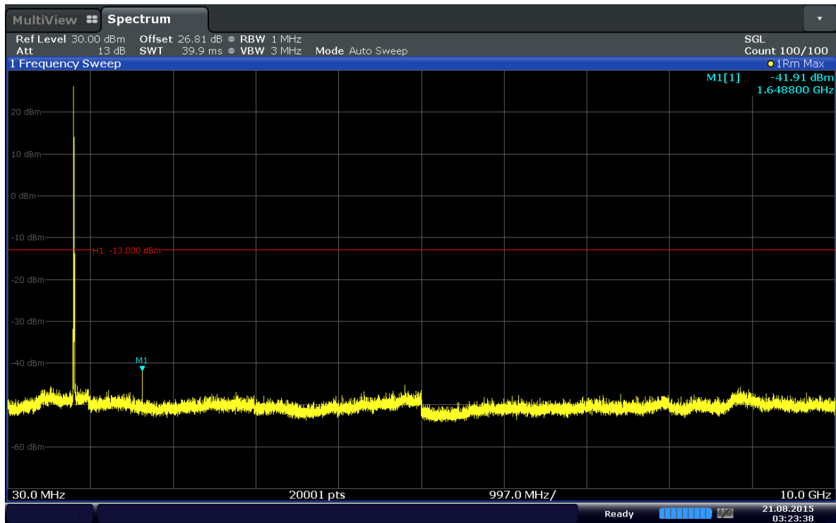
Plot 6-63. Conducted Spurious Plot (Band 5–5.0MHz–QPSK–RB Size 1–RB Offset 0–Ch.20425)
