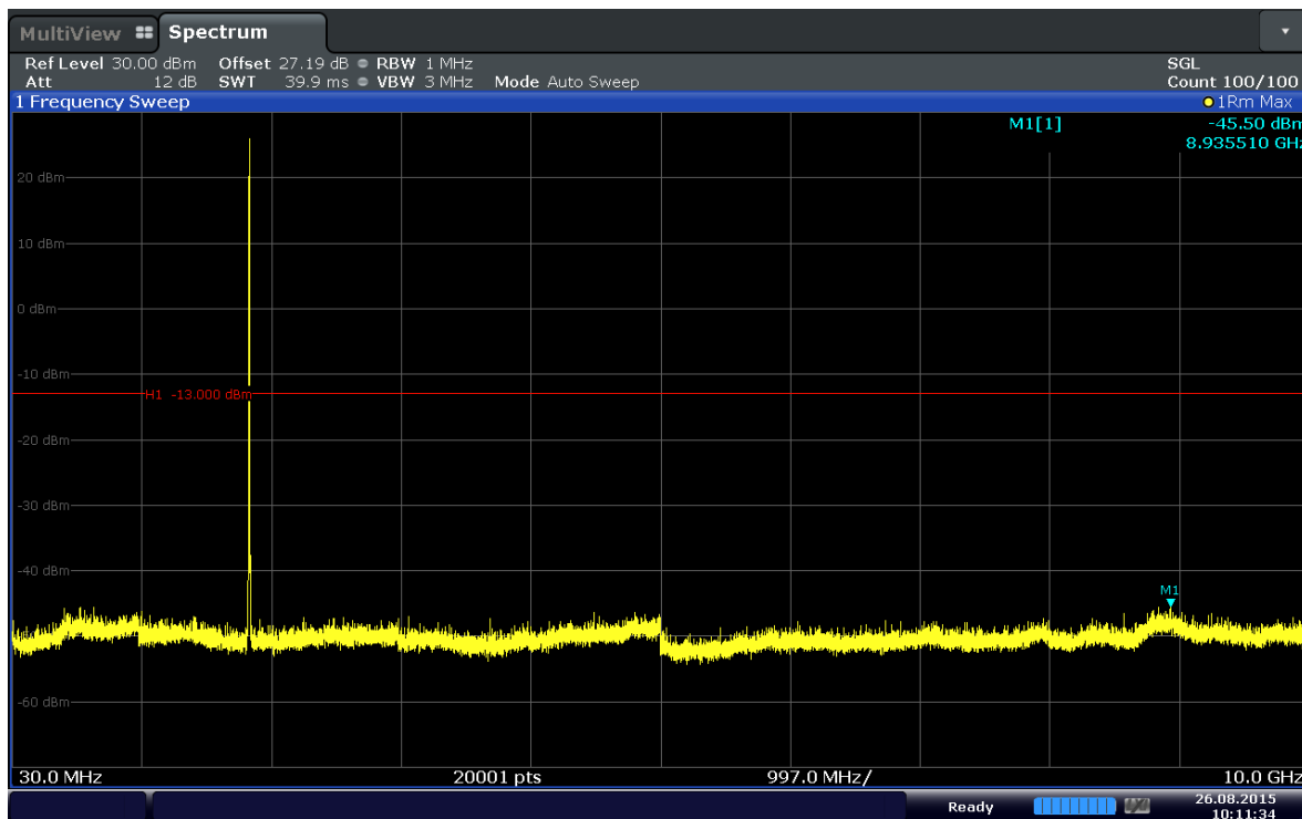
Plot 6-27. Conducted Spurious Plot (Band 2–3.0MHz–QPSK–RB Size 1–RB Offset 7–Ch.18615)
