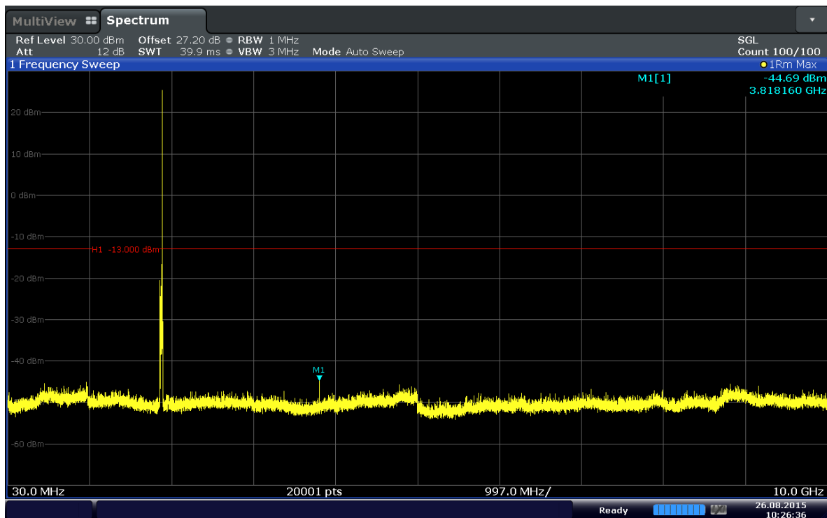
Plot 6-49. Conducted Spurious Plot (Band 2–15.0MHz–QPSK–RB Size 1–RB Offset 74–Ch.19125)
