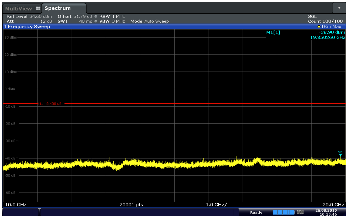
Plot 6-34. Conducted Spurious Plot (Band 2–5.0MHz–QPSK–RB Size 1–RB Offset 12–Ch.18625)
