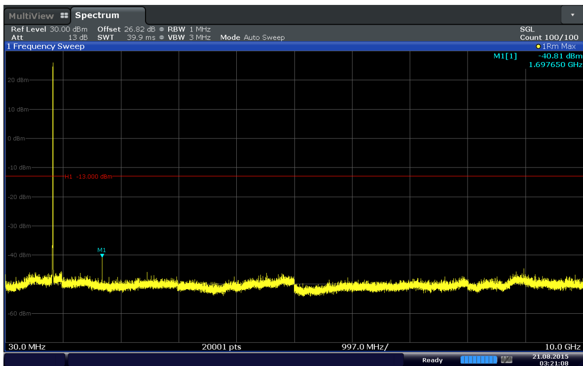
Plot 6-62. Conducted Spurious Plot (Band 5–3.0MHz–QPSK–RB Size 1–RB Offset 14–Ch.20635)
