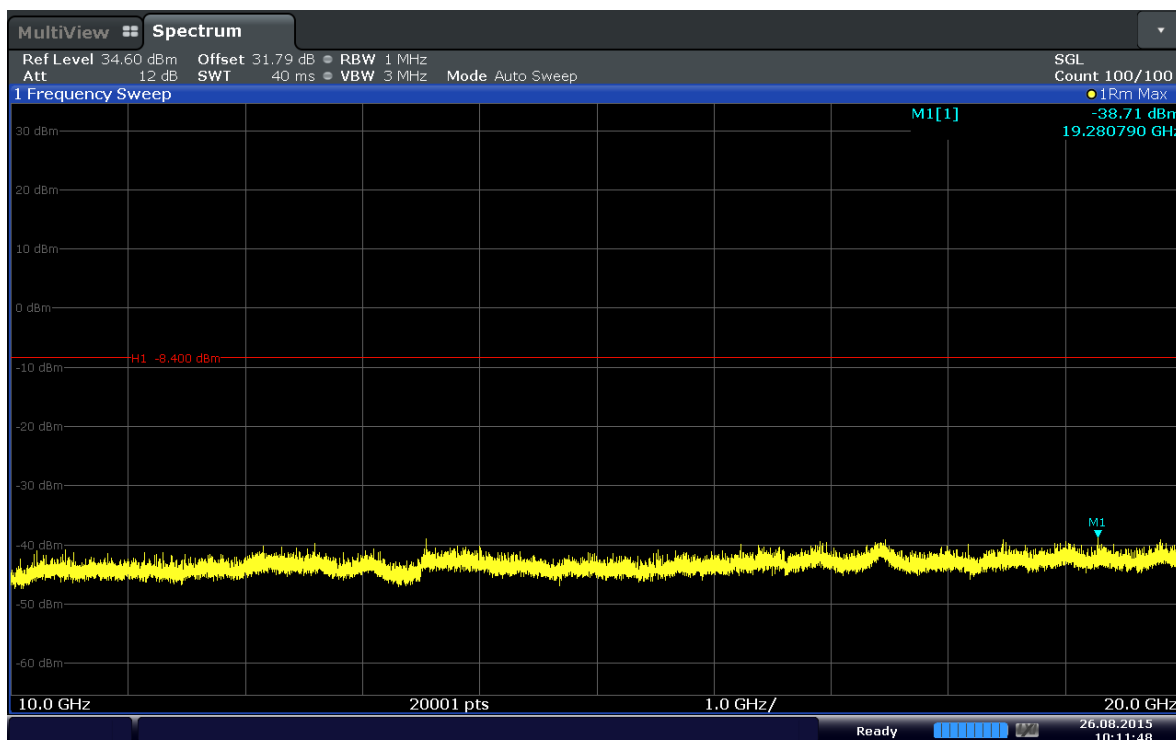
Plot 6-28. Conducted Spurious Plot (Band 2–3.0MHz–QPSK–RB Size 1–RB Offset 7–Ch.18615)
