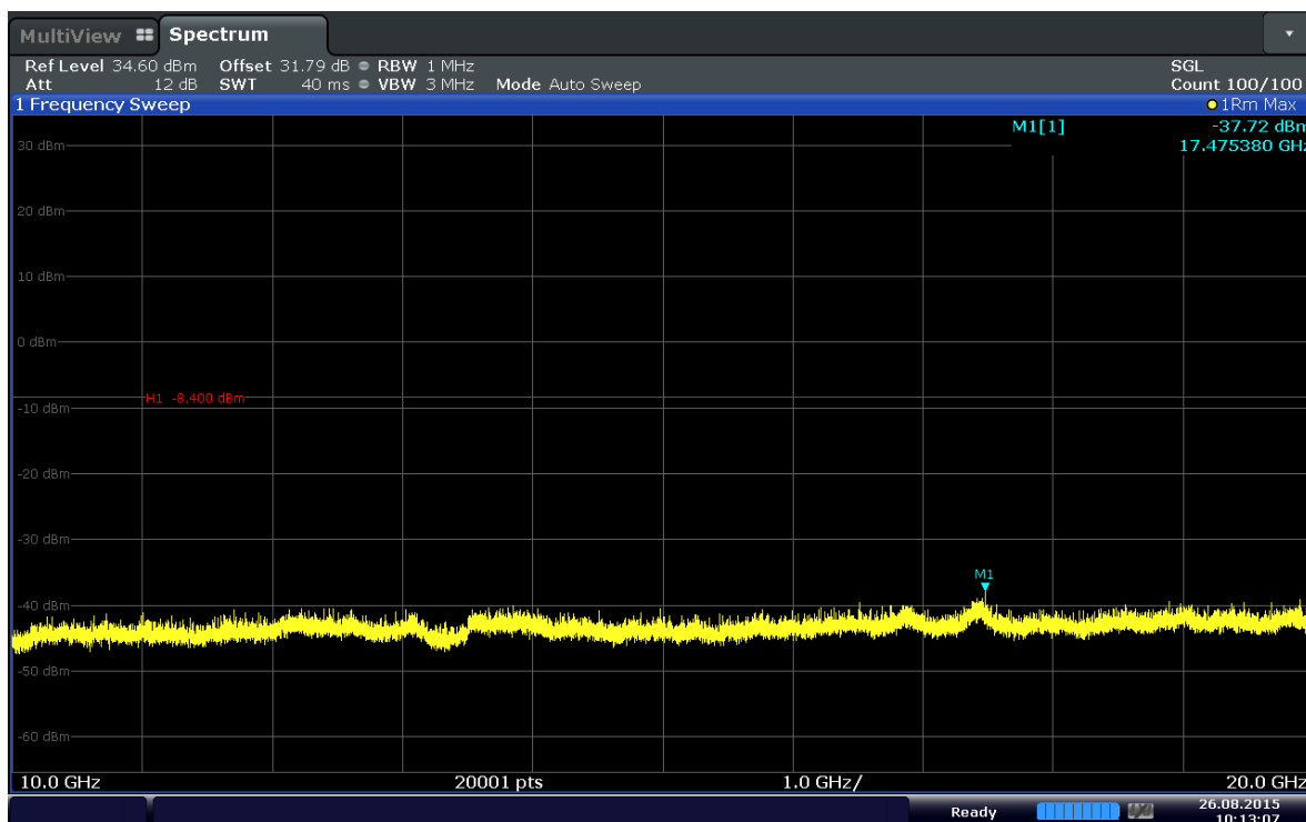
Plot 6-30. Conducted Spurious Plot (Band 2–3.0MHz–QPSK–RB Size 1–RB Offset 7–Ch.18900)
