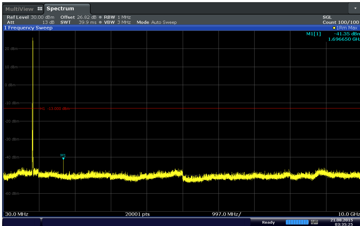
Plot 6-68. Conducted Spurious Plot (Band 5–10.0MHz–QPSK–RB Size 1–RB Offset 49–Ch.20600)
